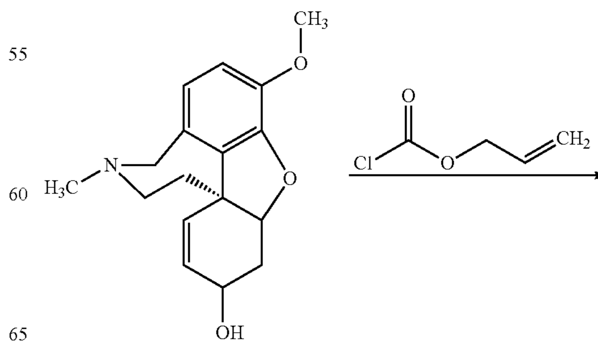
Scheme 27: Galanthamine
