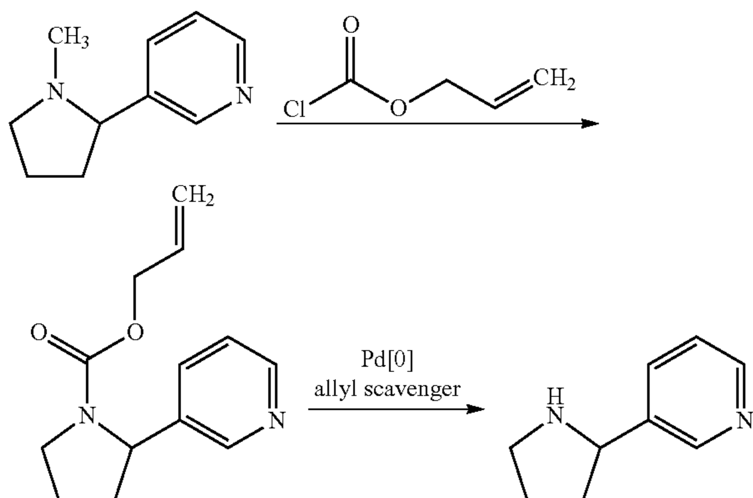
Scheme 28: Nicotine
