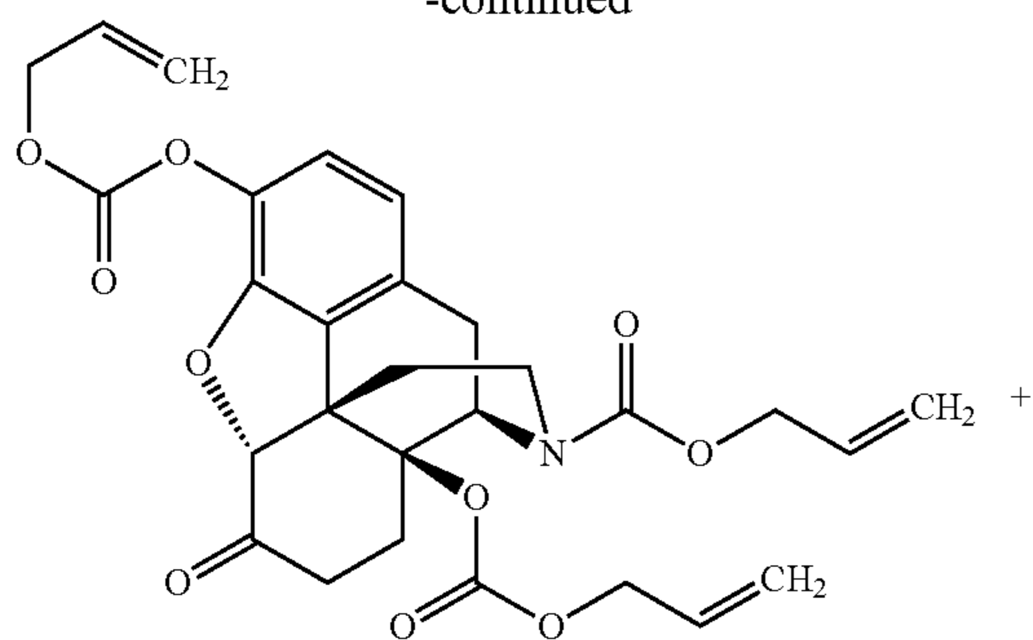
3, 14, 17-Tri-allyloxycarbonyl-noroxymorphone
