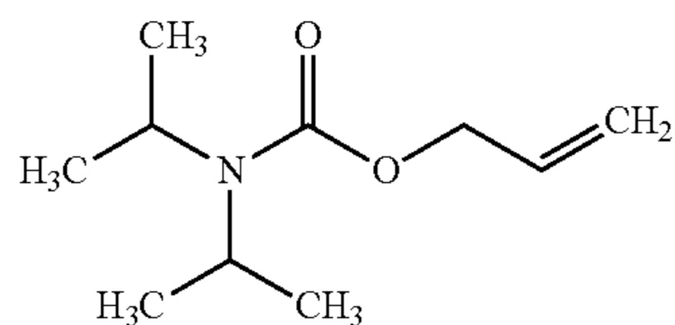
Allyl diisopropylcarbamate
