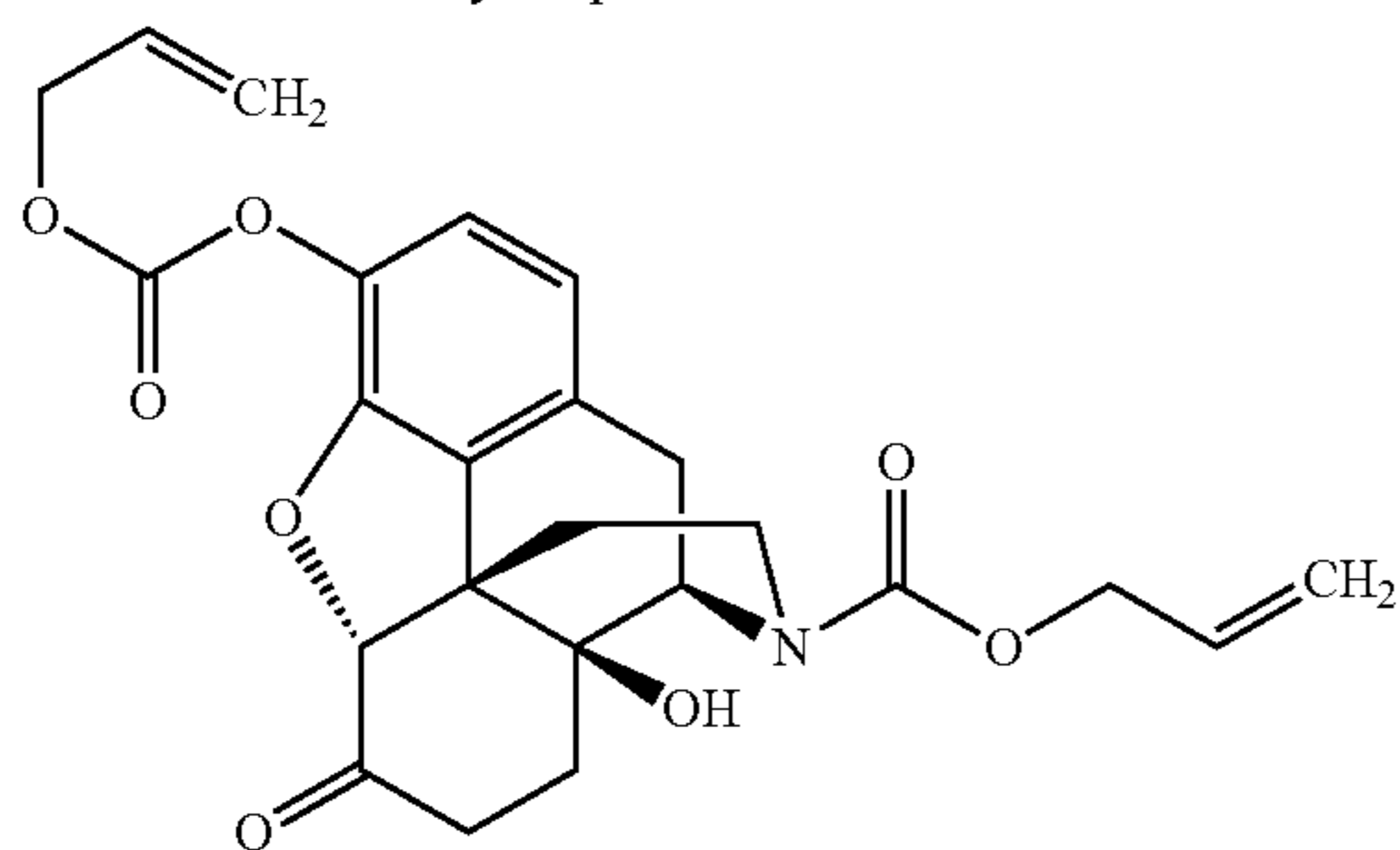
3, 17-Di-allyloxycarbonyl-noroxymorphone
