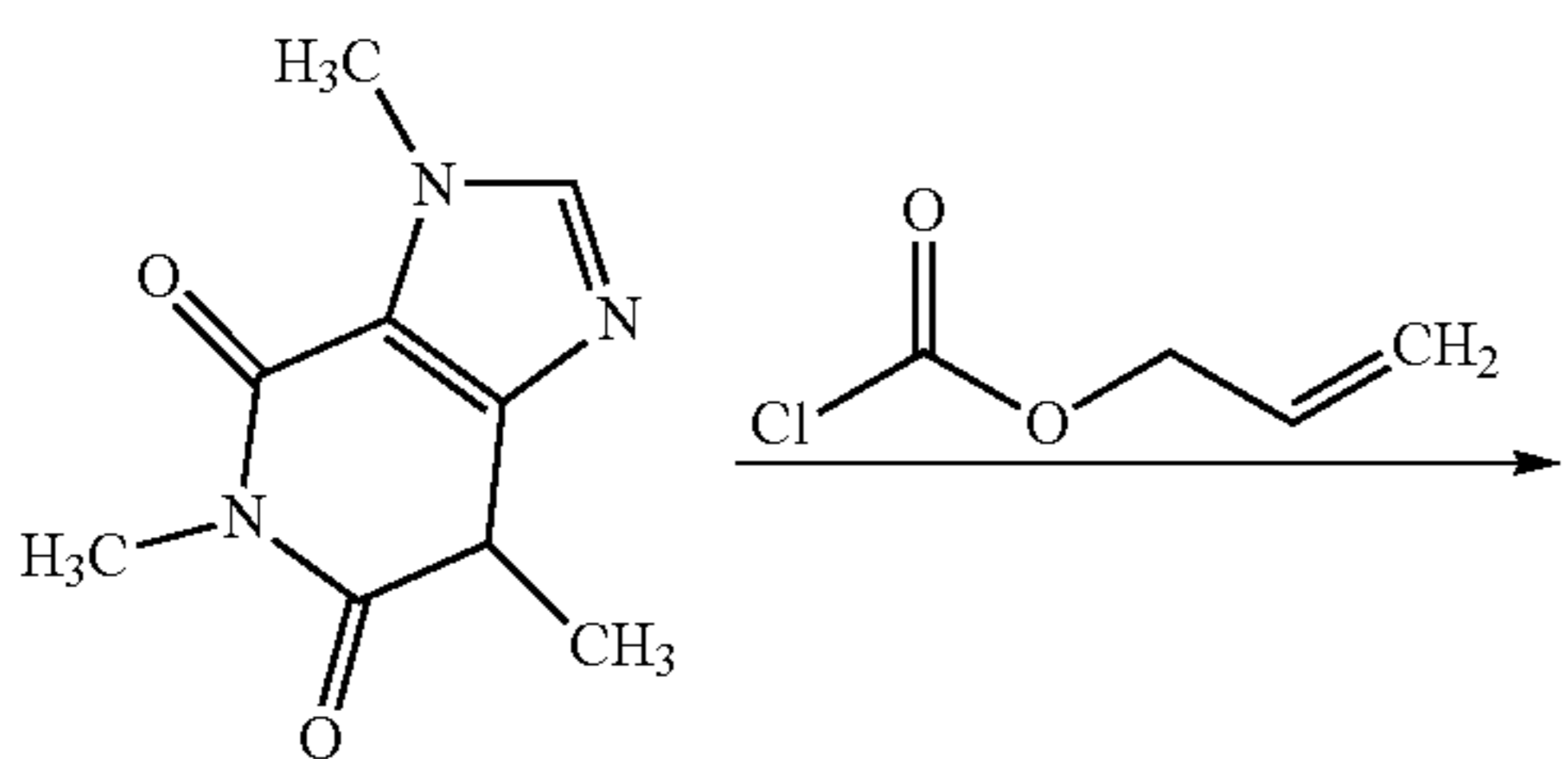
Scheme 25: Caffeine
