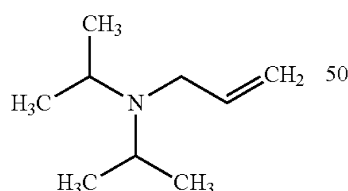
N,N-Diisopropylallylamine
