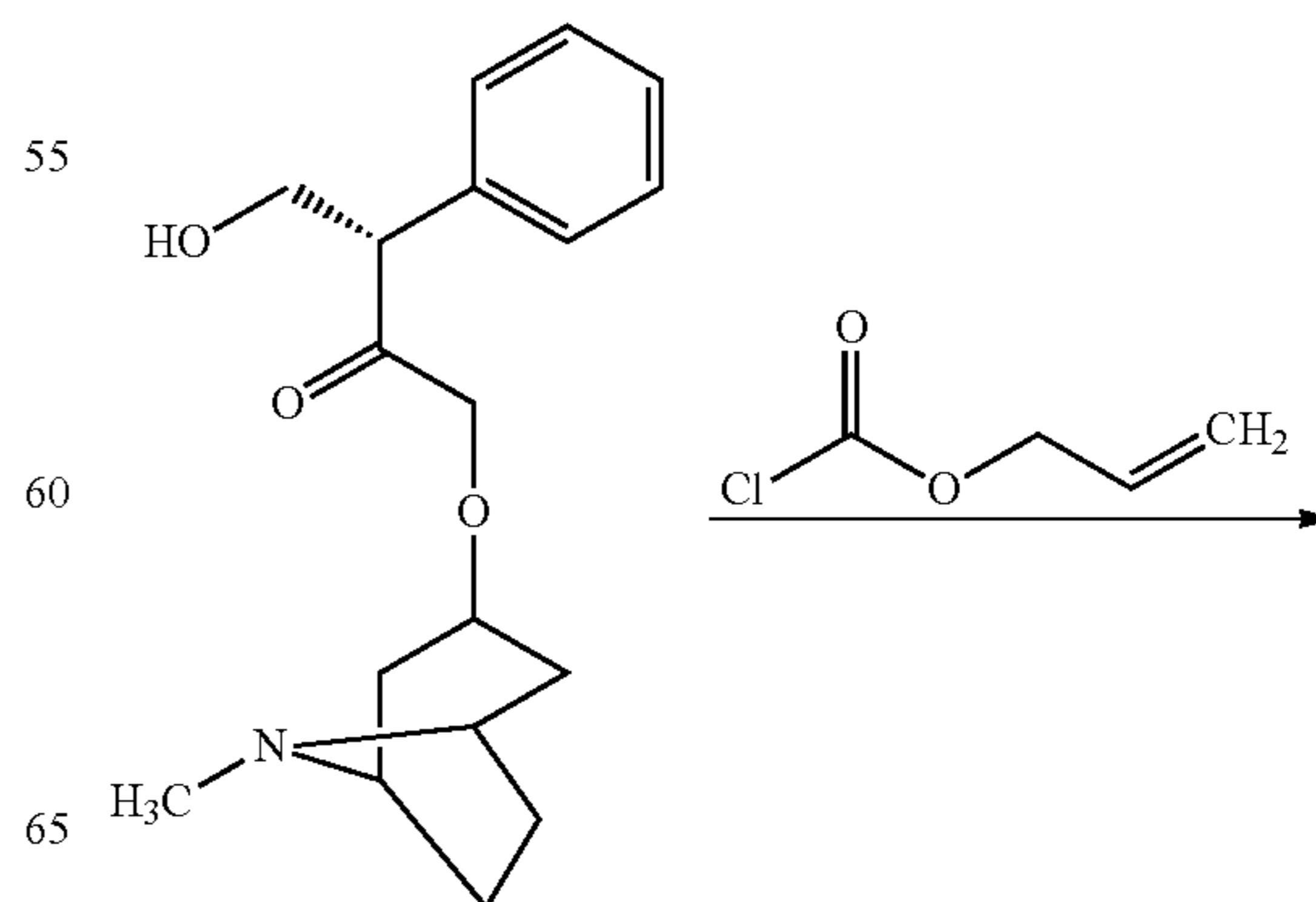
Scheme 24: Atropine
