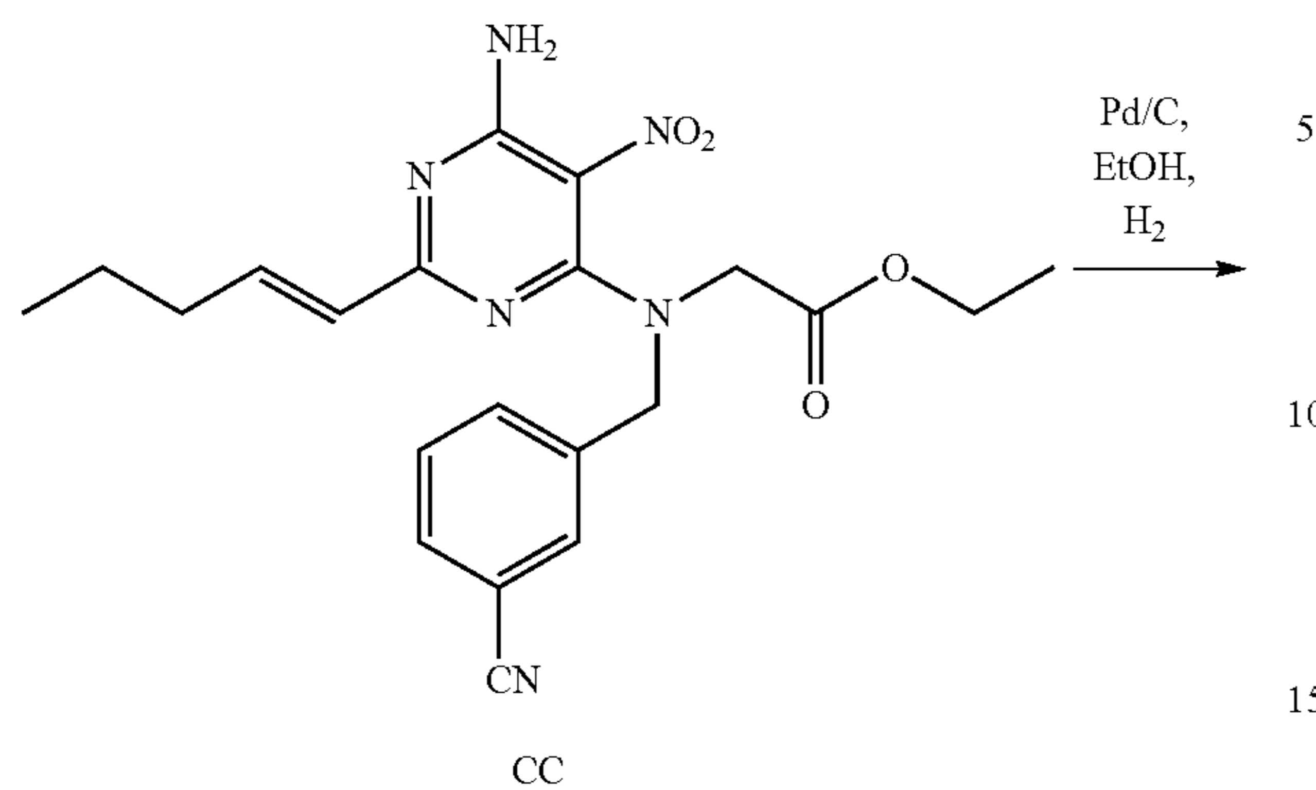
Scheme 51
