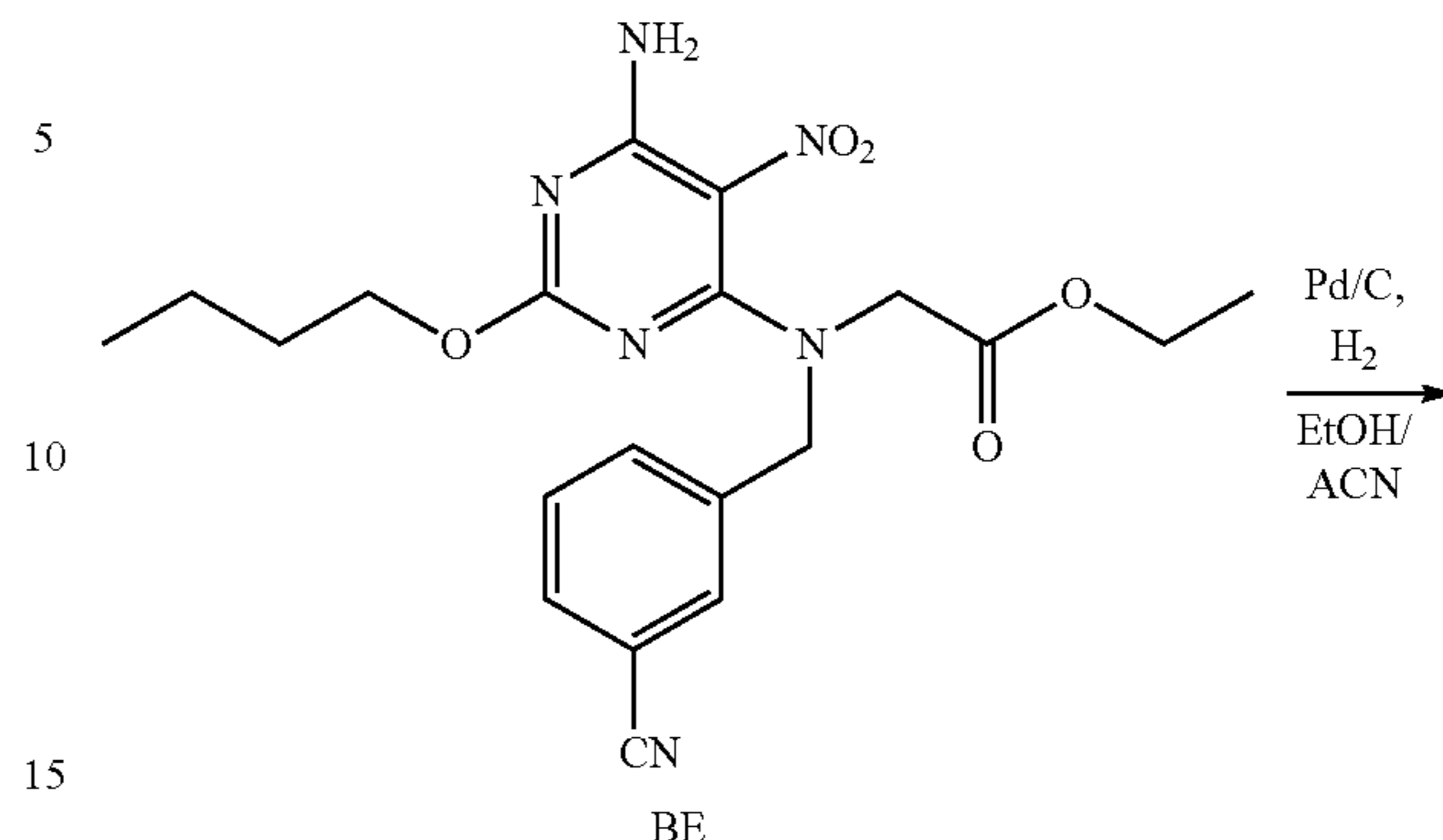
Scheme 23
