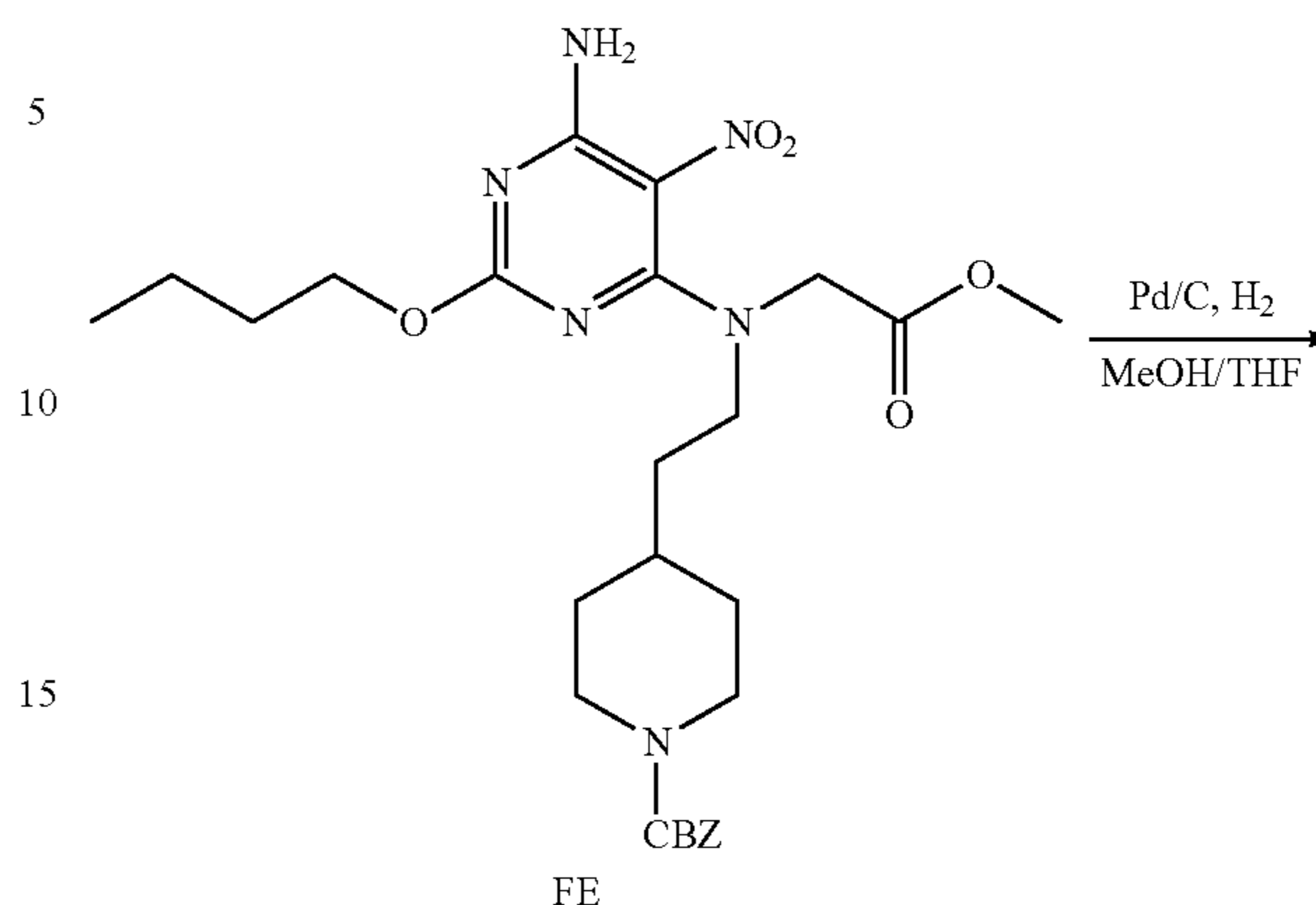
Scheme 94
