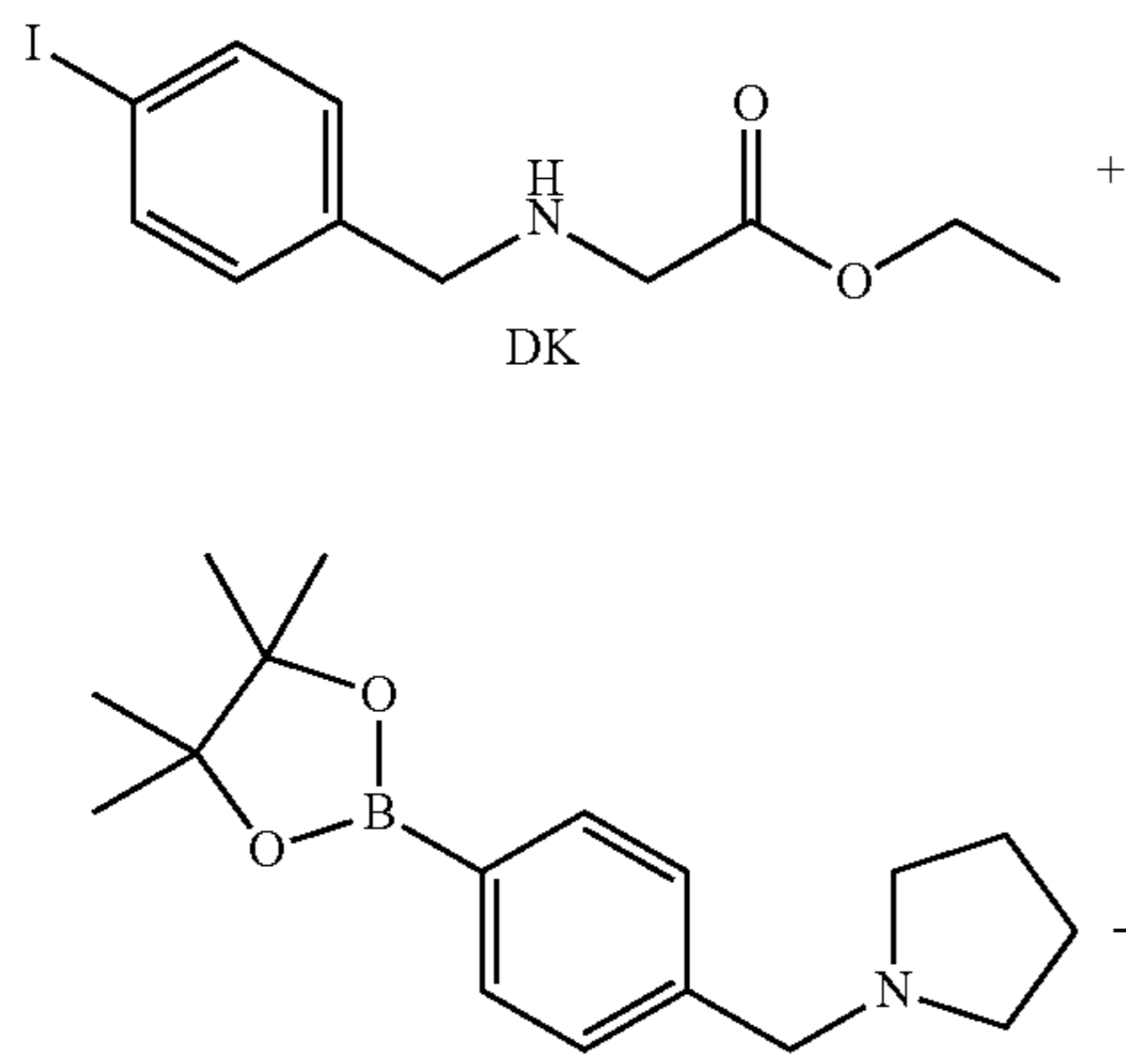
Scheme 79
