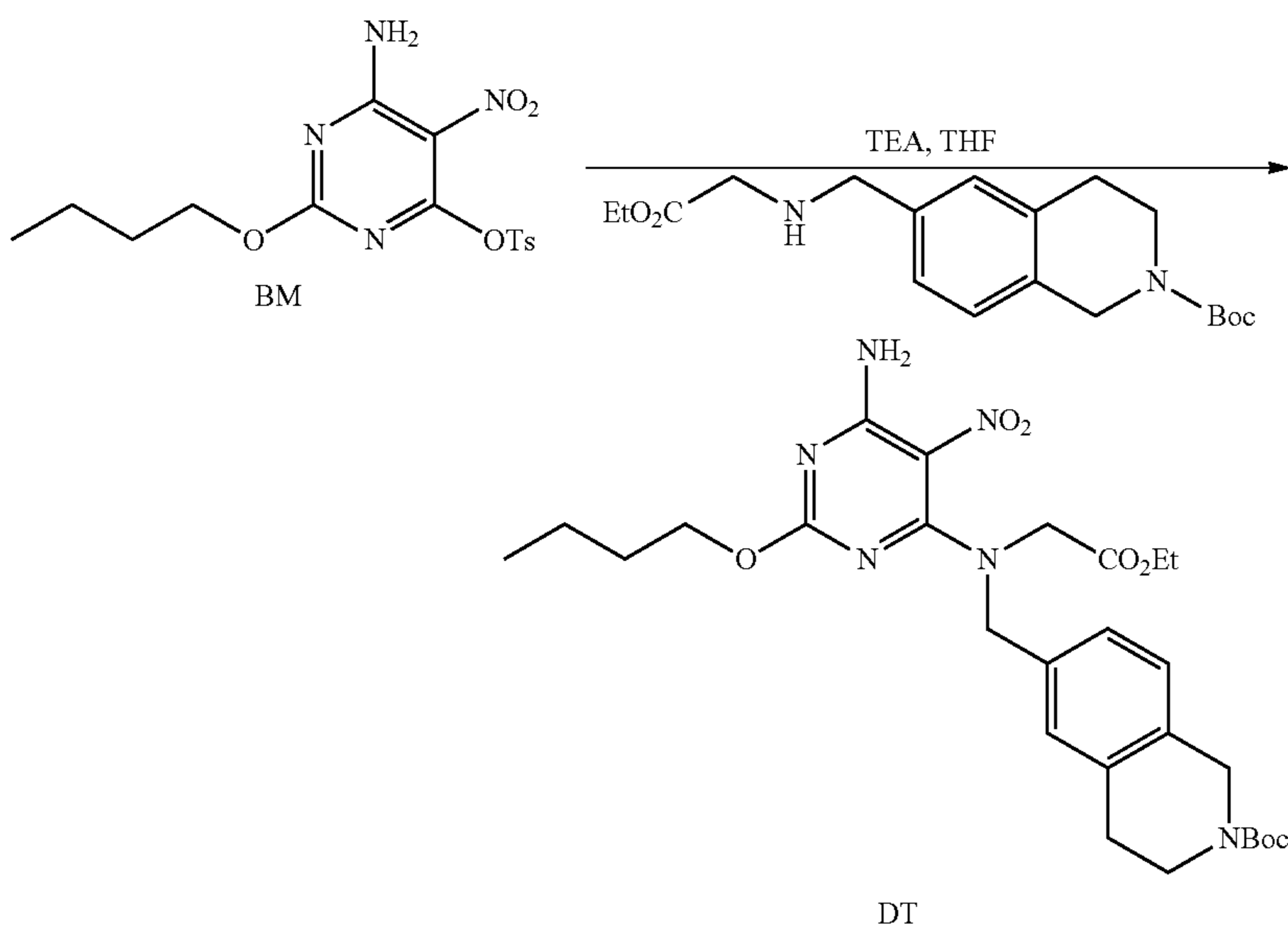
Scheme 89:
