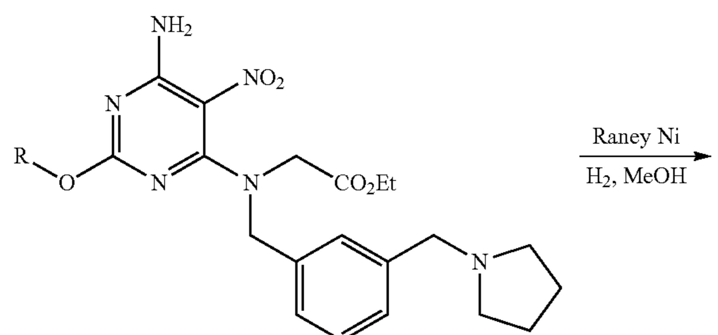
Scheme 15
