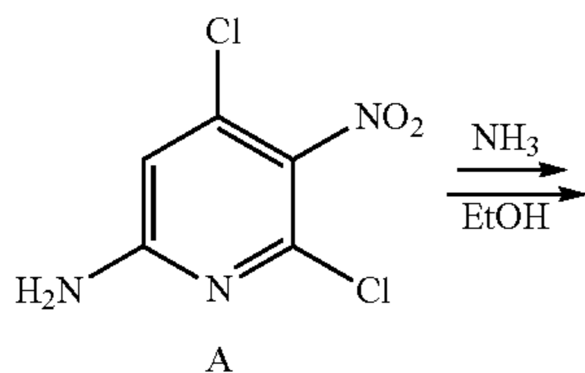
Scheme 1
