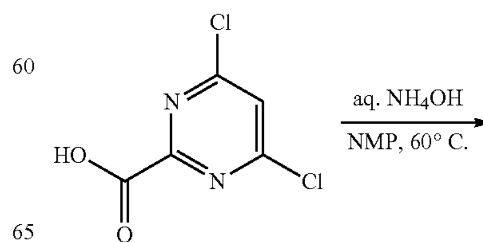
Scheme 80
