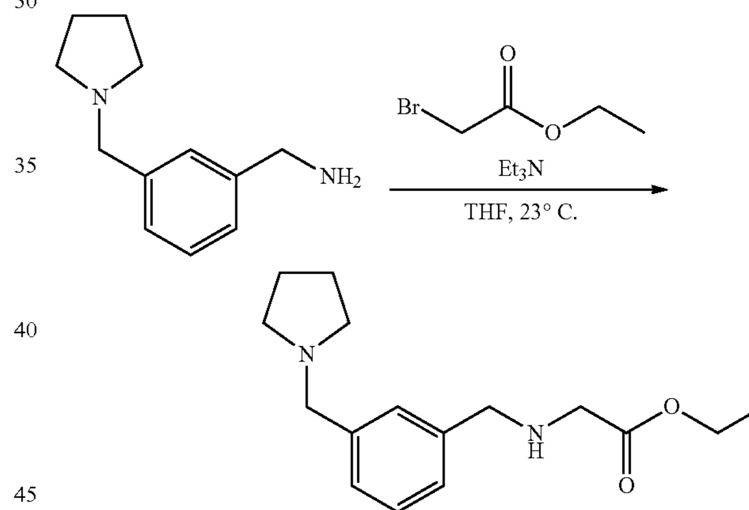
Scheme 6
