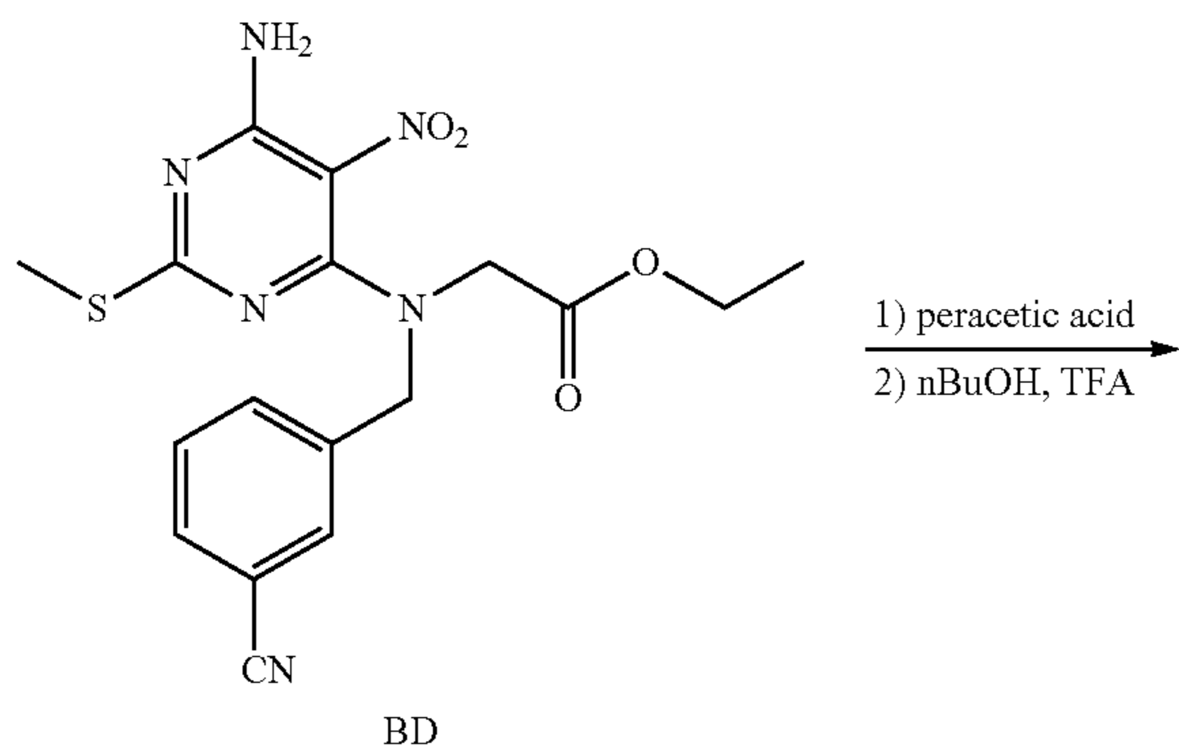
Scheme 22
