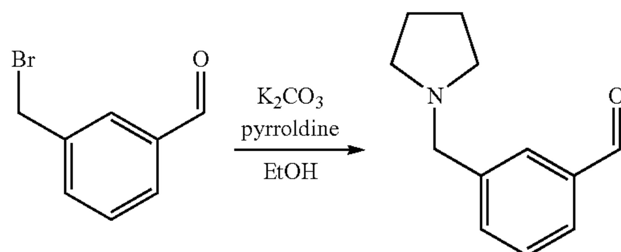
Scheme 4
