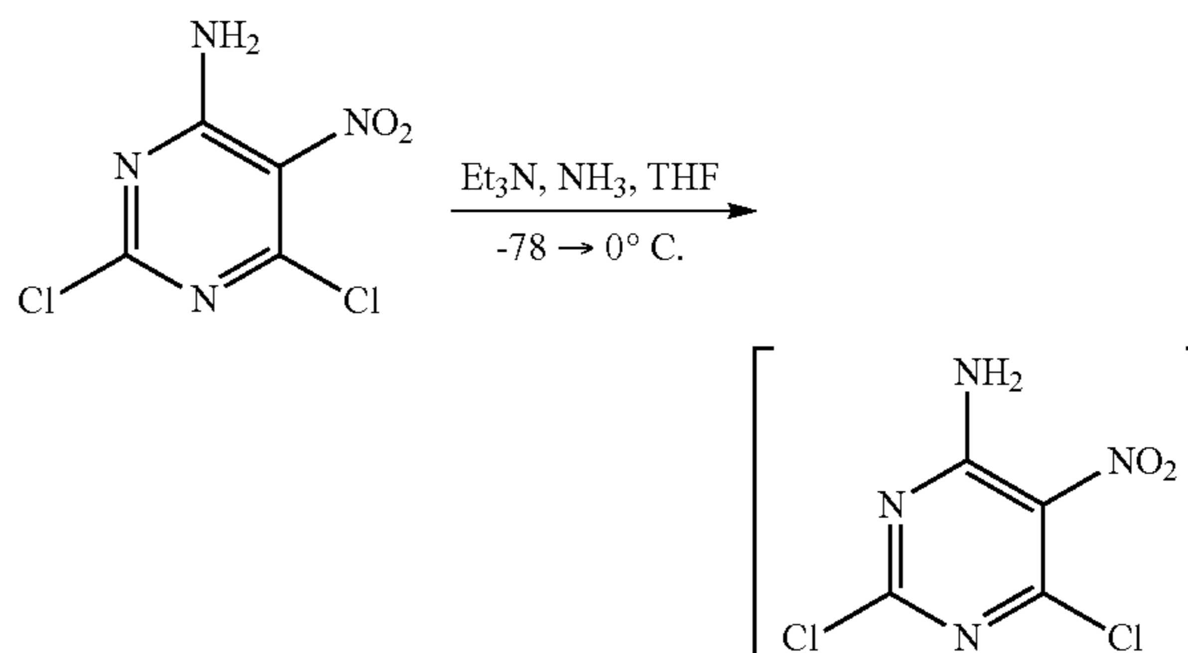
Scheme 39
