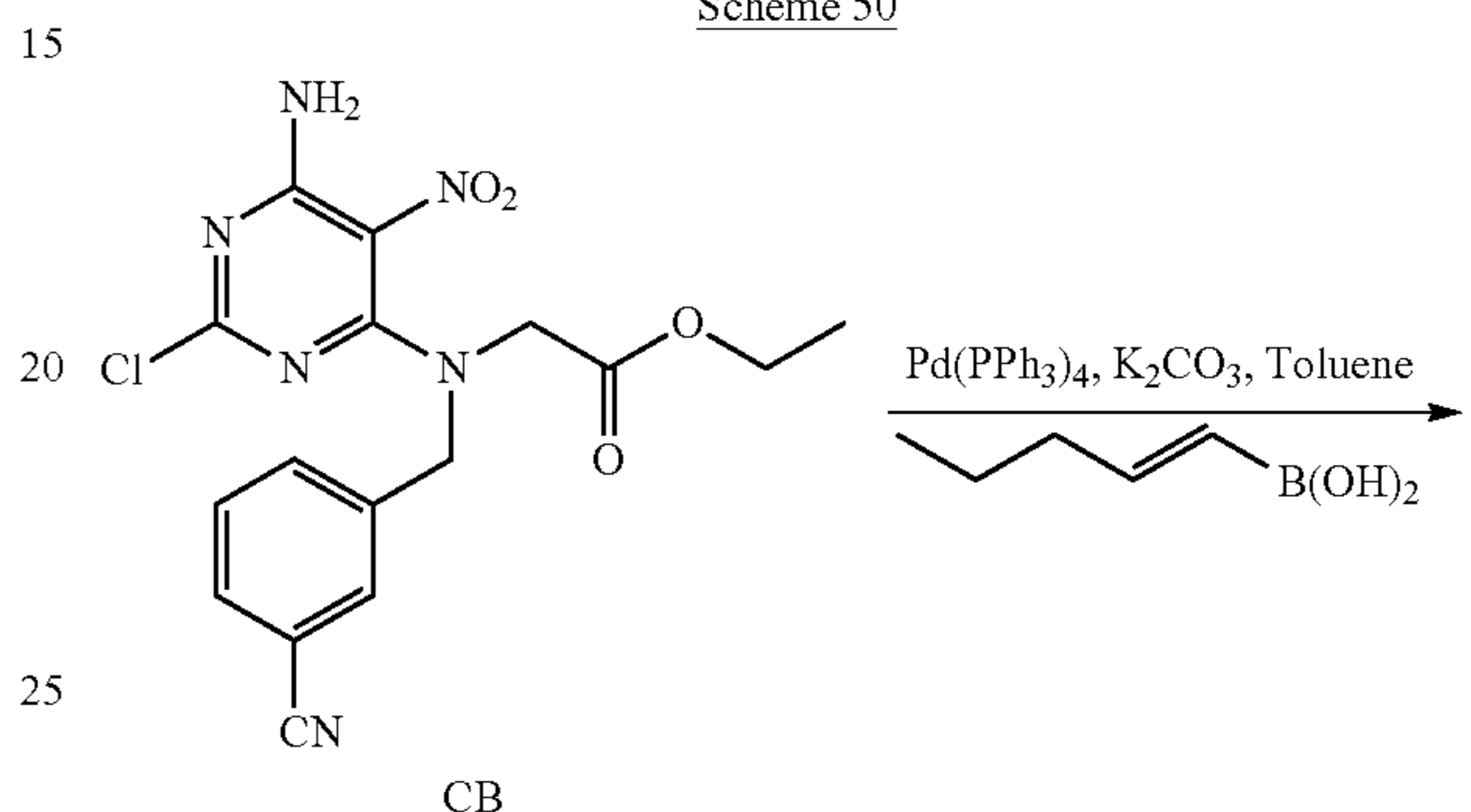
Scheme 50
