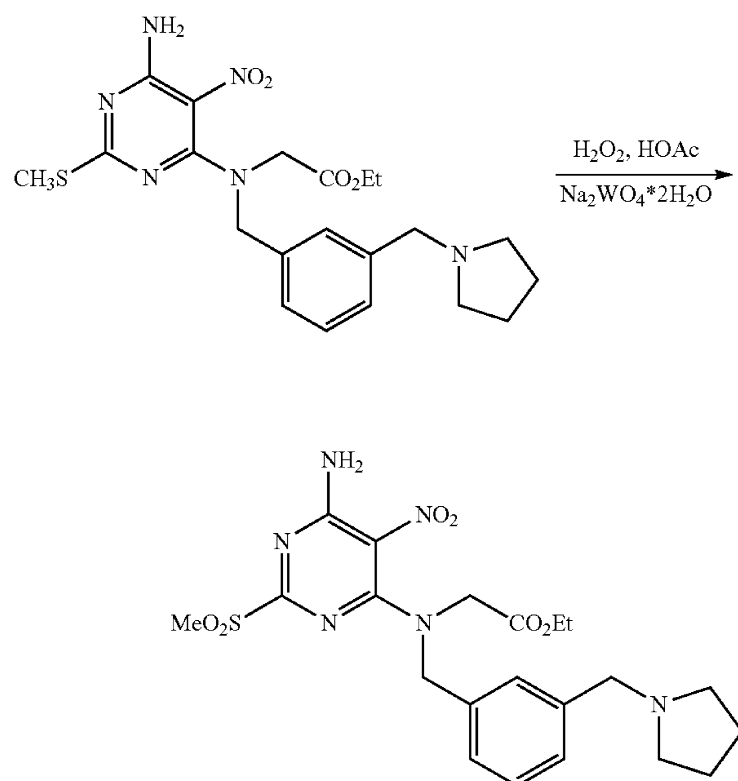
Scheme 11
