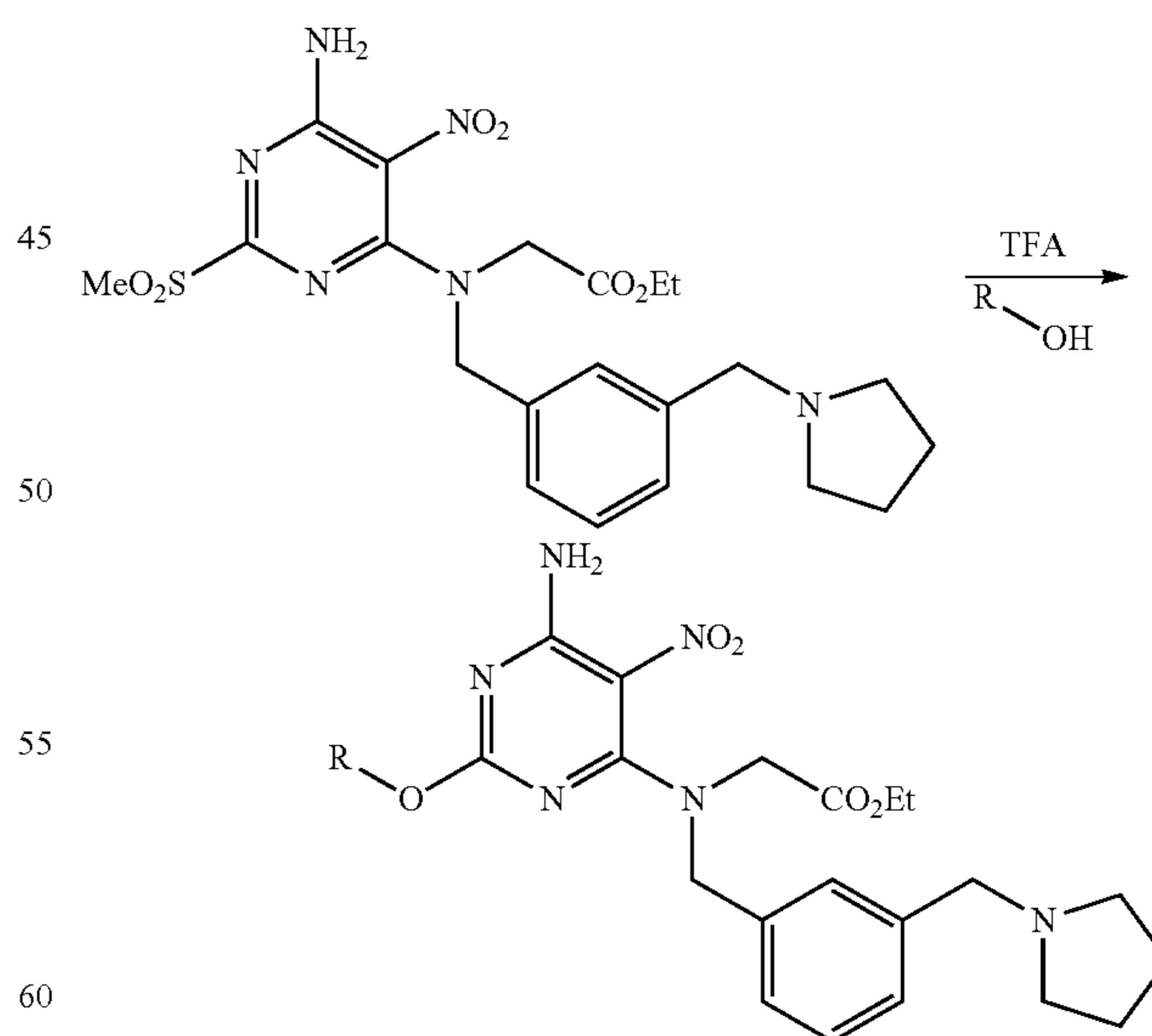
Scheme 13
