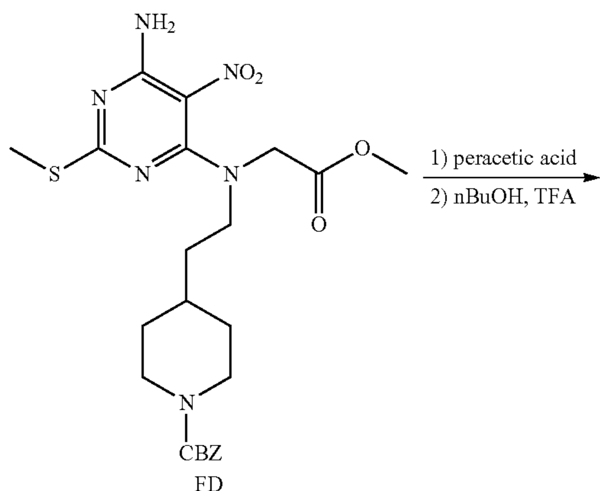
Scheme 93
