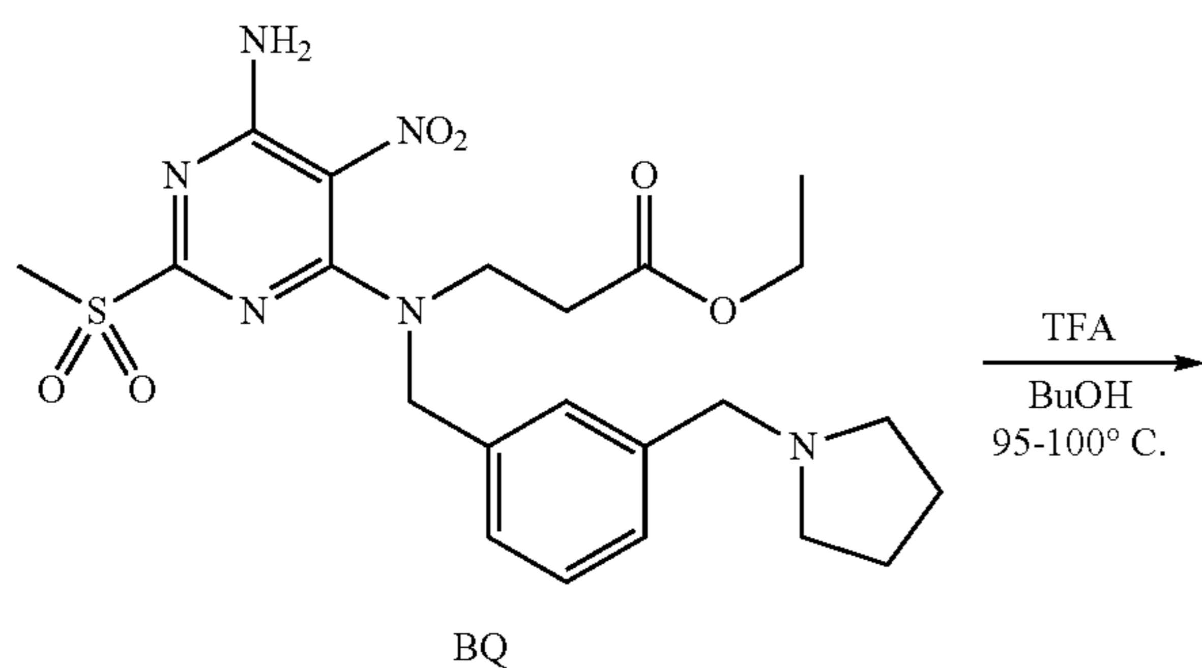
Scheme 37
