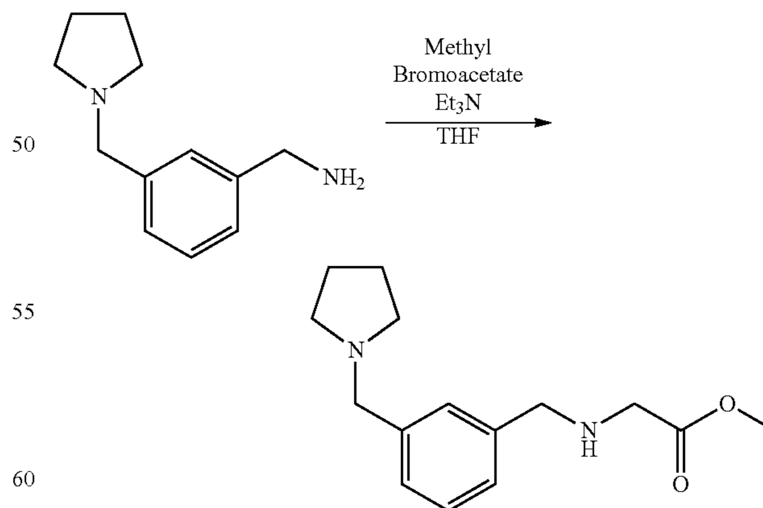
Scheme 20
