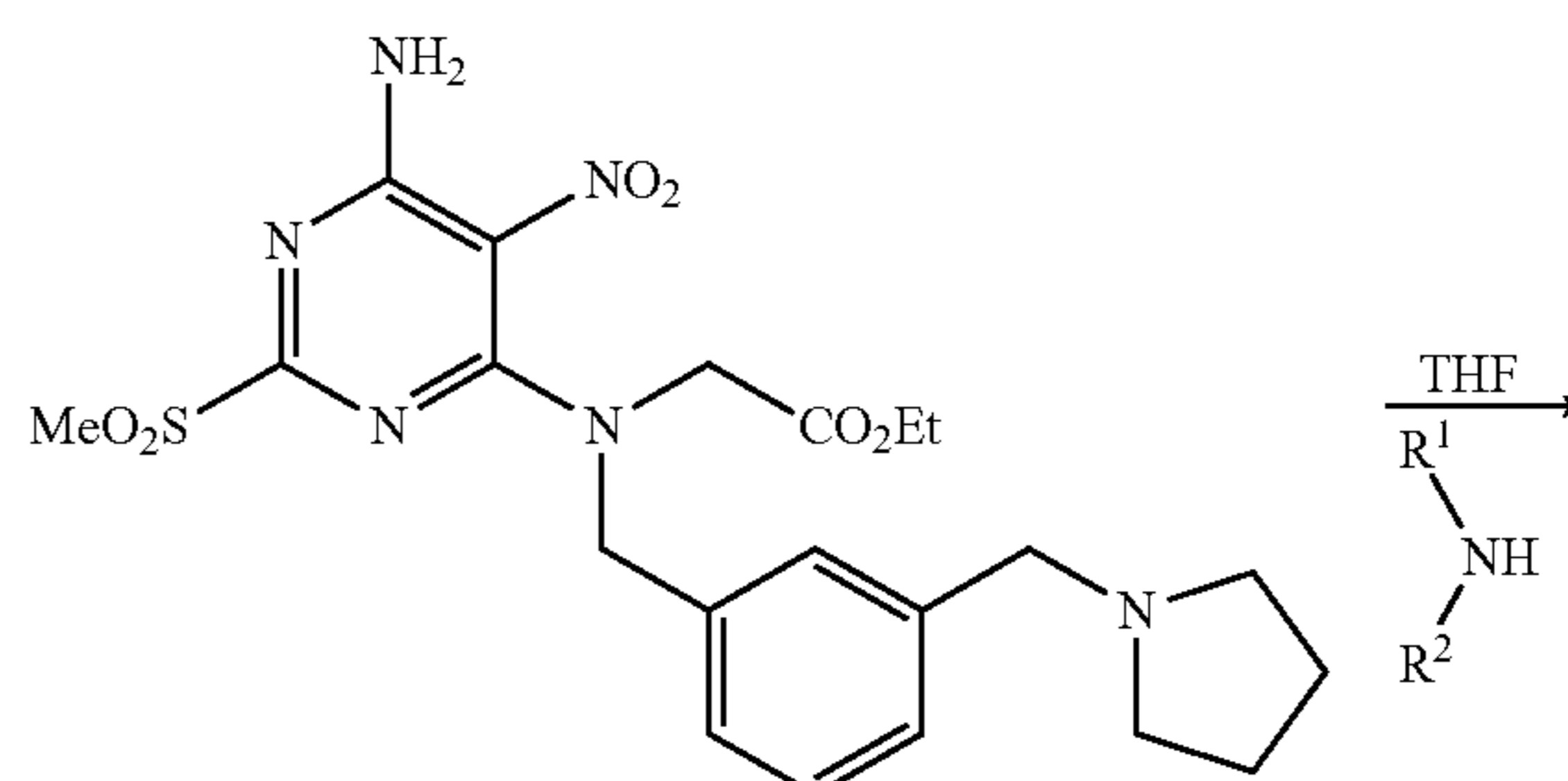
Scheme 16
