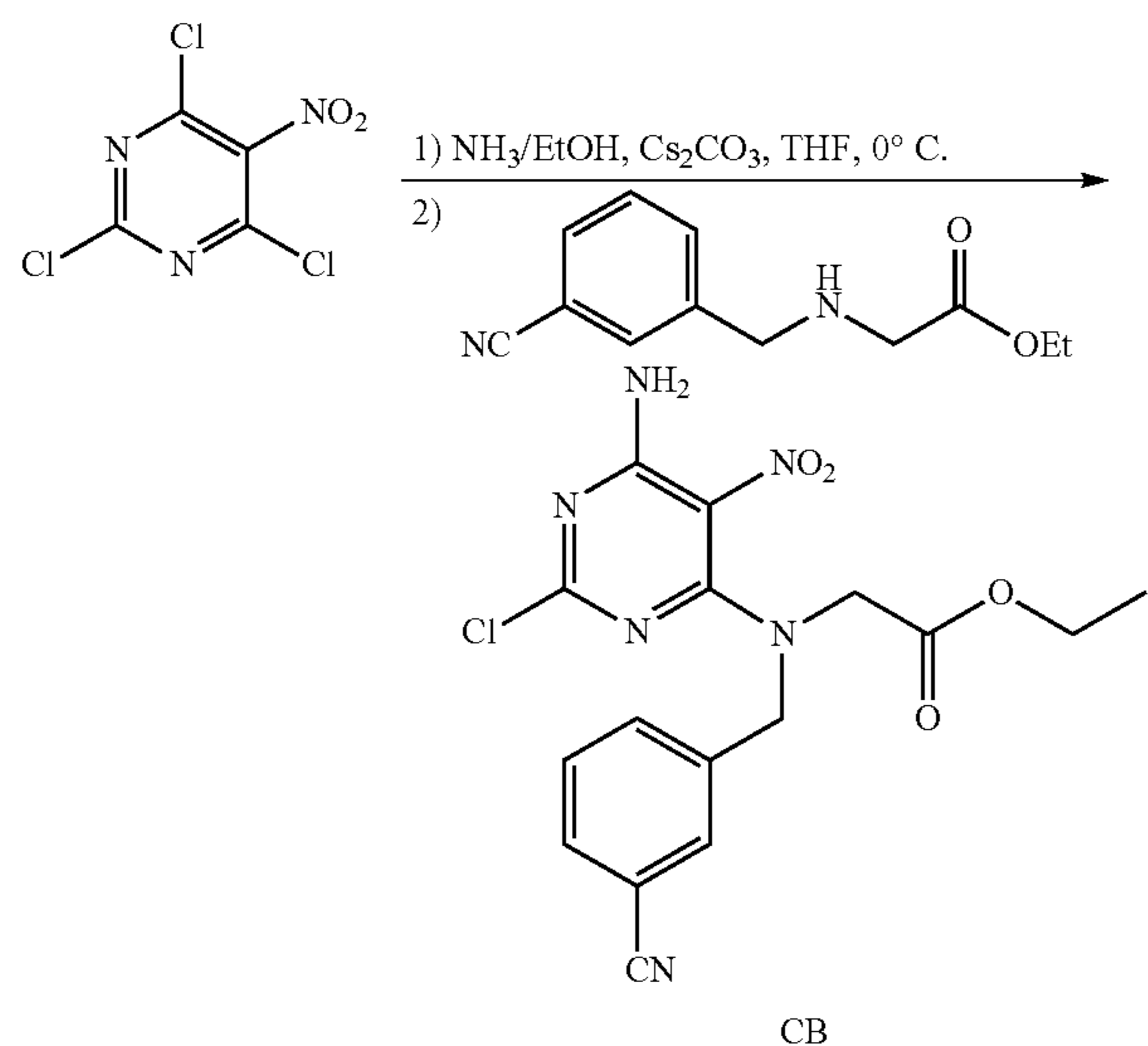
Scheme 49
