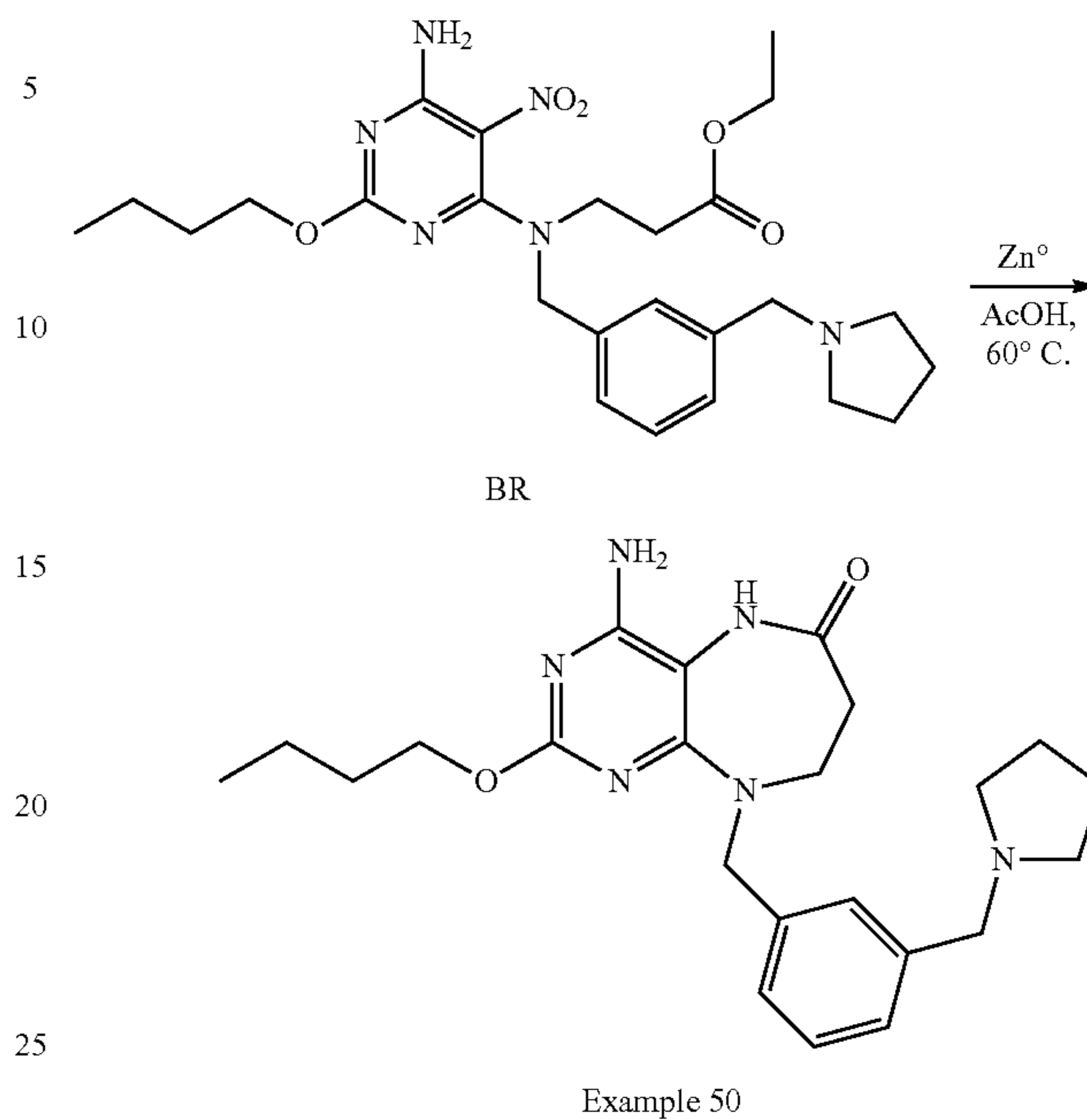
Scheme 38: Example 50
