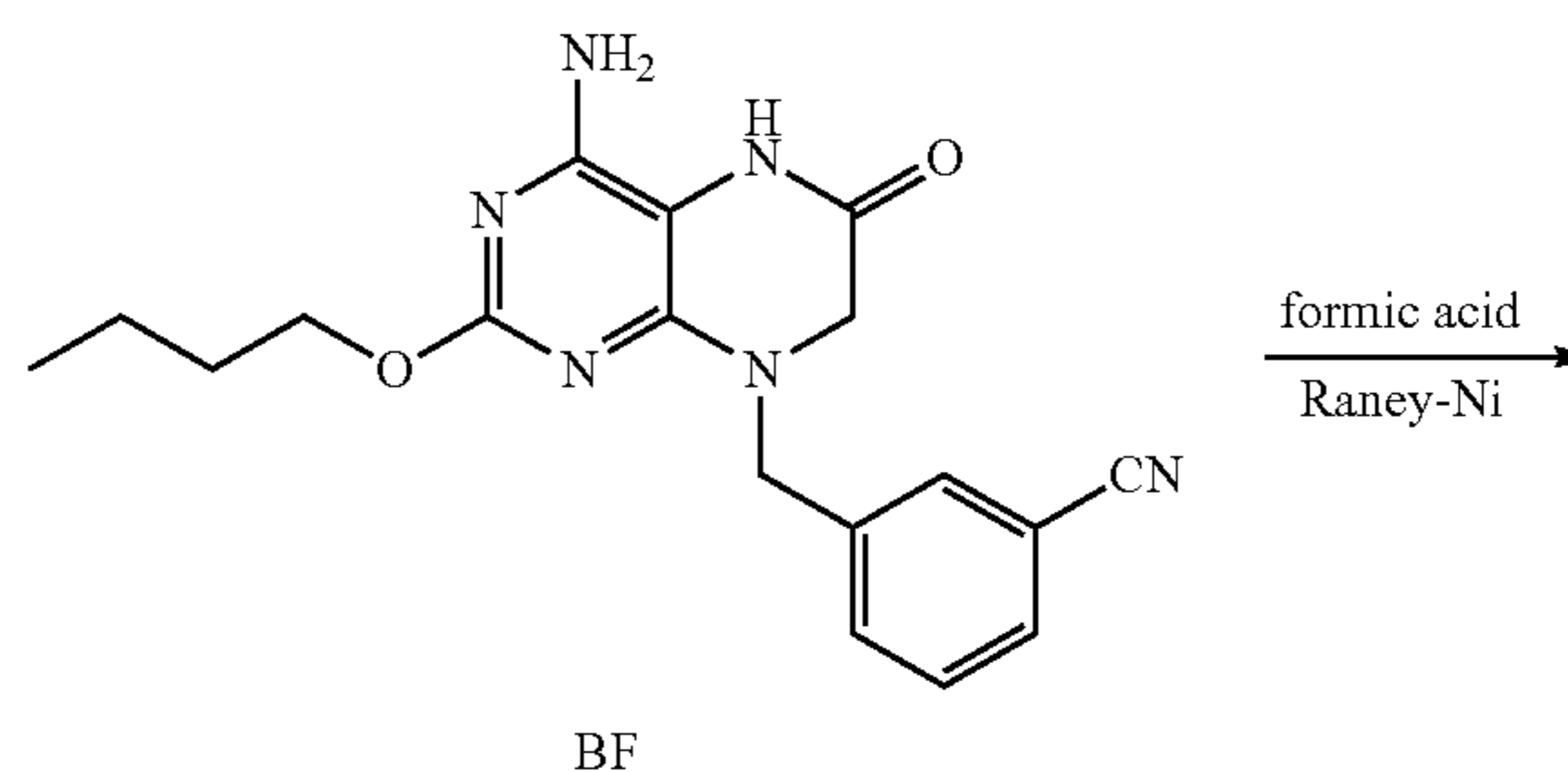
Scheme 24
