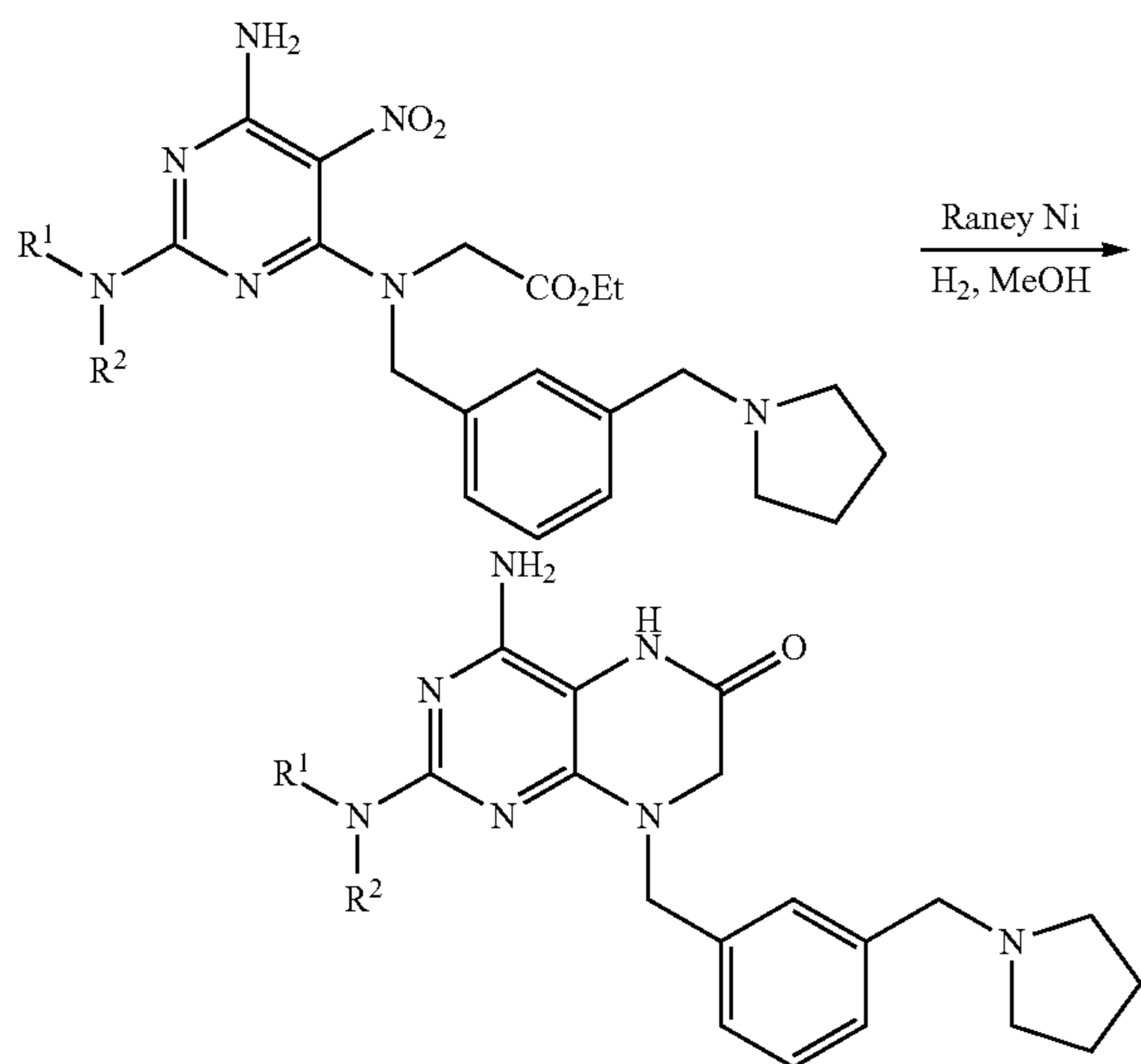
Scheme 17
