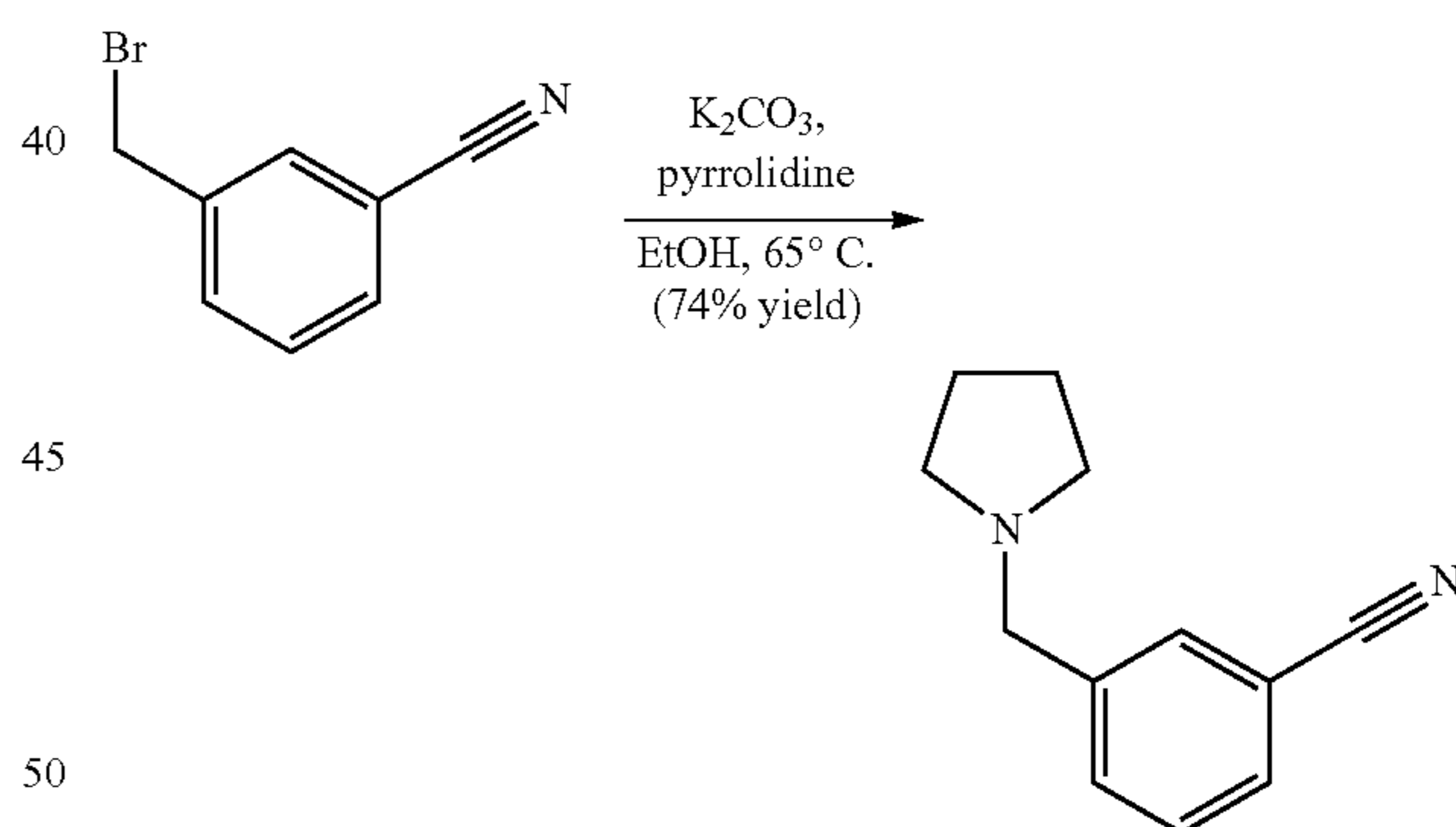
Scheme 3
