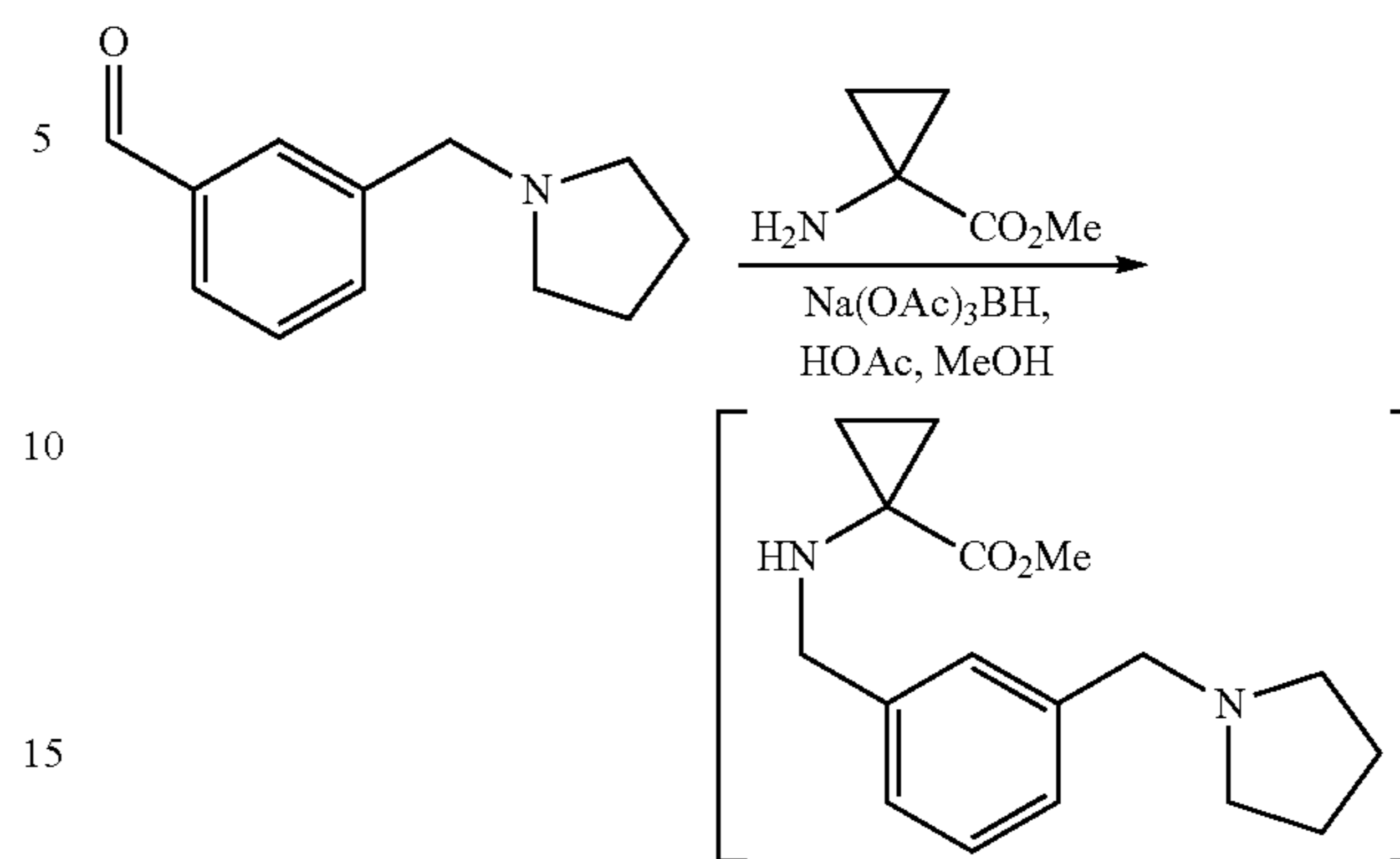
Scheme 12
