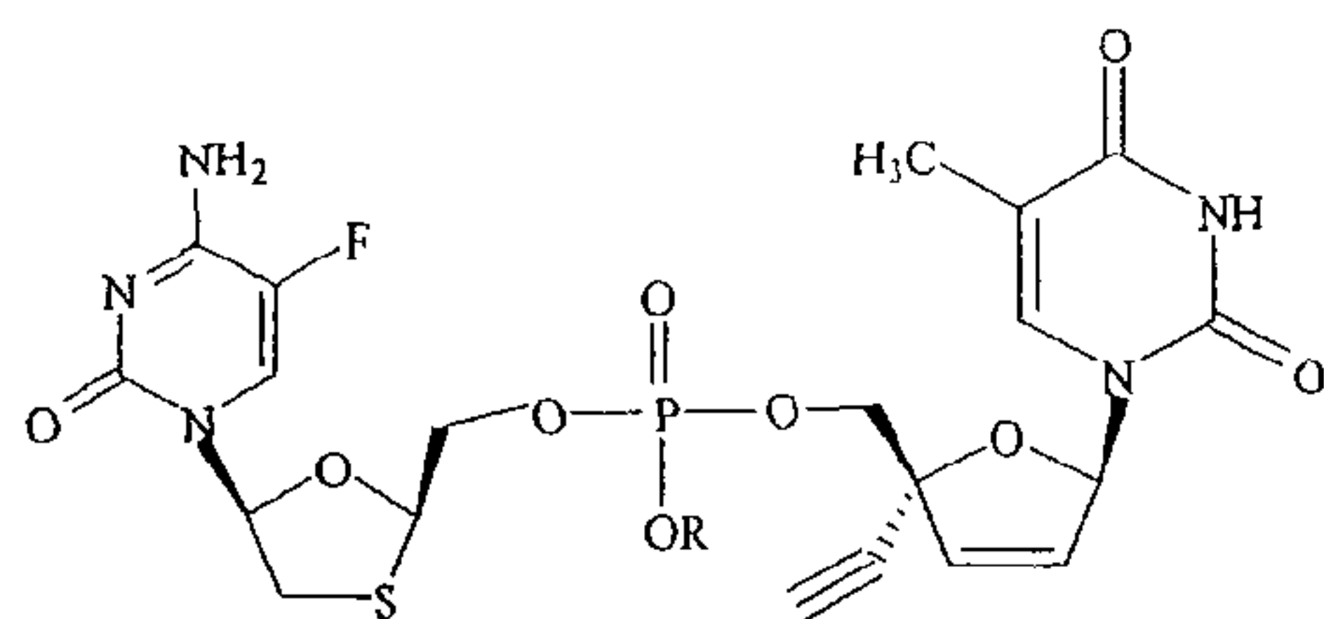
FTC and TKD-4-114 Dinucleoside Phosphate
