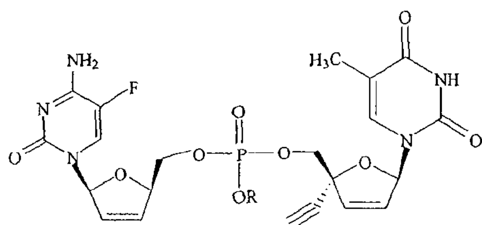
BLFd4C and TKD-4-114 Dinucleoside Phosphate
