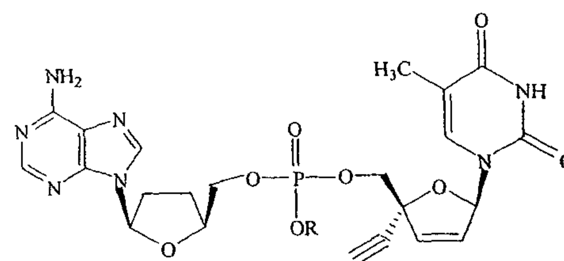
ddA and TKD-4-114 Dinucleoside Phosphate
