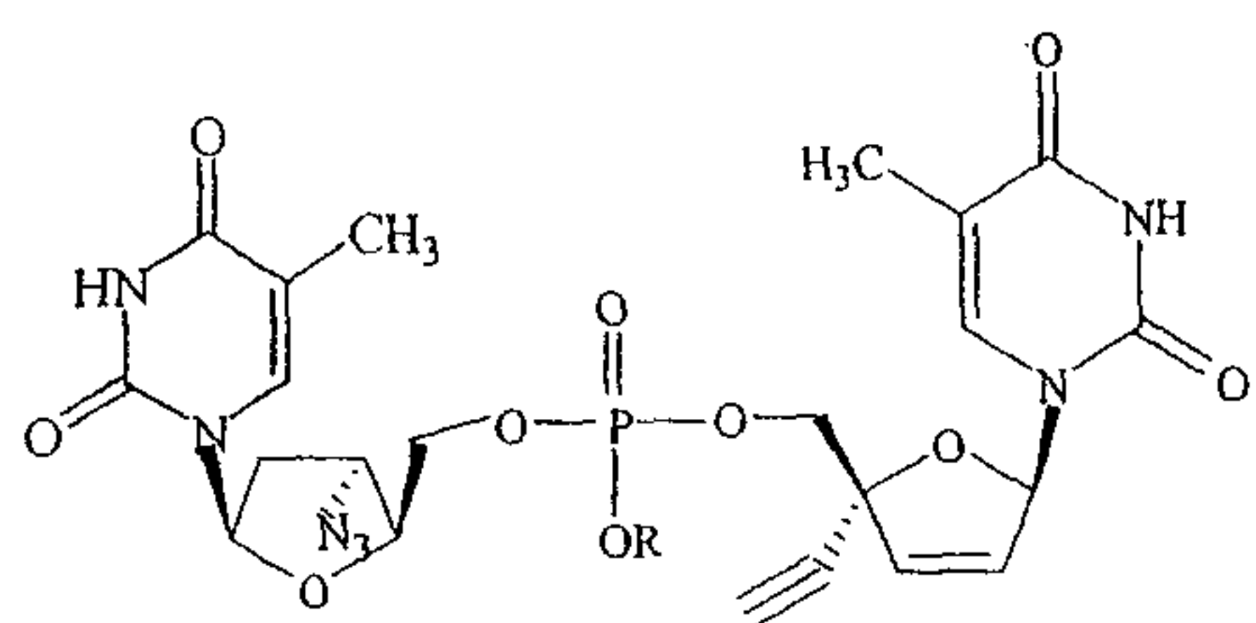
AZT and TKD-4-114 Dinucleoside Phosphate
