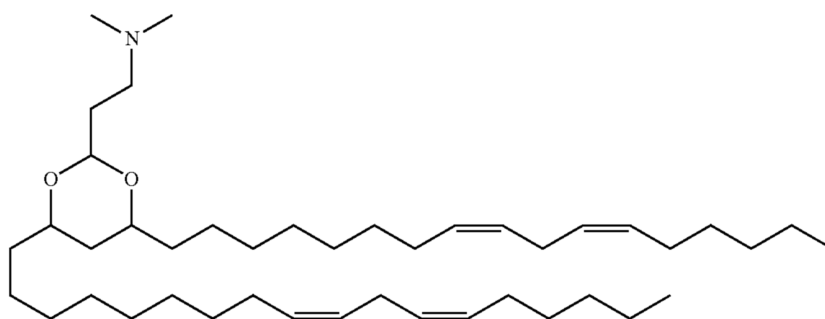
2-(4-((8Z,11Z)-heptadeca-8,11-dien-1-yl)-6-((9Z,12Z)-octadeca-9,12-dien-1-yl)-1,3-dioxan-2-yl)-N,N-dimethylethanamine (8)
