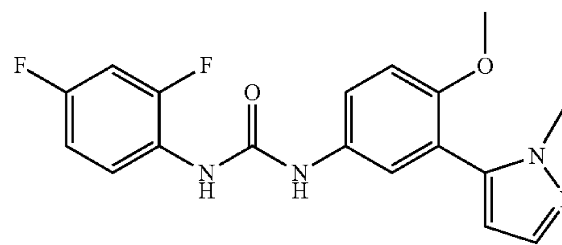
1-(2,4-difluorophenyl)-3-(4-methoxy-3-(1-methyl-1H-pyrazol-5-yl)phenyl)urea
