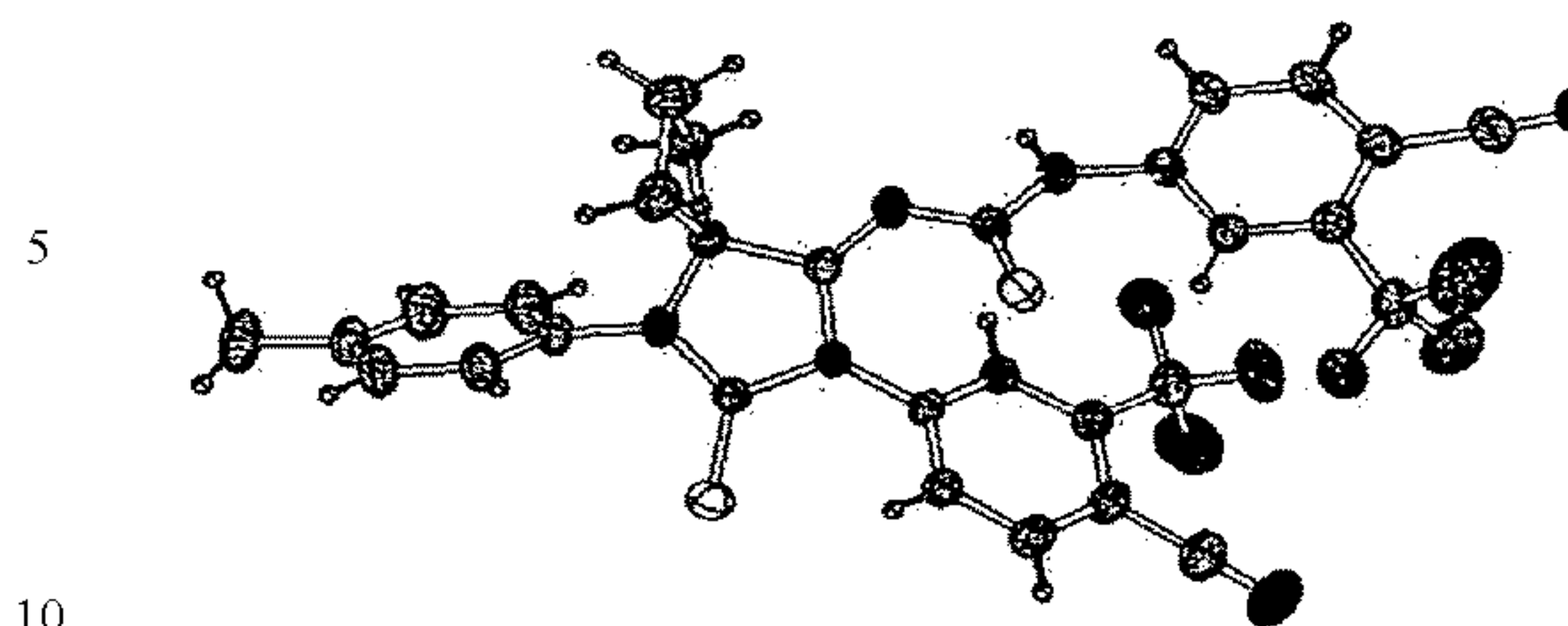
X-ray structure of 35a
