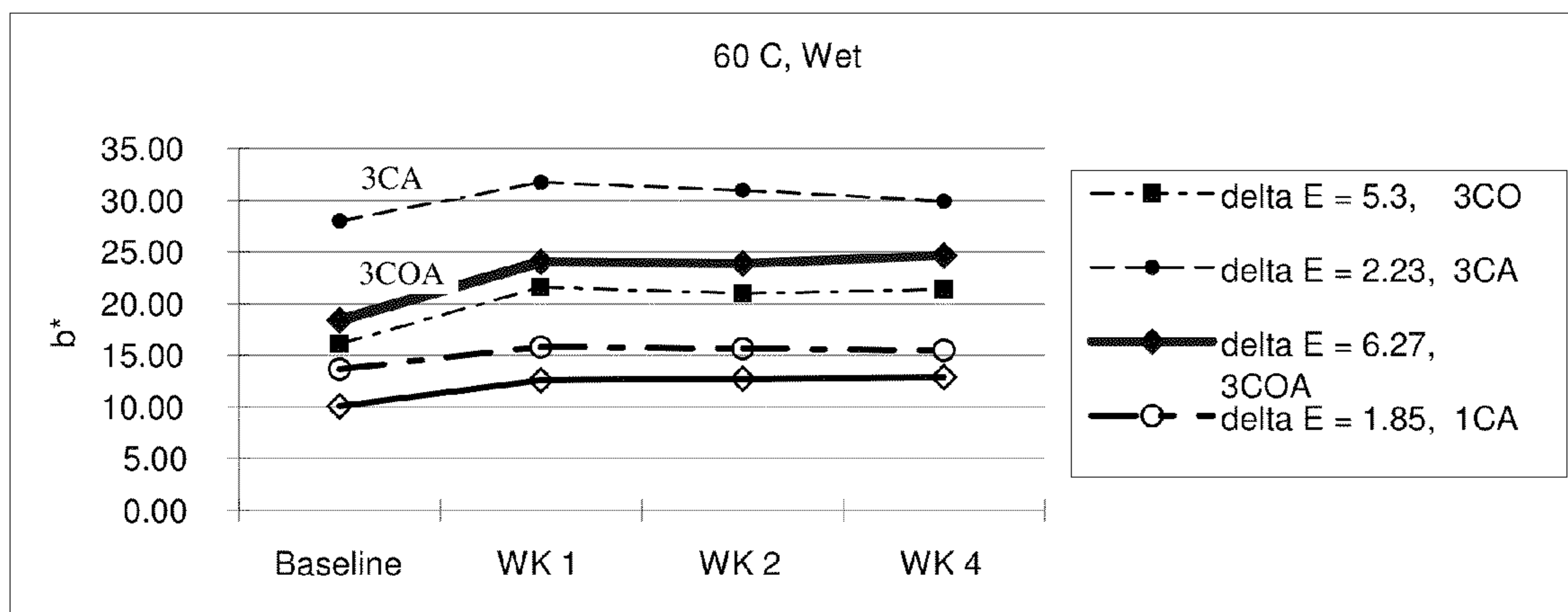
Change of b* values with high temperature and wet conditions
