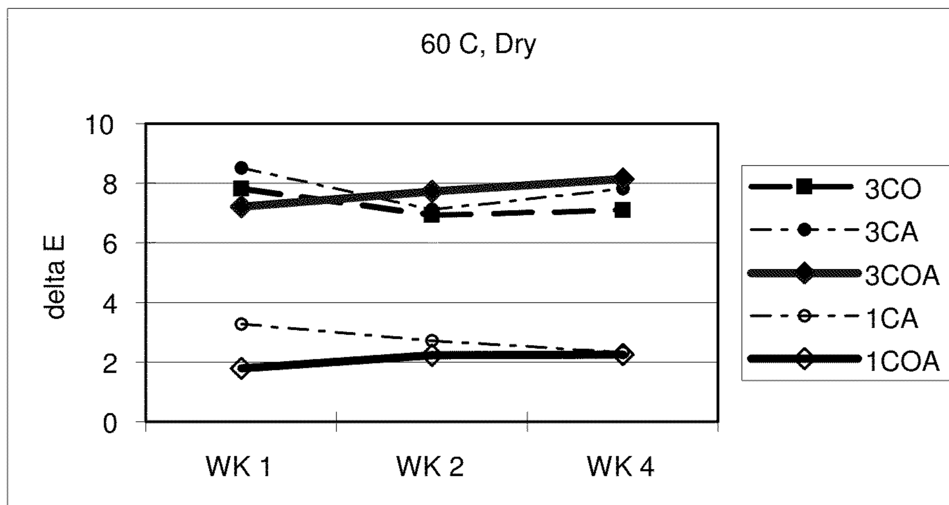
Change of \Delta E values with 60 C, dry conditions
