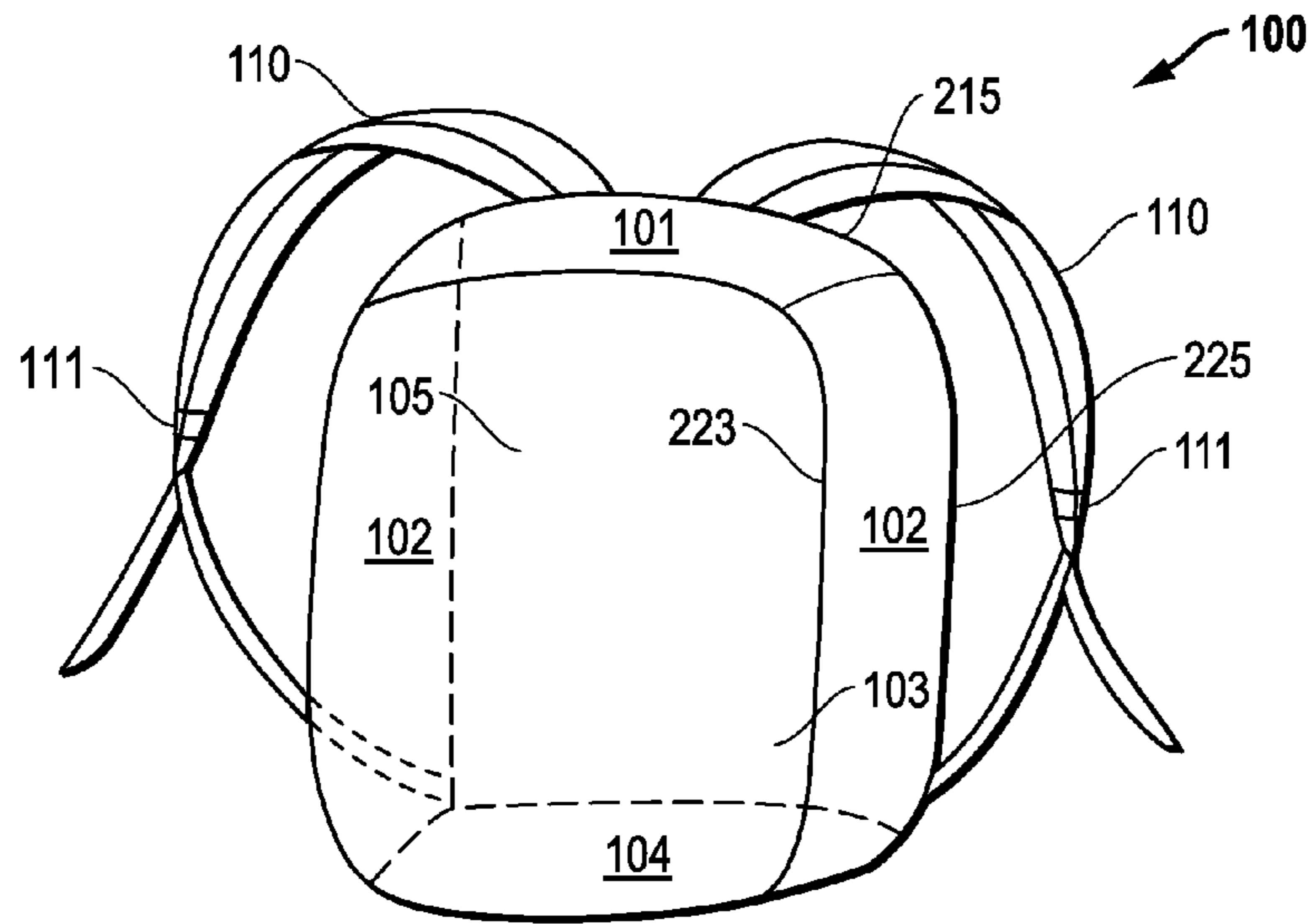
FIG. 1 (Prior Art)
