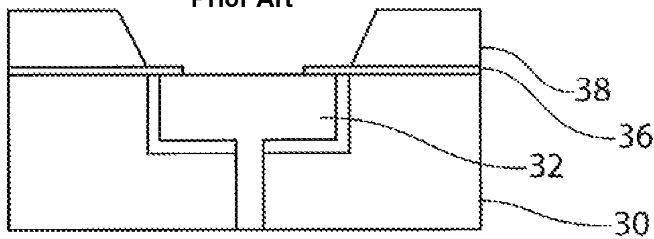
FIG. 2C "Prior Art"
