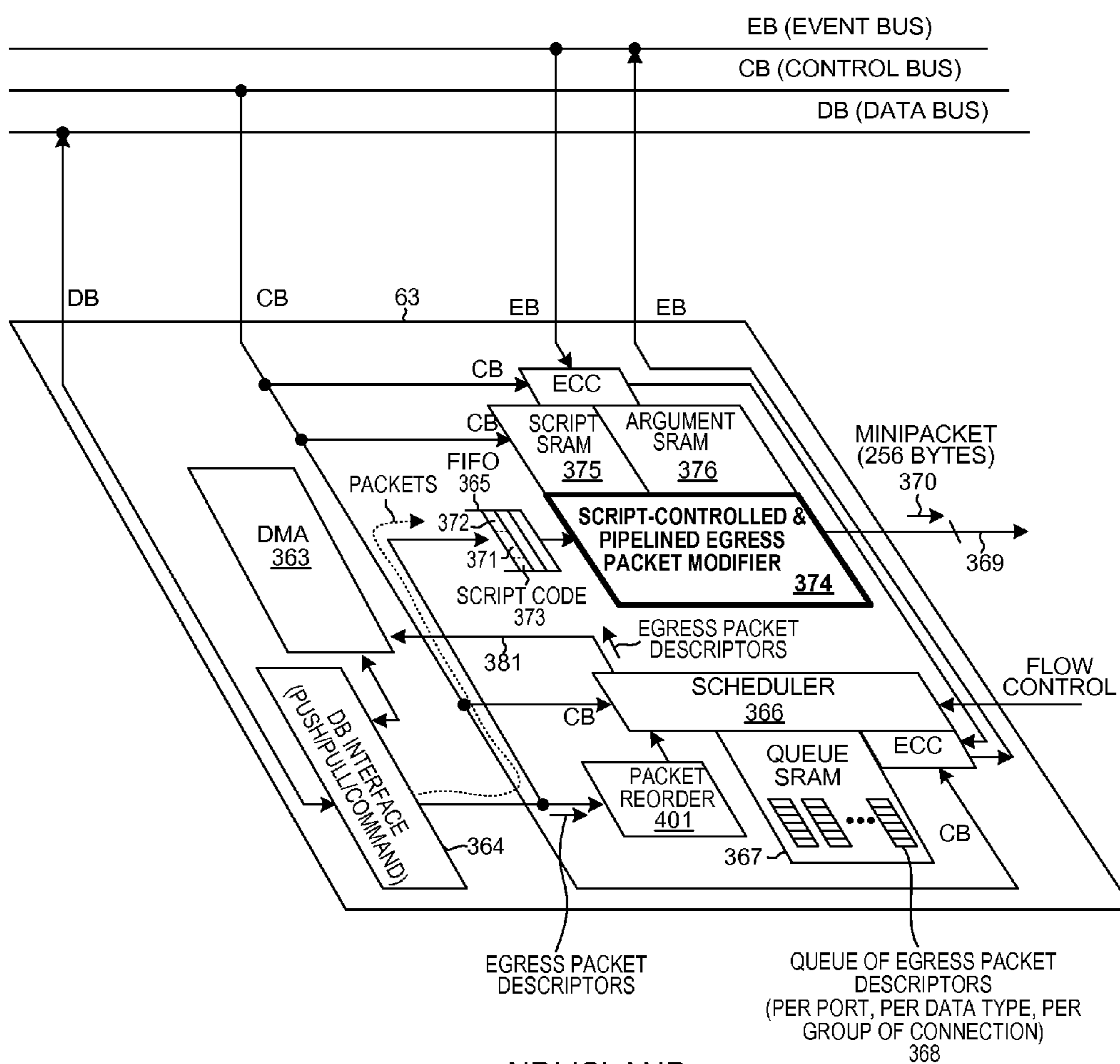
NBI ISLAND (EGRESS) FIG. 10
