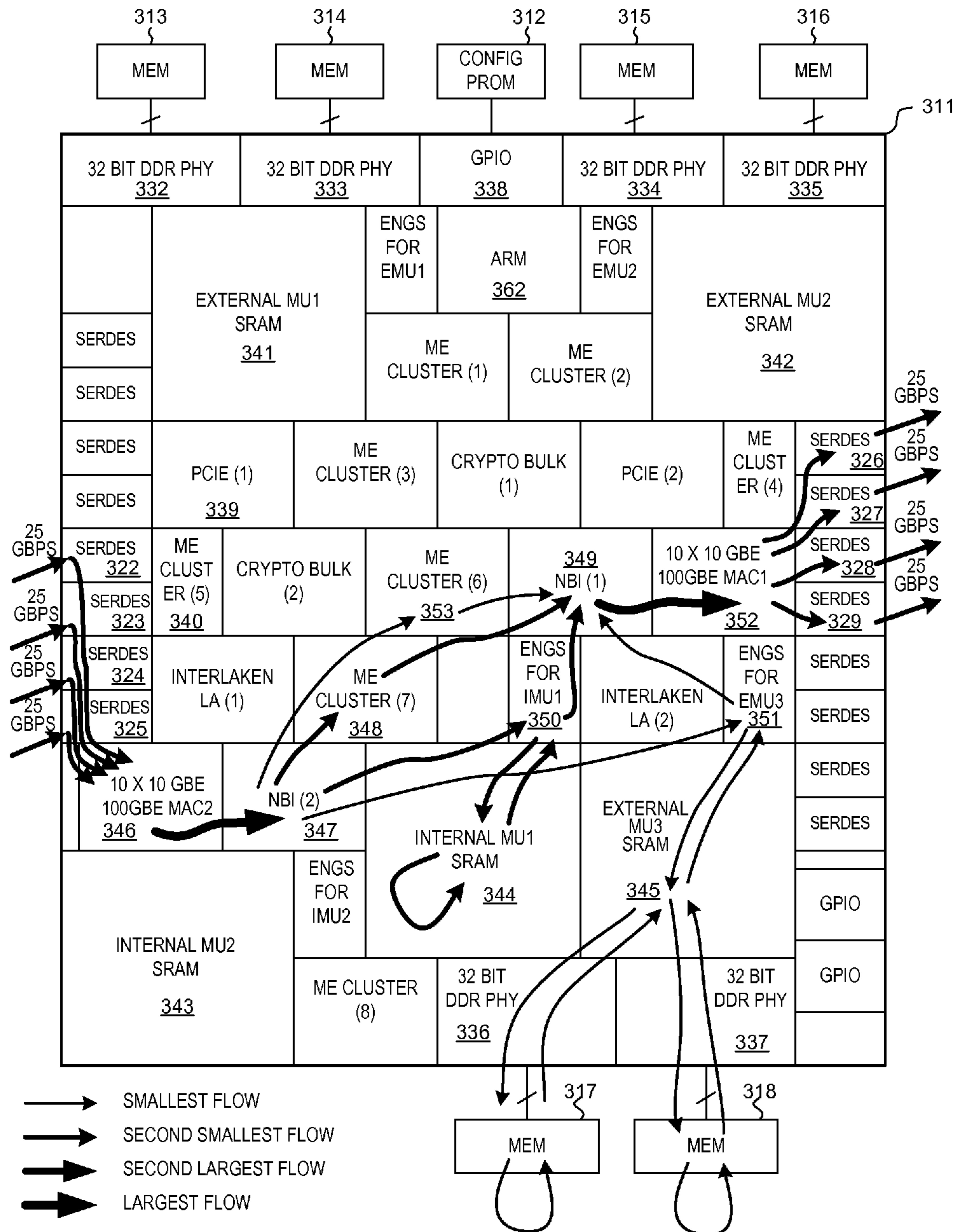
ISLAND-BASED NETWORK FLOW PROCESSOR INTEGRATED CIRCUIT FIG. 8
