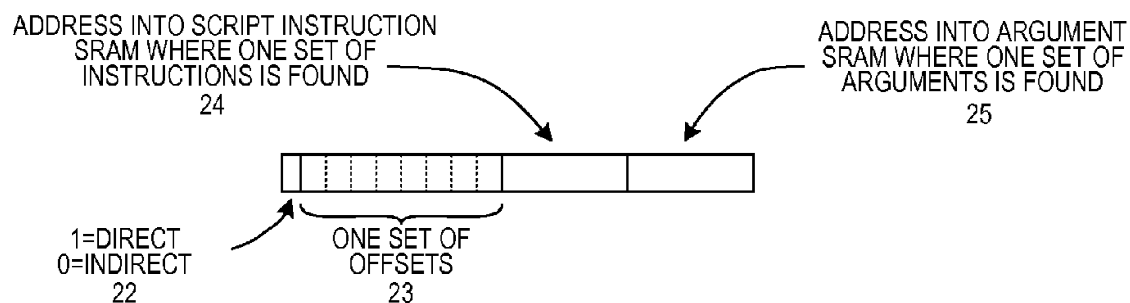
STRUCTURE OF A SCRIPT CODE
