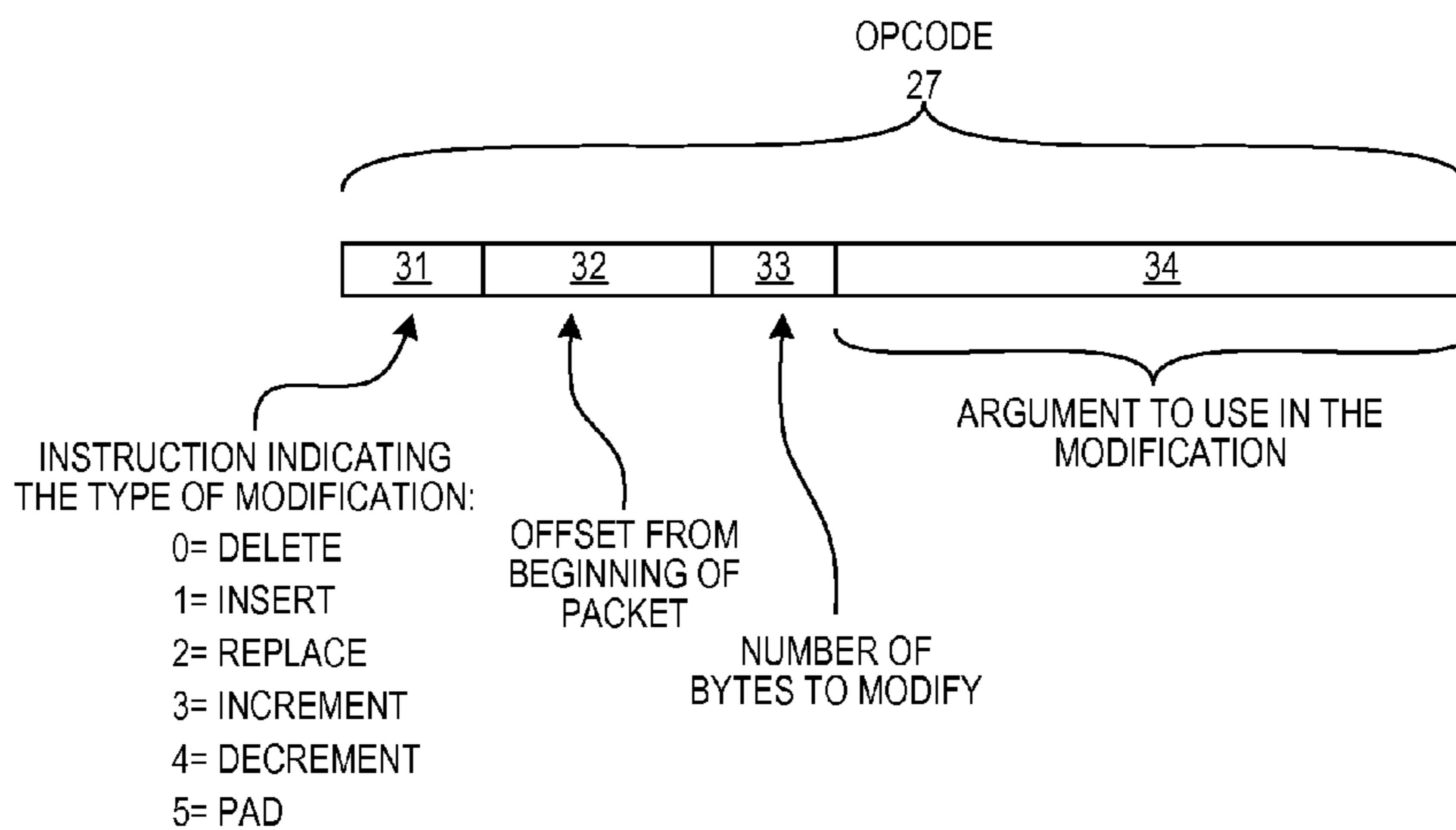
STRUCTURE OF AN OPCODE
