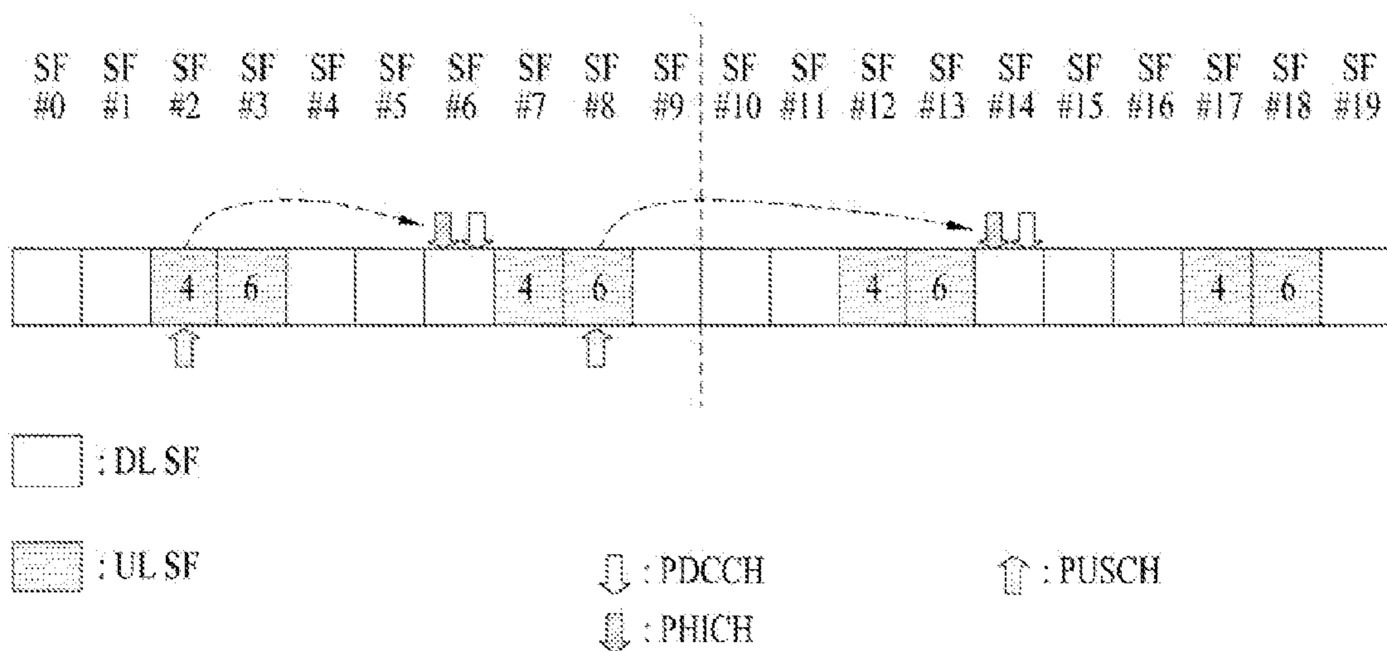
PUSCH-PHICH/UL grant timing (UL-DL configuration #1)
