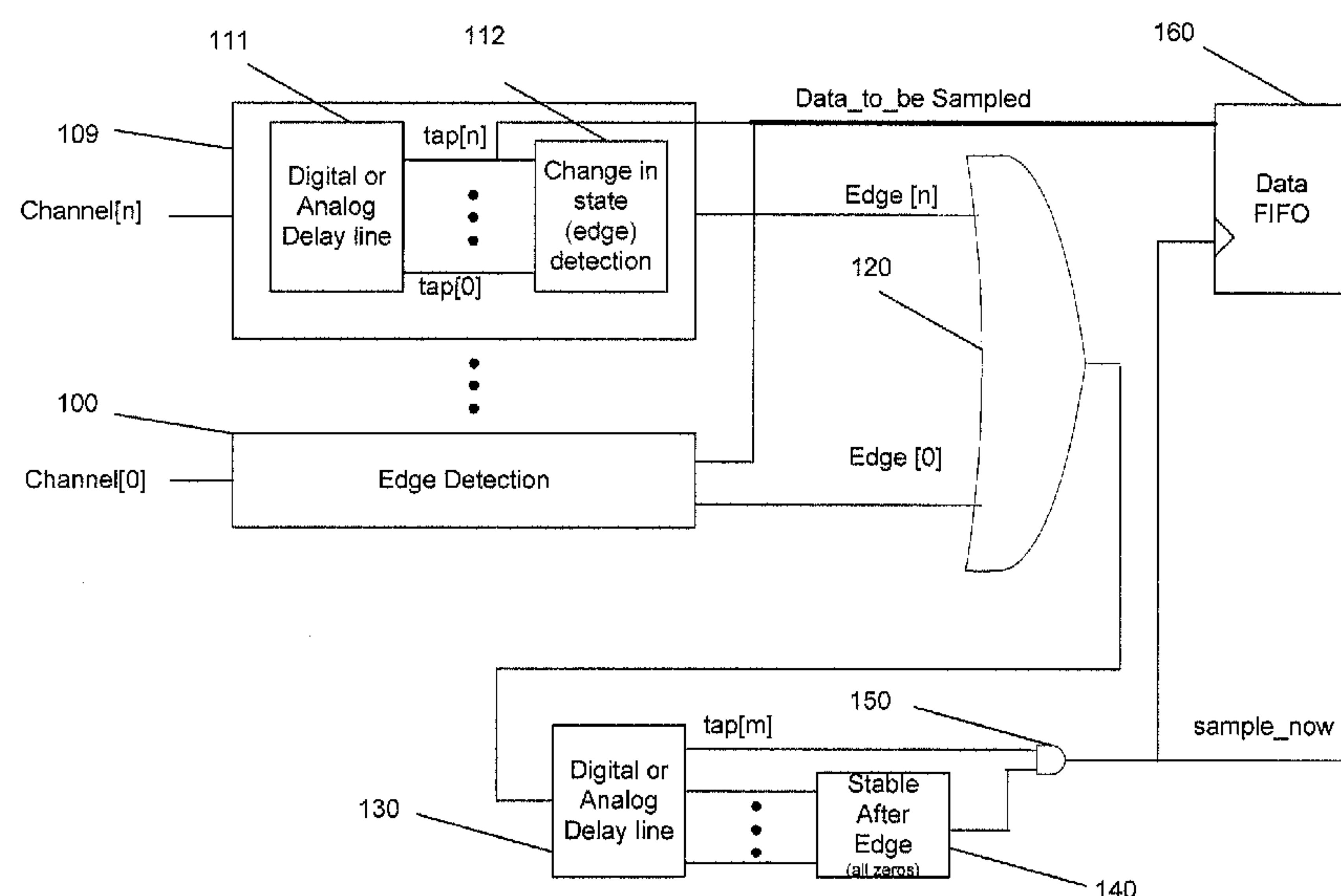
Data Extraction Hardware
