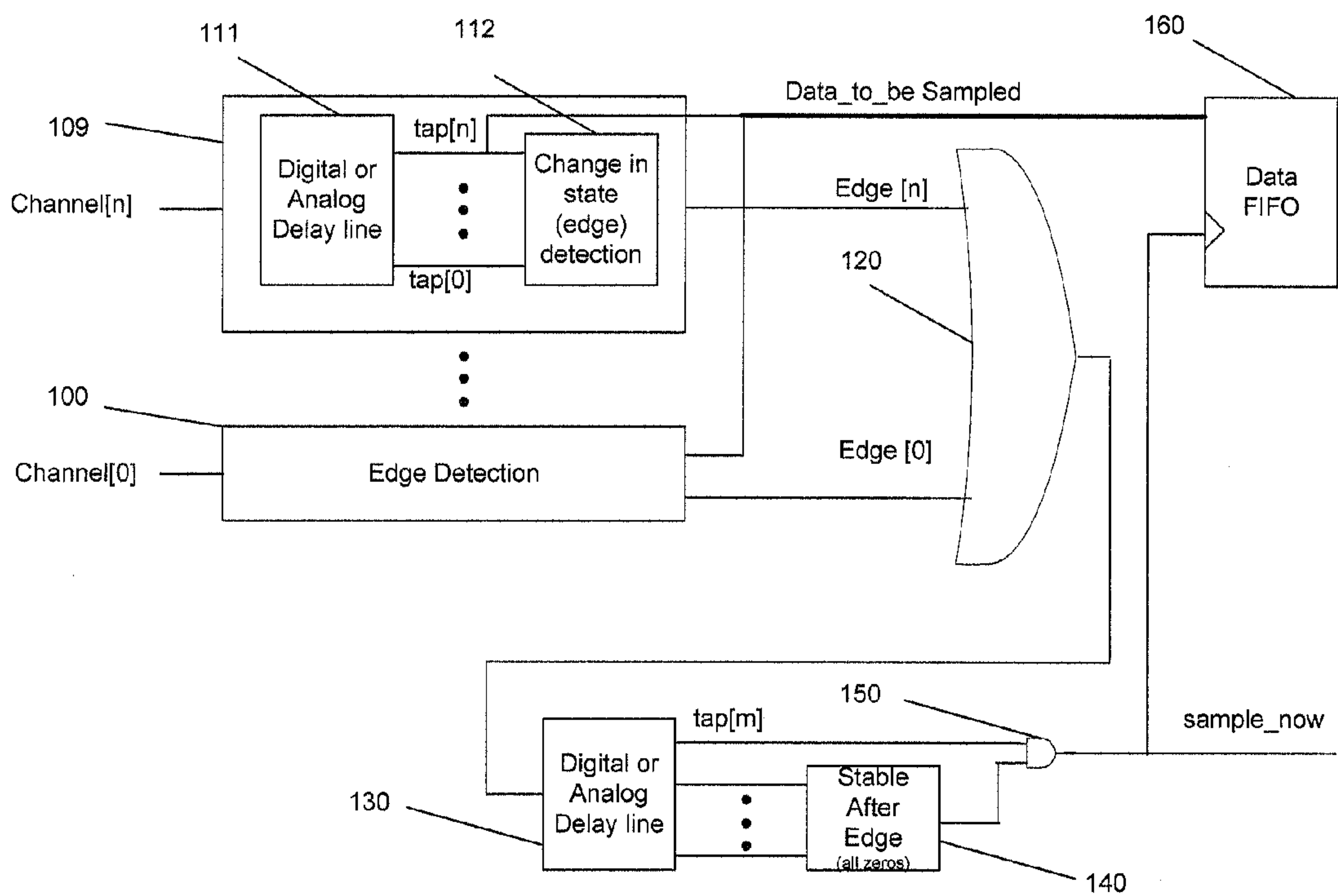
Figure 7 – Data Extraction Hardware
