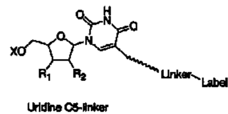
Uridine C5-linker
