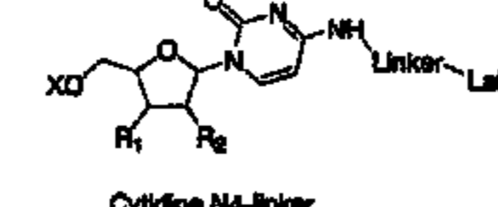
Cytidine N4-linker
