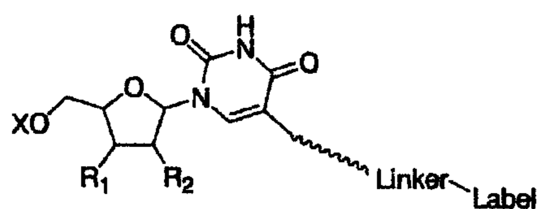
Uridine C5-linker
