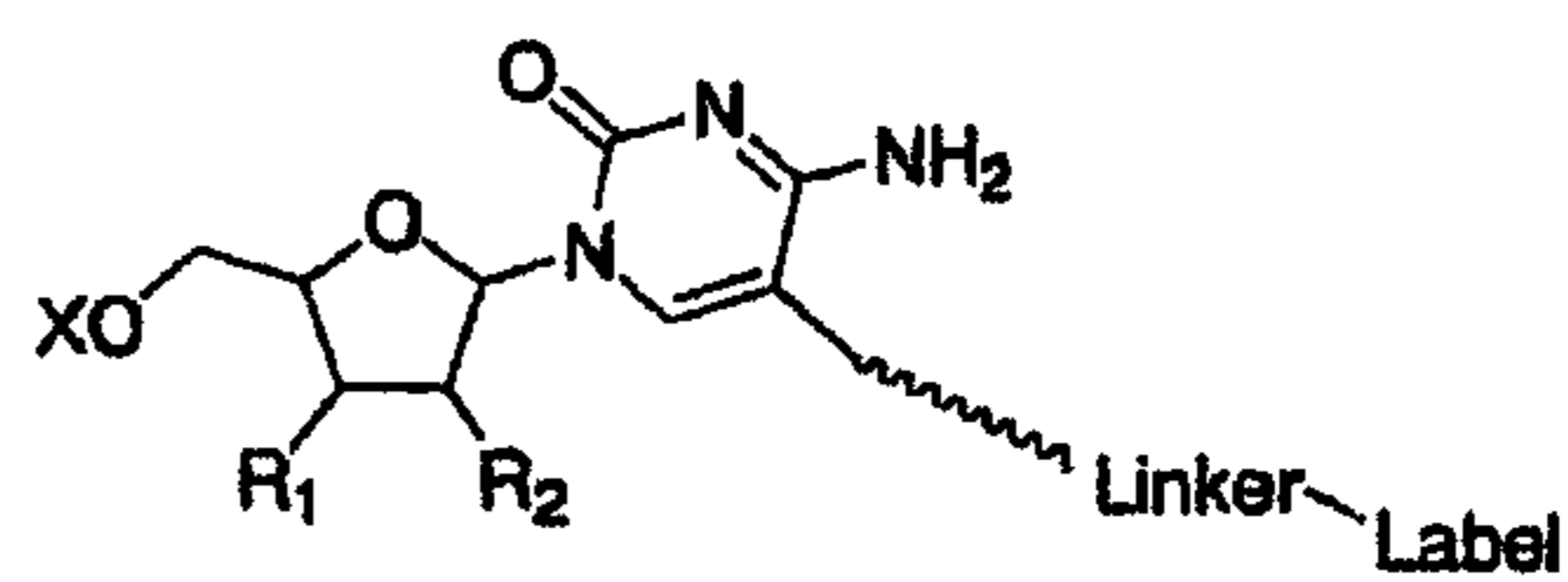
Cytidine C5-linker
