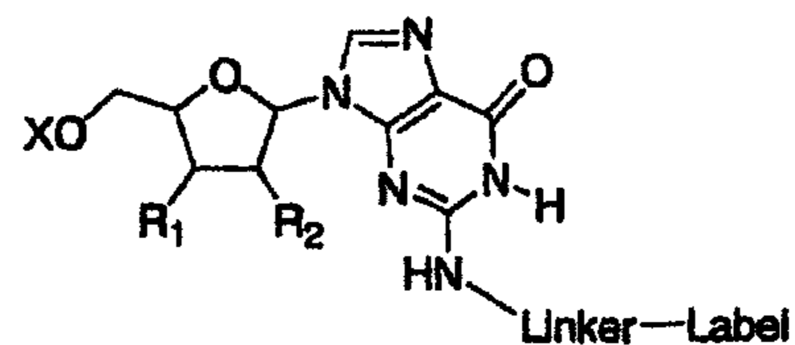
Guanosine N2-linker
