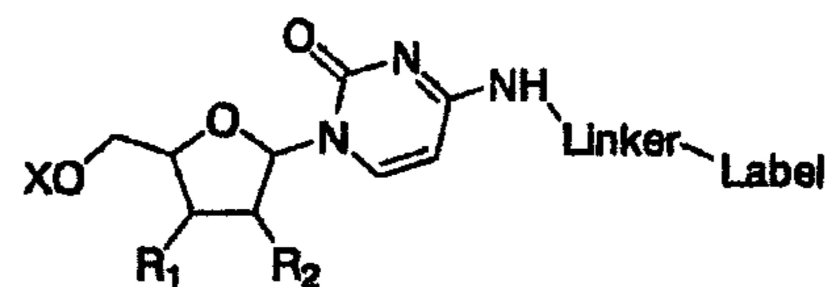
Cytidine N4-linker
