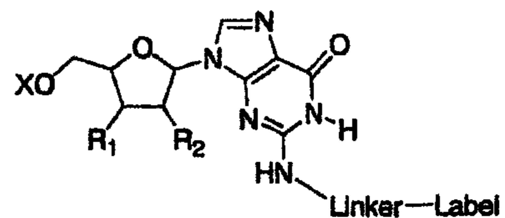
Guanosine N2-linker
