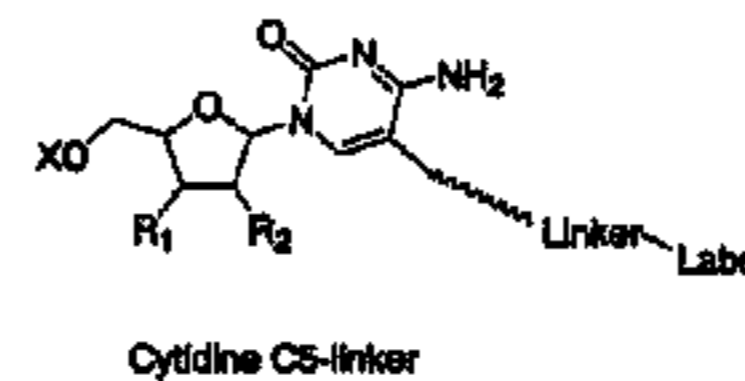
Cytidine C5-linker
