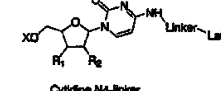
Cytidine N4-linker
