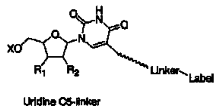
Uridine C5-linker
