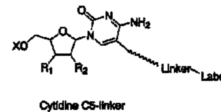
Cytidine C5-linker
