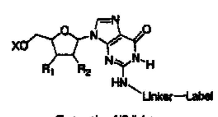
Guanosine N2-linker
