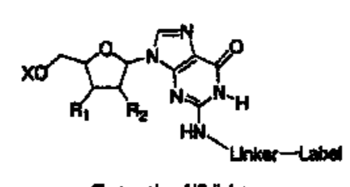
Guanosine N2-linker
