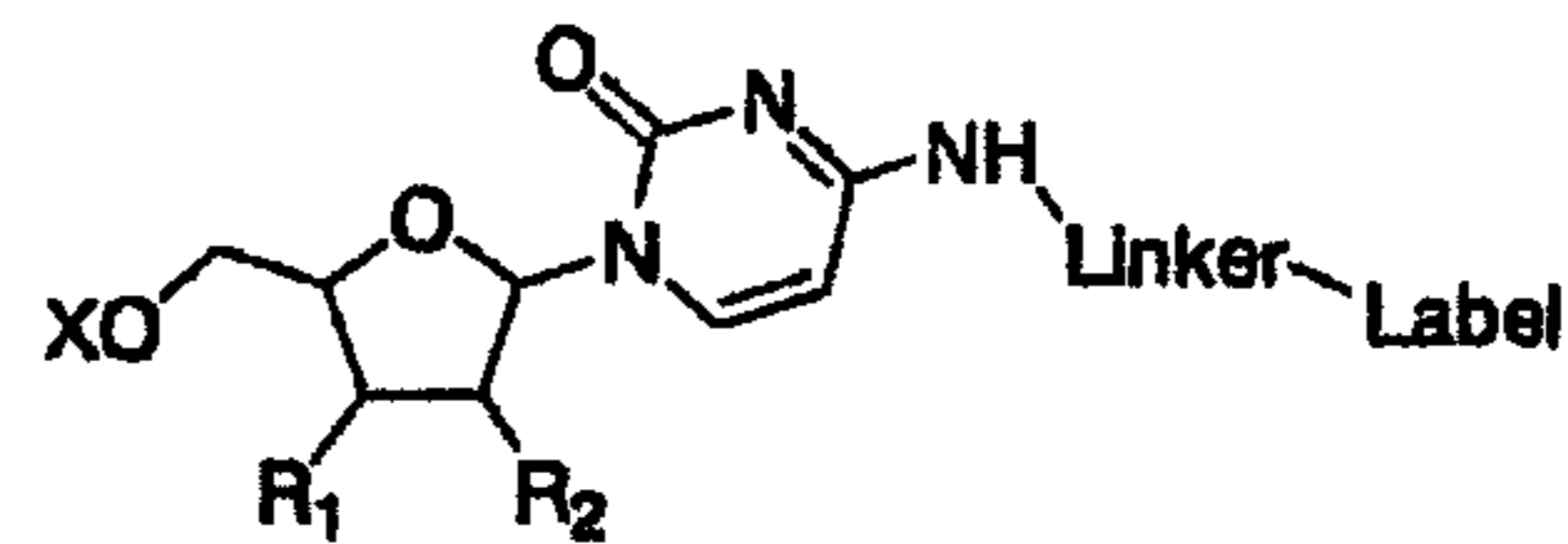
Cytidine N4-linker
