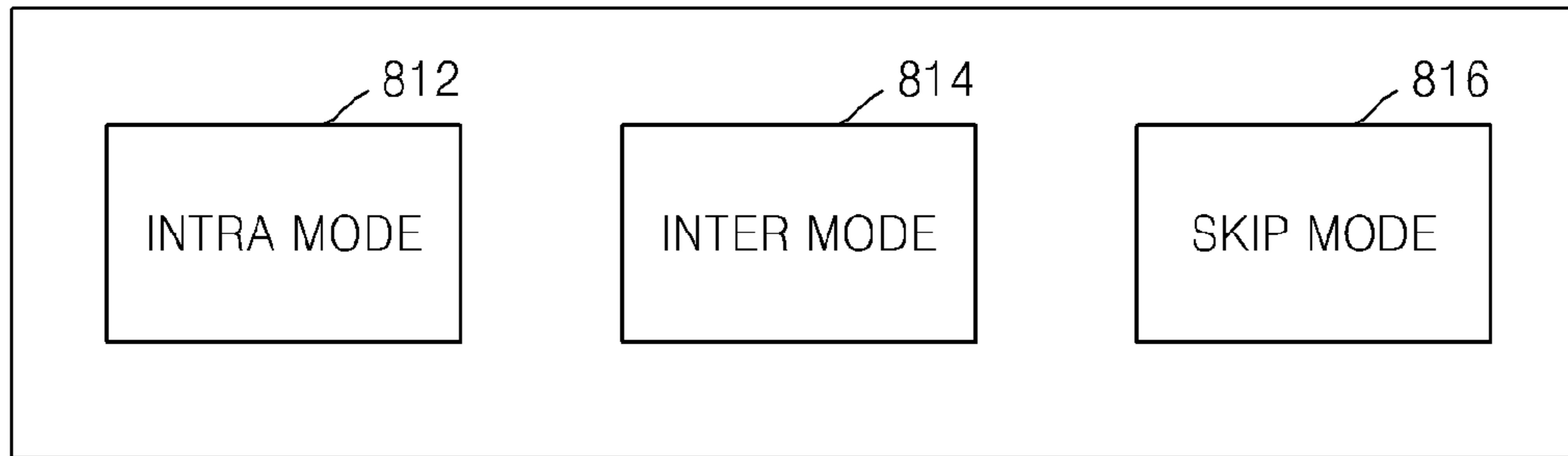
'PREDICTION MODE'-INFORMATION (810)
