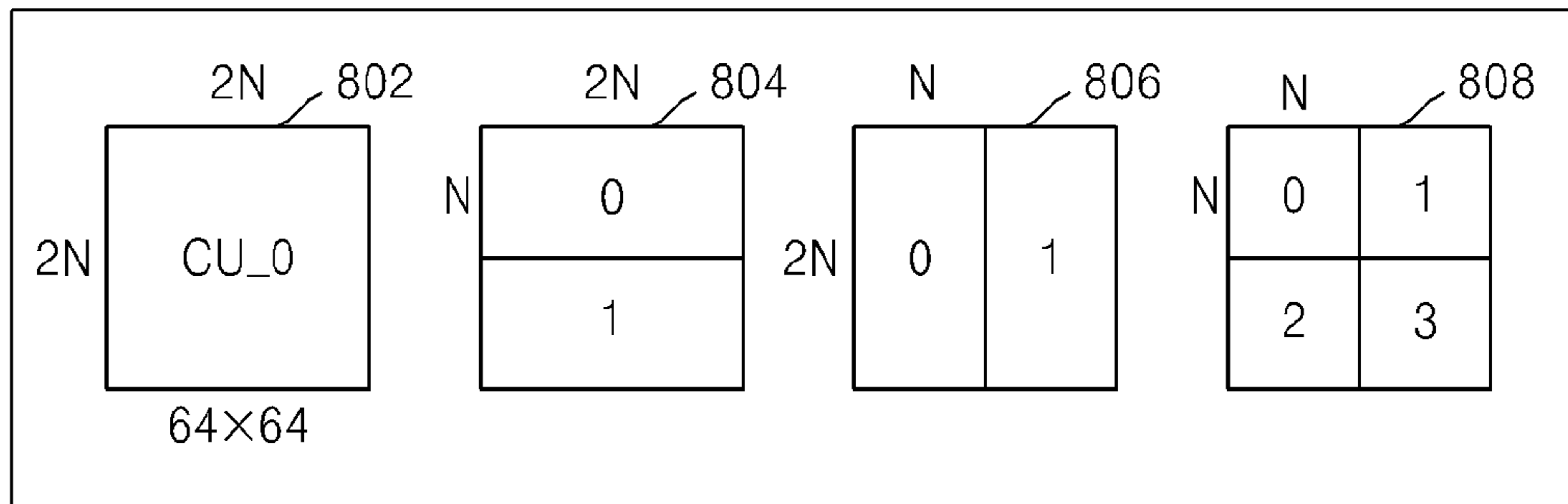
'PARTITION TYPE'-INFORMATION (800)
