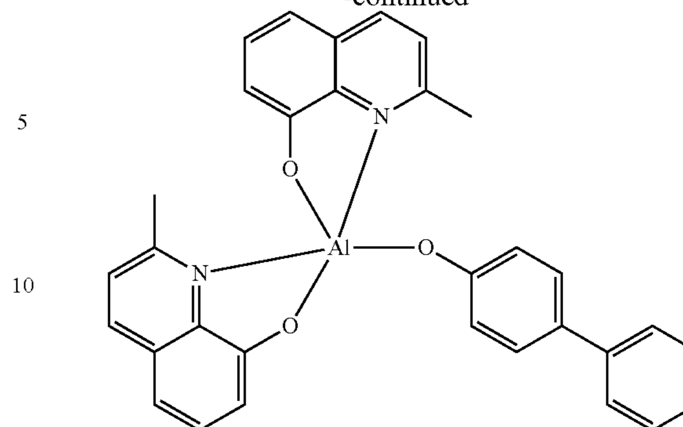
Bis-(2-methyl-8-quinolinolato)-4-(phenyl-phenolato)-aluminium-(III)
