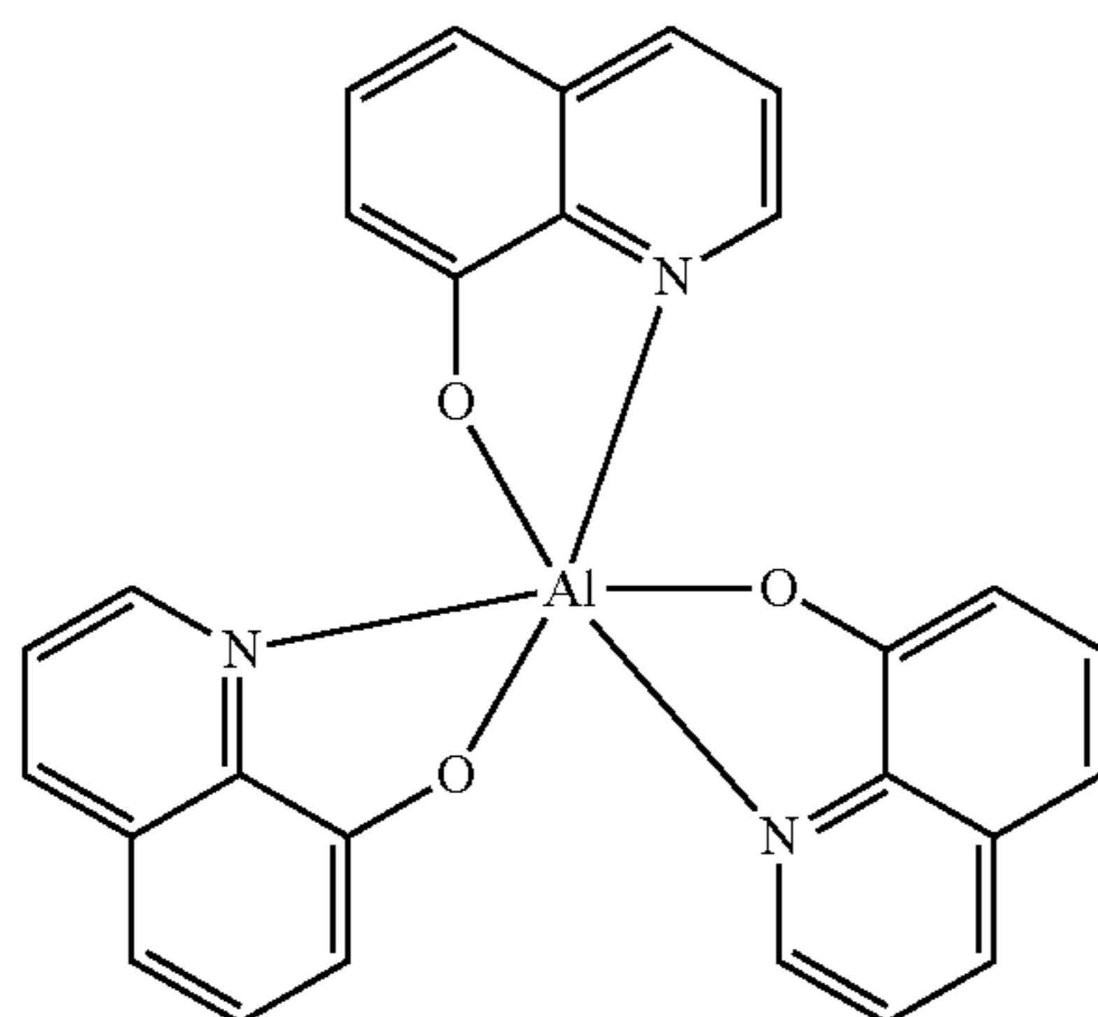
tris (8-hydroxy-quinolinato)-aluminium
