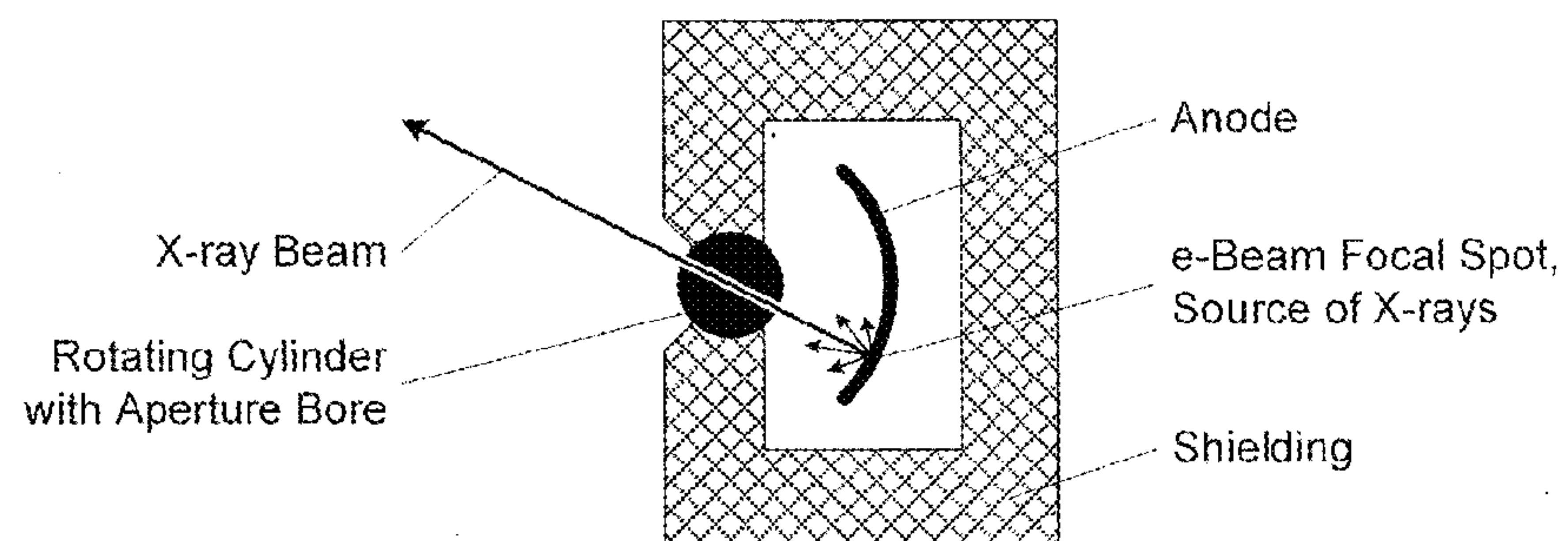
Fig. 1C (Prior Art)
