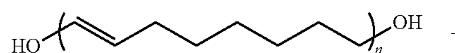
Scheme 3.
