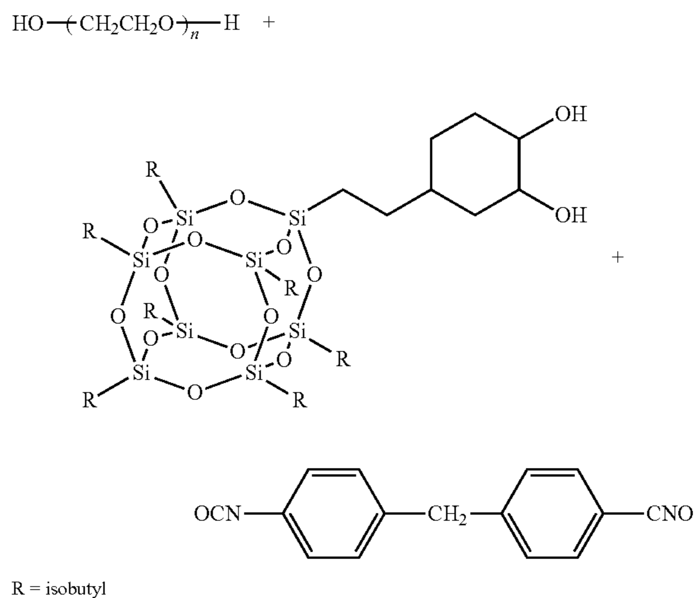
Scheme 1.
