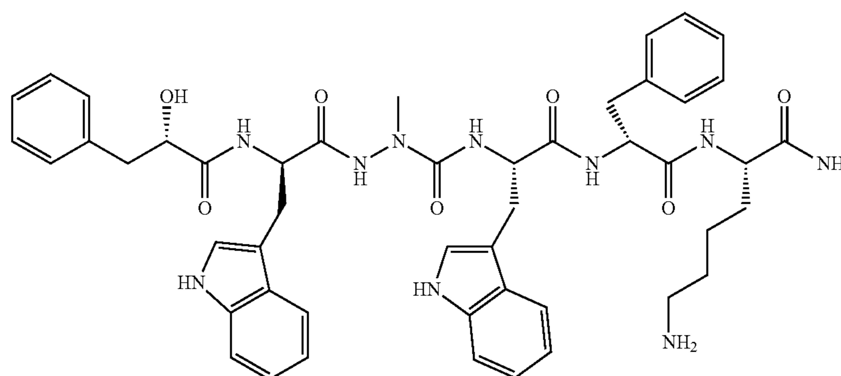
Ph-CH 2 -CH(OH)-CO-D-Trp-azaAla-Trp-D-Phe-Lys-NH 2
