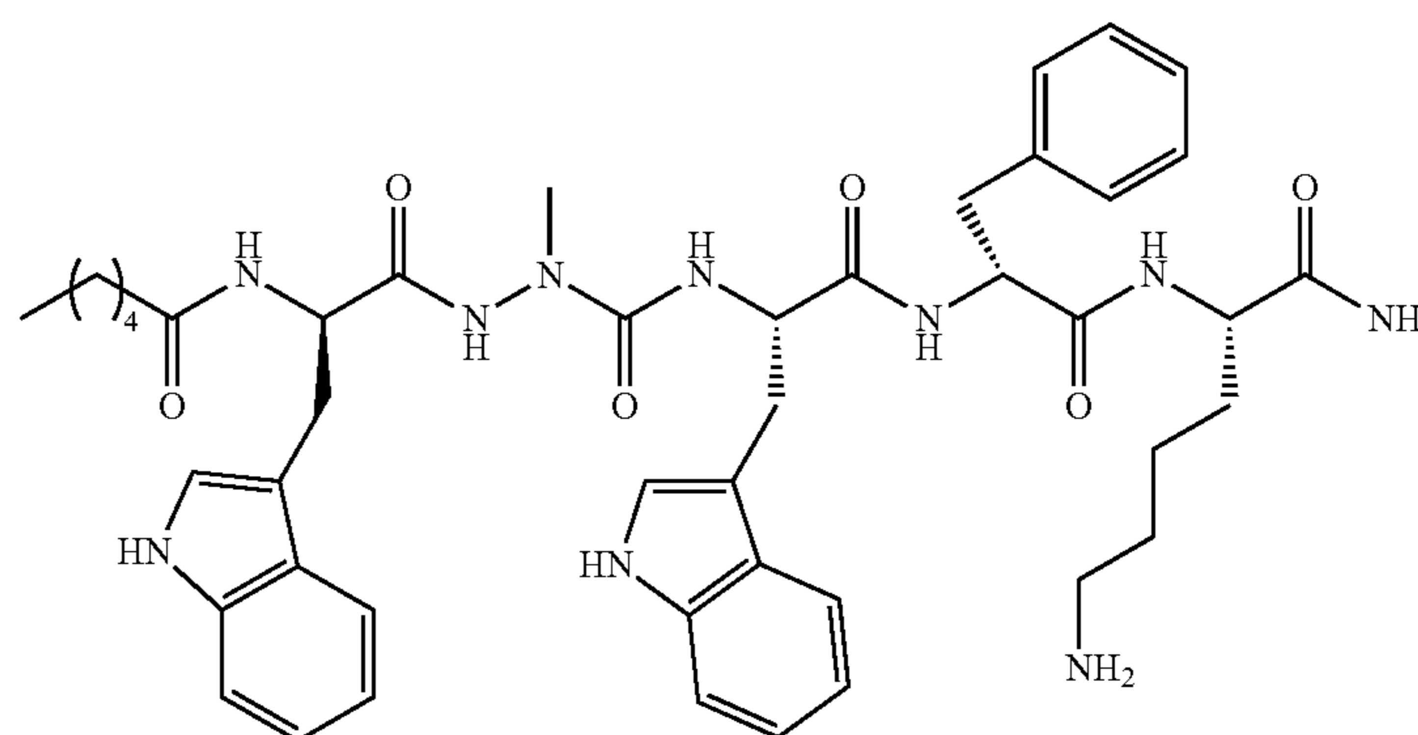
\text{CH}_3(\text{CH}_2)_4\text{CO-D-Trp-azaAla-D-Phe-Lys-NH}_2
