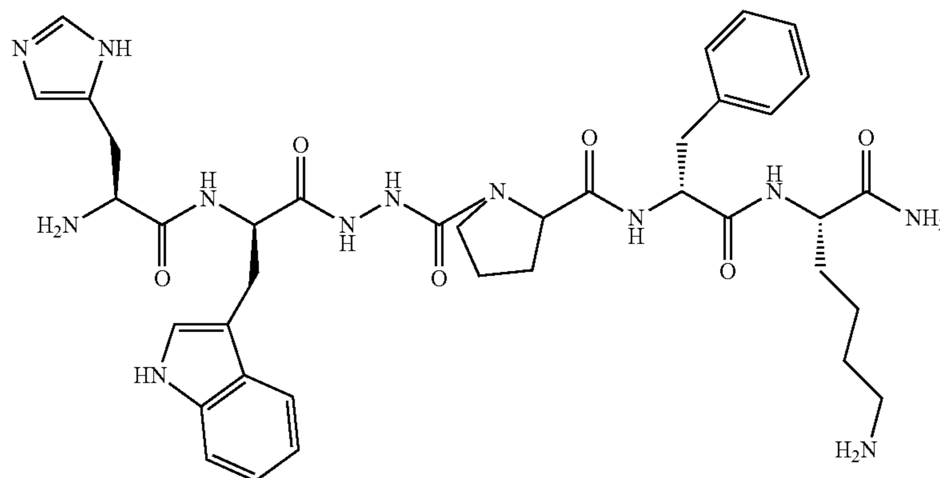
His-D-Trp-azaGly-Pro-D-Phe-Lys-NH 2
