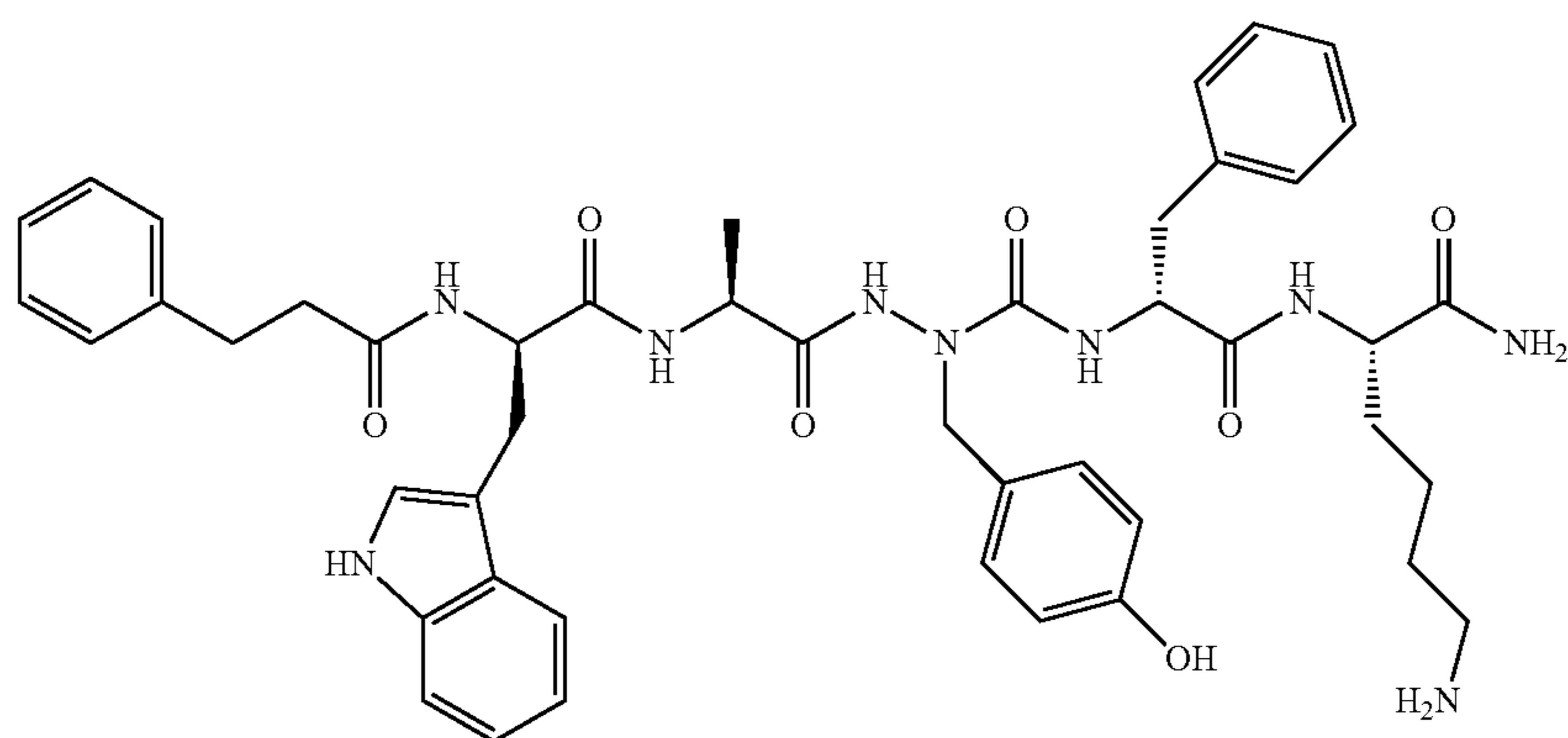
Hydrocinnamyl-D-Trp-Ala-AzaPhe-D-Phe-Lys-NH 2
