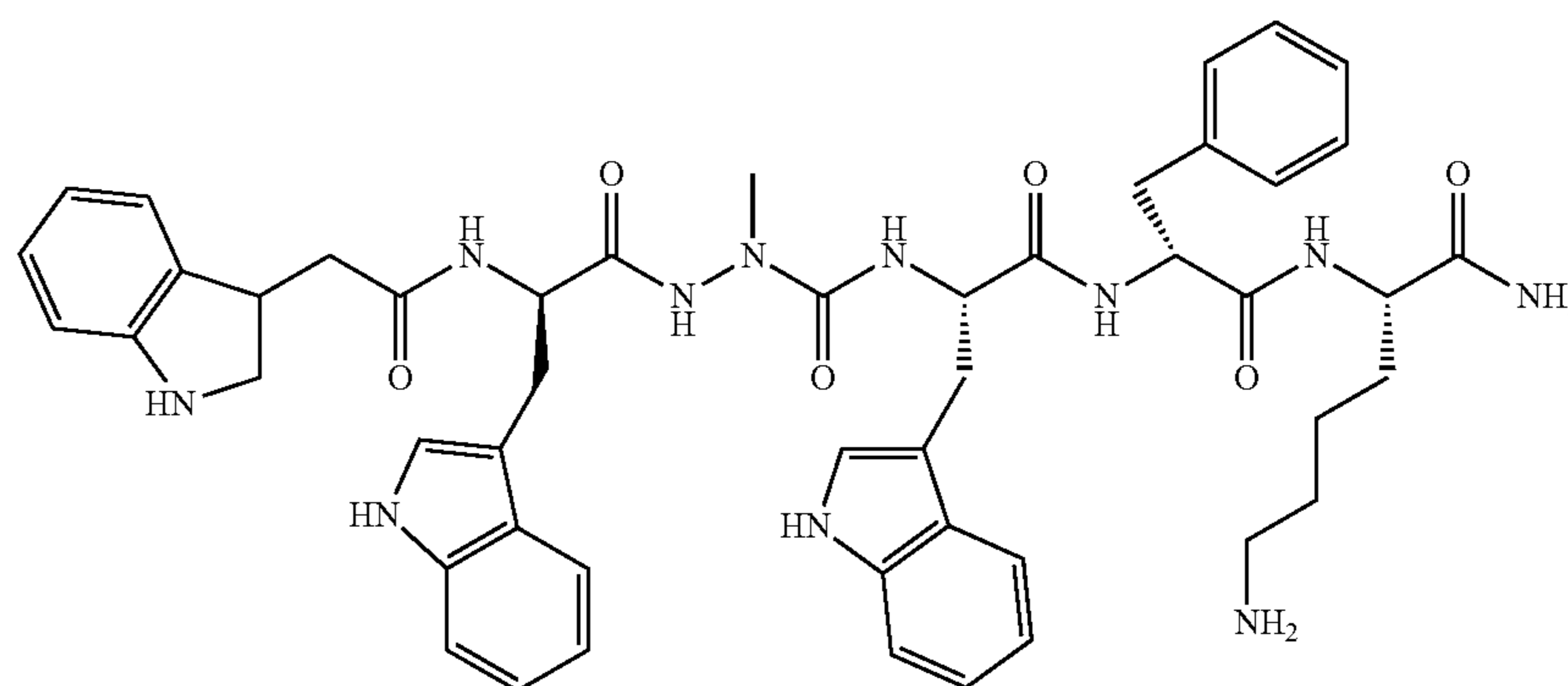
In-CO-D-Trp-azaAla-Trp-D-Phe-Lys-NH 2
