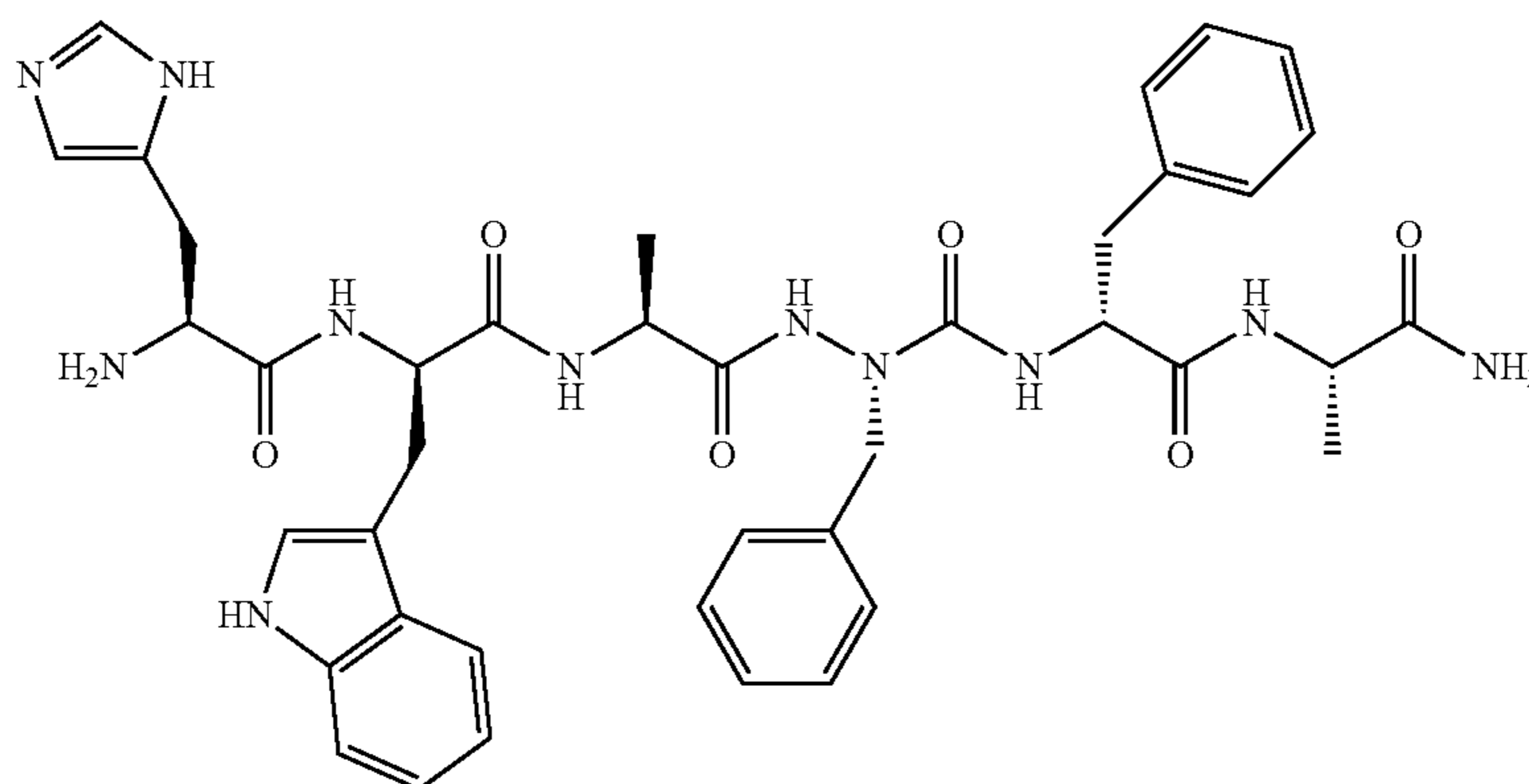
His-D-Trp-Ala-azaPhe-D-Phe-Ala-NH 2
