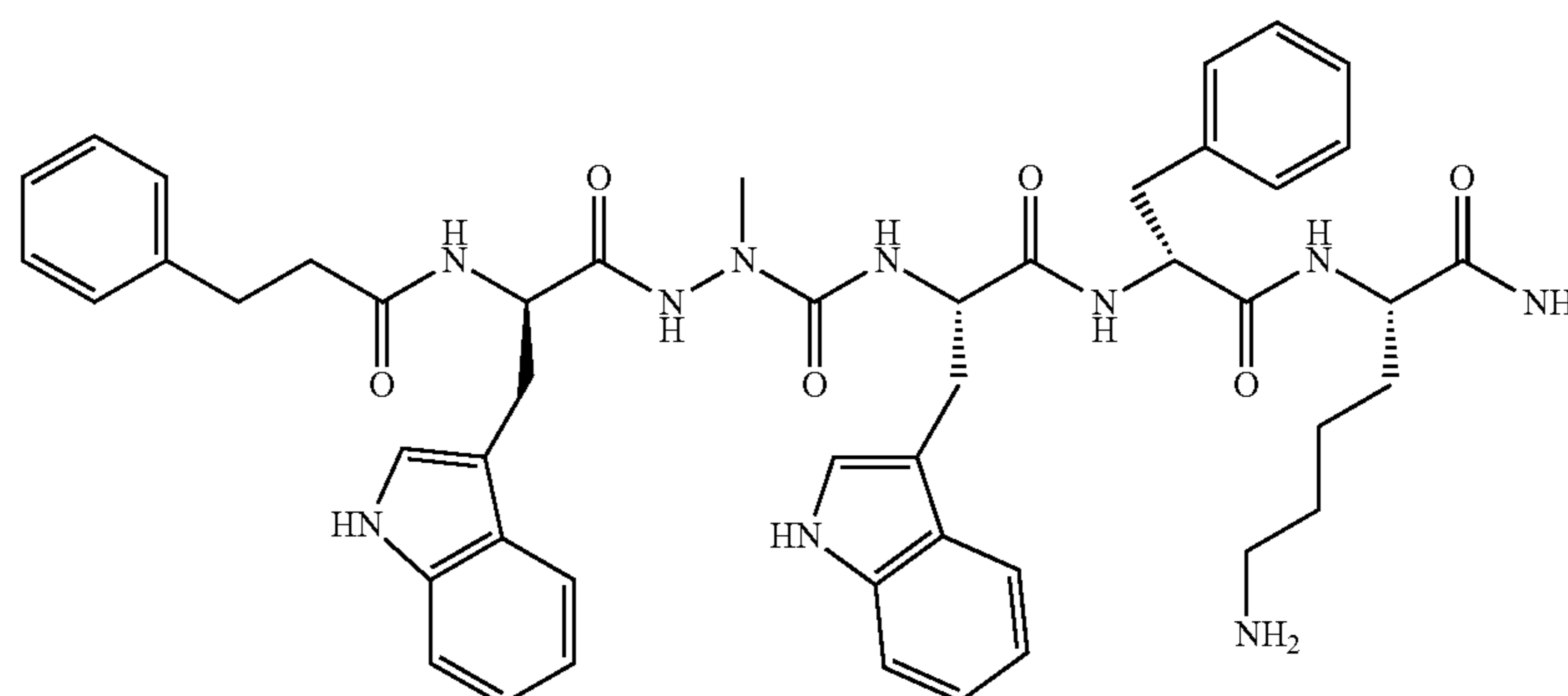
\text{Ph}-(\text{CH}_2)_2-\text{CO-D-Trp-azaAla-Trp-D-Phe-Lys-NH}_2
