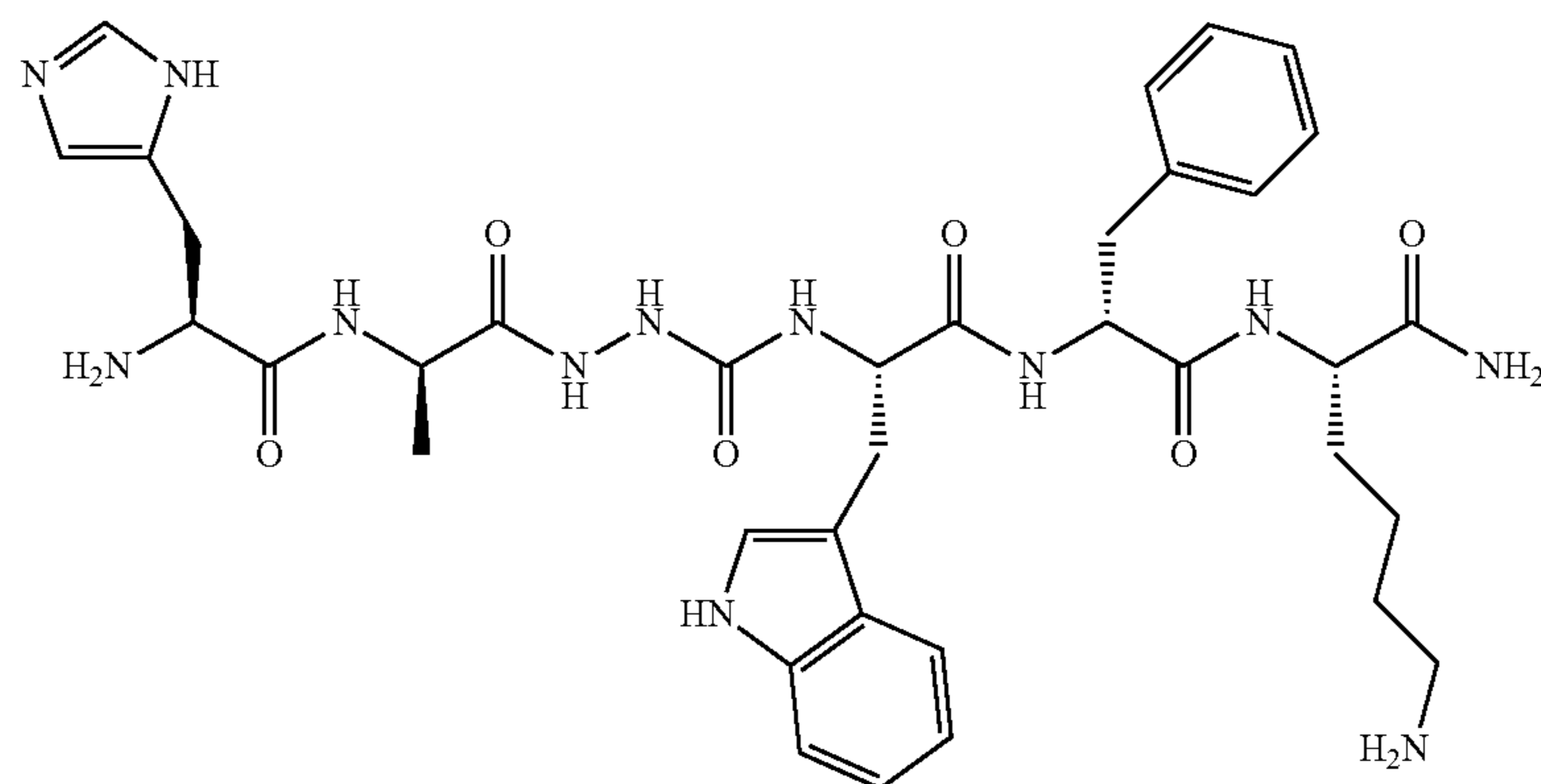
His-D-Ala-azaGly-Trp-D-Phe-Lys-NH 2
