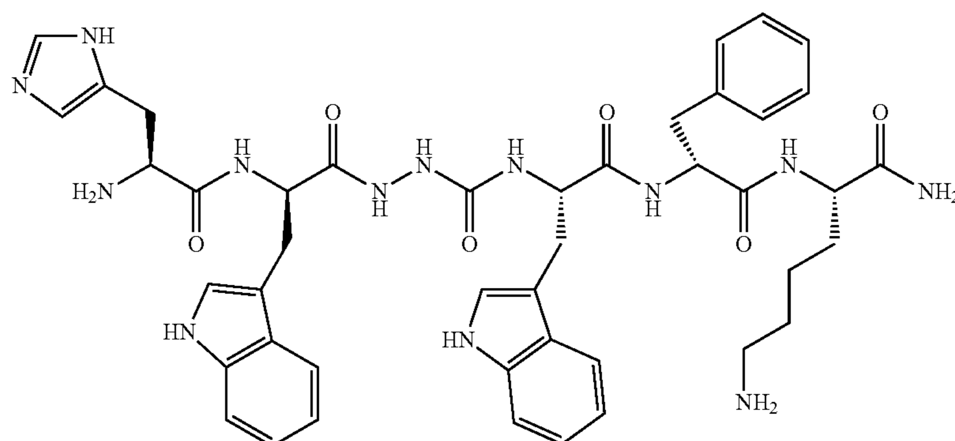
His-D-Trp-azaGly-Trp-D-Phe-Lys-NH 2
