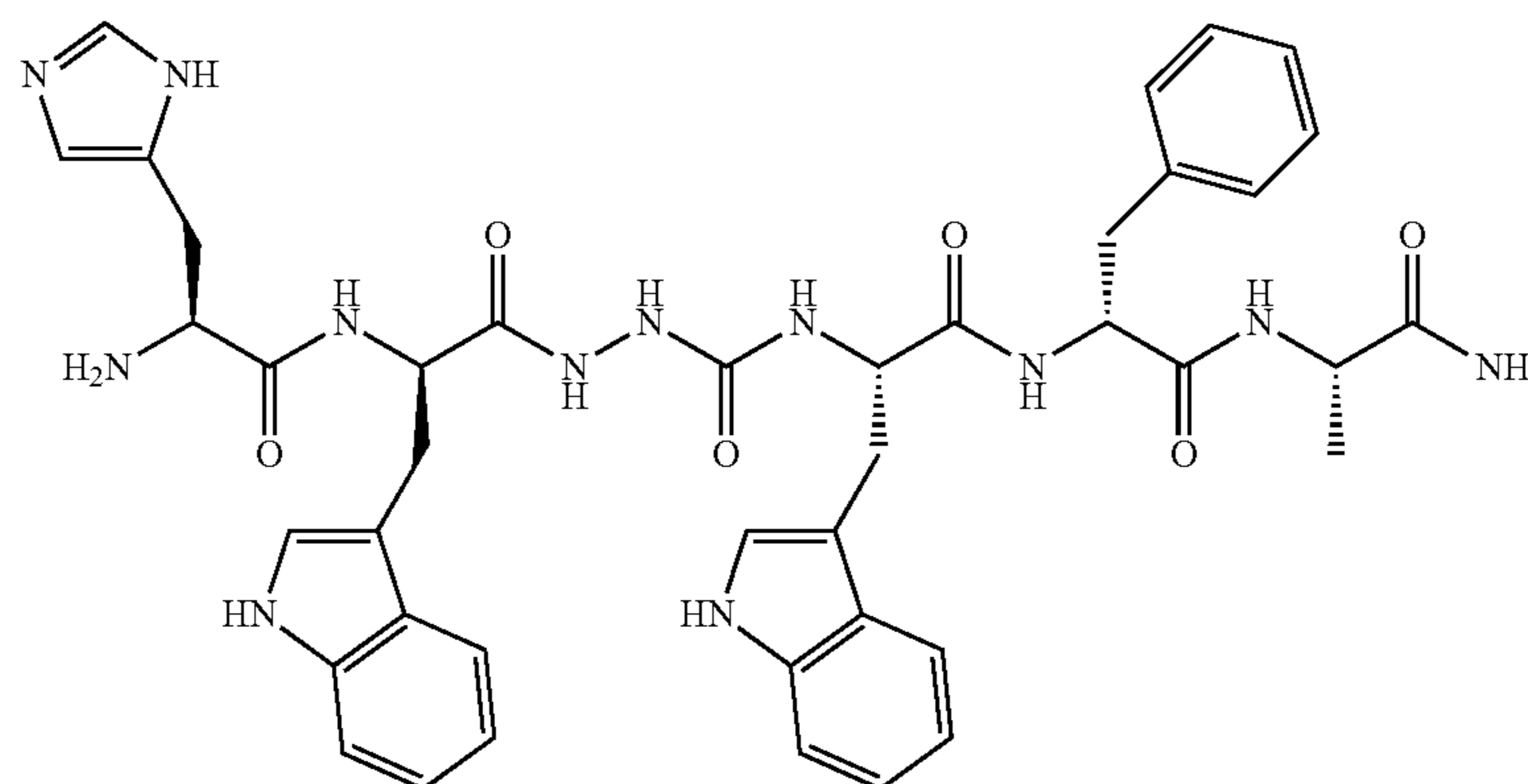
His-D-Trp-azaGly-Trp-D-Phe-Ala-NH 2
