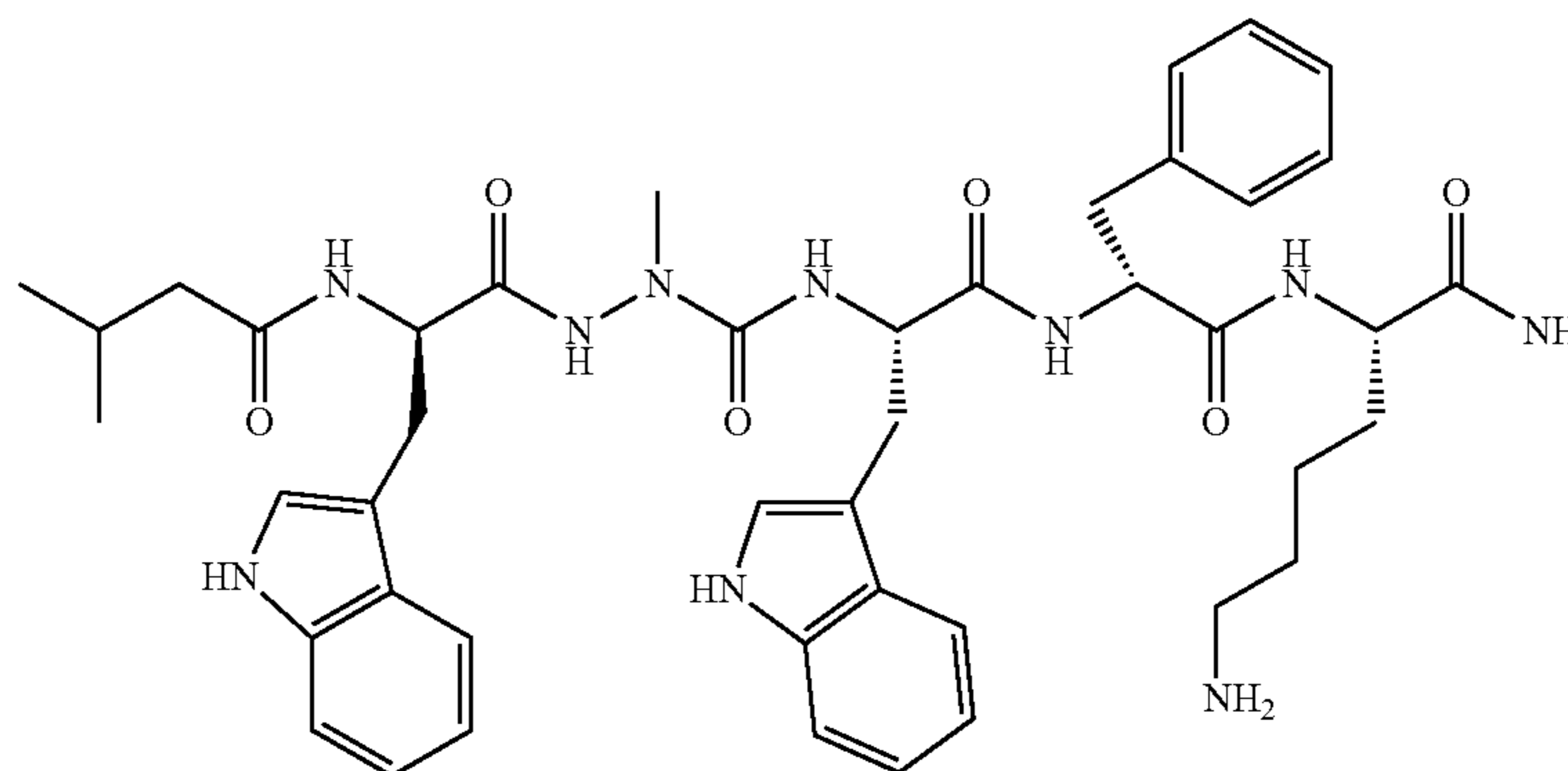
(\text{CH}_3)_2\text{CHCH}_2\text{CO-D-Trp-azaAla-D-Phe-Lys-NH}_2
