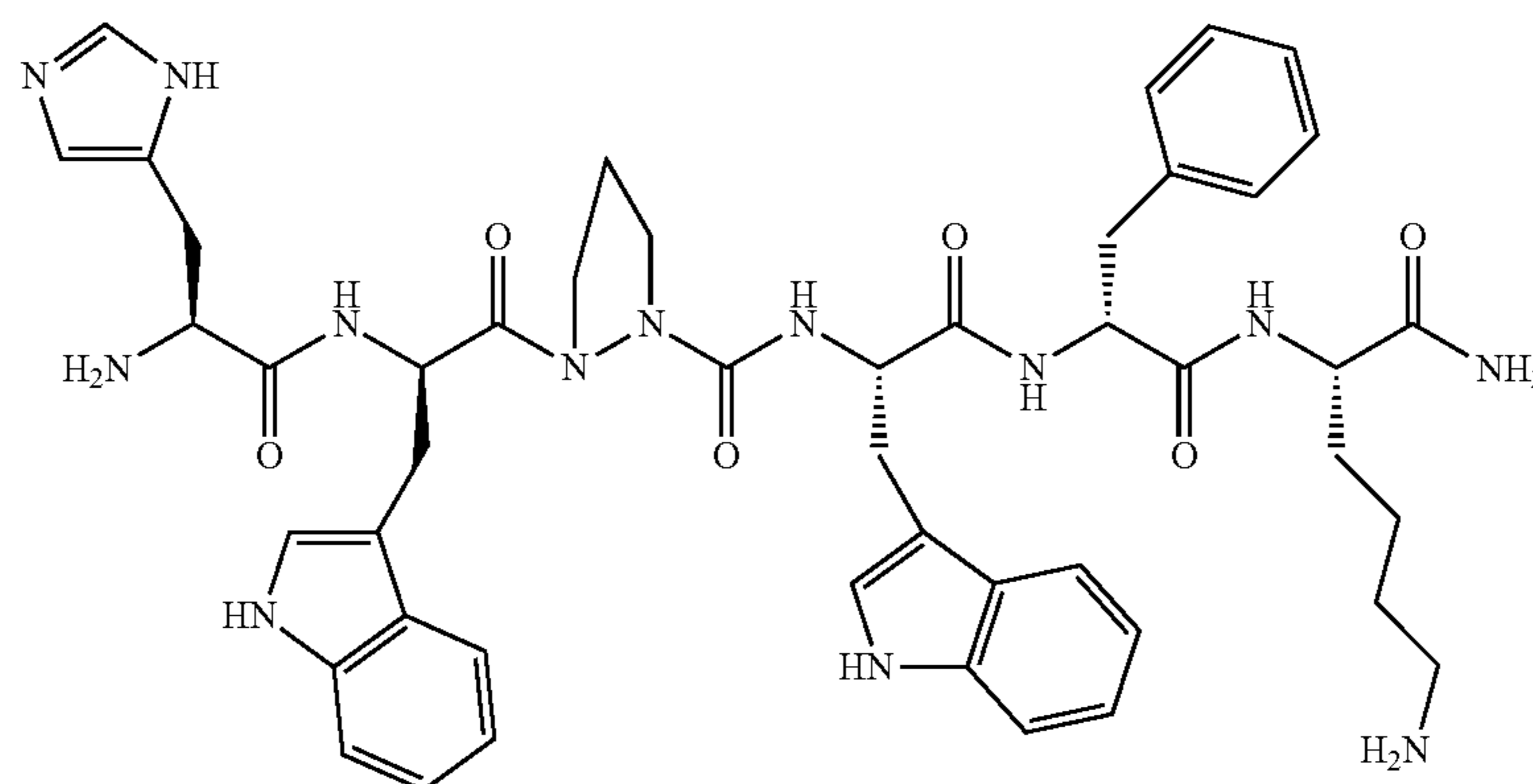
His-D-Trp-azaPro-Trp-D-Phe-Lys-NH 2
