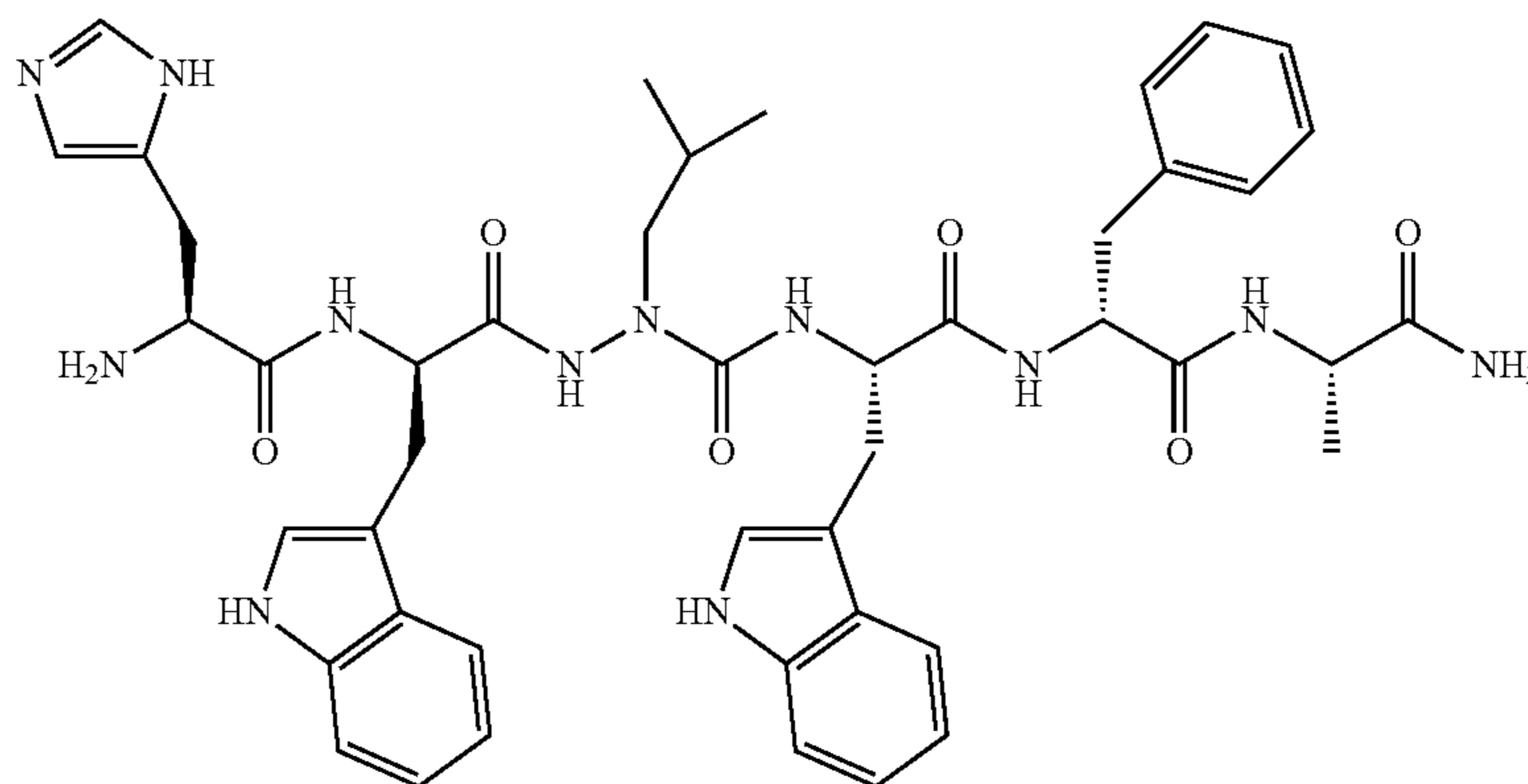
His-D-Trp-azaLeu-Trp-D-Phe-Ala-NH 2
