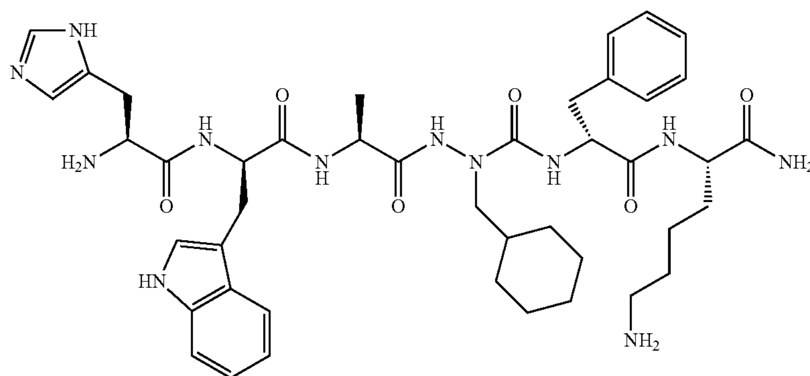
His-D-Trp-Ala-azaCha-D-Phe-Lys-NH 2
