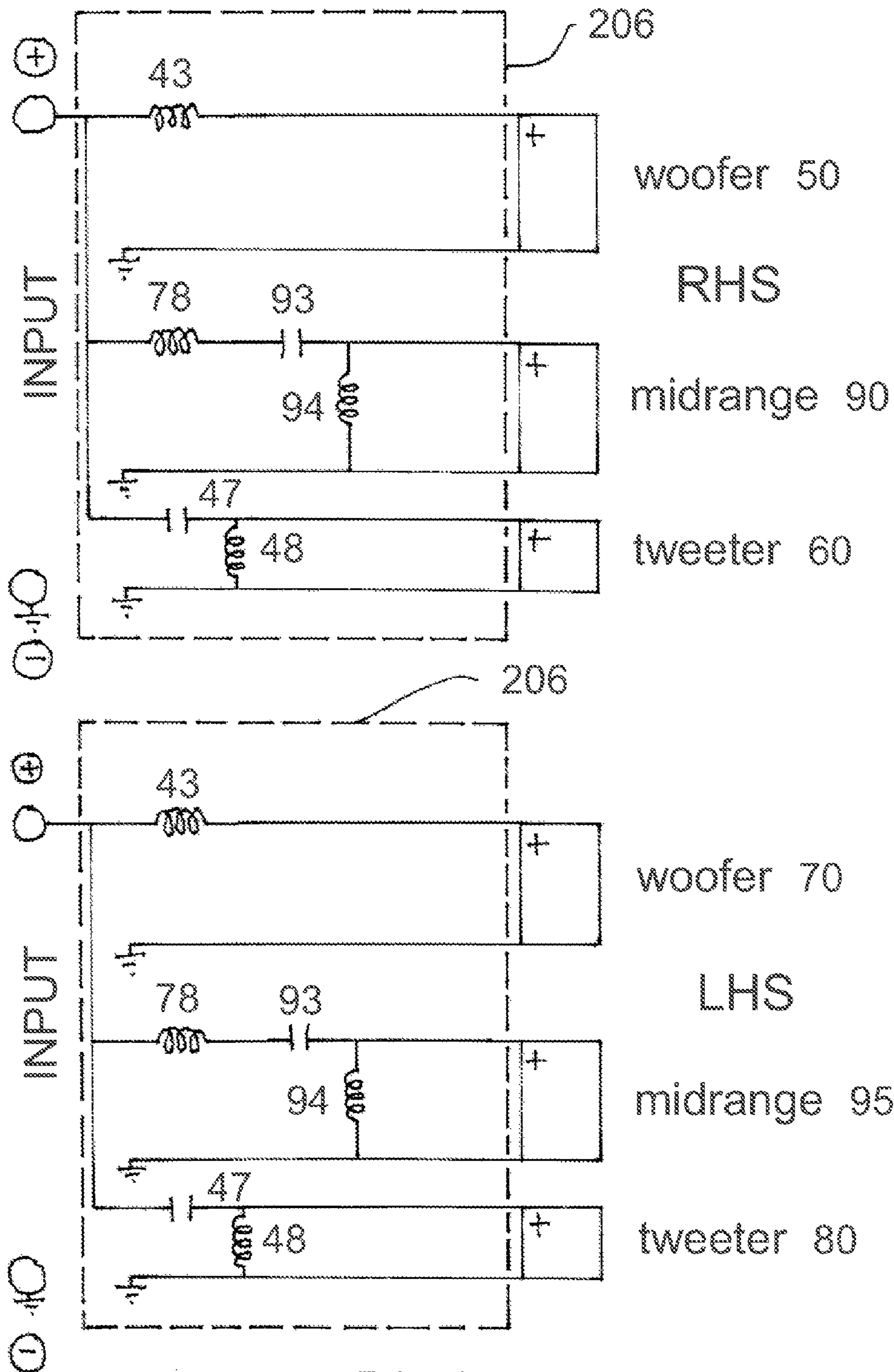
Prior Art Fig. 24
