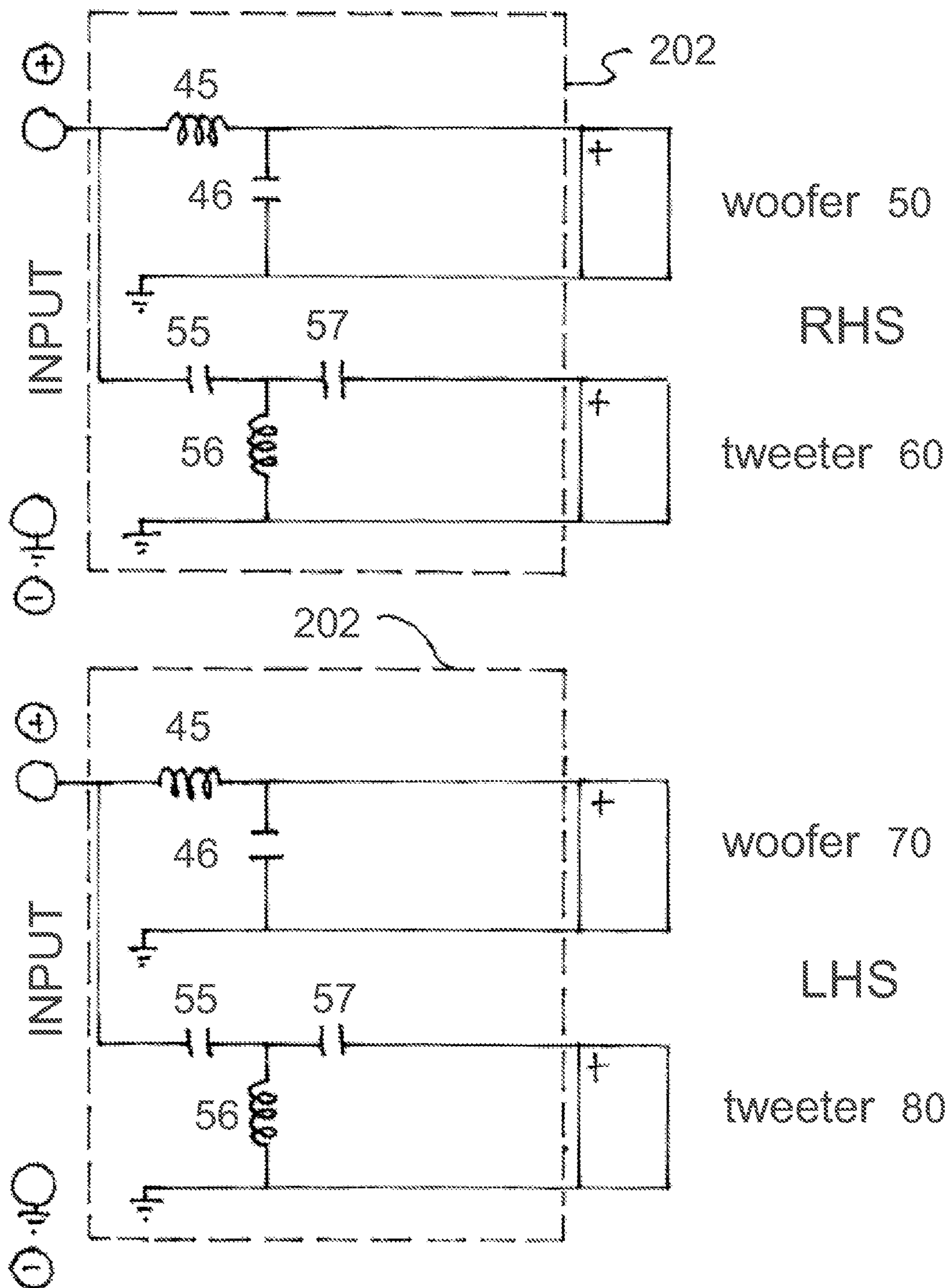
Prior Art Fig. 14
