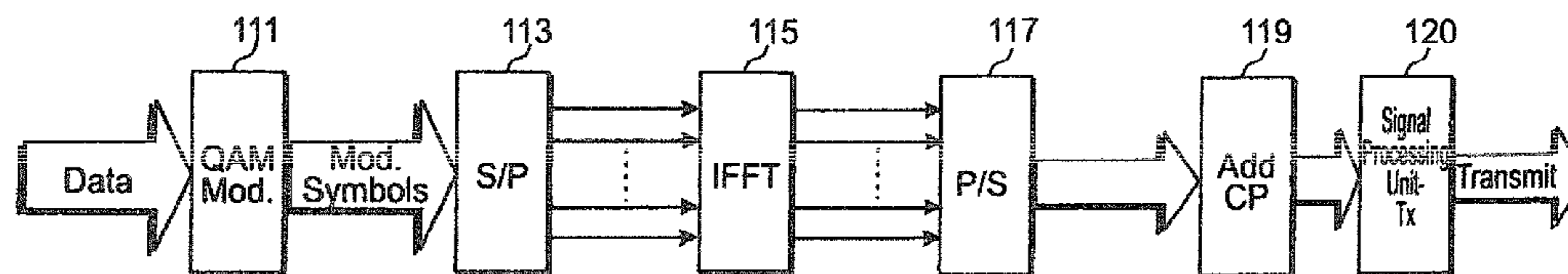
TRANSMITTER
