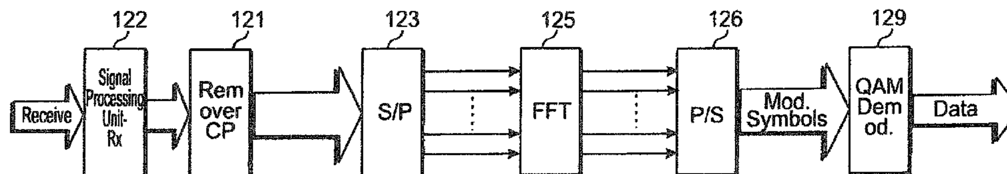
RECEIVER
