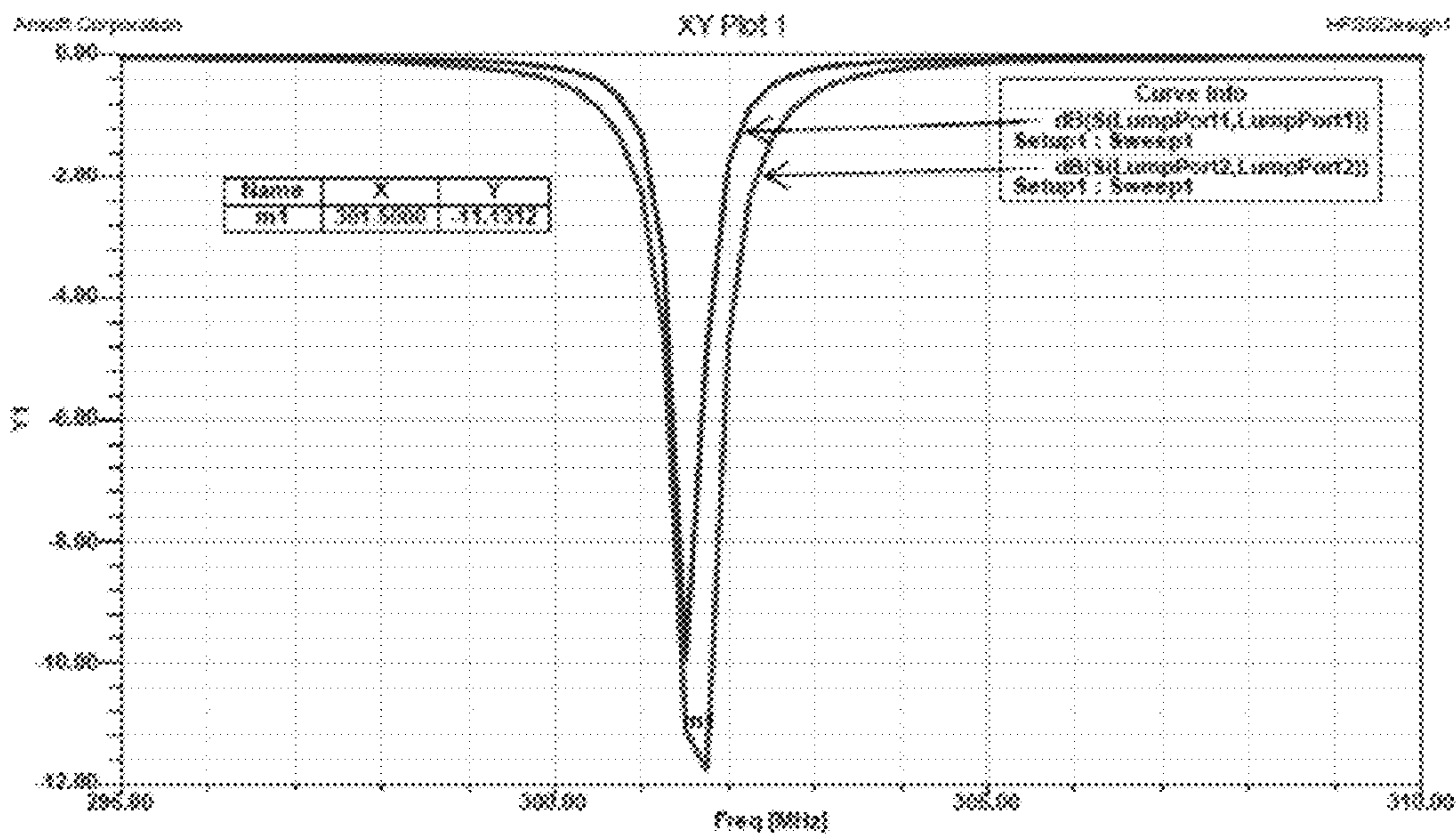
Return Loss seen at each RF Port (S11 and S22 in dB) as a function of frequency (MHz)
