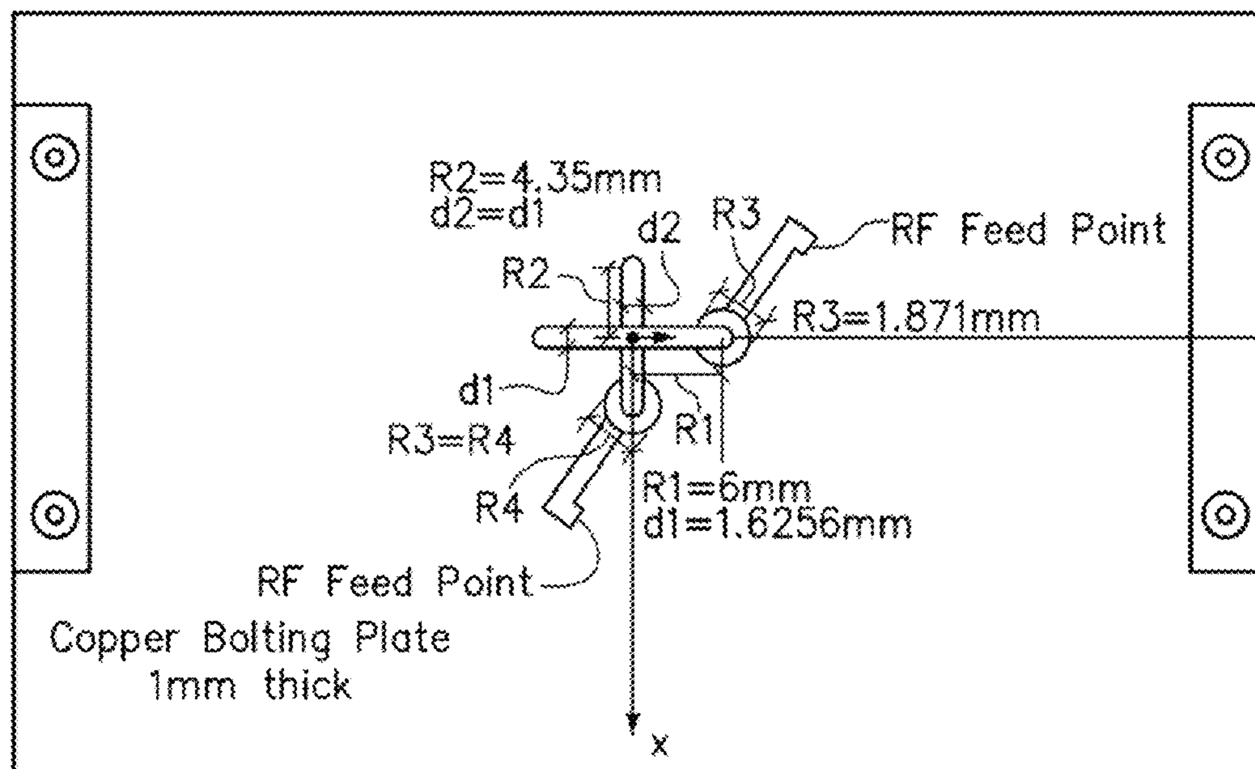
Copper Half Loops with Dimensions (cage removed)
