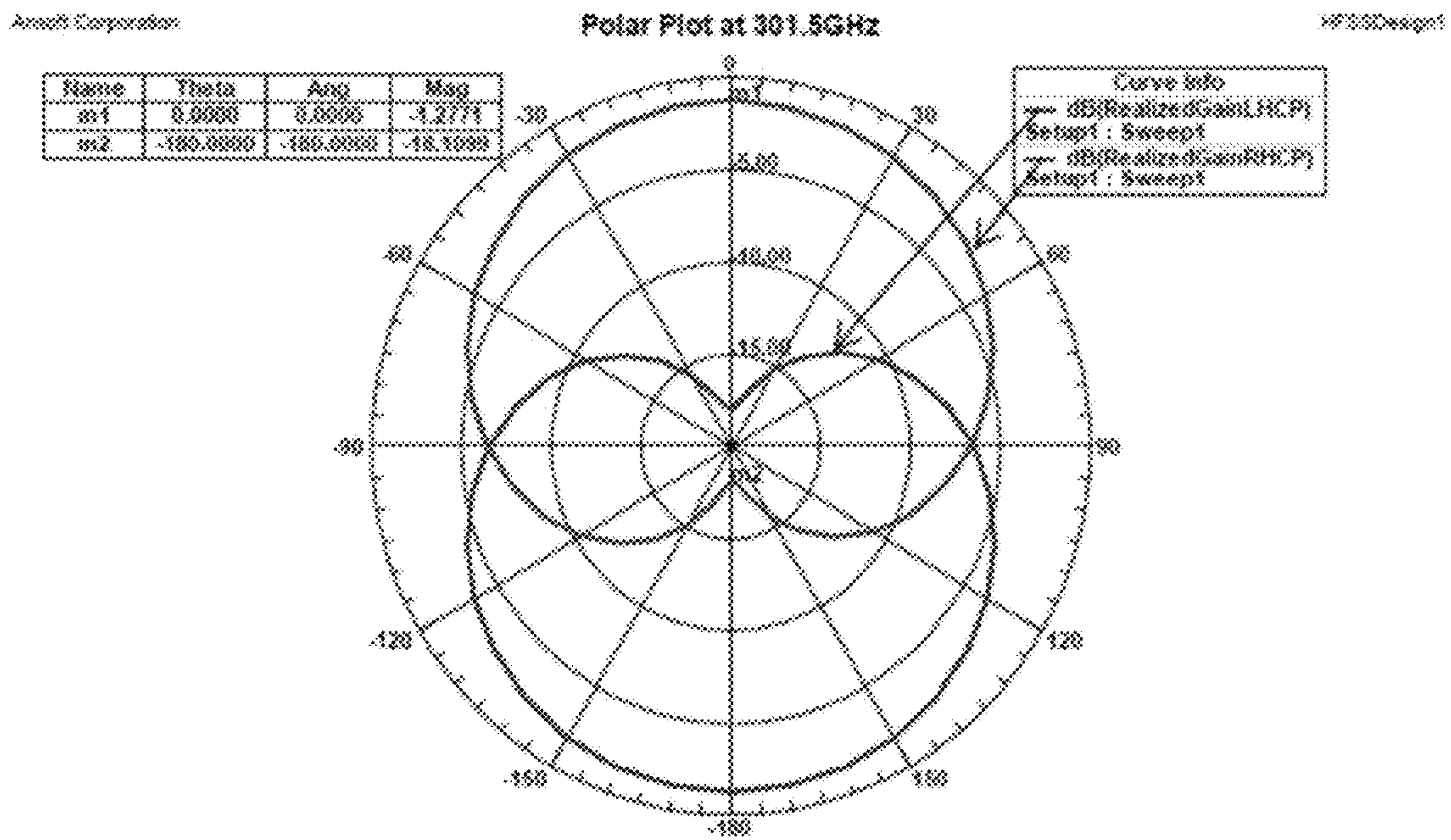
Polar Plot of Right Hand and Left Hand Circular Polarization (in dB) at 301.5MHz
