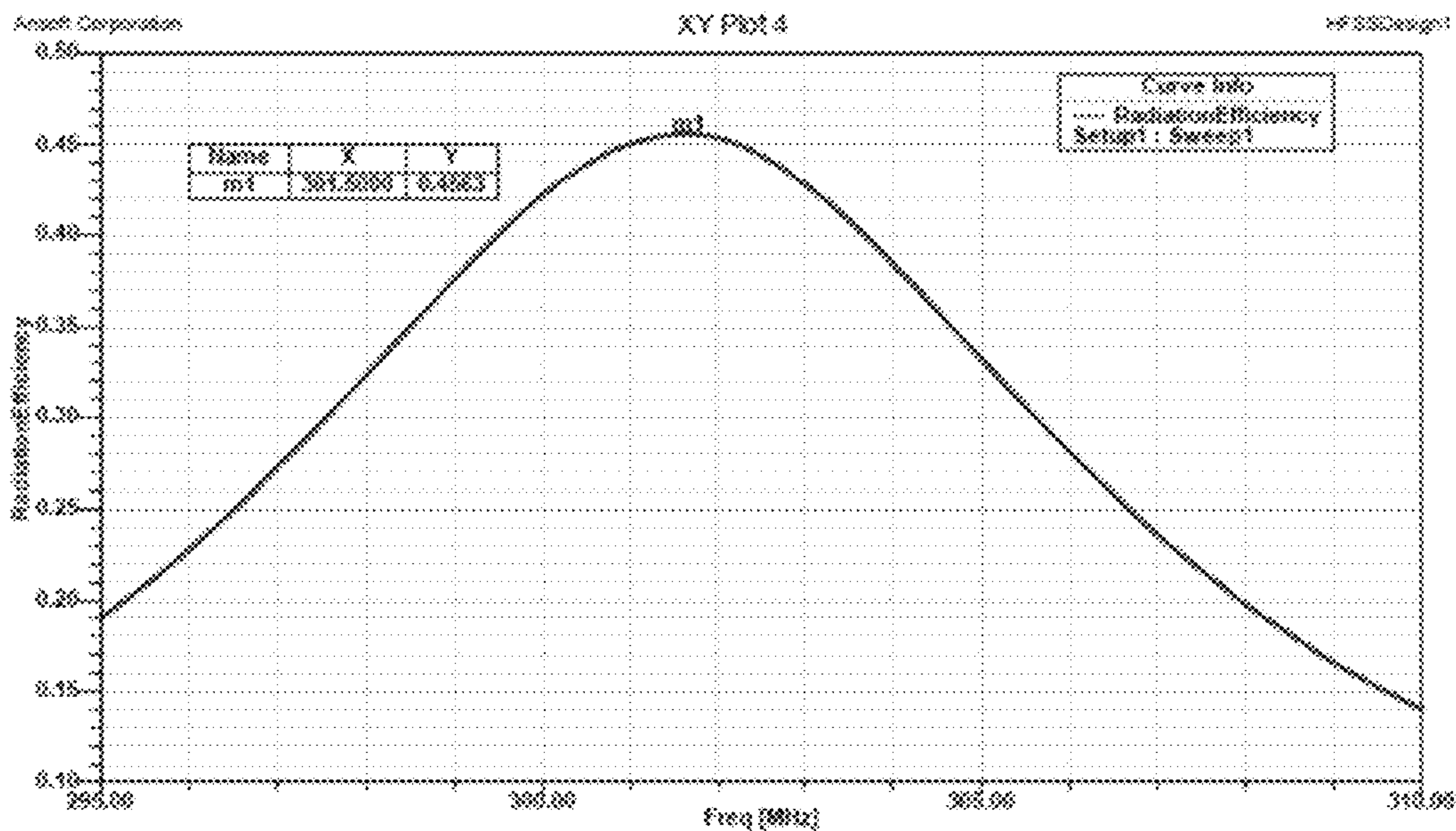
Radiation Efficiency of Antenna as a function of frequency (MHz) FIGURE 9
