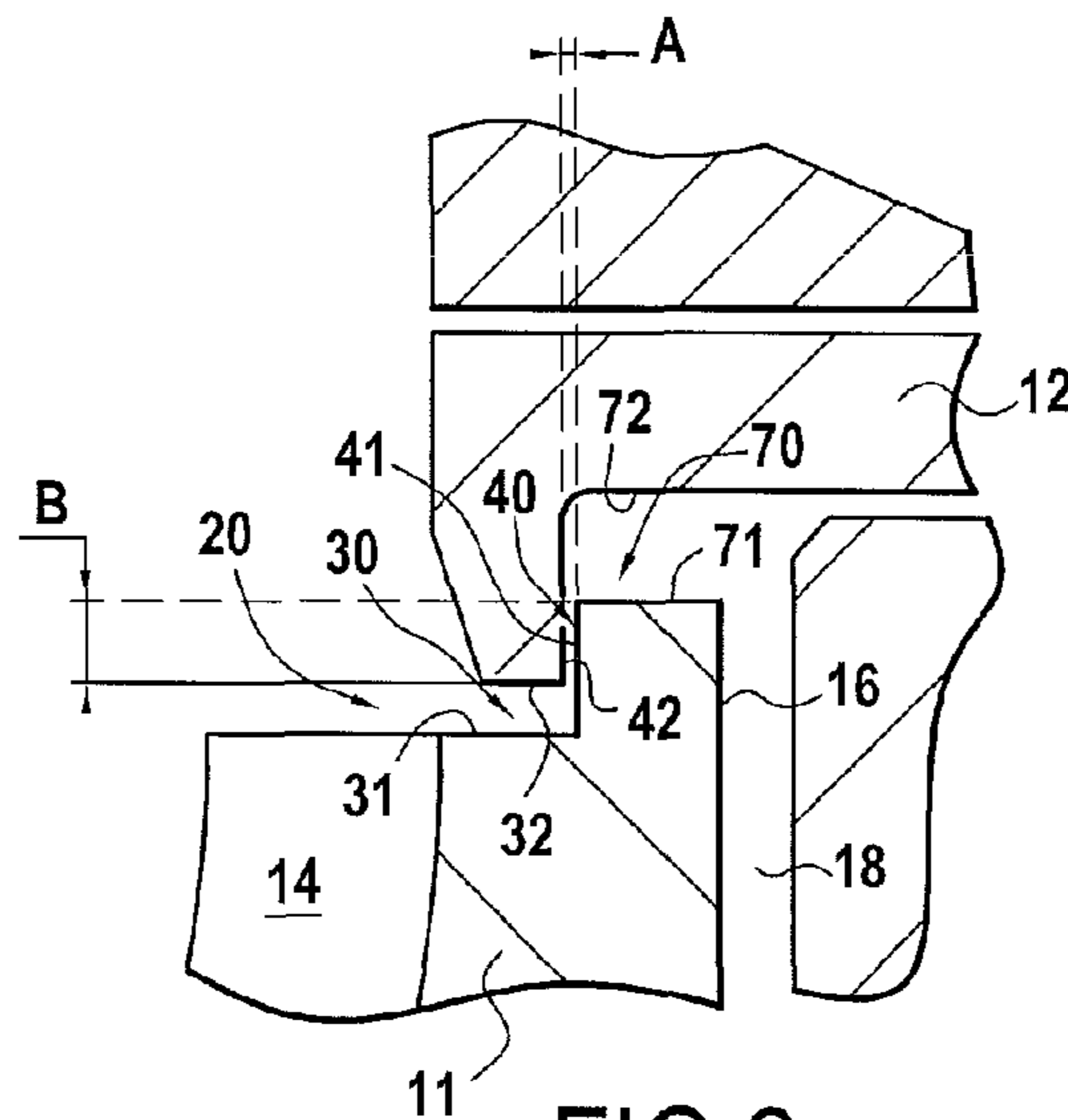
FIG. 2 PRIOR ART
