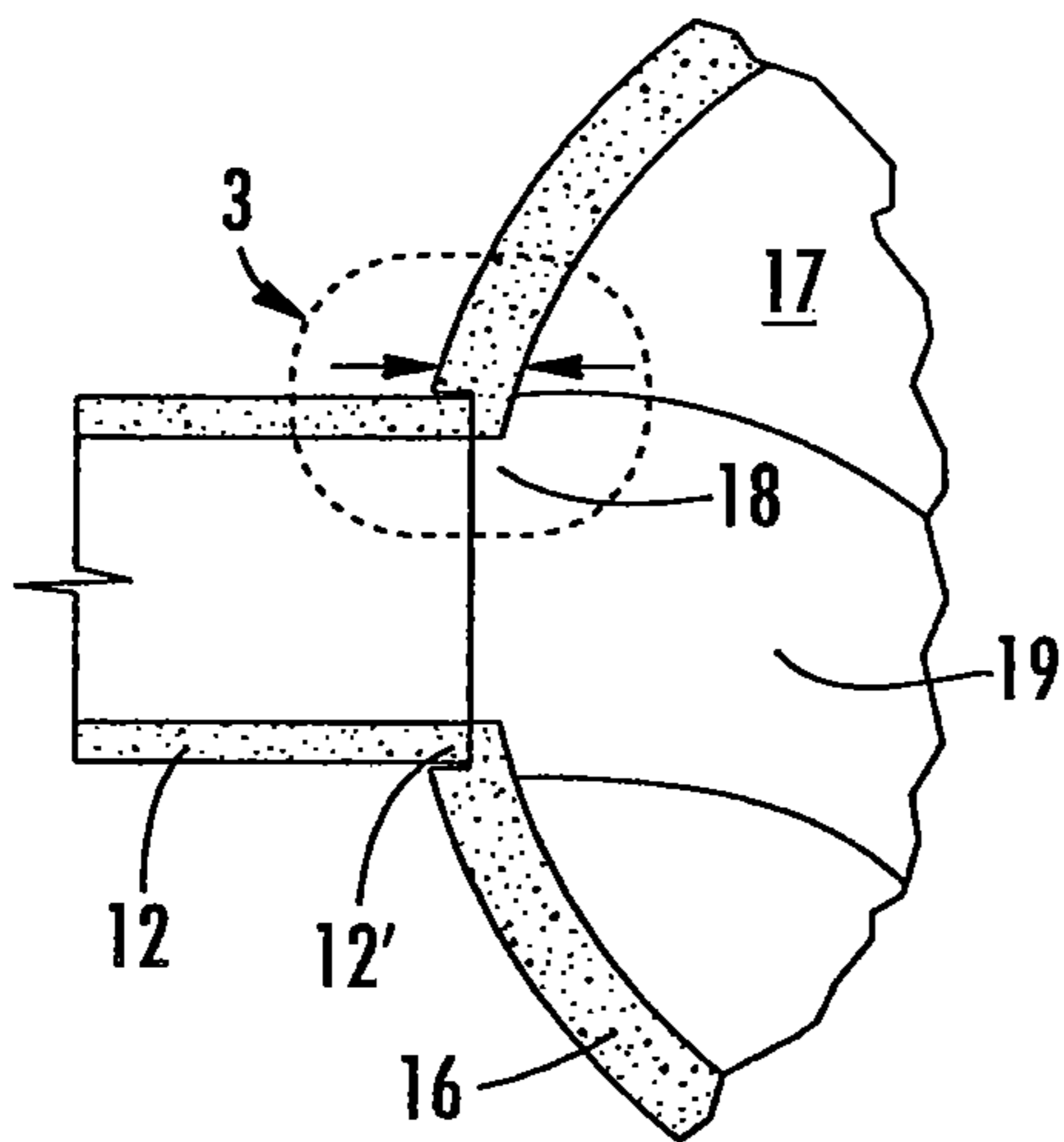
FIG. 2 PRIOR ART
