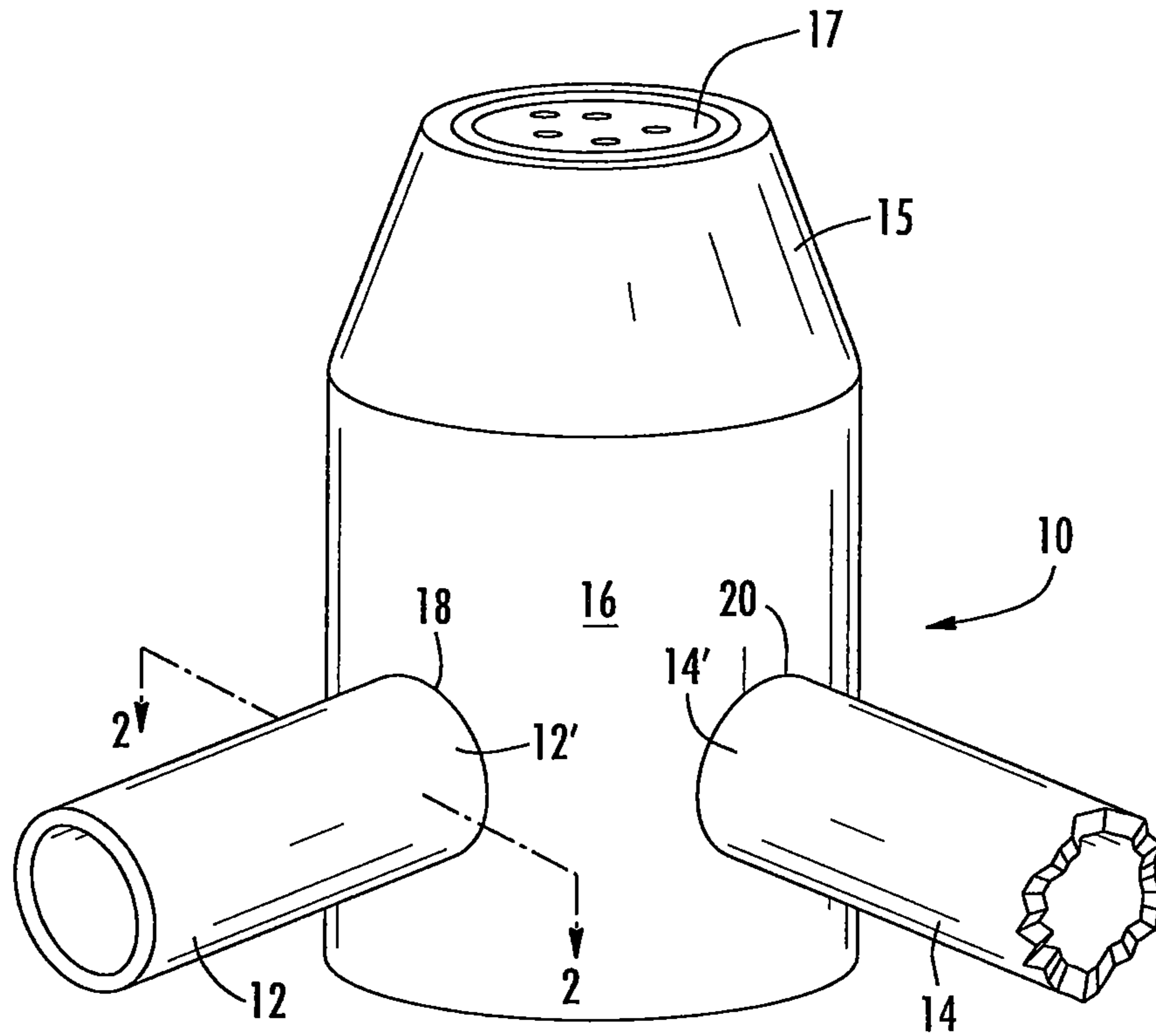
FIG. 1 PRIOR ART
