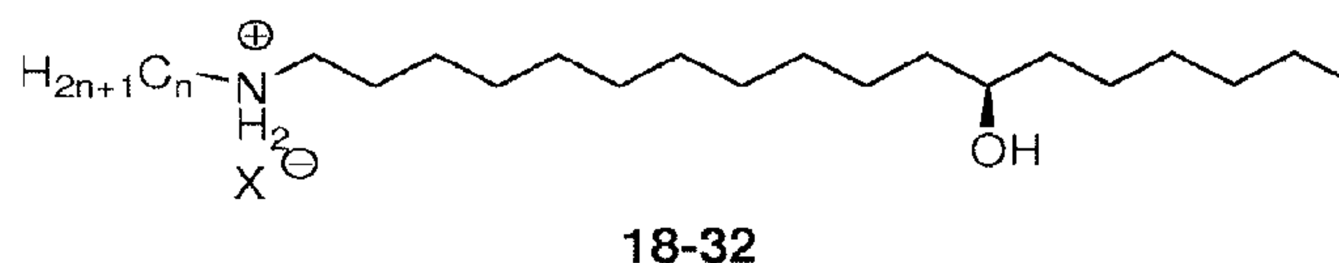
FIG. 48 Structures of gelators of the formulas: 18 to 24 ( n = 0 to 6 ), 25 ( n = 18 ) and X = Cl ; 26 ; n = 3 , X = Br ; 27 ; n = 3 , X = I ; 28 ; n = 3 , X = NO_3 ; 29 ; n = 3 , X = BF_4 ; 30 ; n = 3 , X = CH_3CO_2 ; 31 ; n = 3 , X = C_8H_{17}CO_2 ; 32 n = 3 , X = CO_2HCO_2 .
