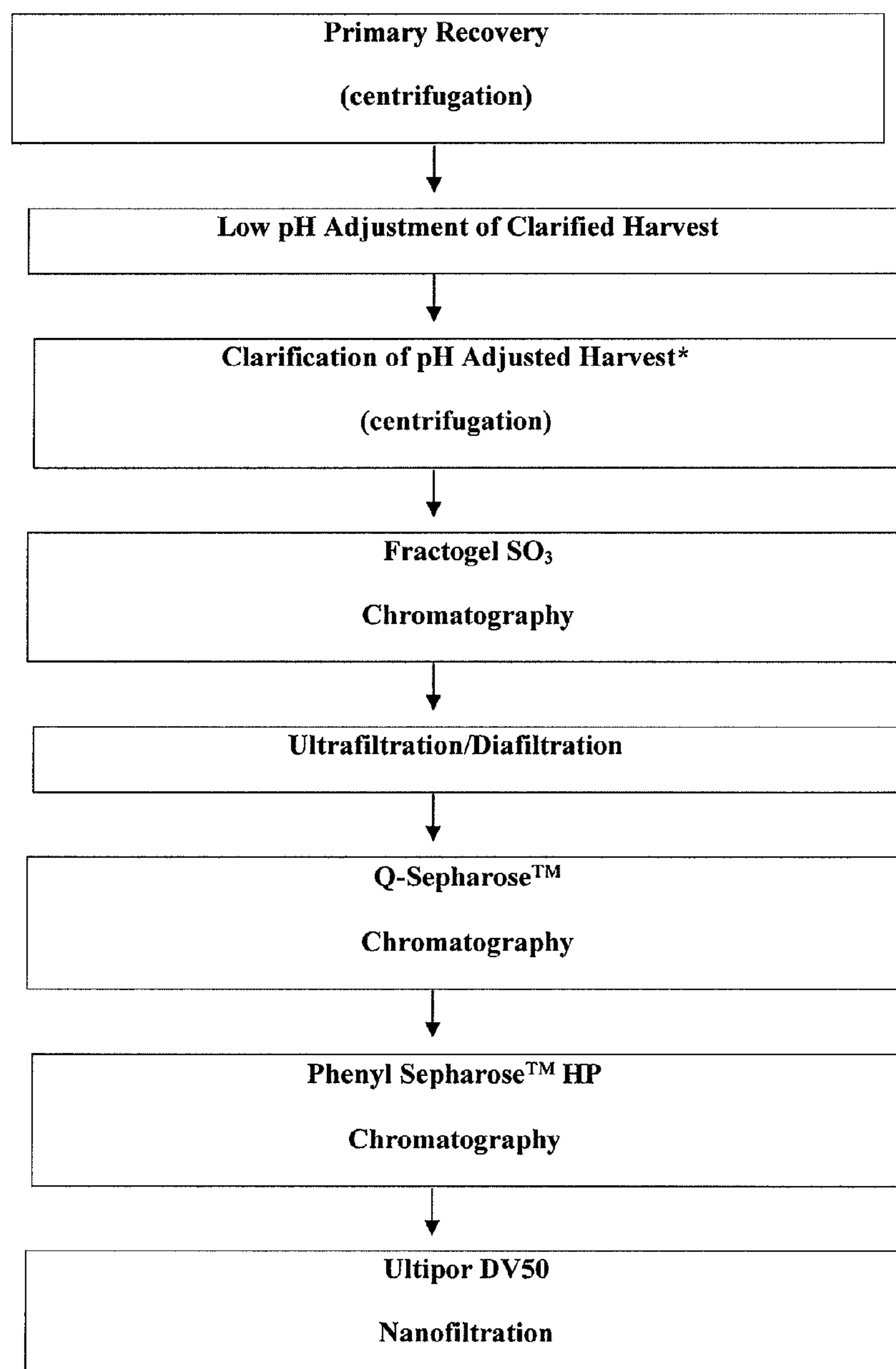
Figure 4. Process flow diagram for the purification of an antibody.
