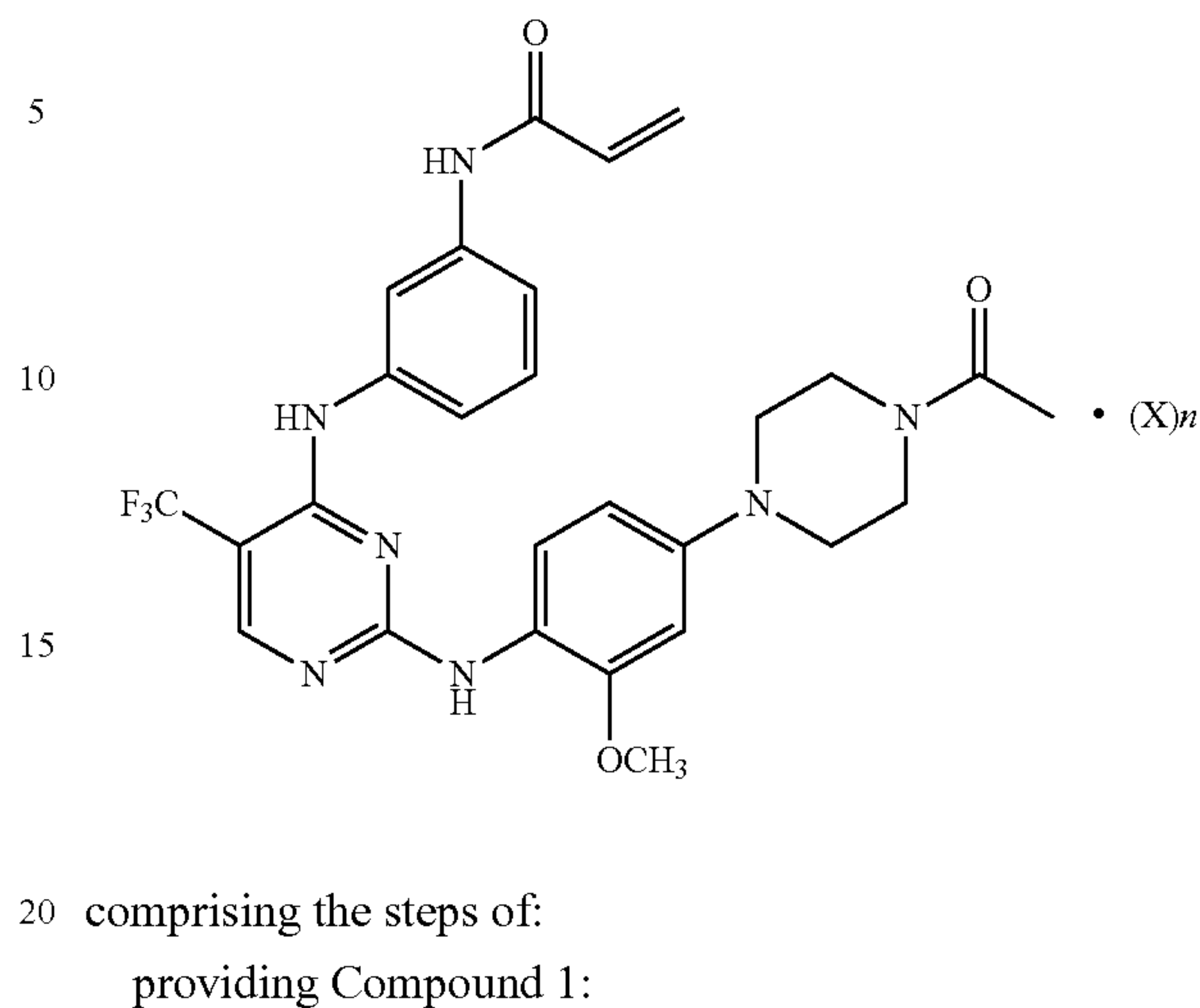
Compound 2
