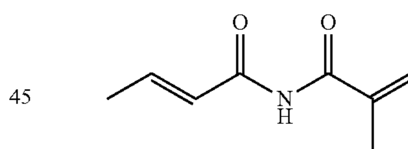
(E)-N-methacryloylbut-2-enamide
