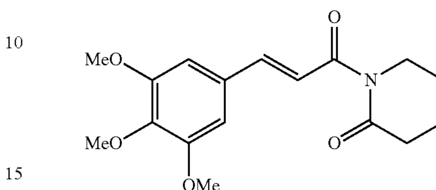
1-[(2E)-3-(3,4,5-trimethoxyphenyl)prop-2-enoyl]-3,6-dihydropyridin-2(1H)-one
