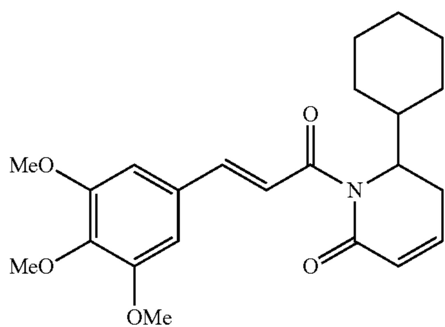
(E)-6-cyclohexyl-1-(3-(3,4,5-trimethoxyphenyl)prop-2-enoyl)-5,6-dihydropyridin-2(1H)-one
