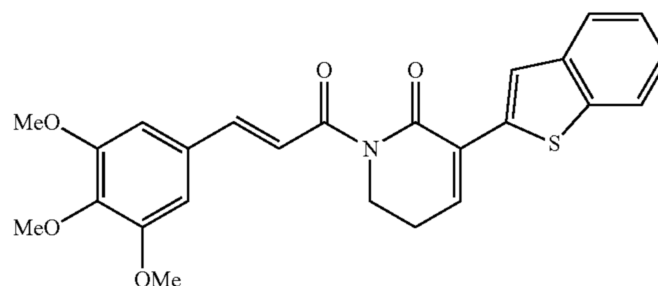
(E)-3-(benzo[b]thiophen-2-yl)-1-(3-(3,4,5-trimethoxyphenyl)prop-2-enoyl)-5,6-dihydropyridin-2(1H)-one
