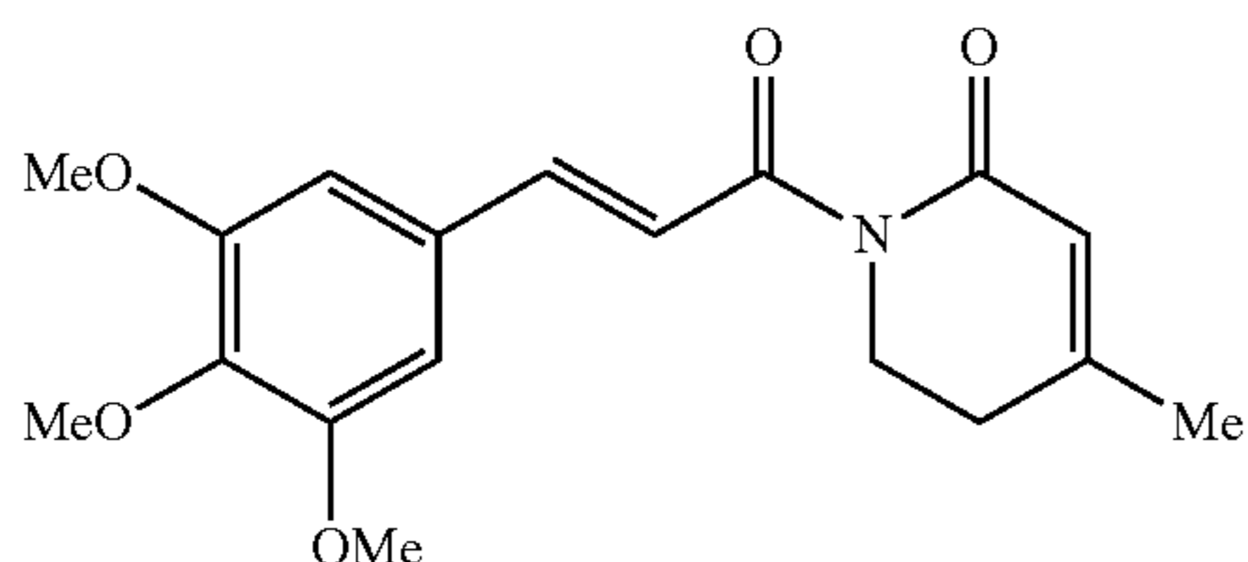
4-methyl-1-[(2E)-3-(3,4,5-trimethoxyphenyl)prop-2-enoyl]-5,6-dihydropyridin-2(1H)-one
