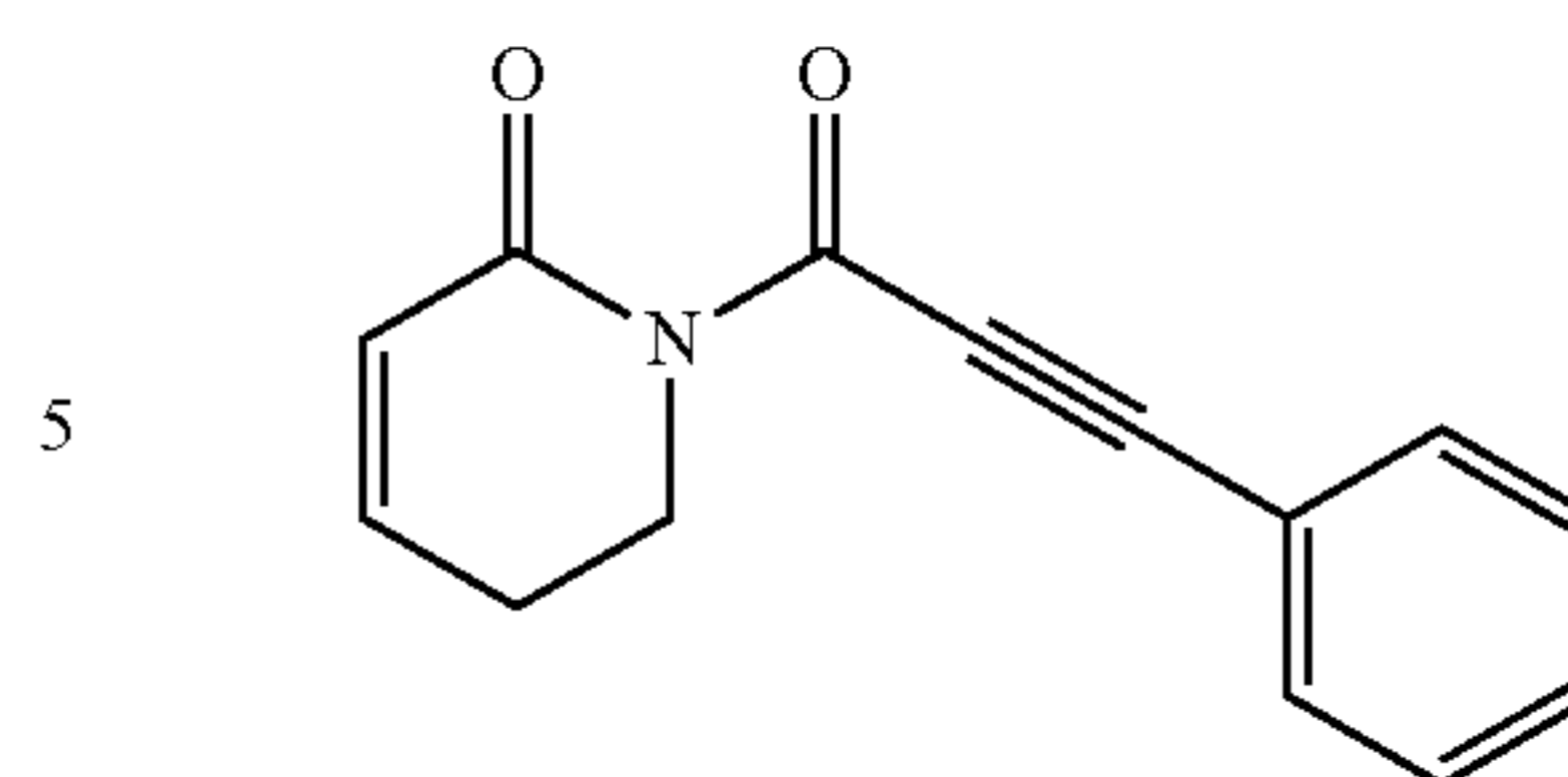
1-(3-Phenylpropioloyl)-5,6-dihydropyridin-2(1H)-one
