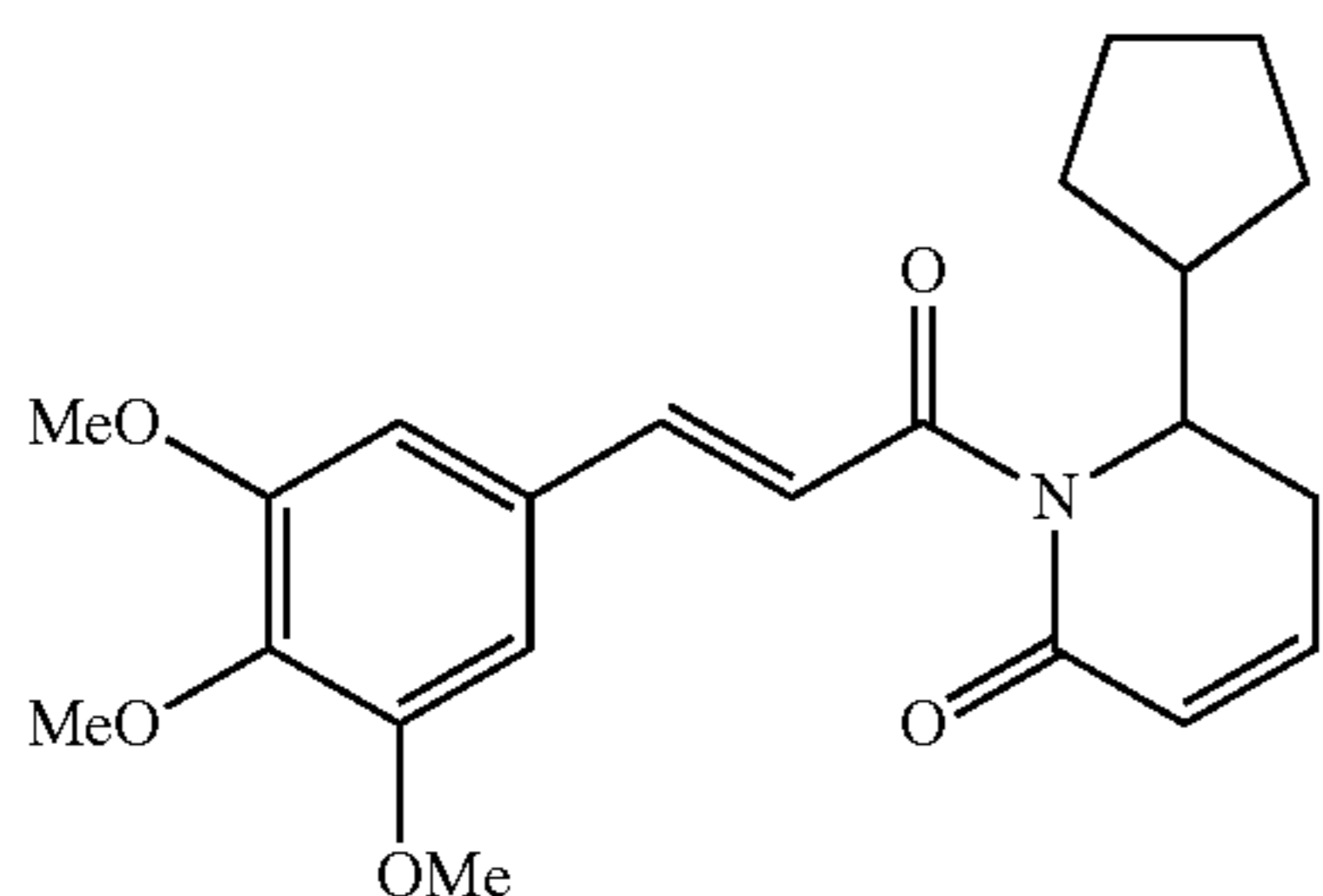
(E)-6-cyclopentyl-1-(3-(3,4,5-trimethoxyphenyl)prop-2-enoyl)-5,6-dihydropyridin-2(1H)-one
