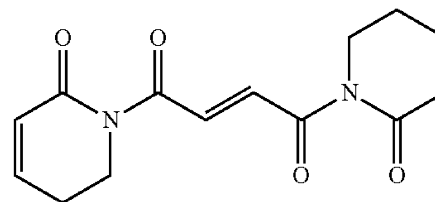
(E)-1,4-bis(2-oxo-5,6-dihydropyridin-1(2H)-yl)but-2-ene-1,4-dione
