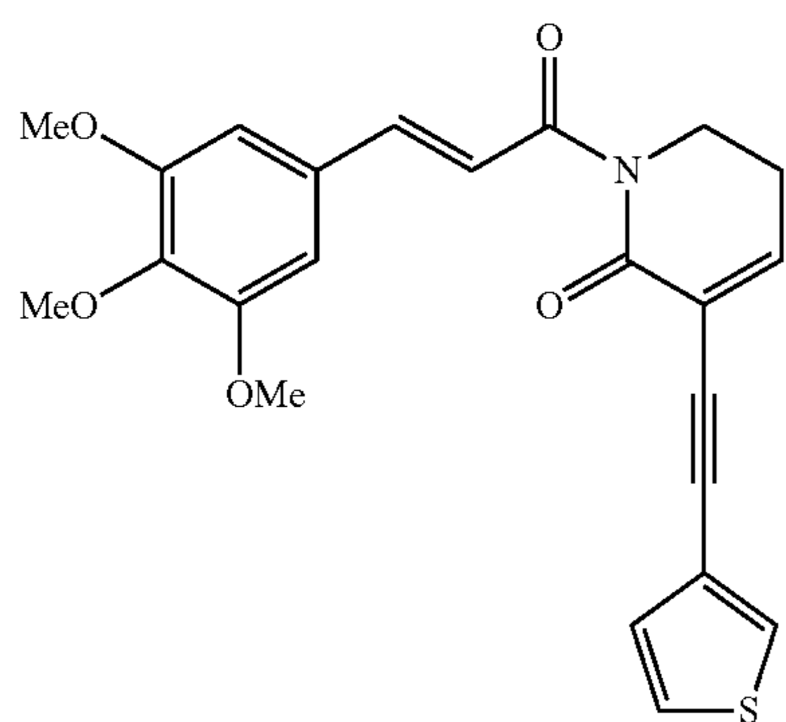
(E)-3-(thiophen-3-ylethynyl)-1-(3-(3,4,5-trimethoxyphenyl)prop-2-enoyl)-5,6-dihydropyridin-2(1H)-one
