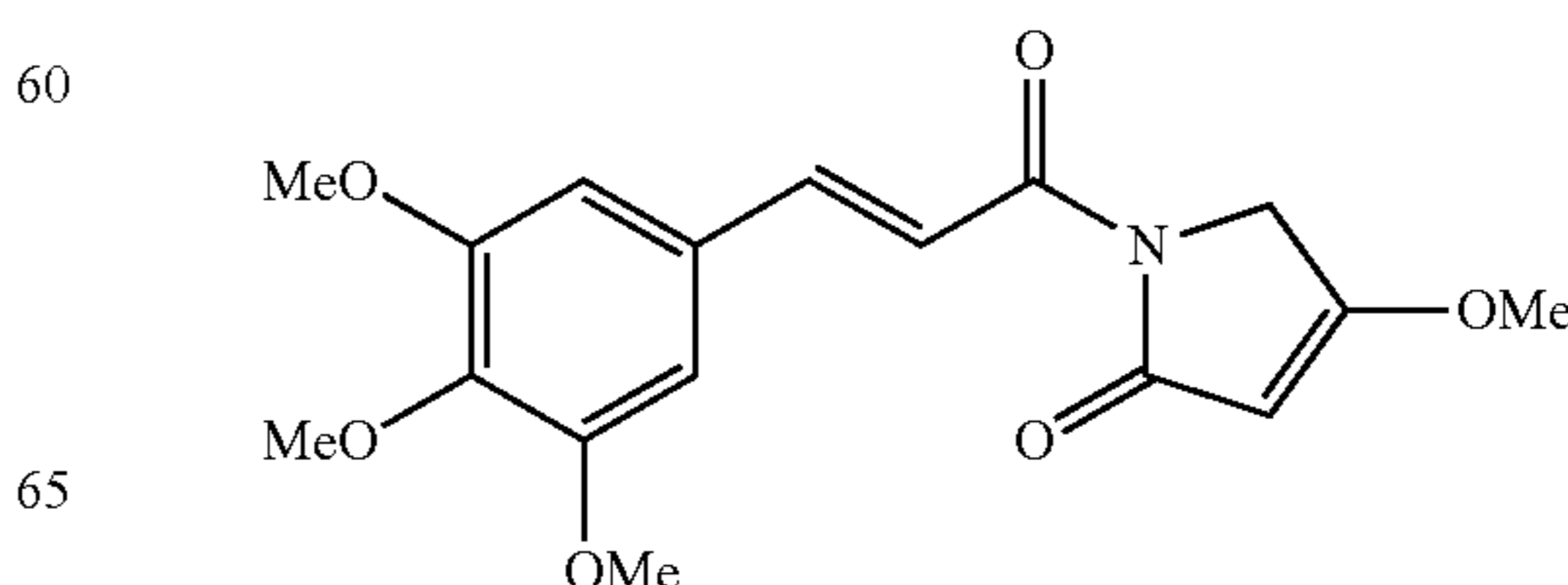
4-methyl-1-[(2E)-3-(3,4,5-trimethoxyphenyl)prop-2-enoyl]-5,6-dihydropyridin-2(1H)-one
