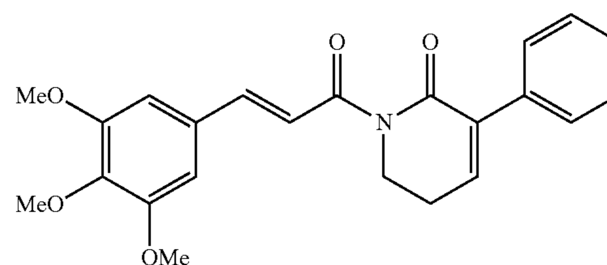
(E)-3-phenyl-1-(3-(3,4,5-trimethoxyphenyl)prop-2-enyl)-5,6-dihydropyridin-2(1H)-one
