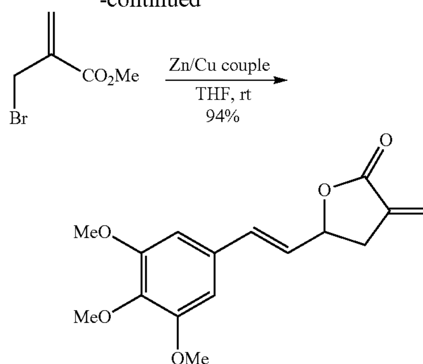
3-methylene-5-[(E)-2-(3,4,5-trimethoxyphenyl)vinyl]dihydrofuran-2(3H)-one
