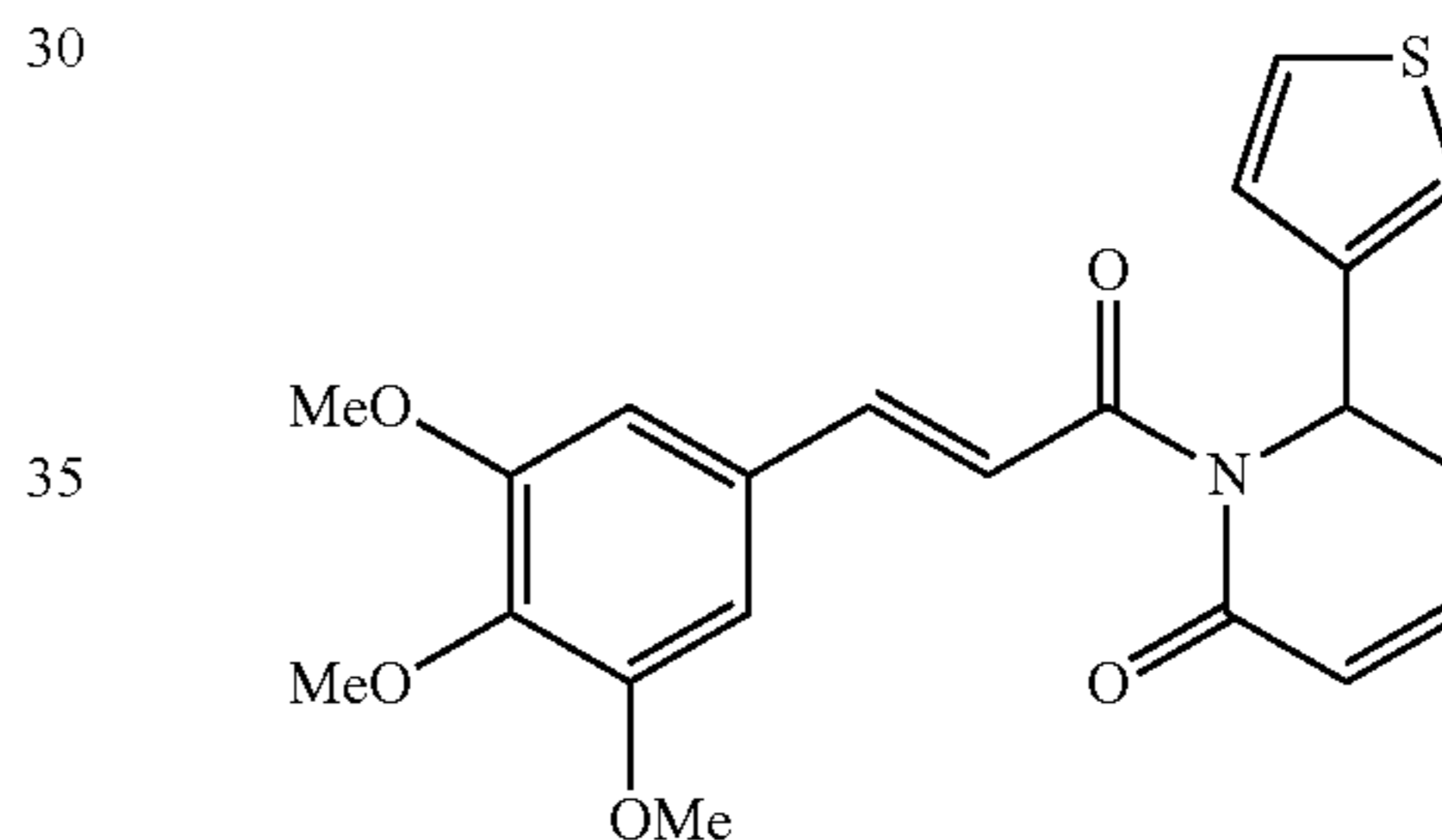
(E)-6-(thiophen-3-yl)-1-(3-(3,4,5-trimethoxyphenyl)prop-2-enoyl)-5,6-dihydropyridin-2(1H)-one
