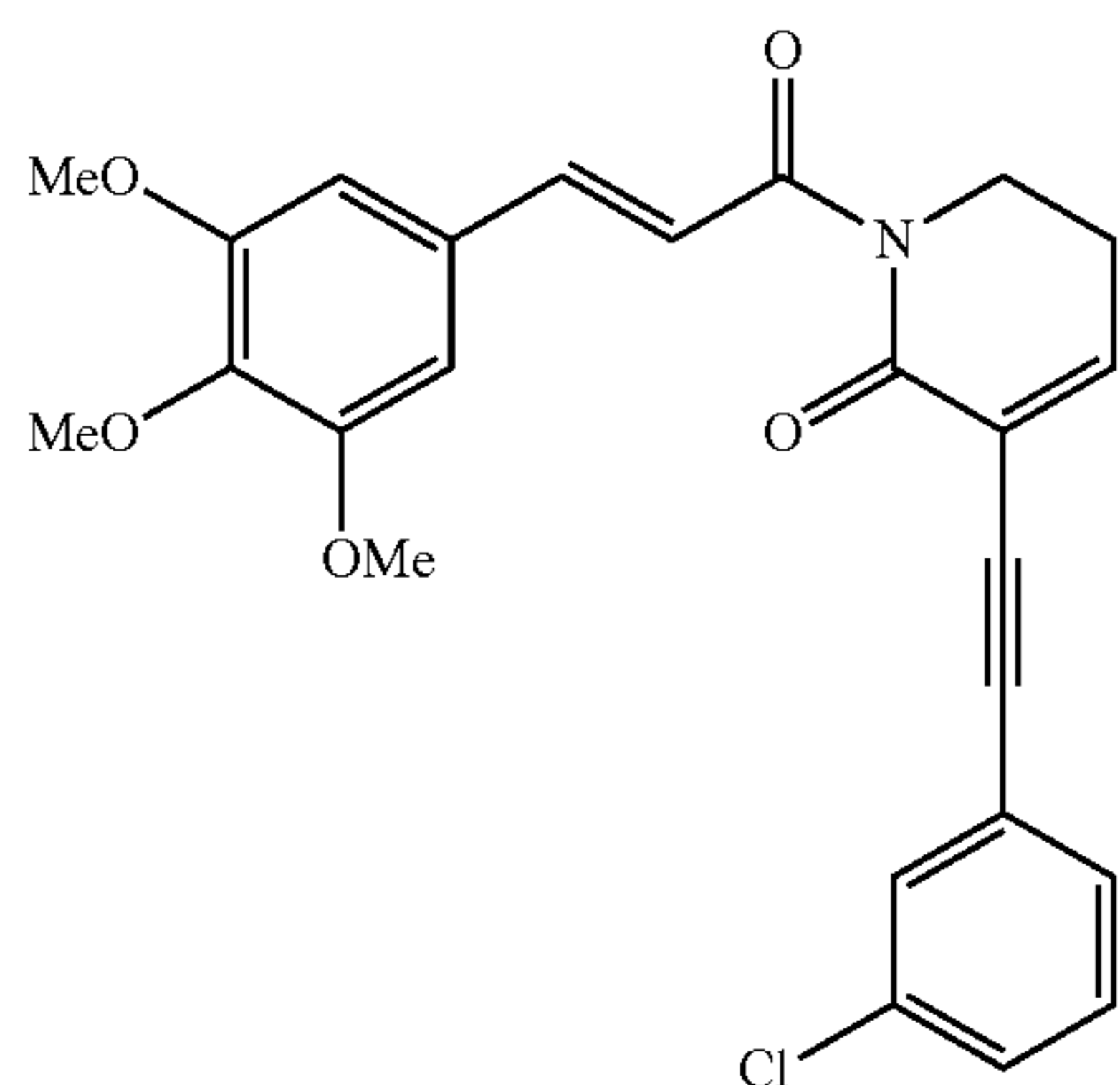
(E)-3-((3-chlorophenyl)ethynyl)-1-(3-(3,4,5-trimethoxyphenyl)prop-2-enoyl)-5,6-dihydropyridin-2(1H)-one
