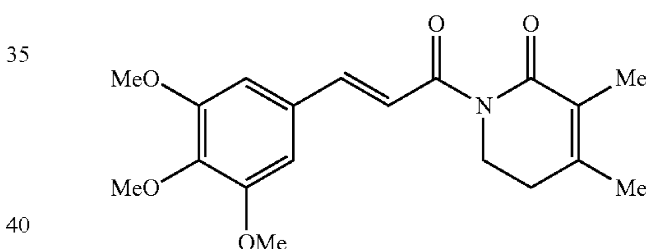
3,4-dimethyl-1-[(2E)-3-(3,4,5-trimethoxyphenyl)prop-2-enoyl]-5,6-dihydropyridin-2(1H)-one
