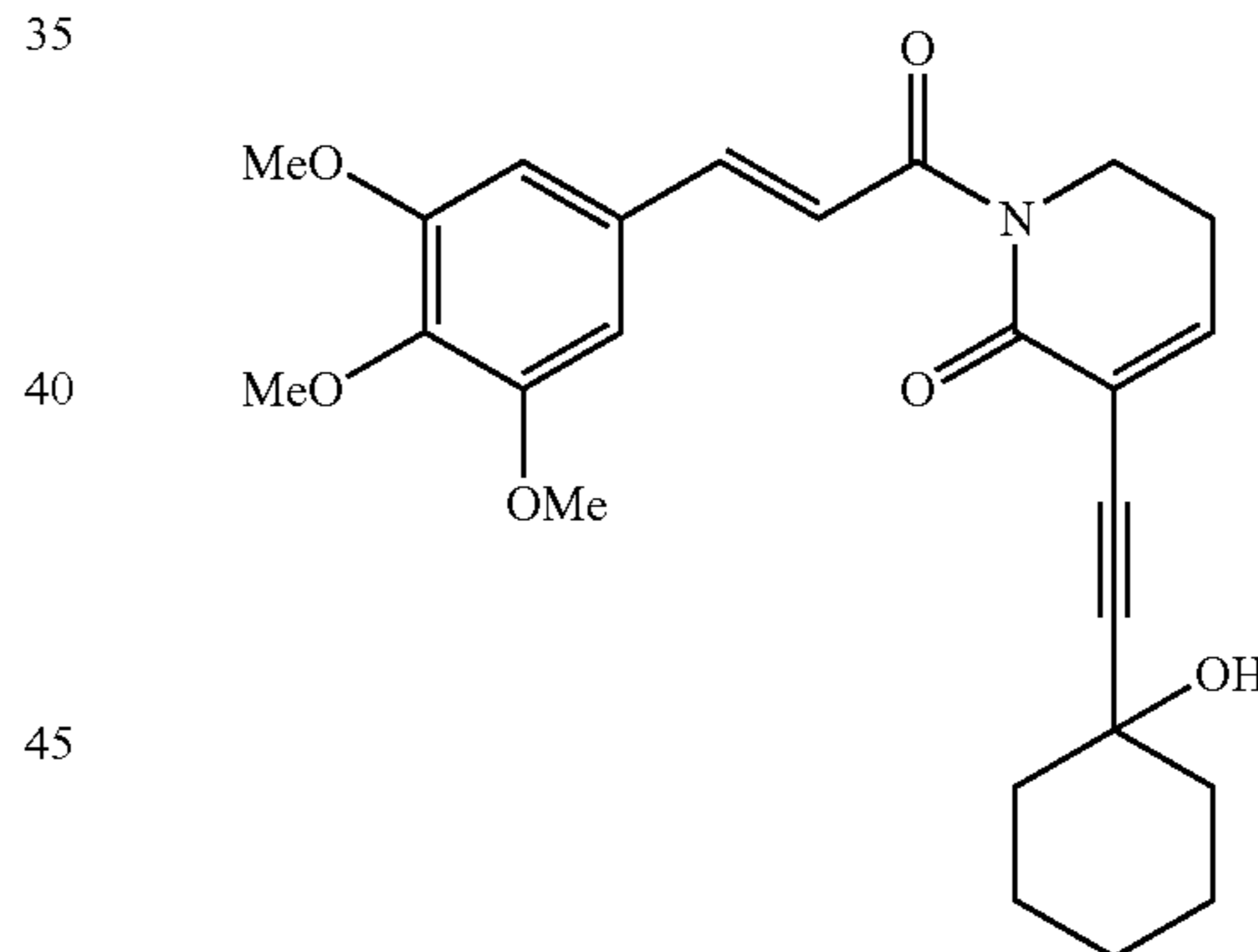
(E)-3-((1-hydroxycyclohexyl)ethynyl)-1-(3-(3,4,5-trimethoxyphenyl)prop-2-enoyl)-5,6-dihydropyridin-2(1H)-one
