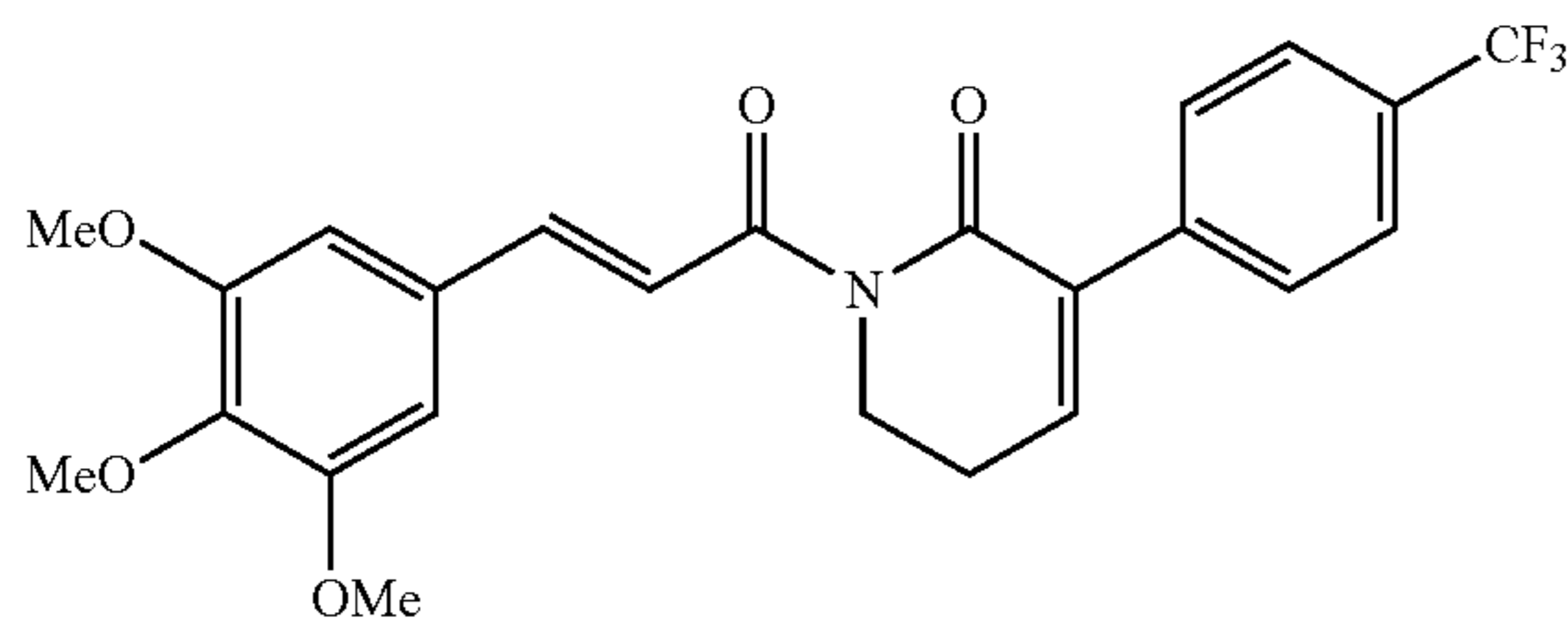
(E)-3-(4-(trifluoromethyl)phenyl)-1-(3-(3,4,5-trimethoxyphenyl)prop-2-enoyl)-5,6-dihydropyridin-2(1H)-one
