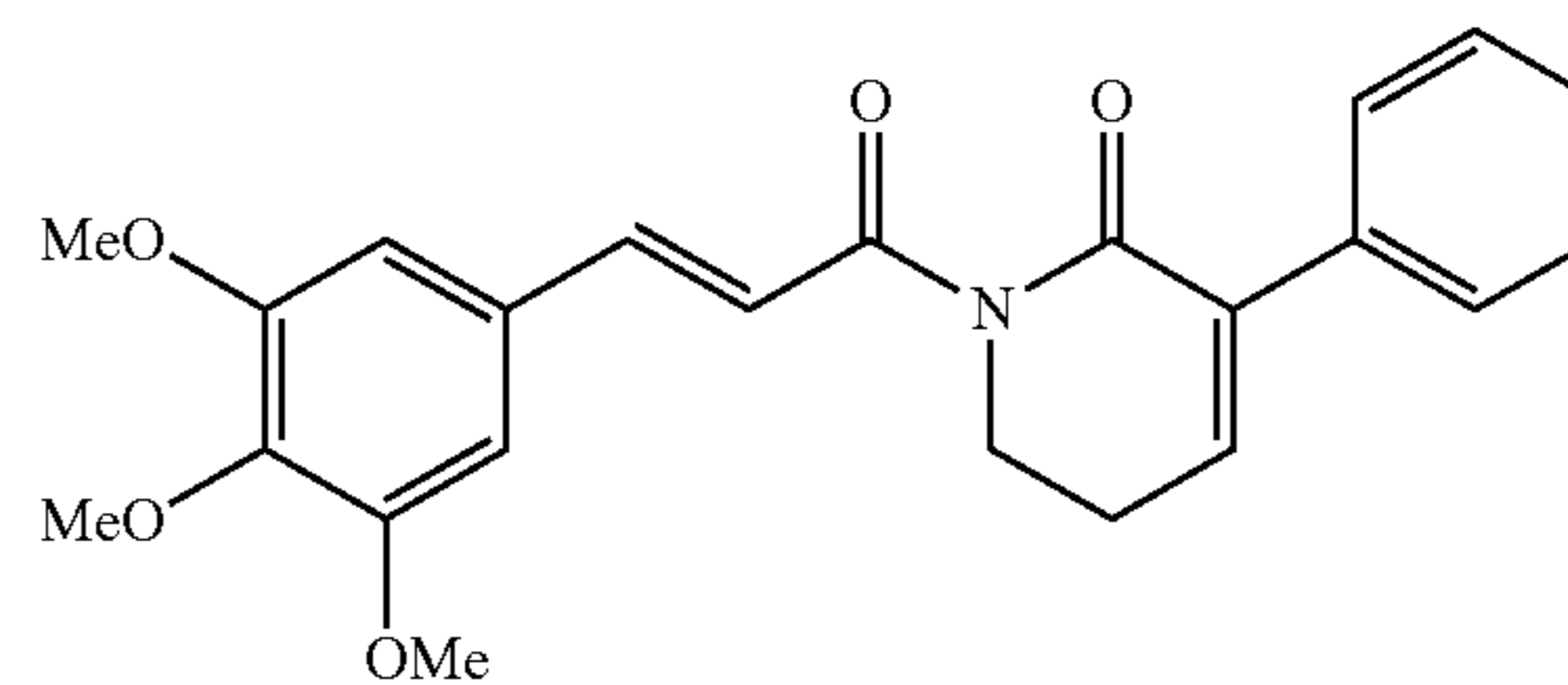
(E)-3-phenyl-1-(3-(3,4,5-trimethoxyphenyl)prop-2-enoyl)-5,6-dihydropyridin-2(1H)-one
