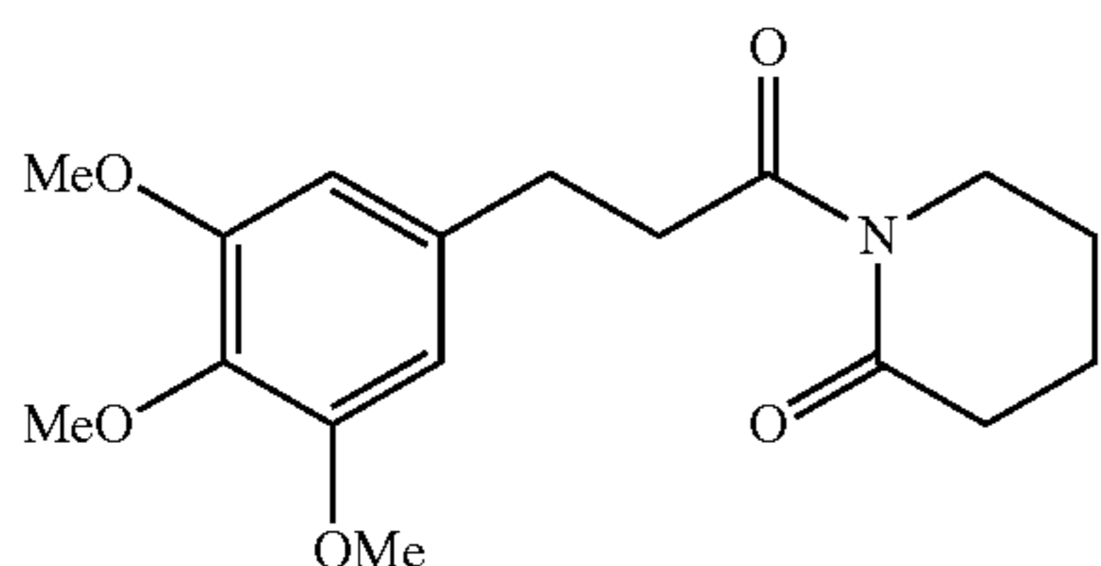
1-(3-(3,4,5-trimethoxyphenyl)propanoyl)piperidin-2-one
