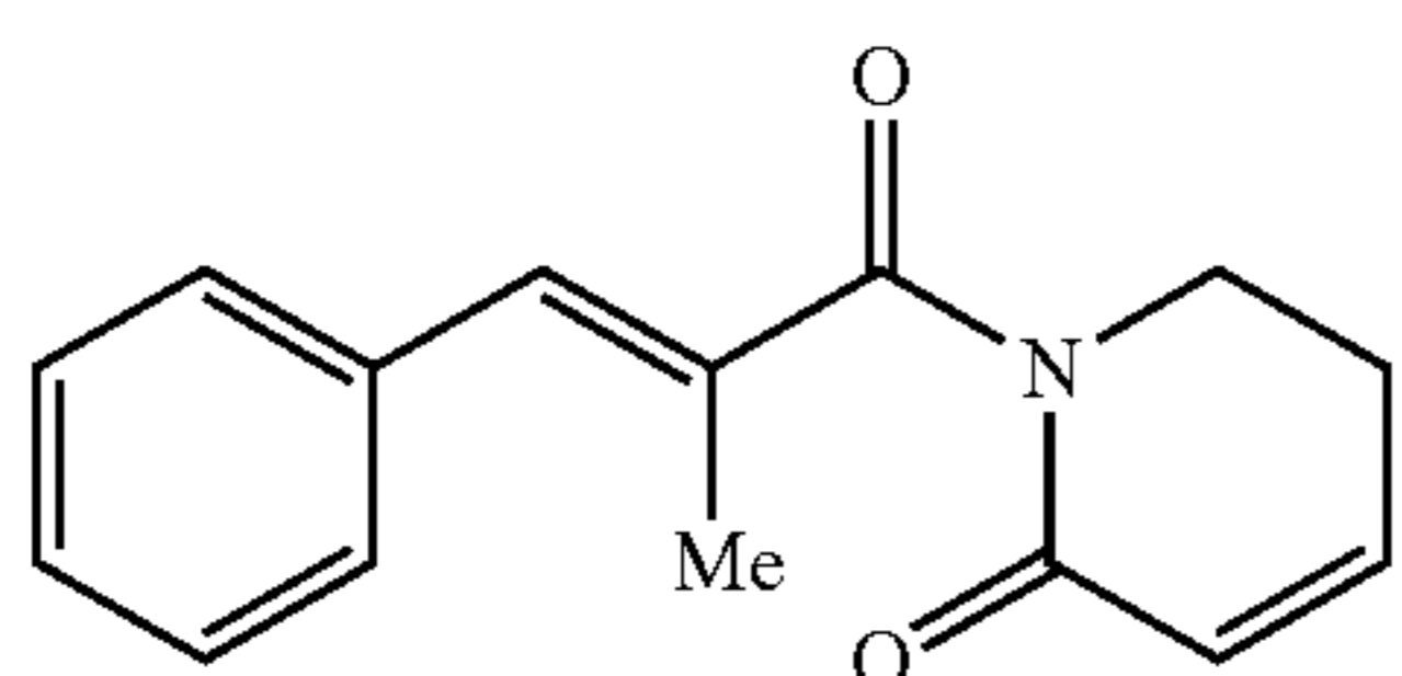
(E)-1-(2-methyl-3-phenylprop-2-enoyl)-5,6-dihydropyridin-2(1H)-one
