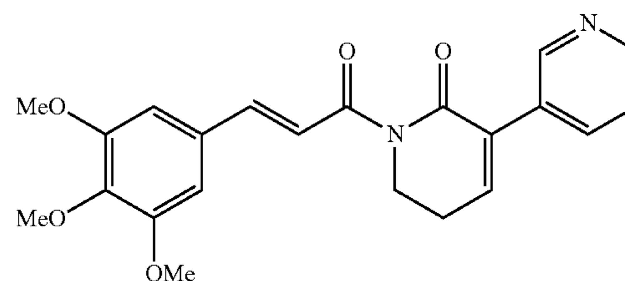
(E)-3-(pyridin-3-yl)-1-(3-(3,4,5-trimethoxyphenyl)prop-2-enoyl)-5,6-dihydropyridin-2(1H)-one
