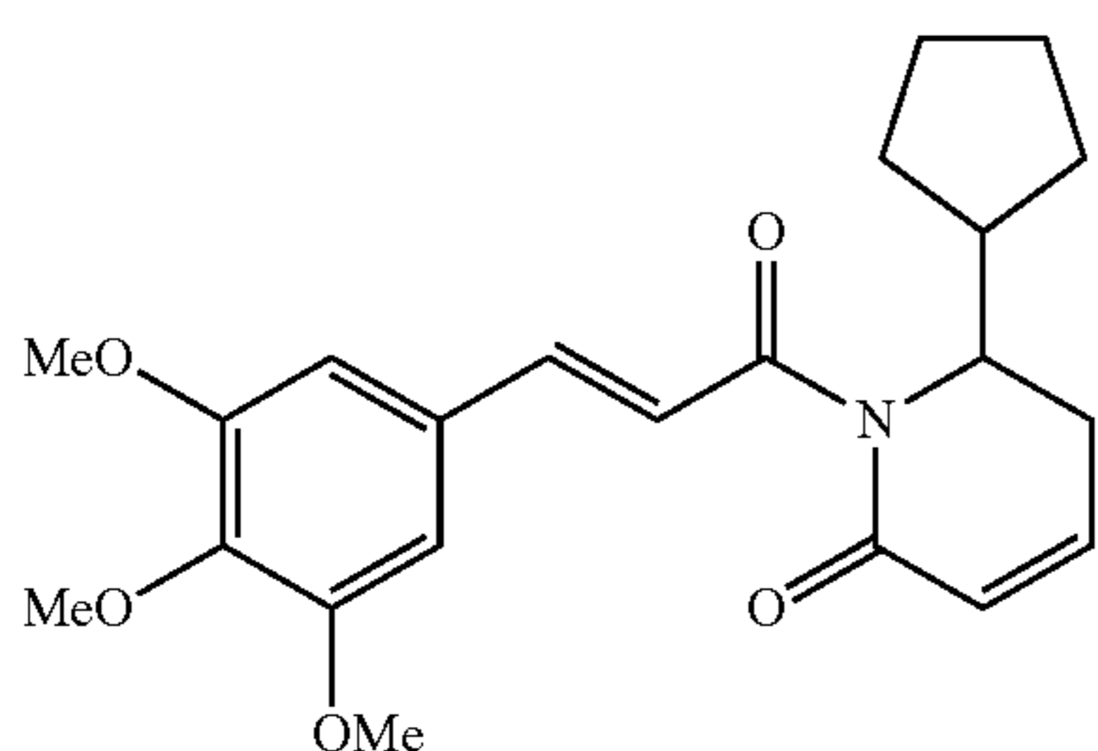
(E)-6-cyclopentyl-1-(3-(3,4,5-trimethoxyphenyl)prop-2-enoyl)-5,6-dihydropyridin-2(1H)-one
