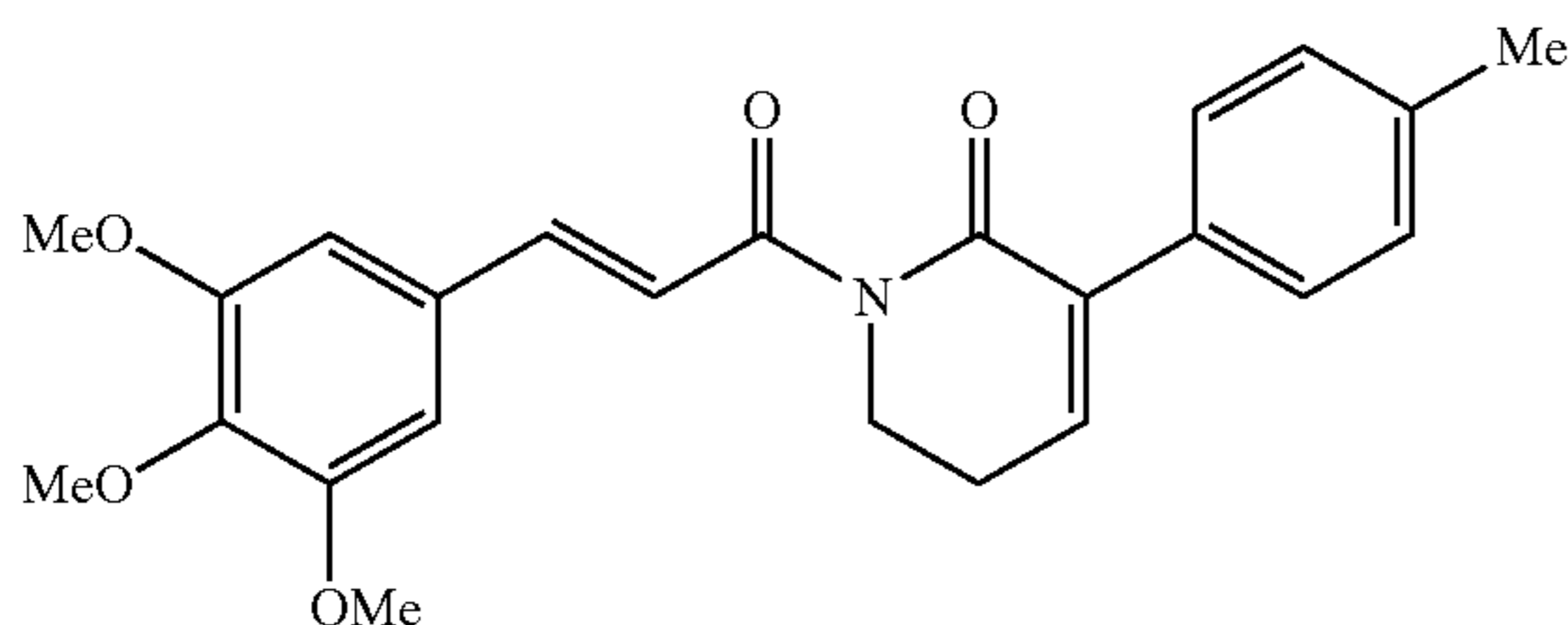
(E)-3-p-tolyl-1-(3-(3,4,5-trimethoxyphenyl)prop-2-enoyl)-5,6-dihydropyridin-2(1H)-one
