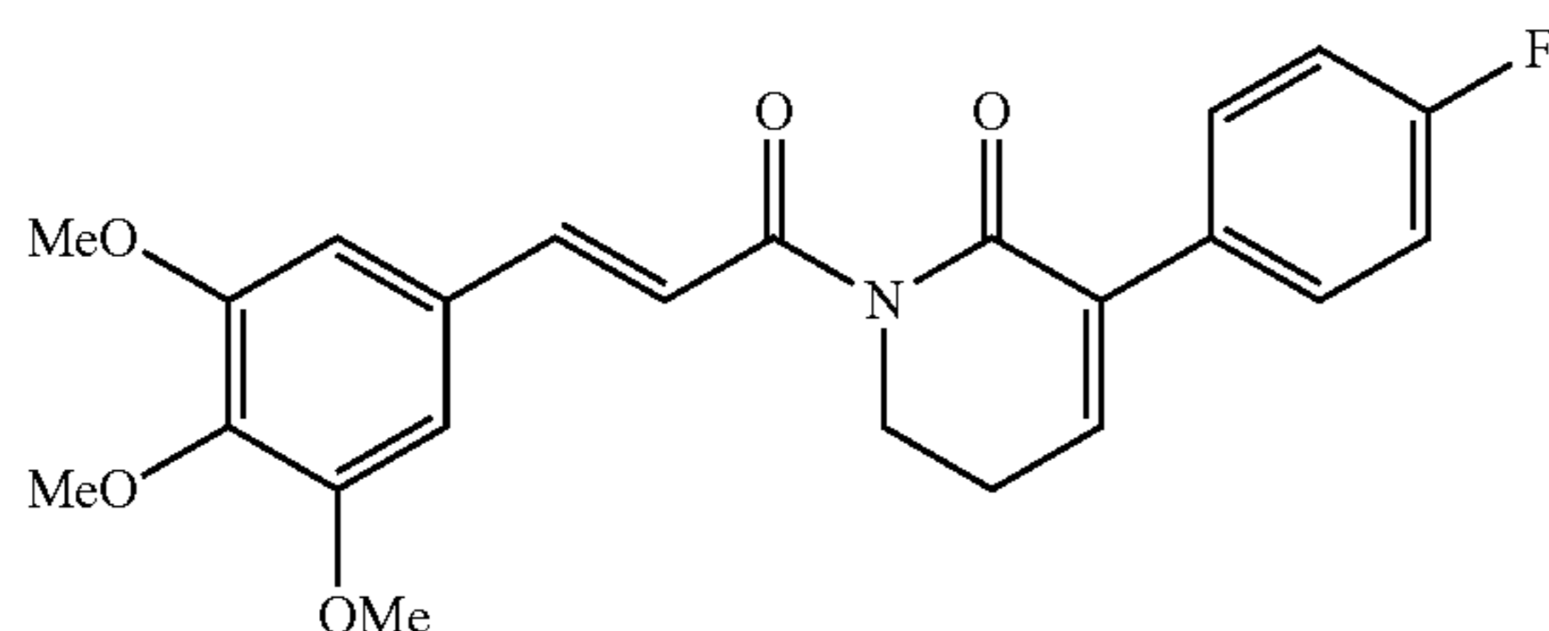
(E)-3-(4-fluorophenyl)-1-(3-(3,4,5-trimethoxyphenyl)prop-2-enoyl)-5,6-dihydropyridin-2(1H)-one
