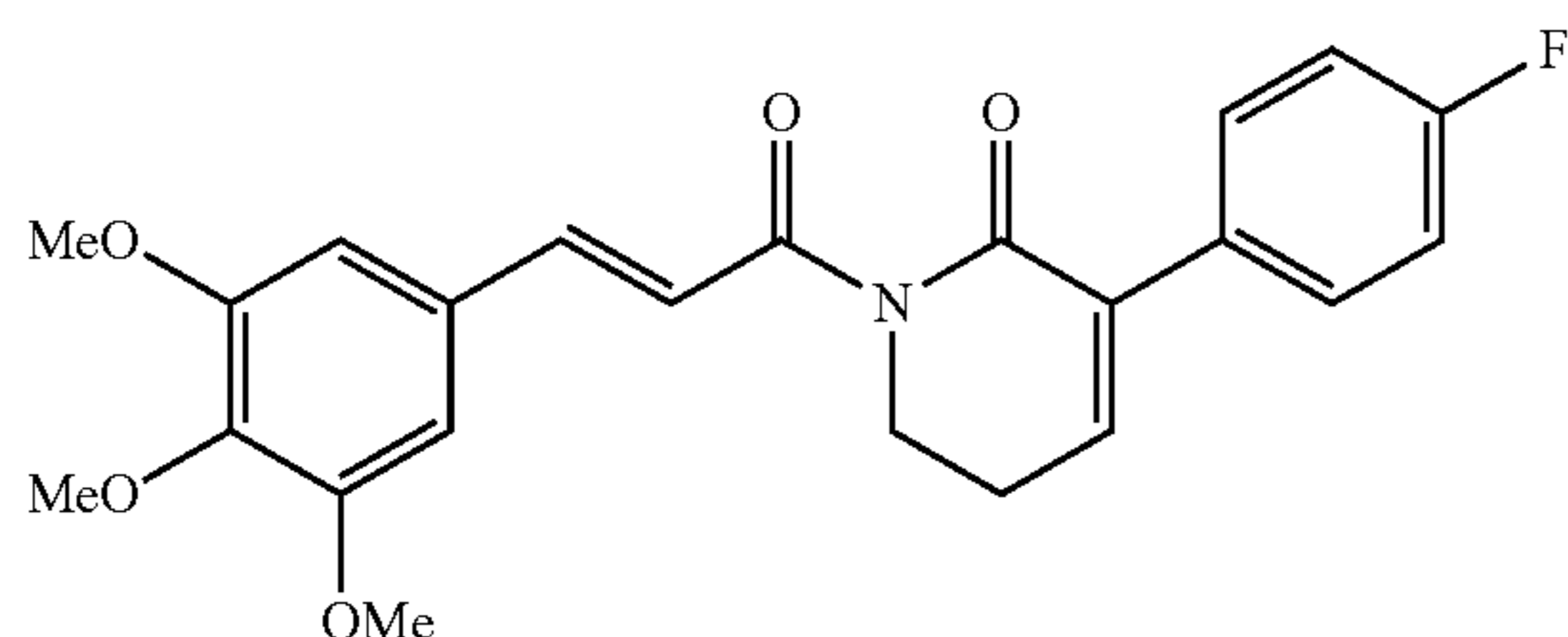
(E)-3-(4-fluorophenyl)-1-(3-(3,4,5-trimethoxyphenyl)prop-2-enoyl)-5,6-dihydropyridin-2(1H)-one
