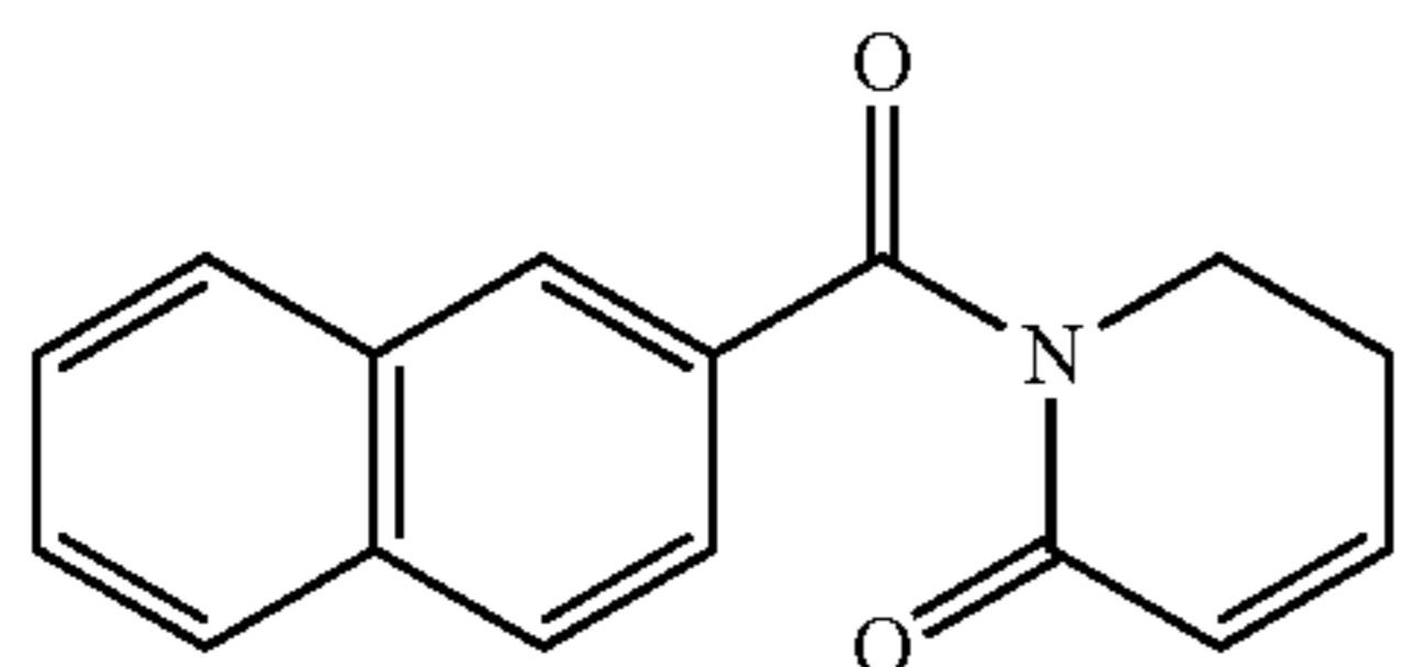
1-(2-naphthoyl)-5,6-dihydropyridin-2(1H)-one
