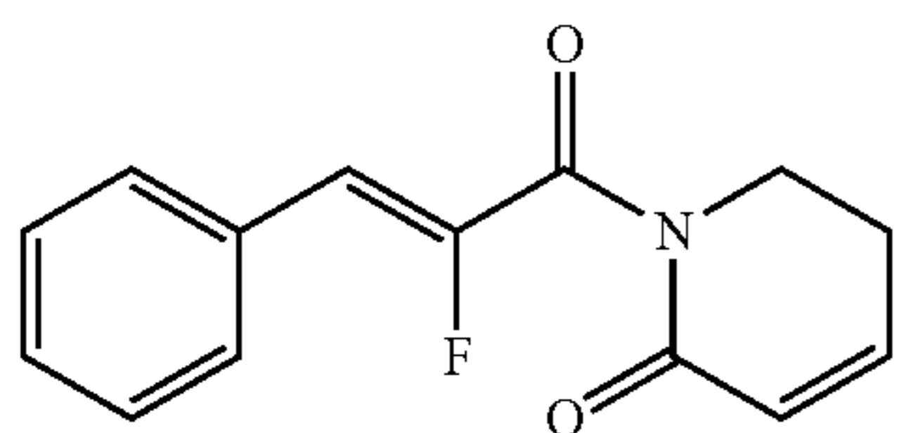
1-[(2Z)-2-fluoro-3-phenylprop-2-enoyl]-5,6-dihydropyridin-2(1H)-one
