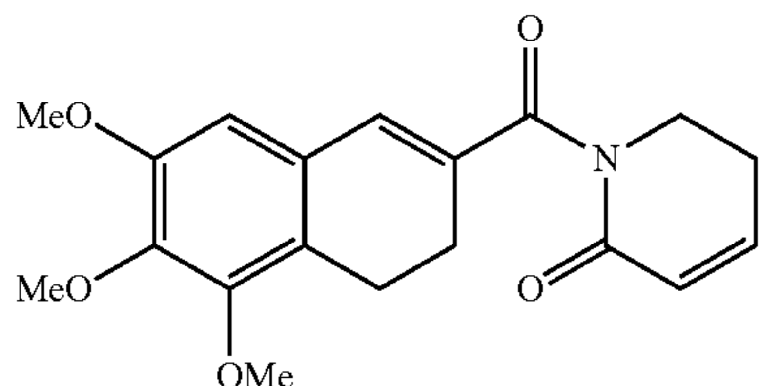
1-(5,6,7-trimethoxy-3,4-dihydronaphthalene-2-carbonyl)-5,6-dihydropyridin-2(1H)-one
