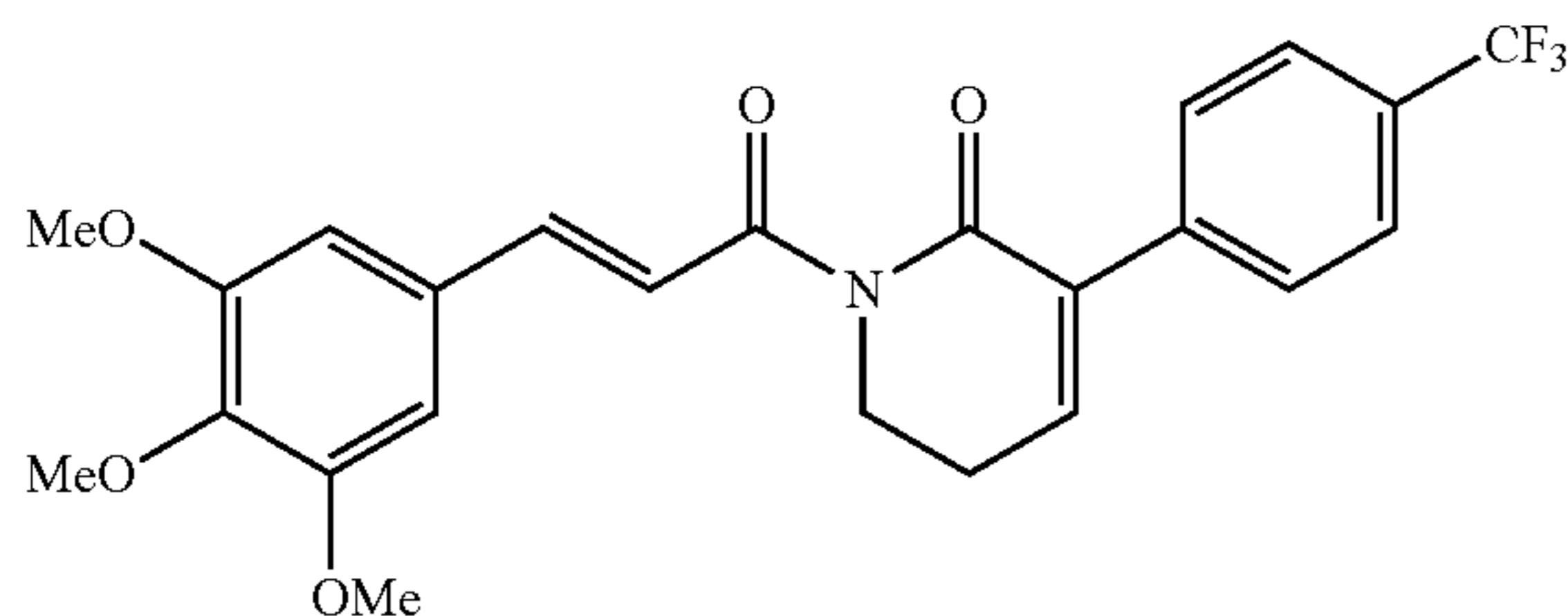
(E)-3-(4-(trifluoromethyl)phenyl)-1-(3-(3,4,5-trimethoxyphenyl)prop-2-enoyl)-5,6-dihydropyridin-2(1H)-one
