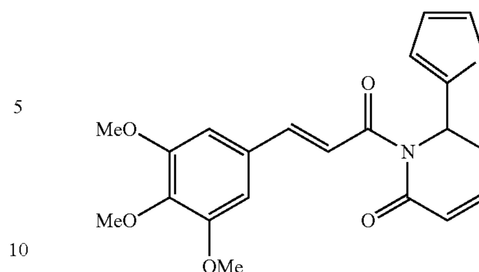
(E)-6-(thiophen-2-yl)-1-(3-(3,4,5-trimethoxyphenyl)prop-2-enoyl)-5,6-dihydropyridin-2(1H)-one
