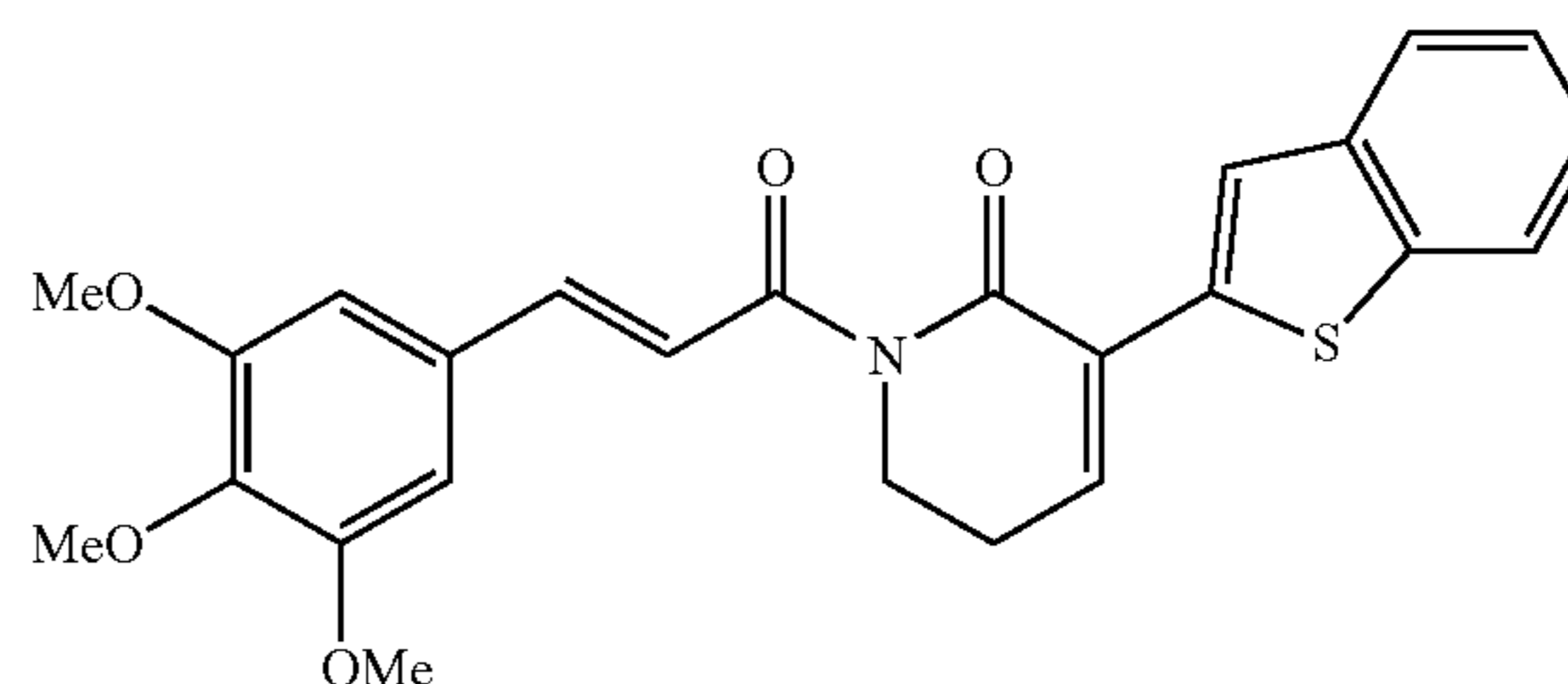
(E)-3-(benzo[b]thiophen-2-yl)-1-(3-(3,4,5-trimethoxyphenyl)prop-2-enoyl)-5,6-dihydropyridin-2(1H)-one
