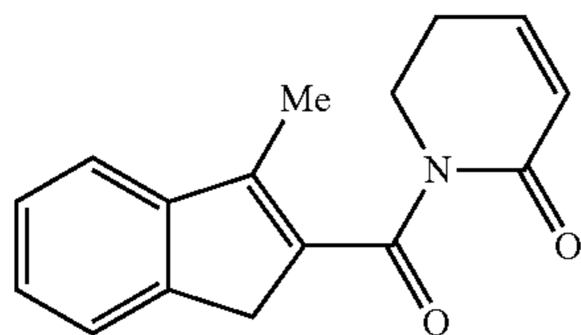
1-(3-methyl-1H-indene-2-carbonyl)-5,6-dihydropyridin-2(1H)-one
