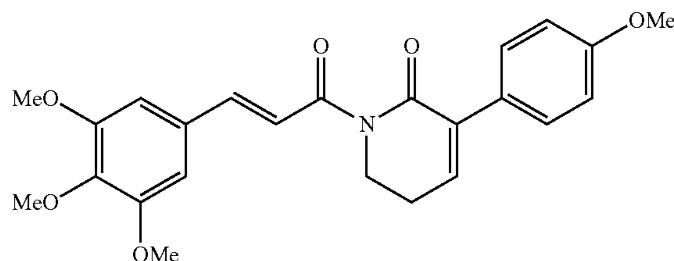
(E)-3-(4-methoxyphenyl)-1-(3-(3,4,5-trimethoxyphenyl)prop-2-enoyl)-5,6-dihydropyridin-2(1H)-one
