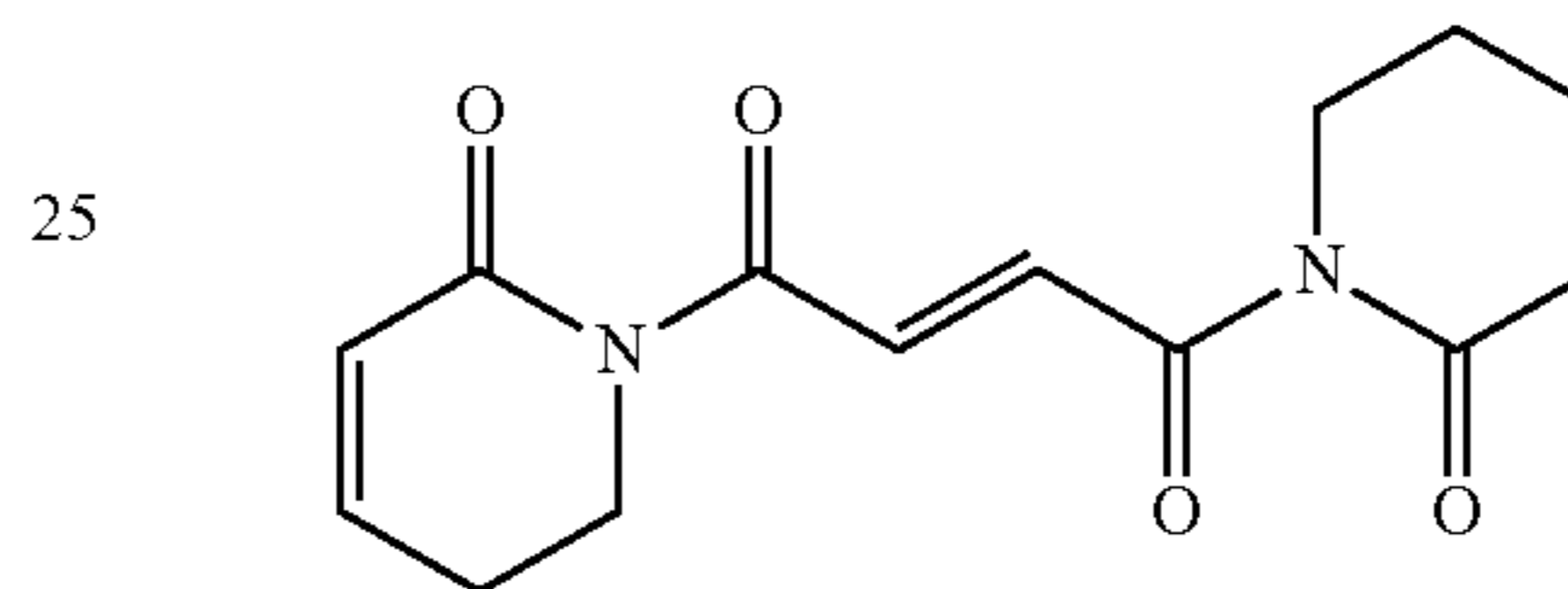
(E)-1,4-bis(2-oxo-5,6-dihydropyridin-1(2H)-yl)but-2-ene-1,4-dione
