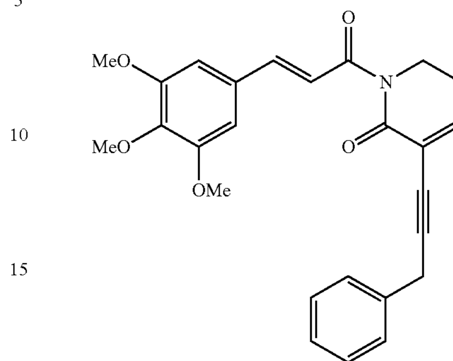
(E)-3-(3-phenylprop-1-ynyl)-1-(3-(3,4,5-trimethoxyphenyl)prop-2-enoyl)-5,6-dihydropyridin-2(1H)-one
