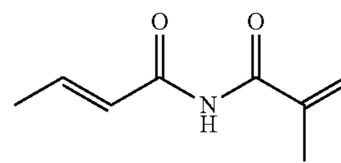
(E)-N-methacryloylbut-2-enamide
