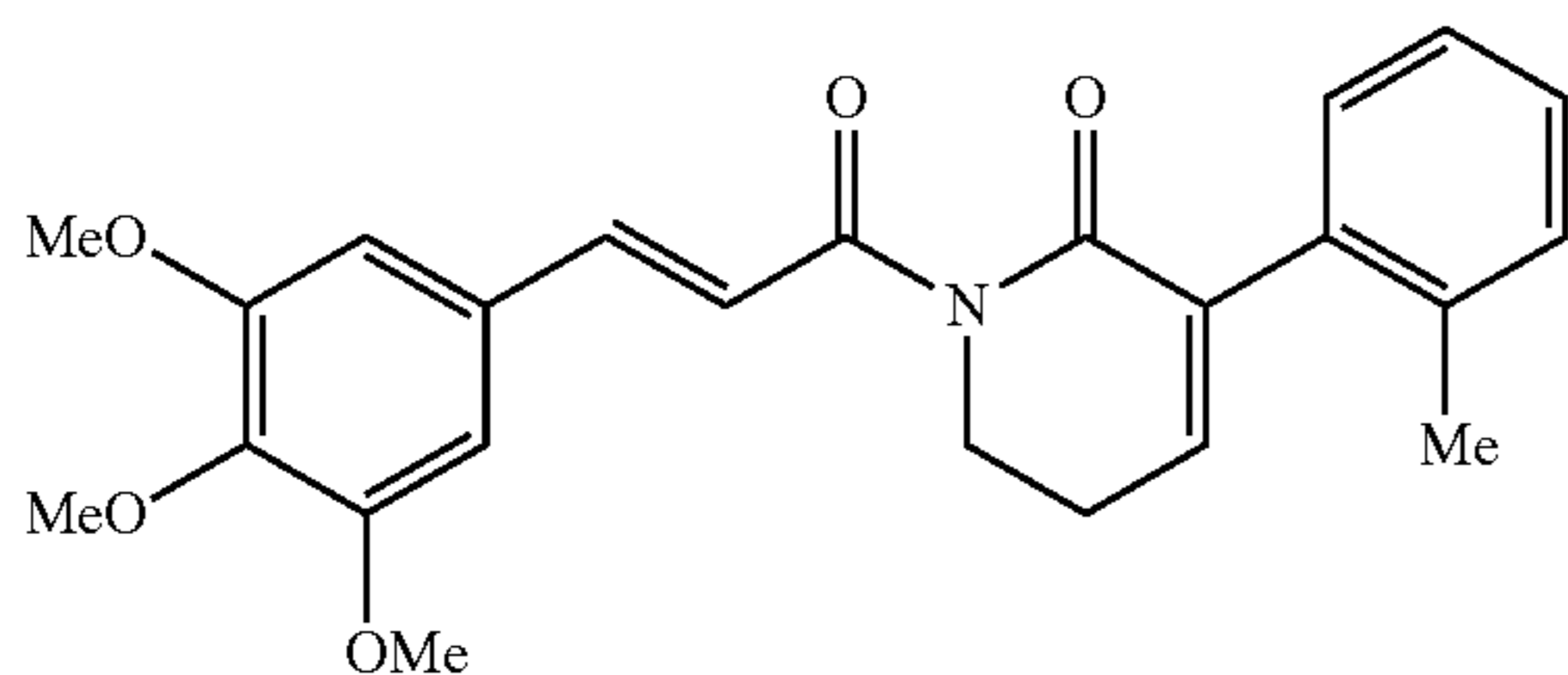
(E)-3-o-tolyl-1-(3-(3,4,5-trimethoxyphenyl)prop-2-enoyl)-5,6-dihydropyridin-2(1H)-one
