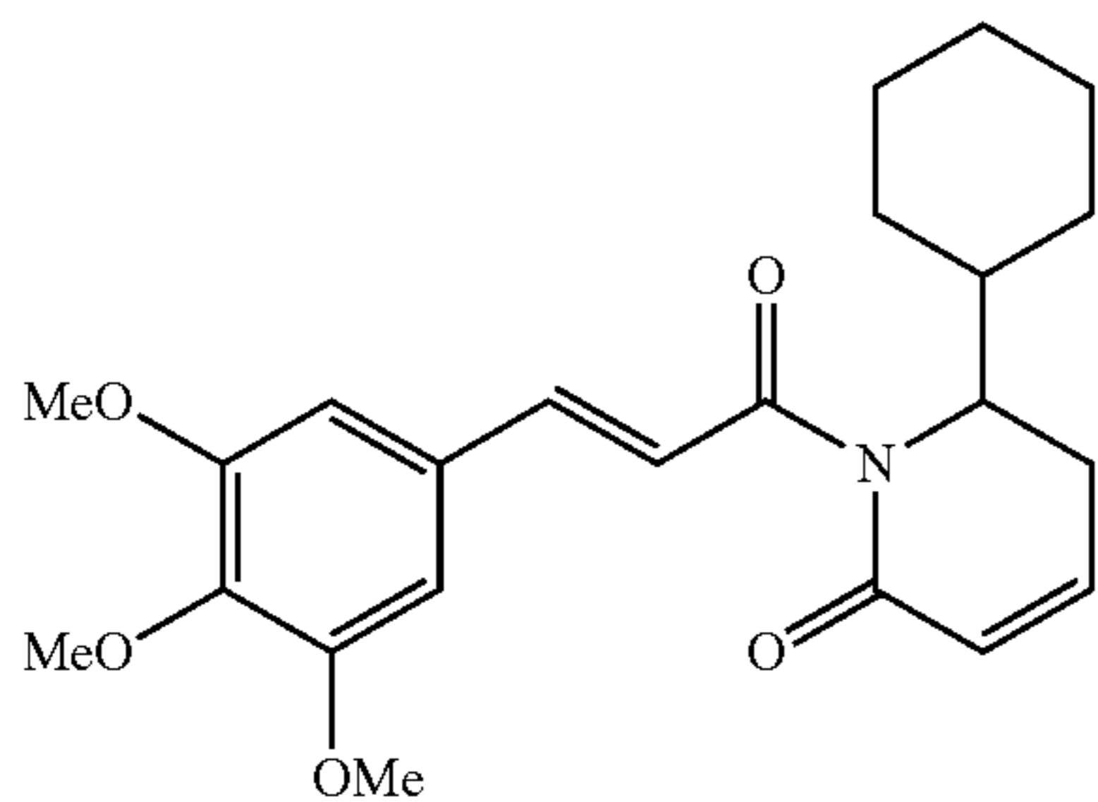
(E)-6-cyclohexyl-1-(3-(3,4,5-trimethoxyphenyl)prop-2-enoyl)-5,6-dihydropyridin-2(1H)-one
