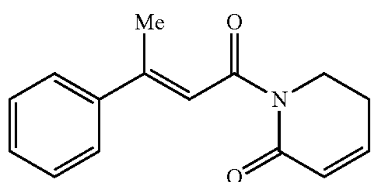
(E)-1-(3-phenylbut-2-enoyl)-5,6-dihydropyridin-2(1H)-one
