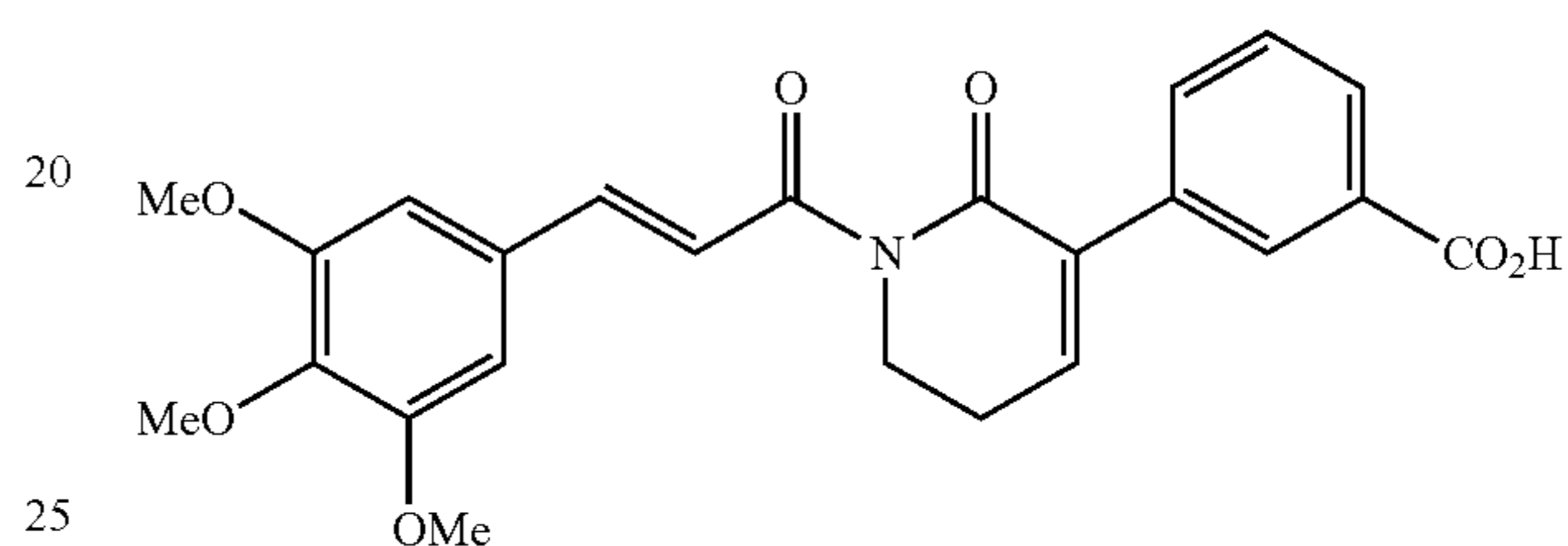
(E)-3-(2-oxo-1-(3-(3,4,5-trimethoxyphenyl)prop-2-enoyl)-1,2,5,6-tetrahydropyridin-3-yl)benzoic acid
