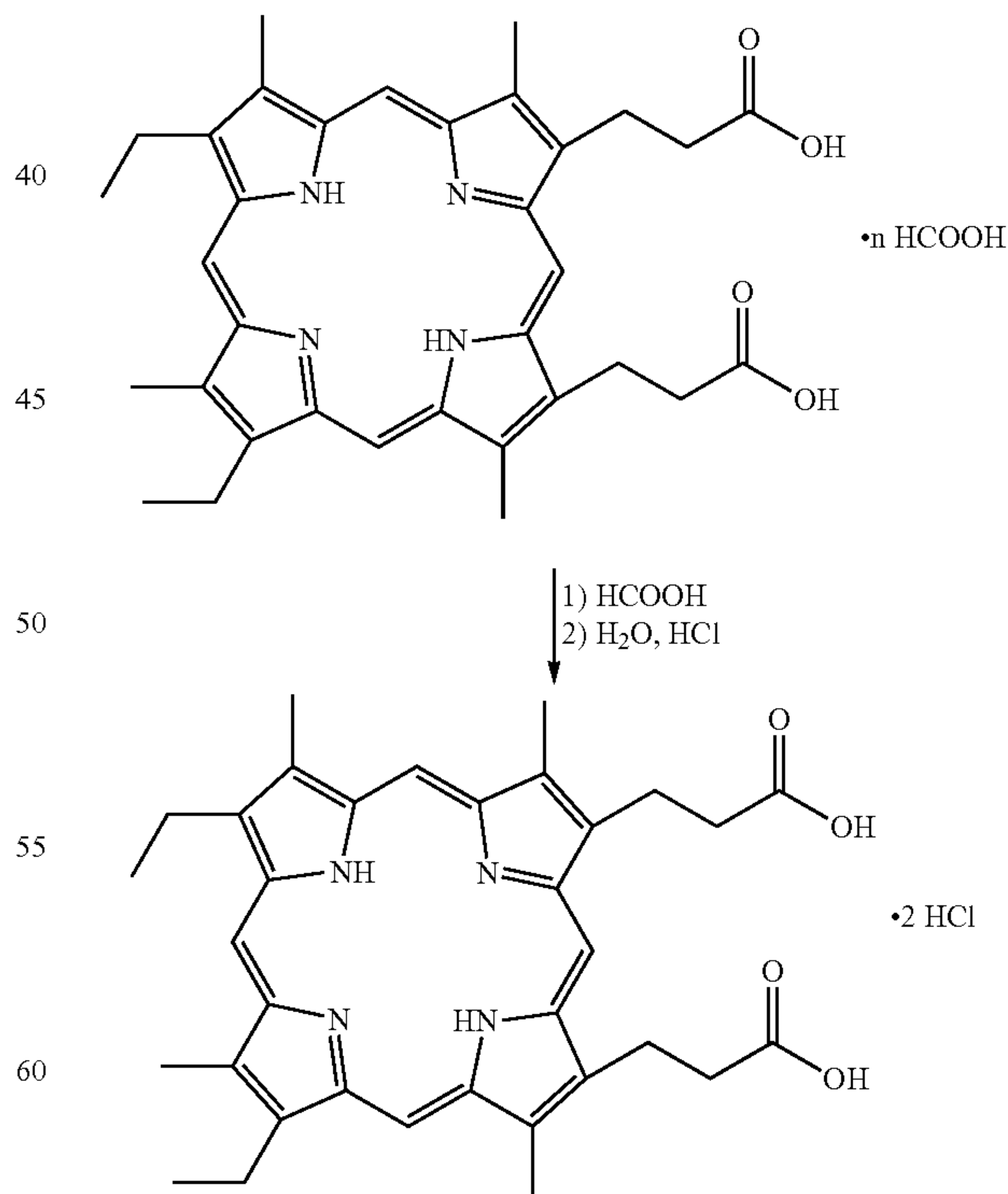
65 Conversion of Mesoporphyrin IX Hydrochloride to Stannoporphyrin (Tin (IV) Mesoporphyrin IX) Via Treatment with Tin (II) Salt
