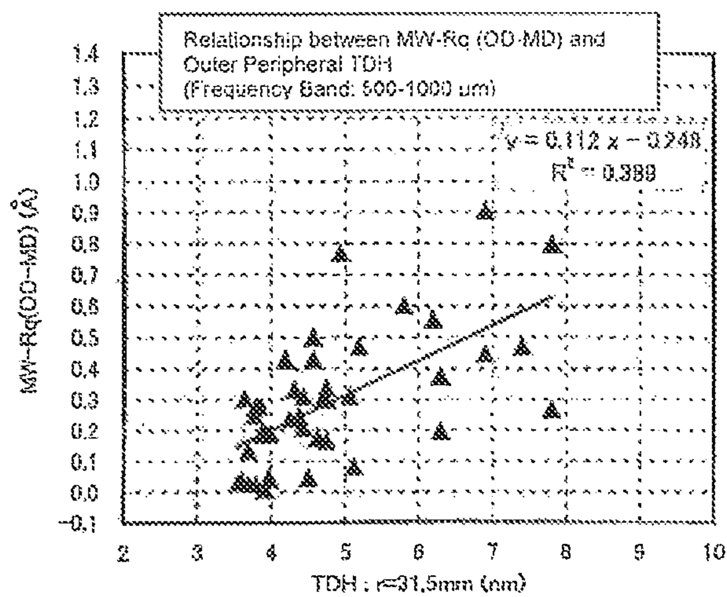
Relationship between MW-Rq (OD-MD) and Outer Peripheral TDH (Frequency Band: 500-1000 μm)
