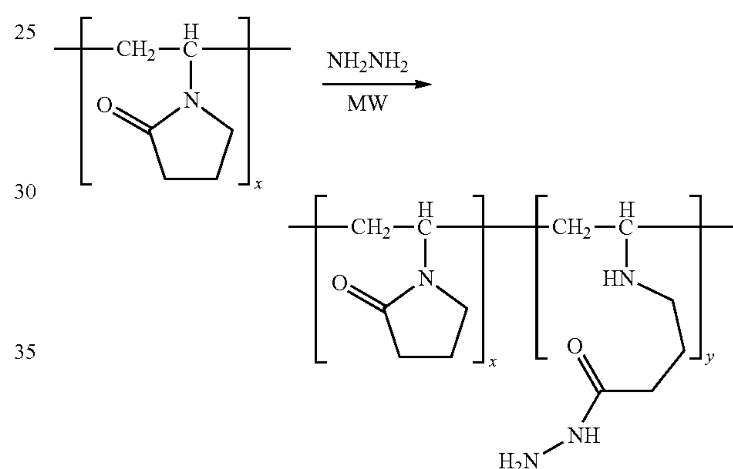
Scheme 2 Polyvinylpyrrolidone Synthesis
