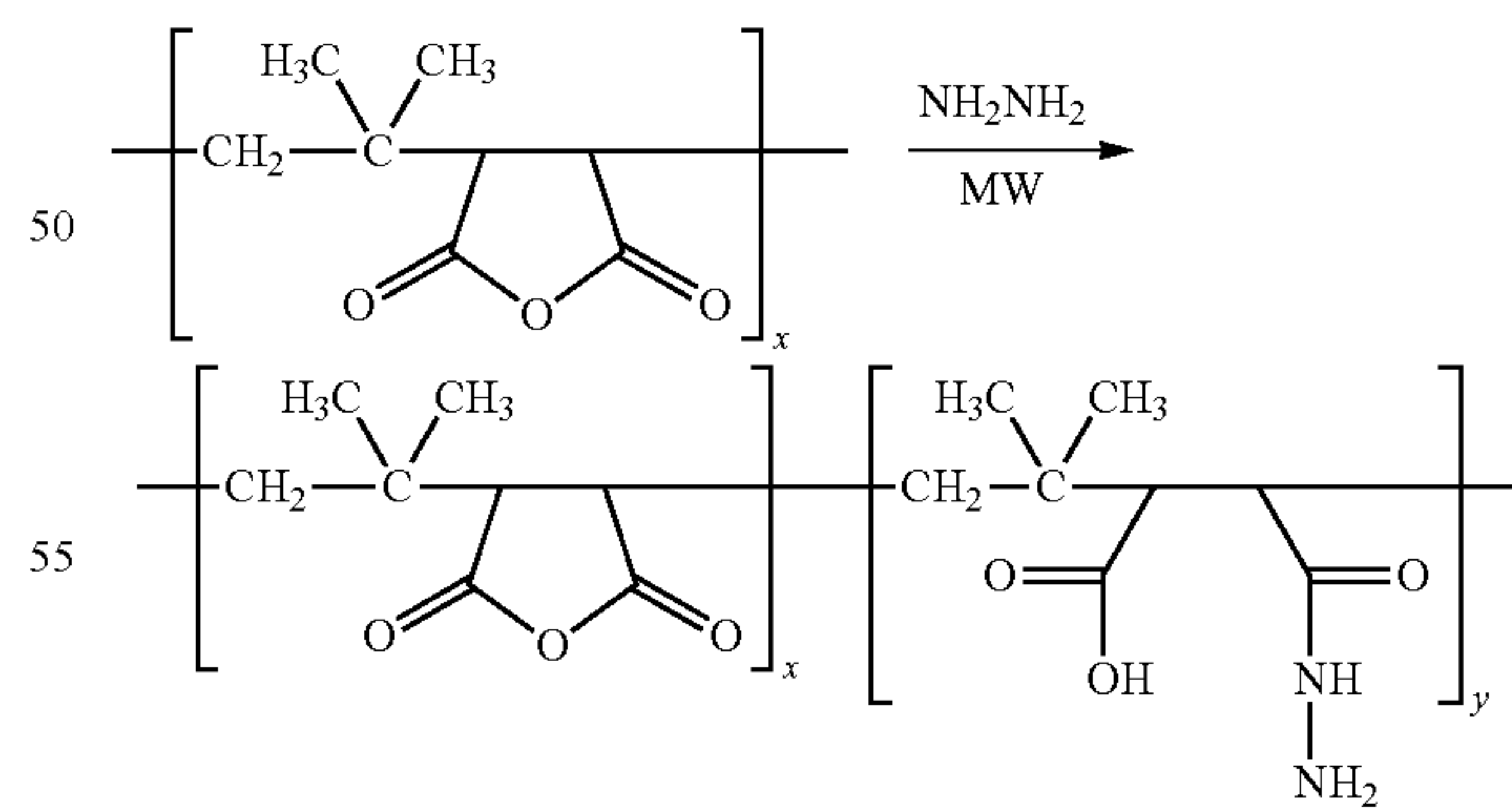
Scheme 3 Polyisobutylene-co-maleic Hydrazide
