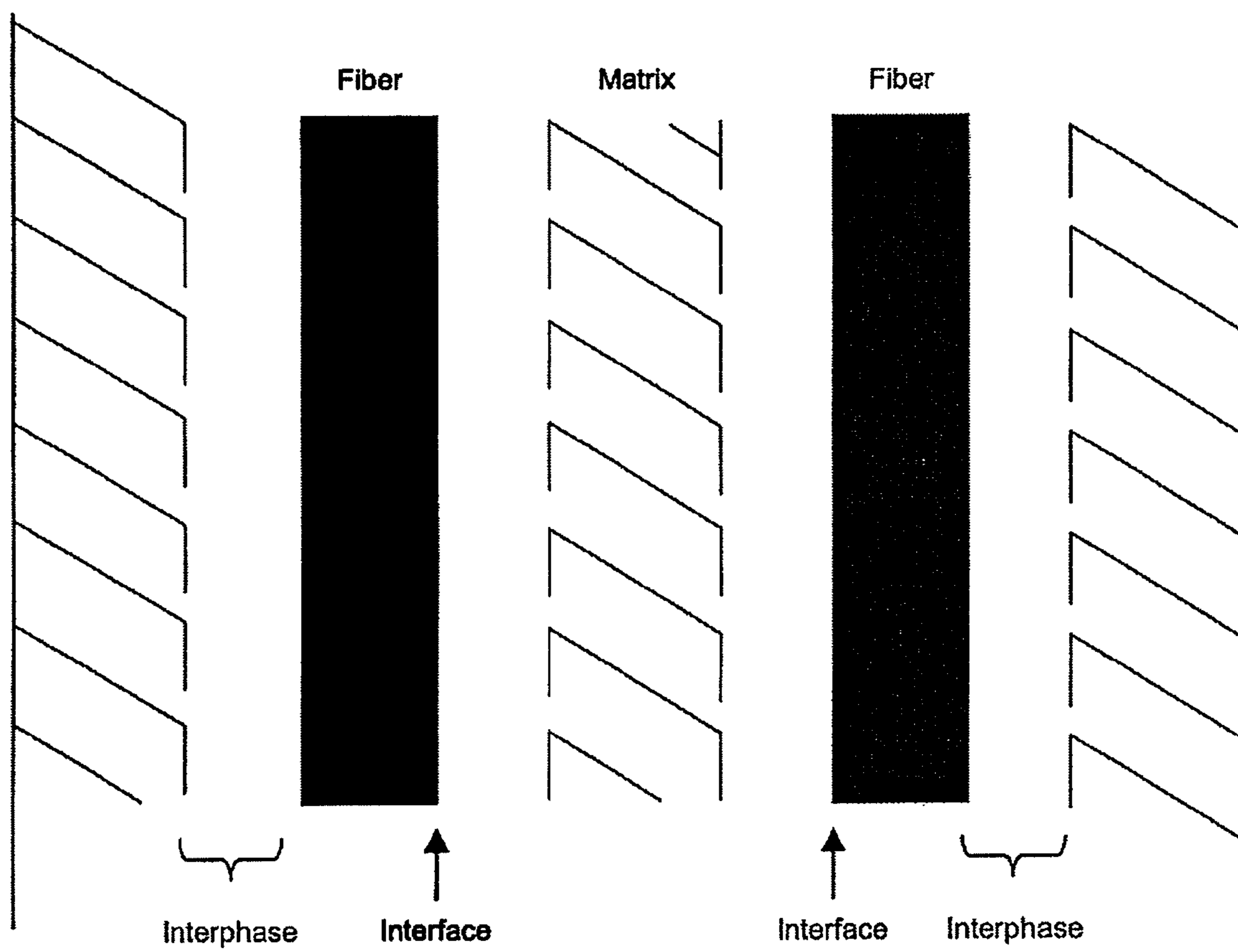
Figure 1. Fiber-Matrix Interface/Interphase in Fibrous Composite Material
