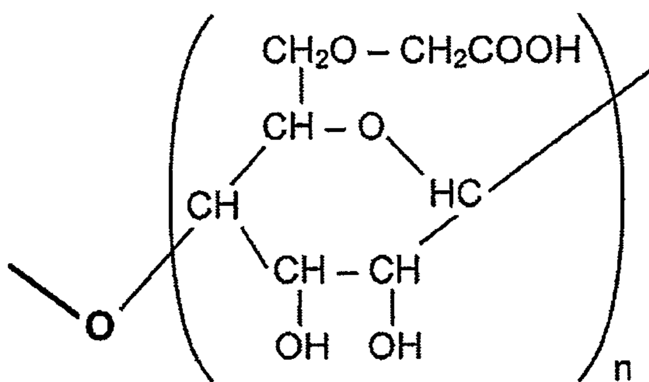
Figure 4. Carboxymethylcellulose
