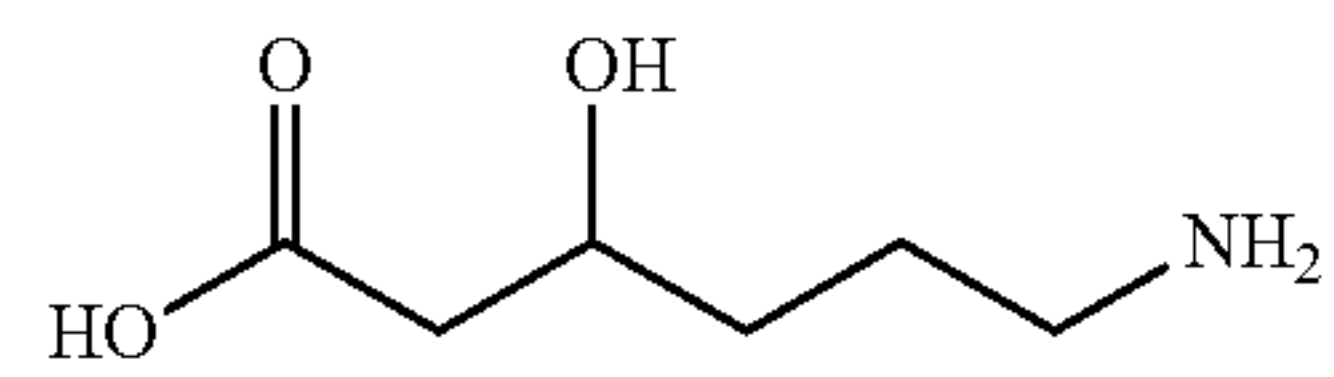
6-amino-3-hydroxyhexanoic acid
