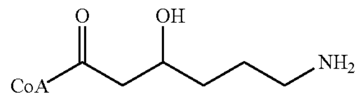
6-amino-3-hydroxyhexanoyl-CoA
