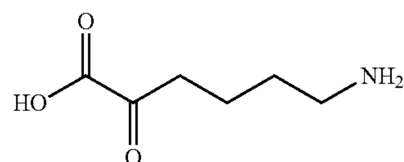
6-amino-2-oxohexanoic acid
