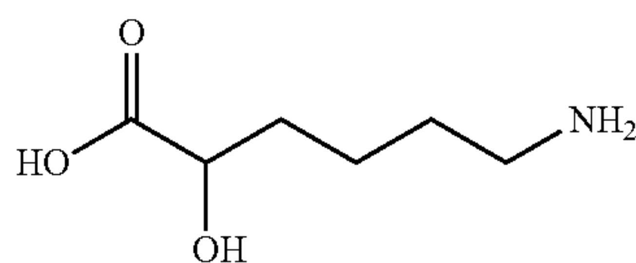
6-amino-2-hydroxyhexanoic acid
