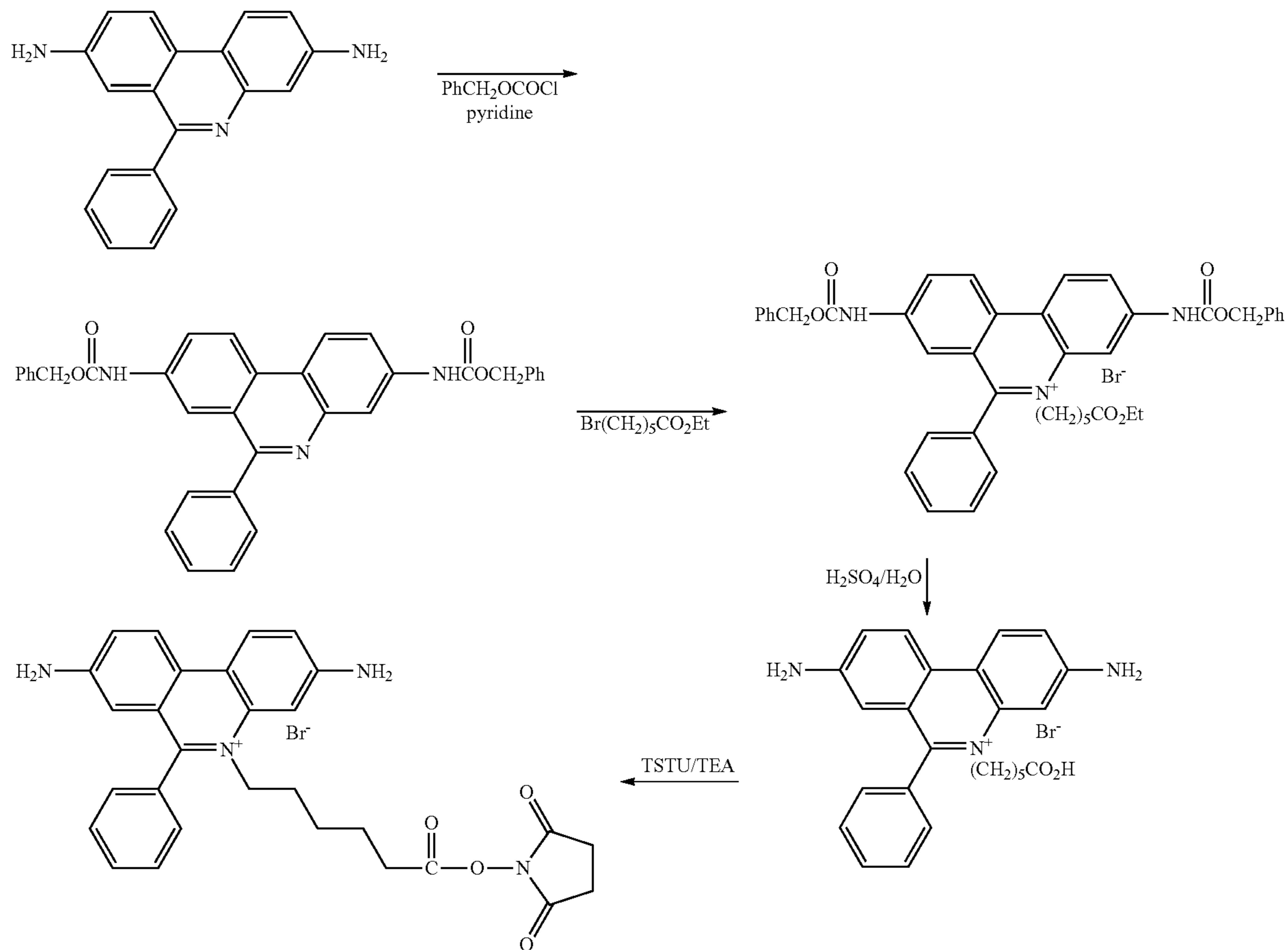
Scheme 4
