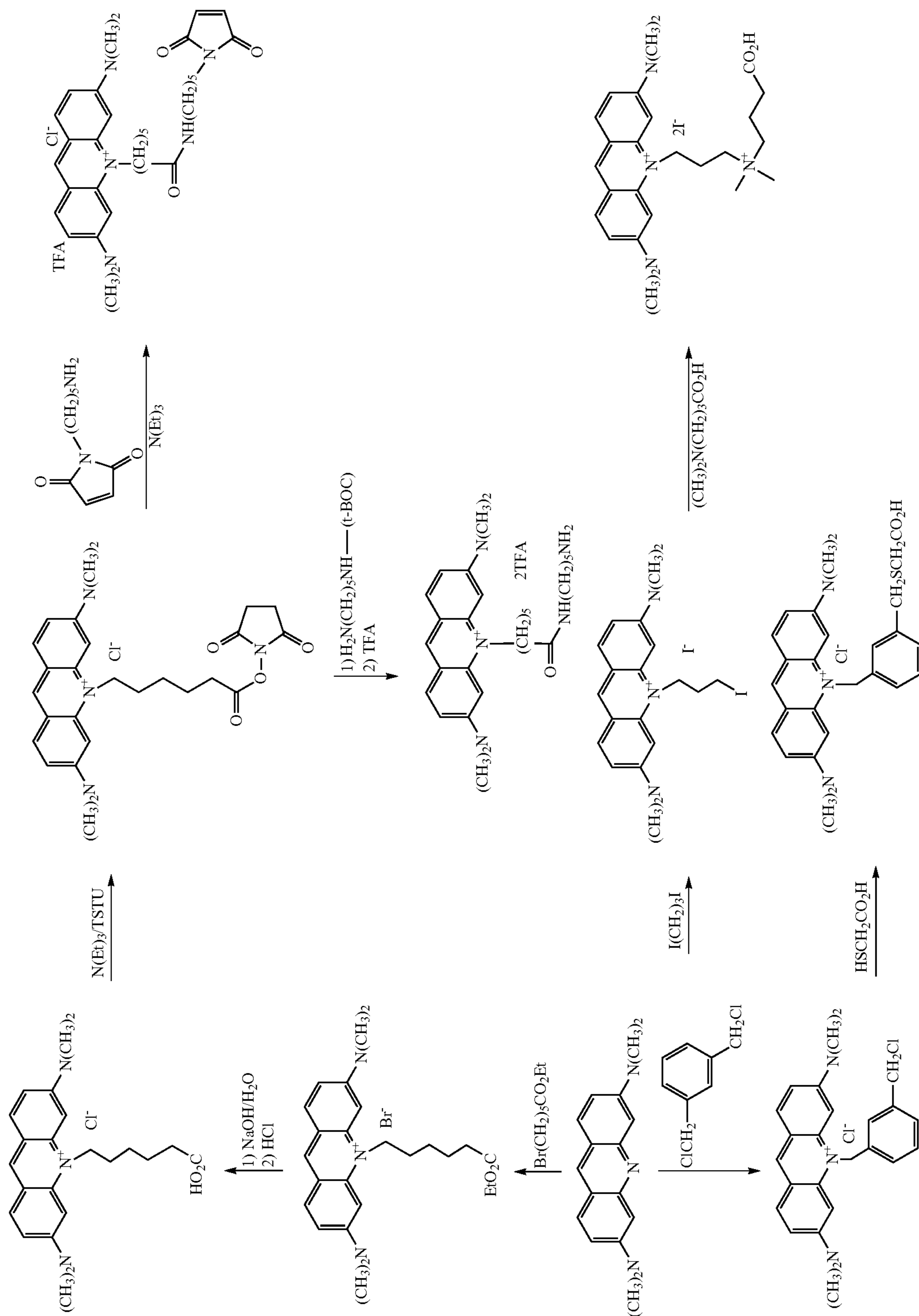
Scheme 1
