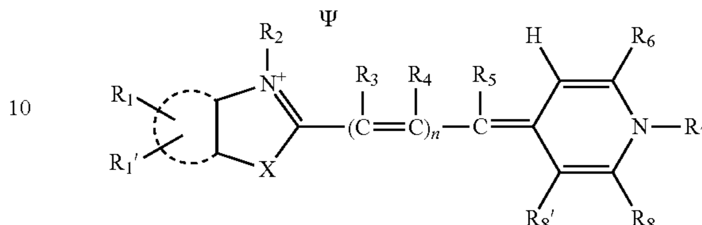
Structure 4
