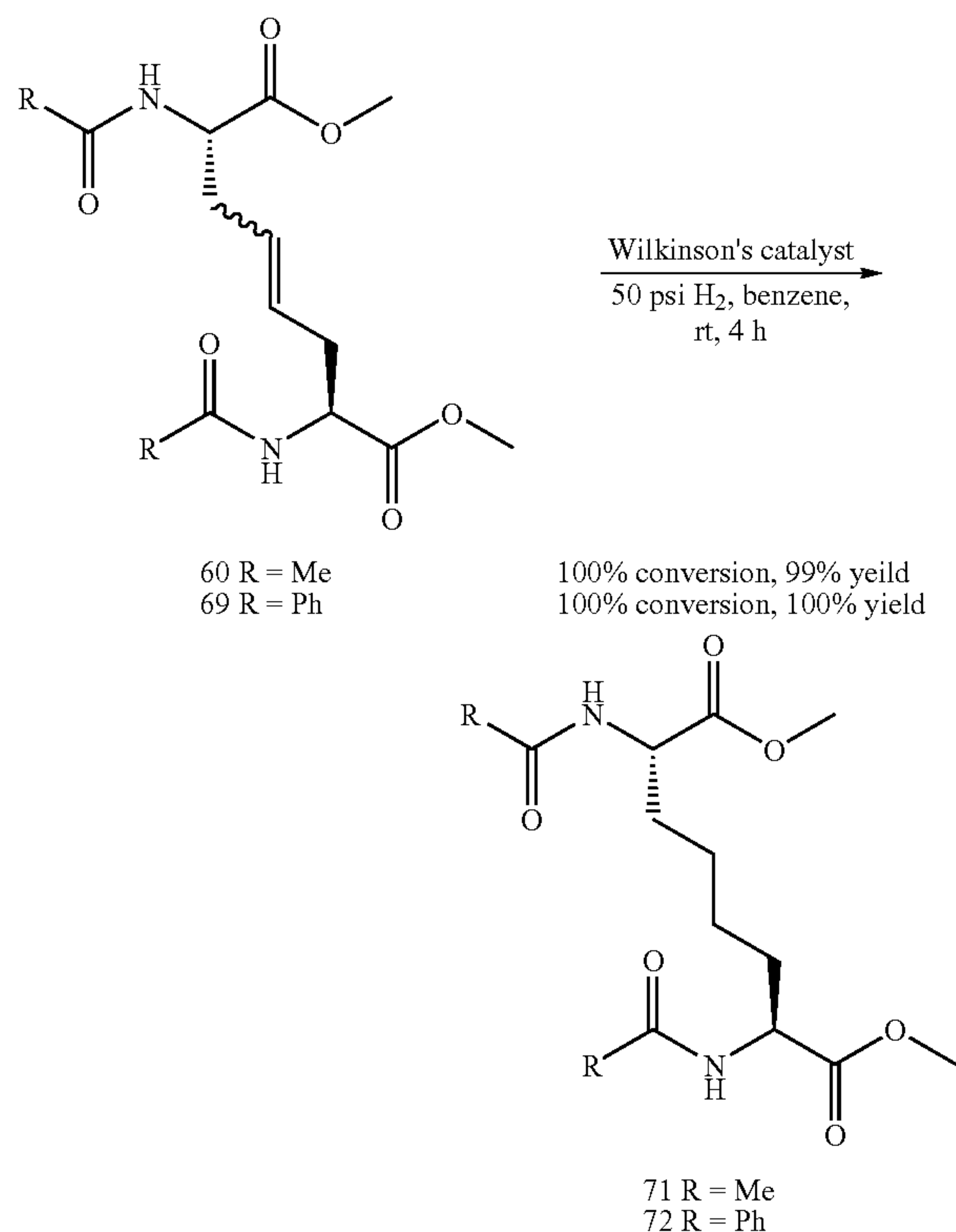
Scheme 4.19
