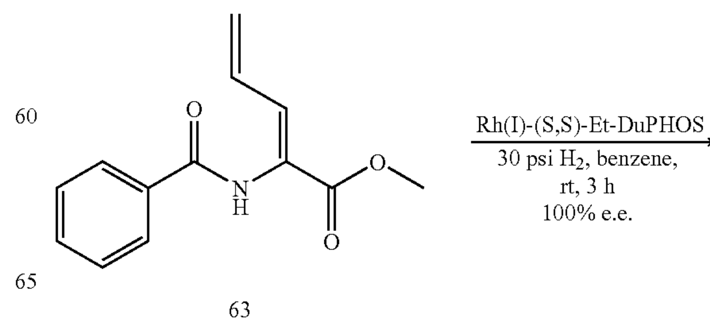
Scheme 4.16
