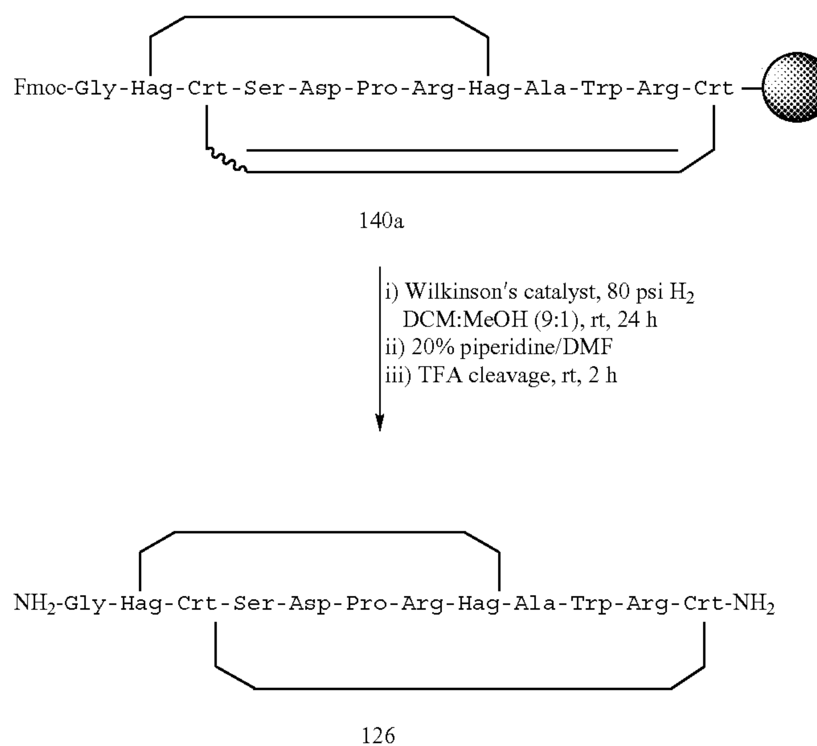
Scheme 6.31
