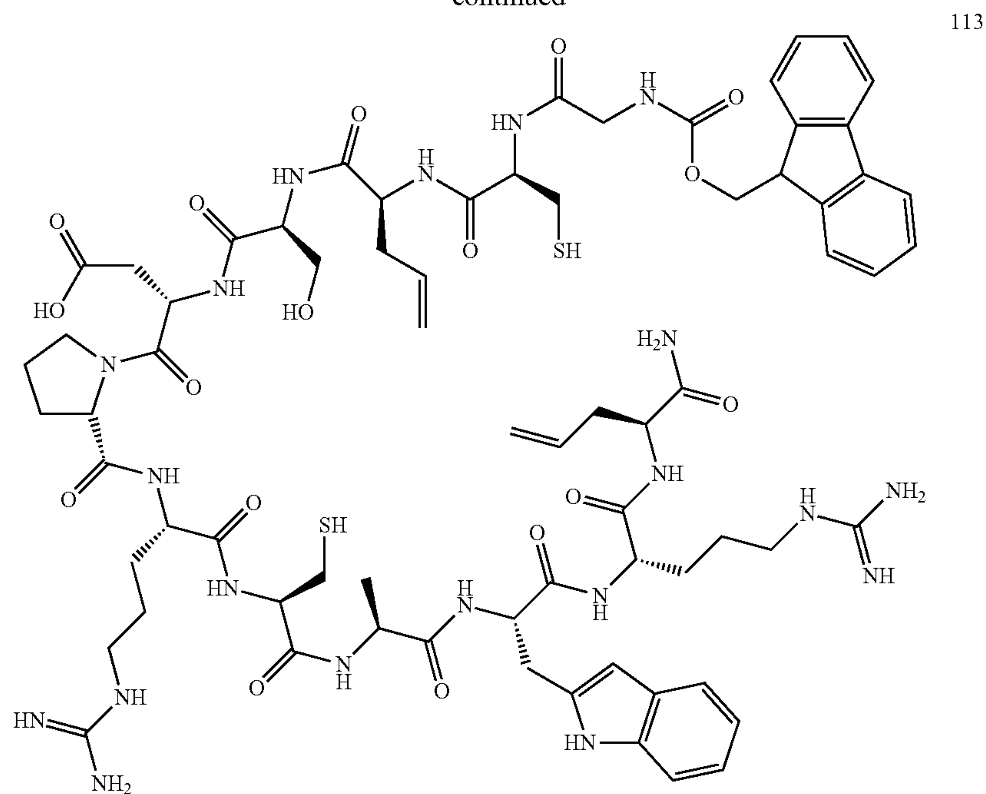
[2,8]-Cys-[3,12]-Hag conotoxin ImI: Fmoc-Gly-Cys-Hag-Ser-Asp-Pro-Arg-Cys-Ala-Trp-Arg-Hag-NH 2 (SEQ ID NO: 30)
