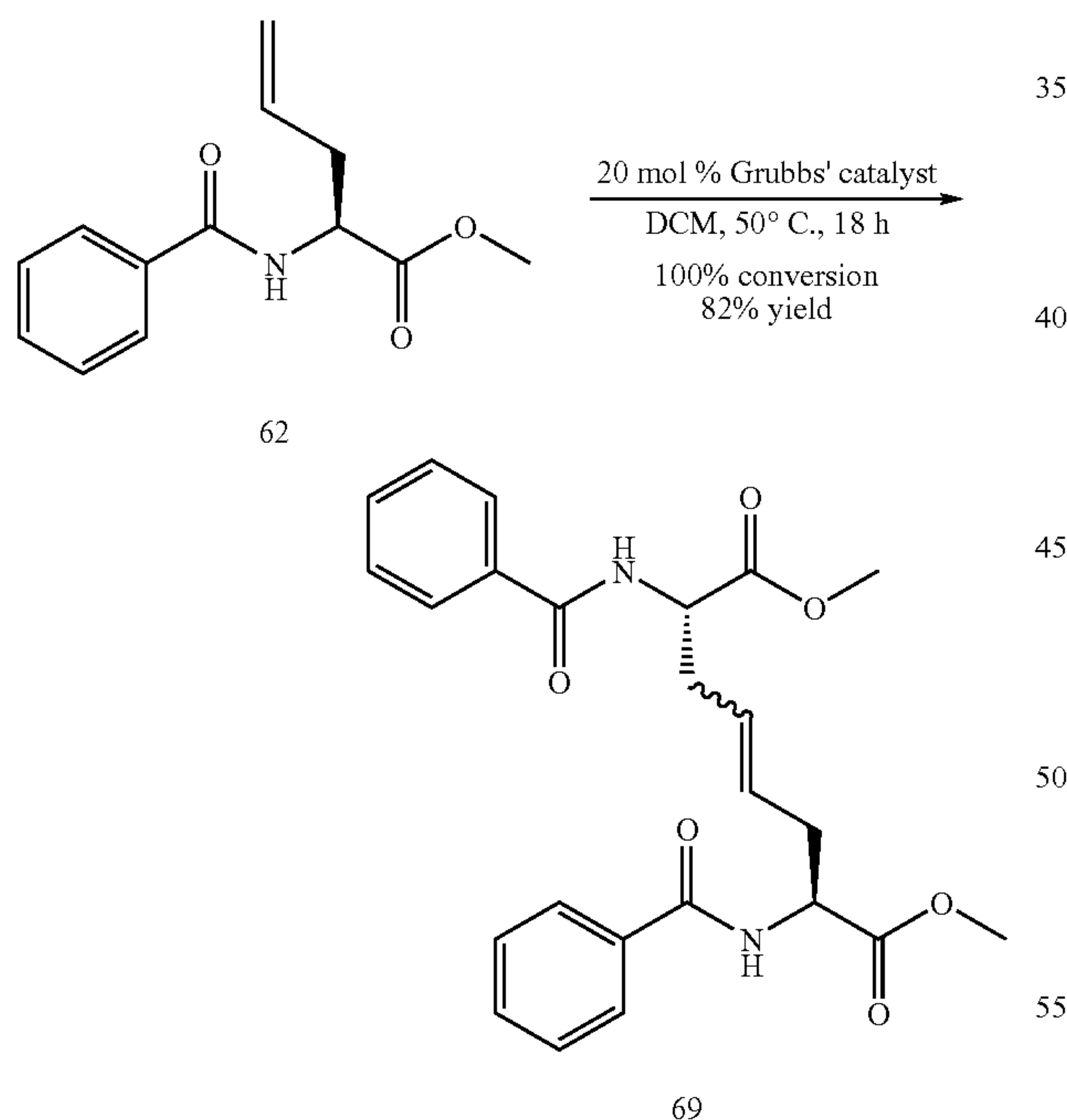
Scheme 4.17
