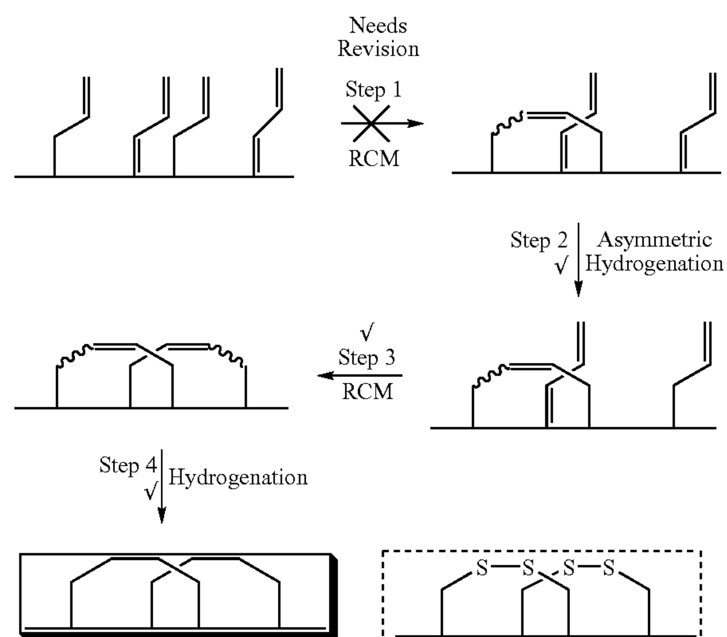
Scheme 4.21
