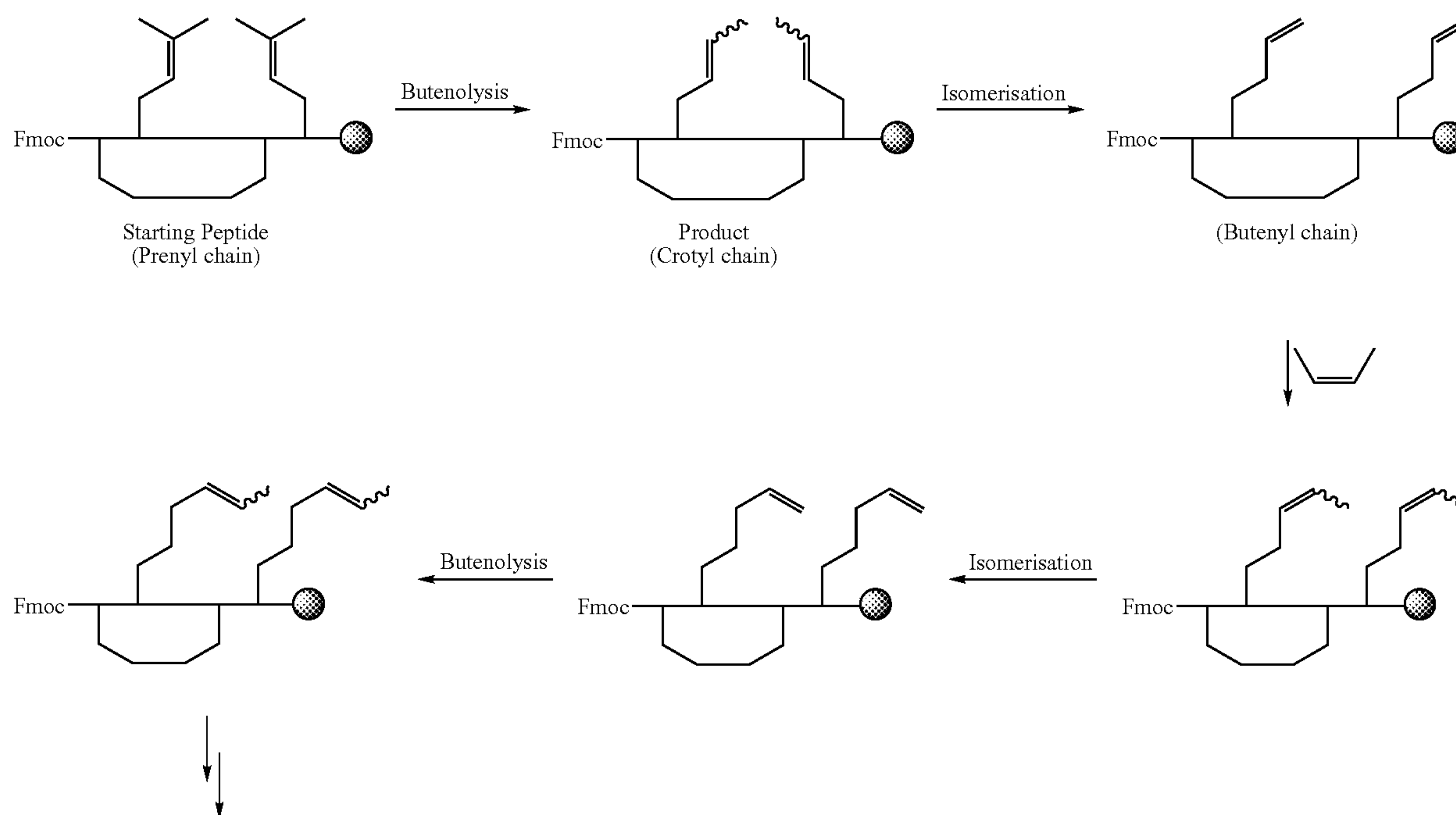
Scheme 6.29
