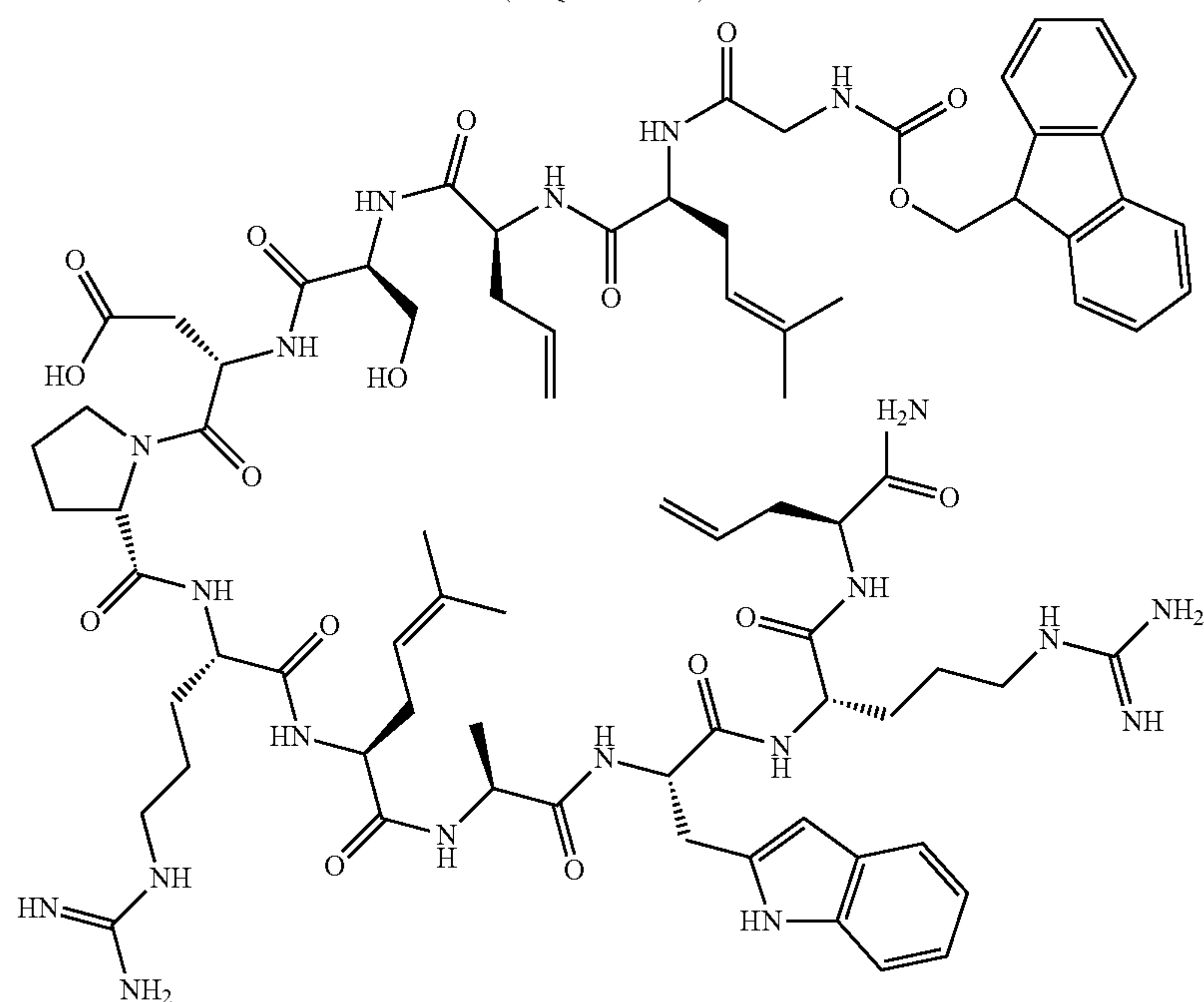
[2,8]-Pre-[3,12]-Hag conotoxin ImI: Fmoc-Gly-Pre-Hag-Ser-Asp-Pro-Arg-Pre-Ala-Trp-Arg-Hag-NH 2 128 (SEQ ID NO: 36)
