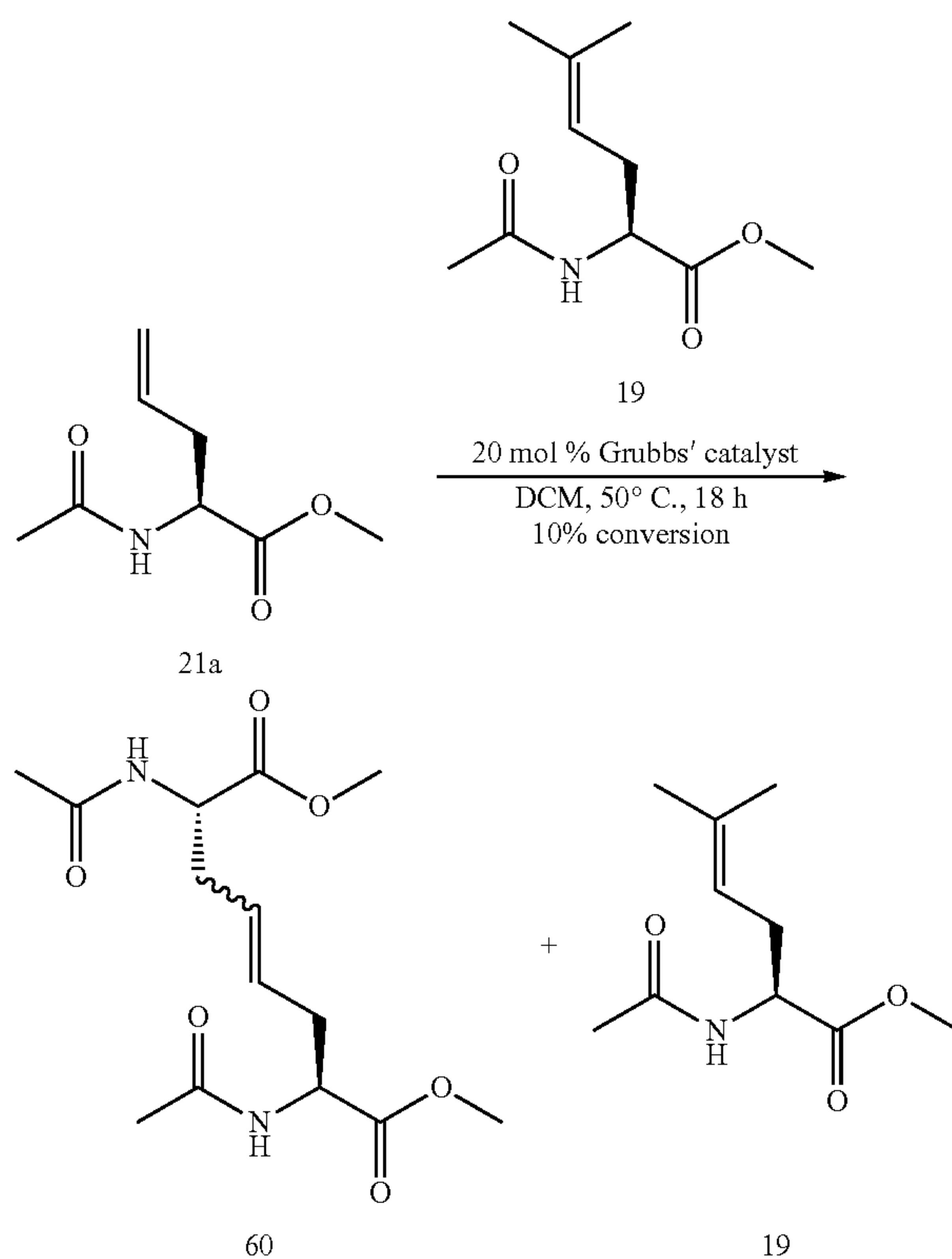
Scheme 4.32
