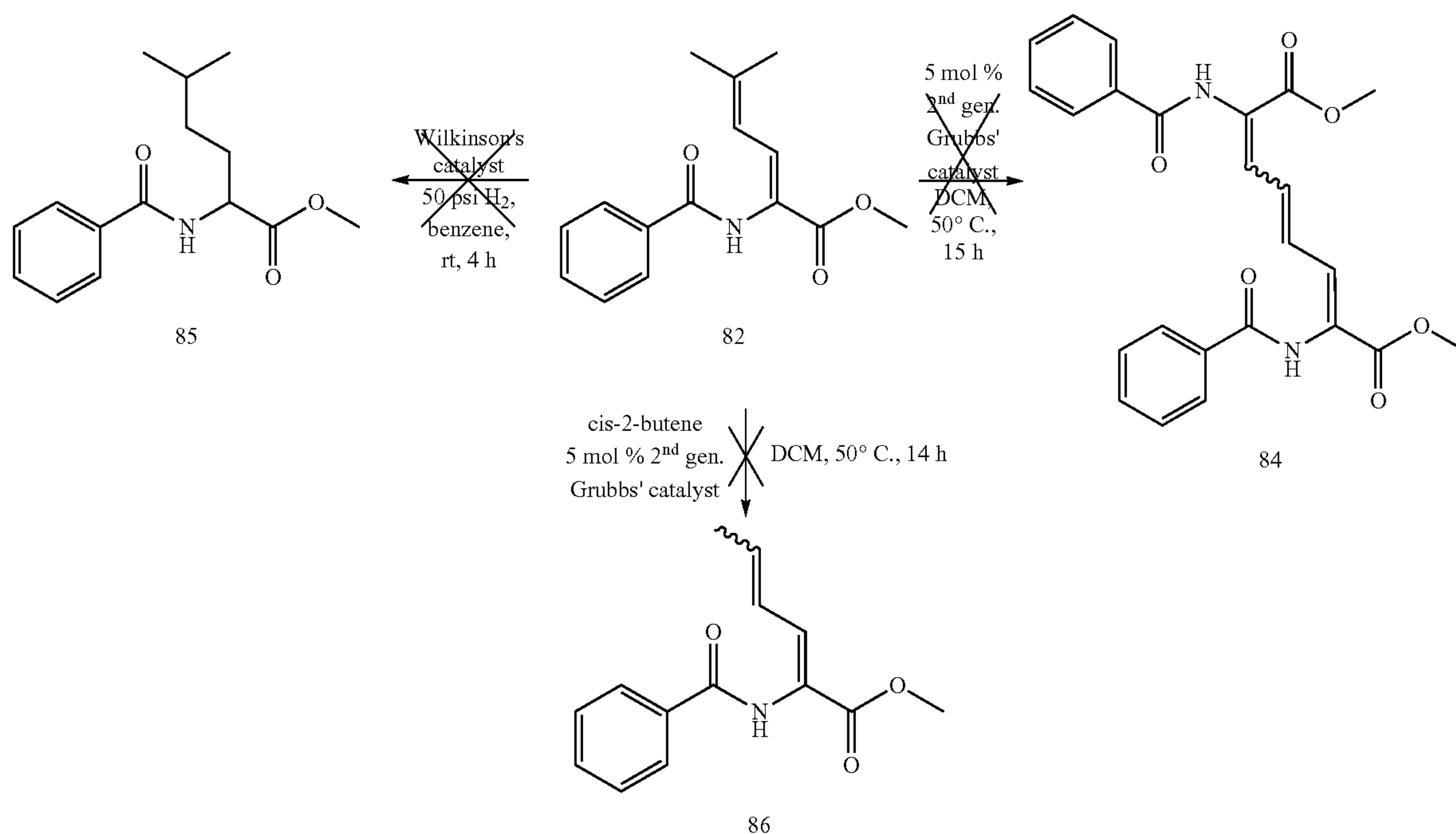
Scheme 5.3
