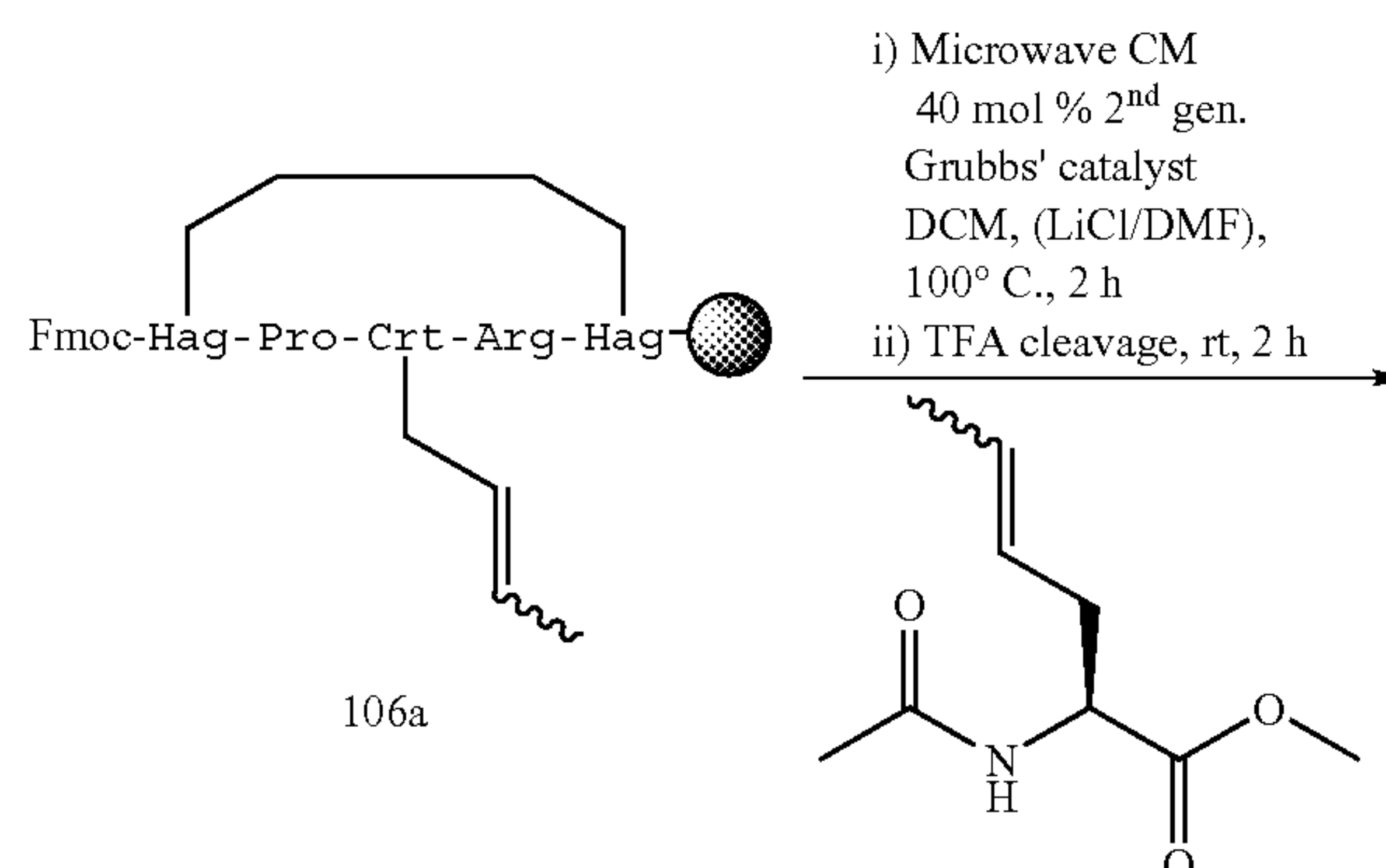
Scheme 6.12
