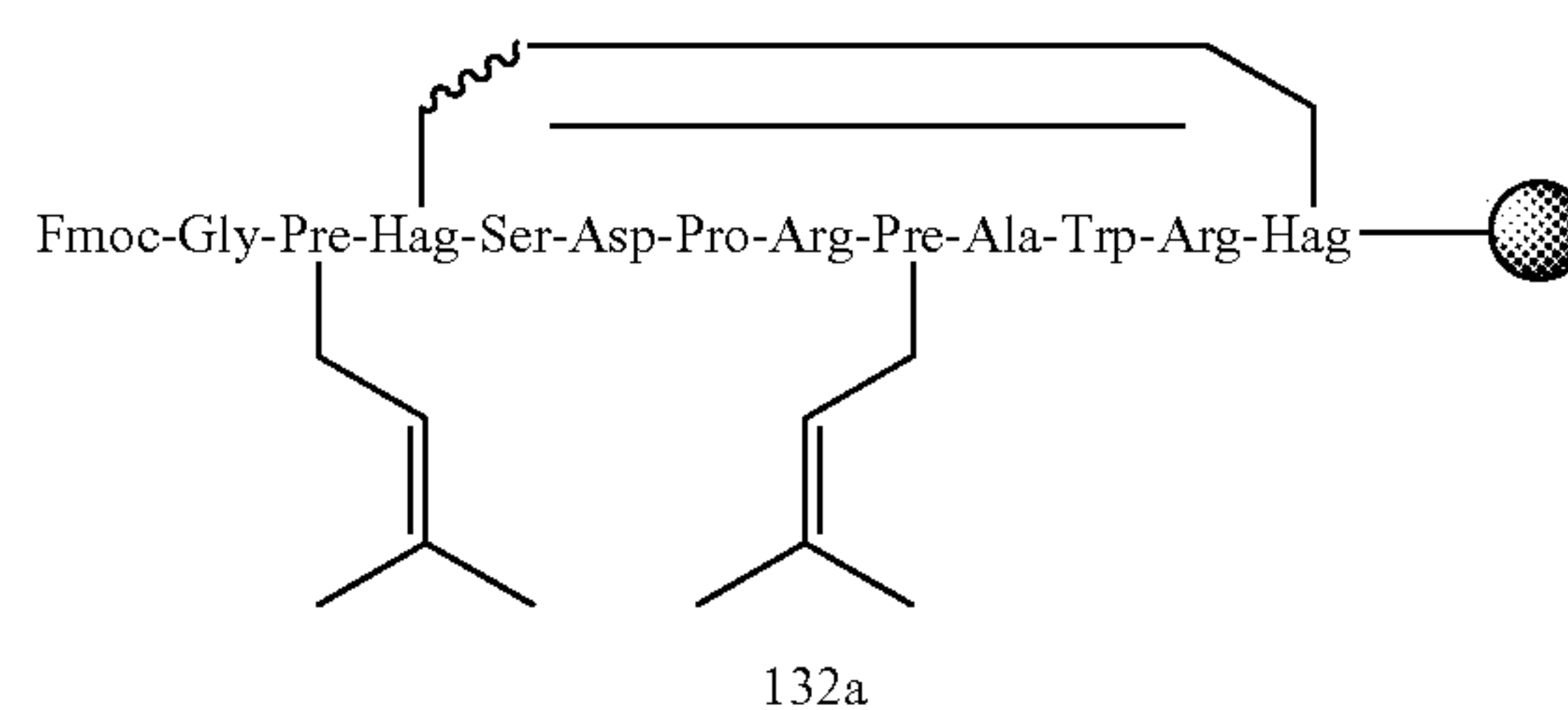
Scheme 6.27
