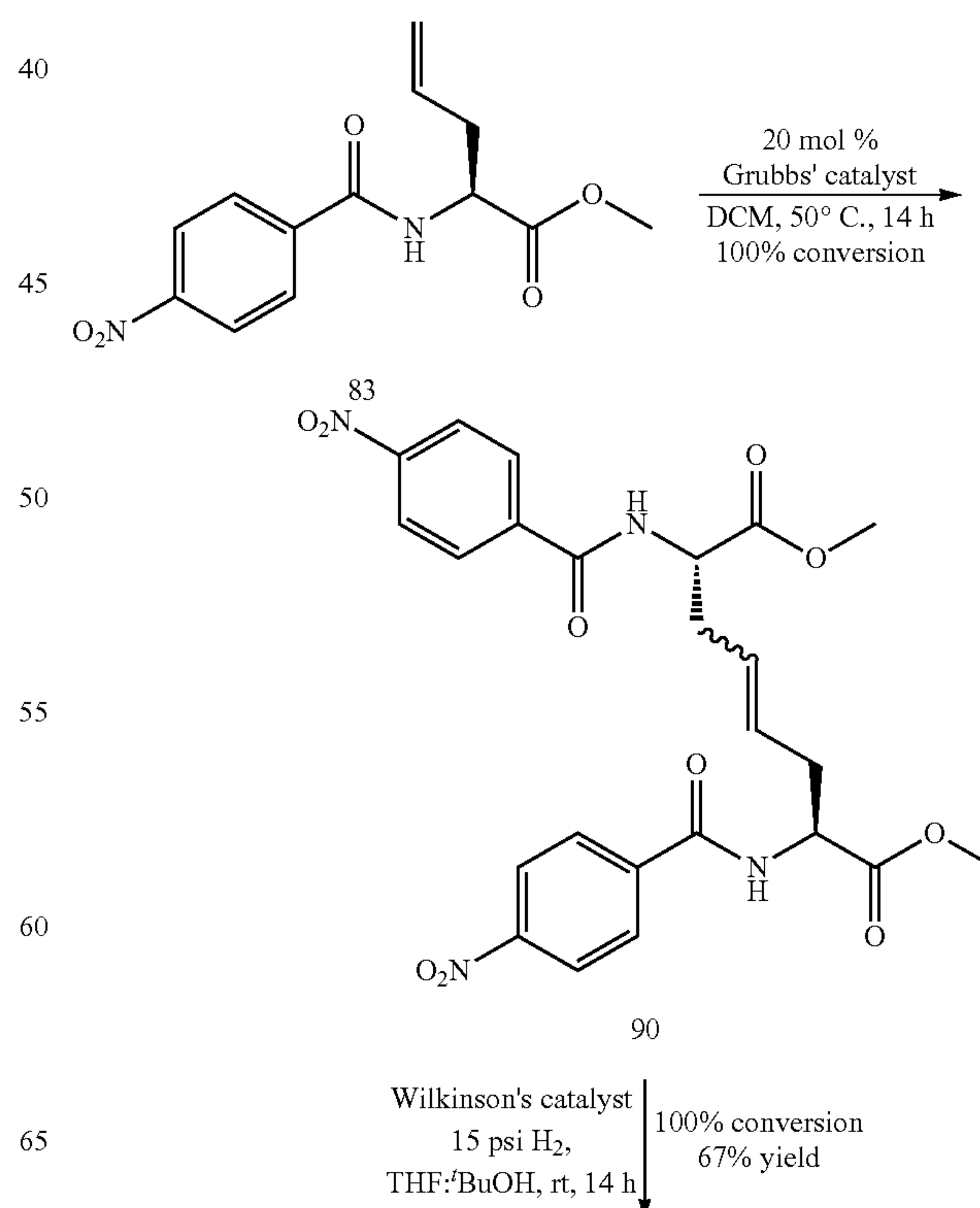
Scheme 5.6
