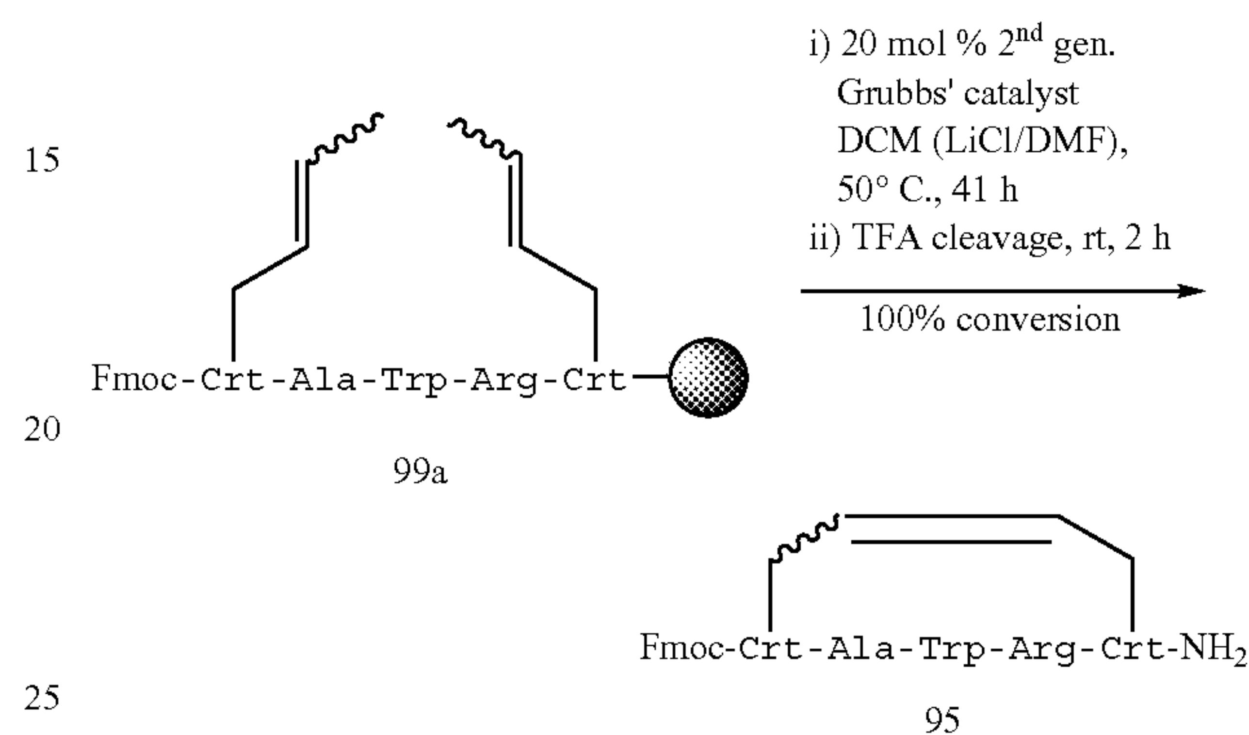
Scheme 6.6
