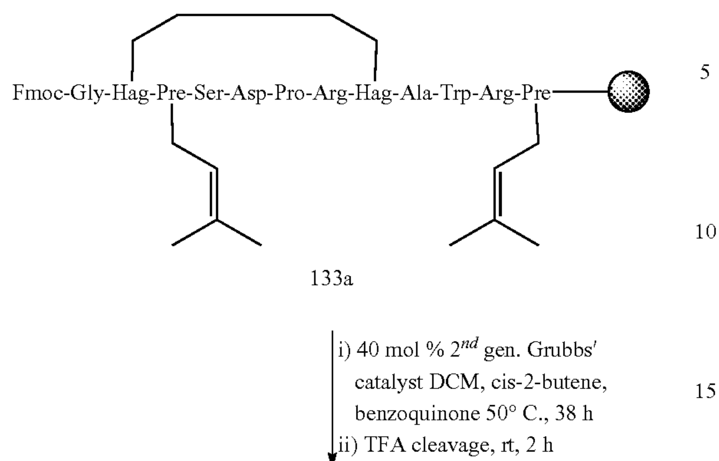
Scheme 6.28
