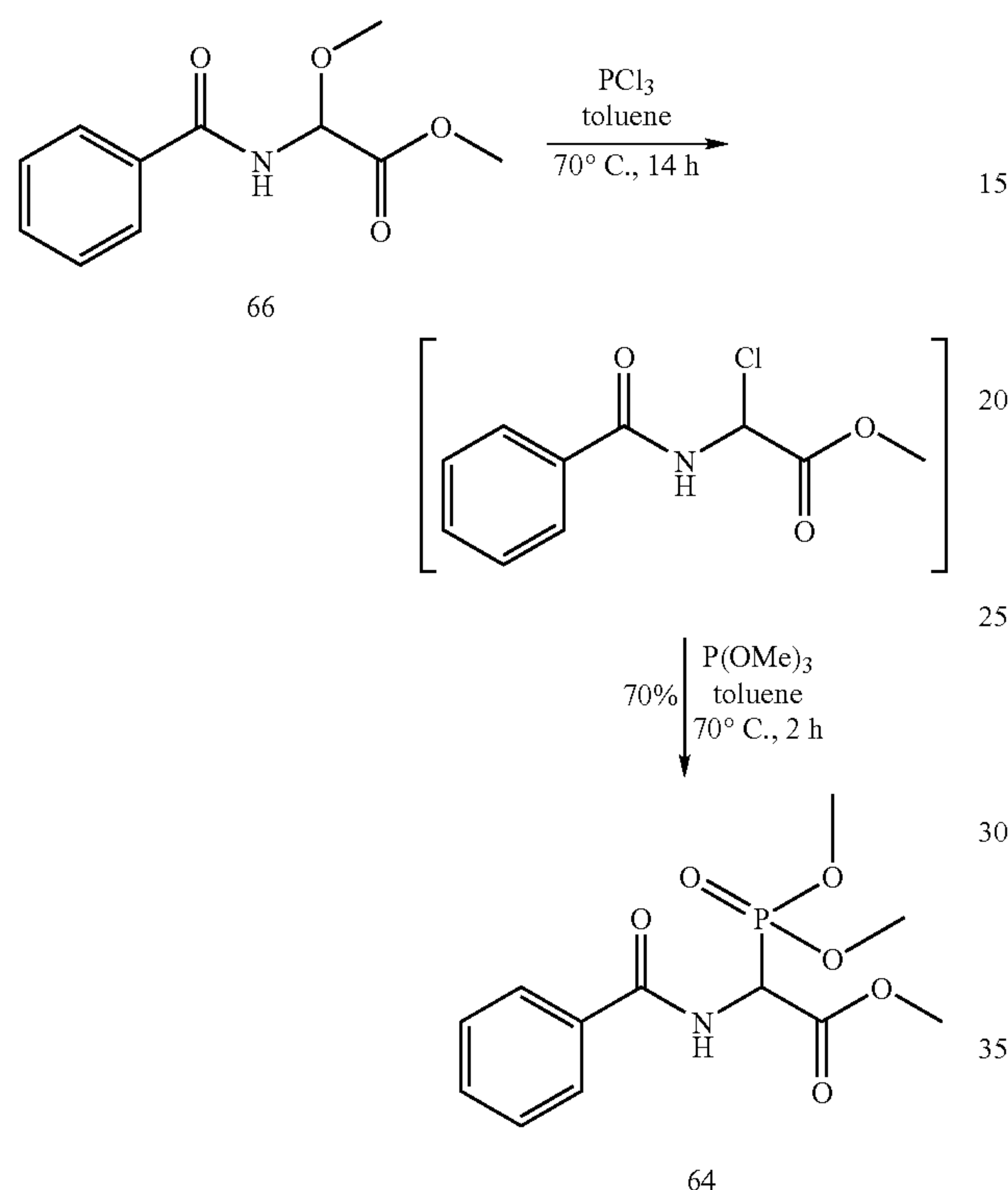
Scheme 4.14
