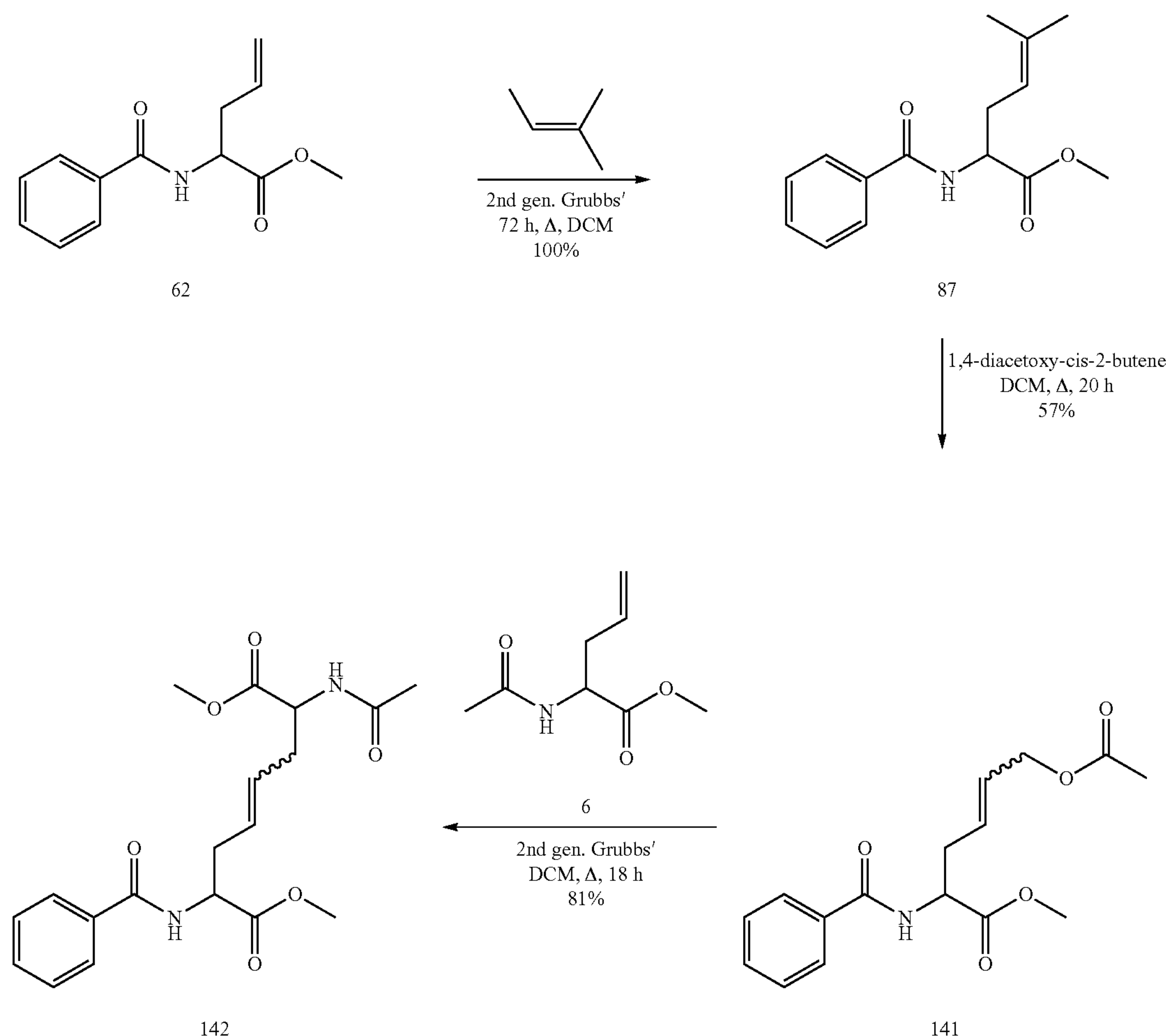
Scheme 6.32
