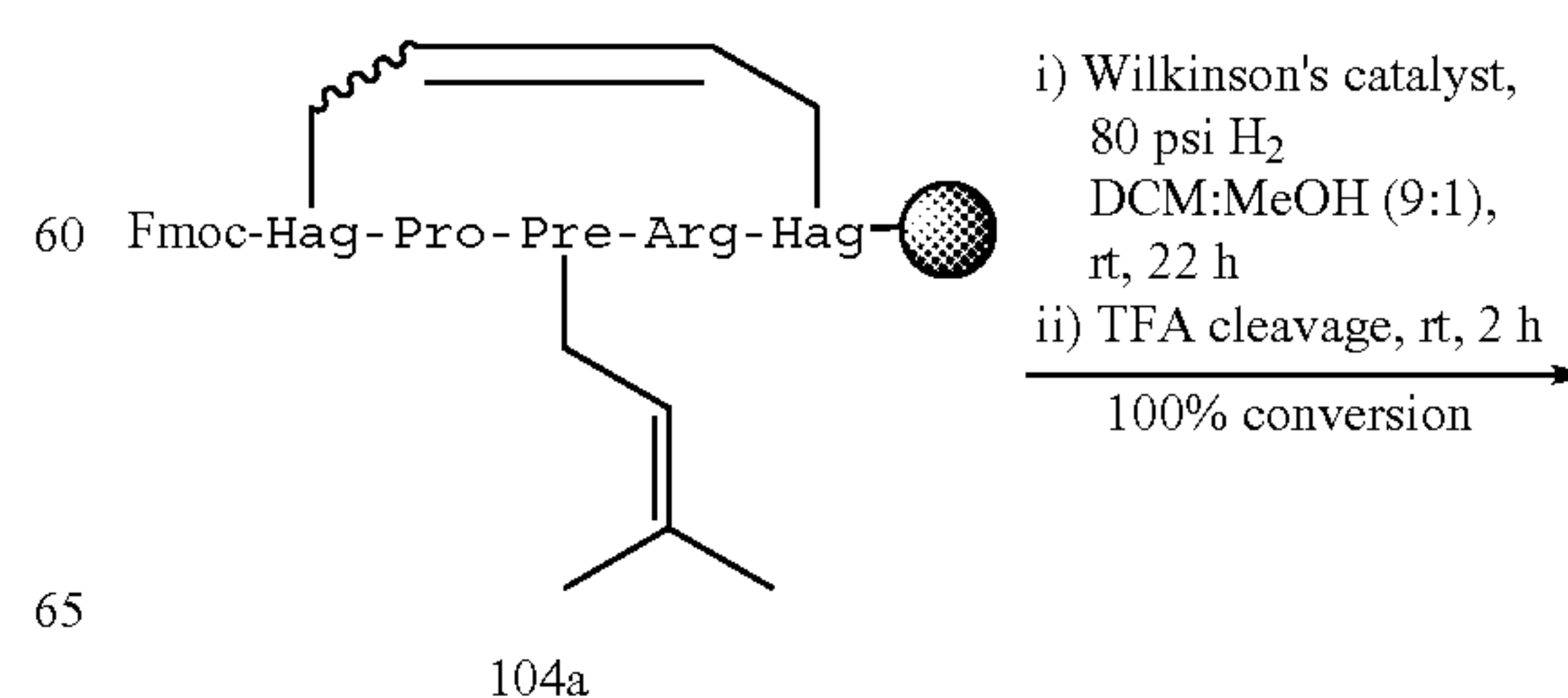
Scheme 6.10
