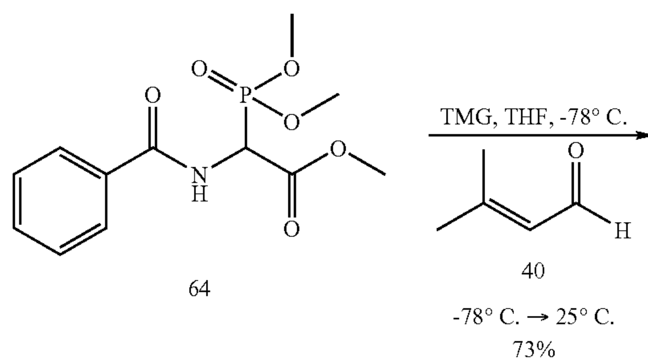
Scheme 5.2
