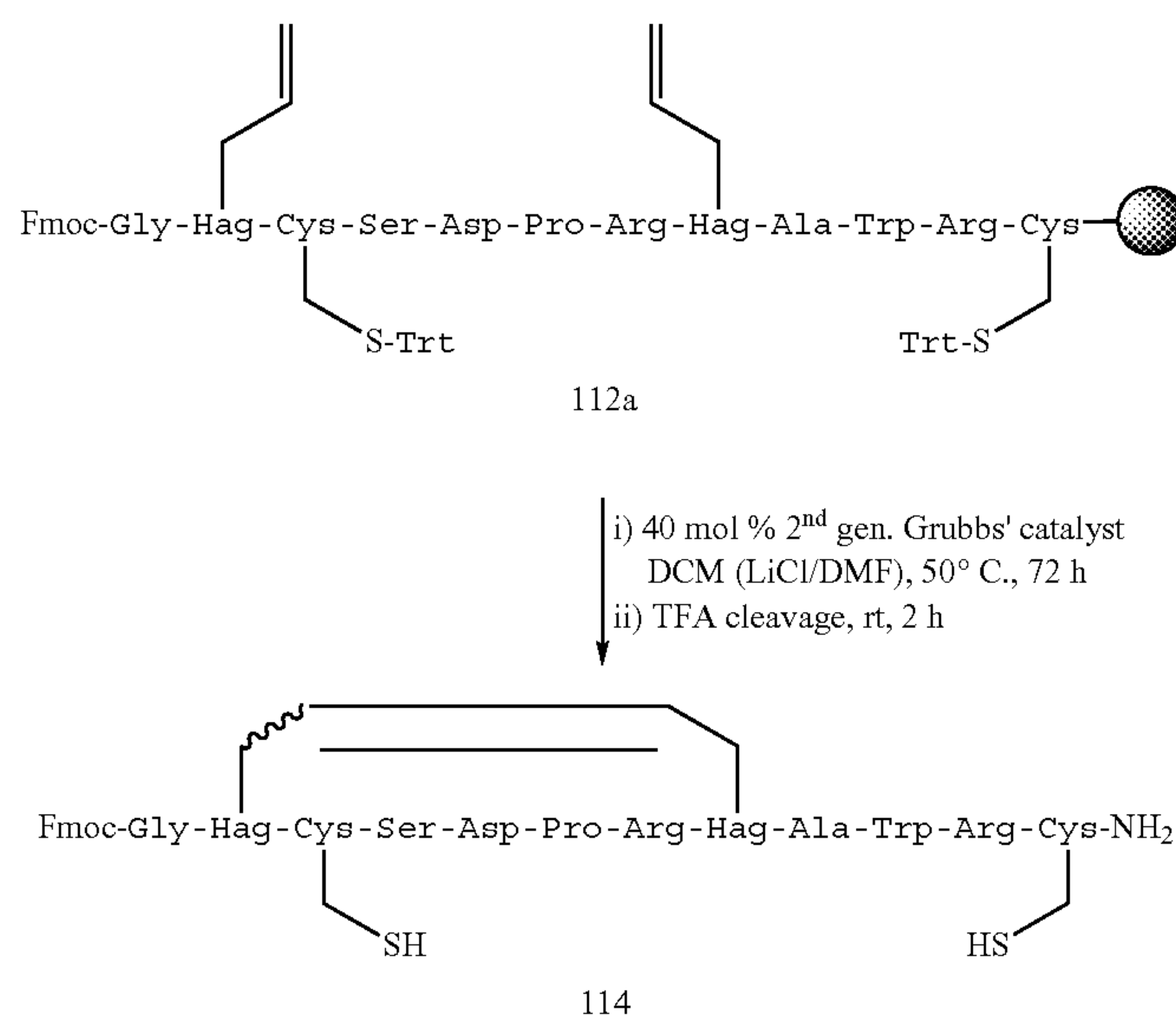
Scheme 6.15
