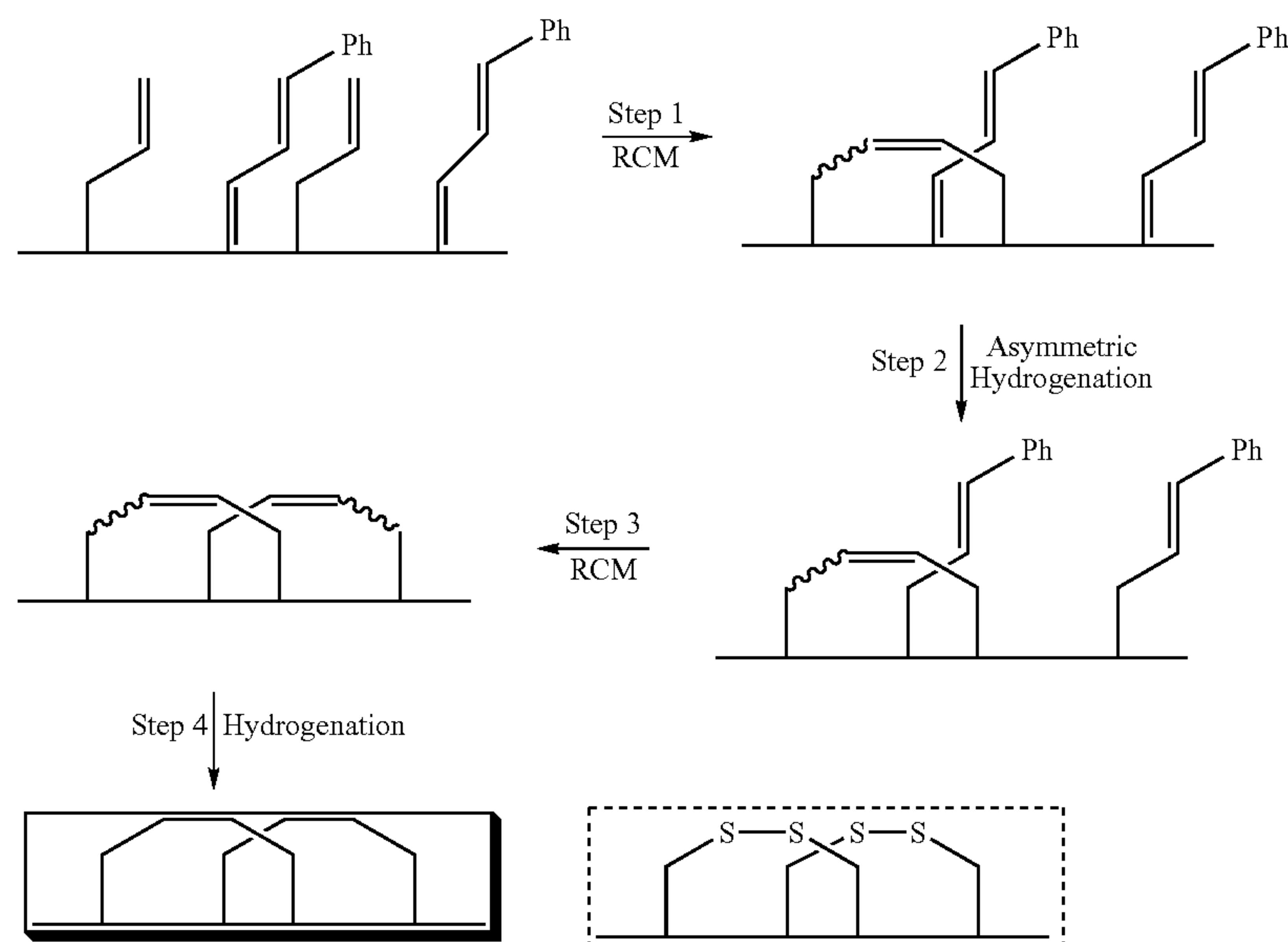
Scheme 4.22
