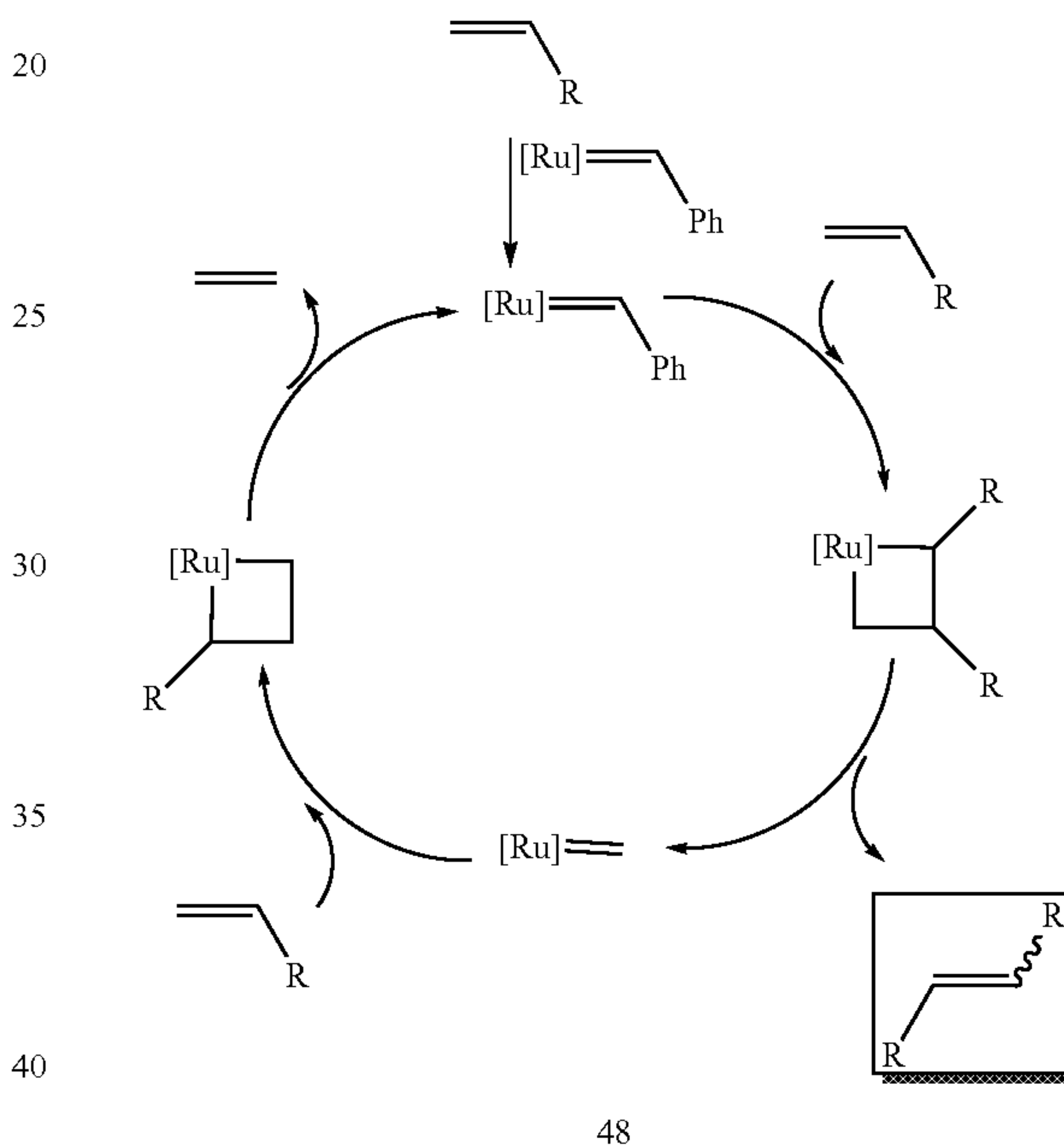
Scheme 4.7
