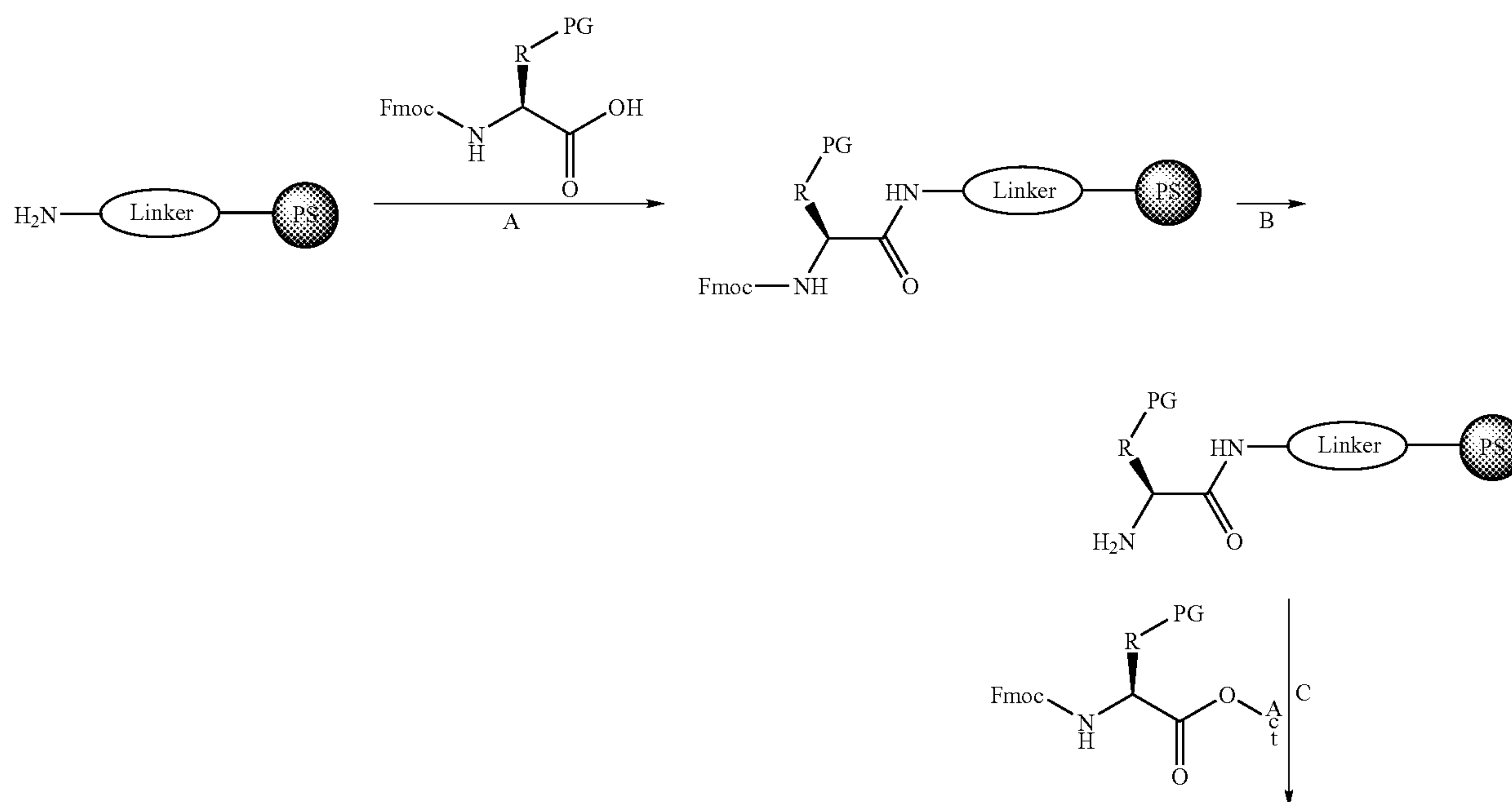
Scheme 6.1
