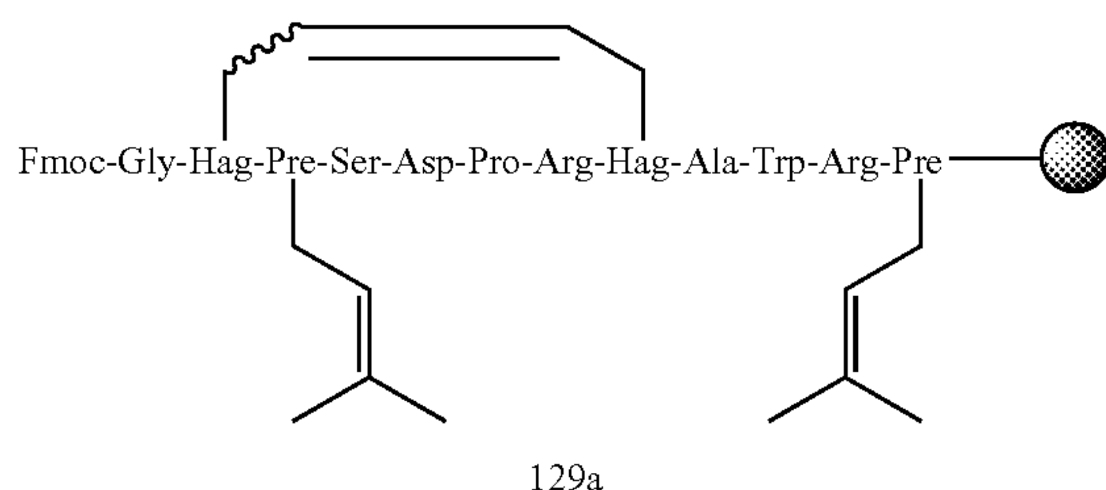
Scheme 6.26
