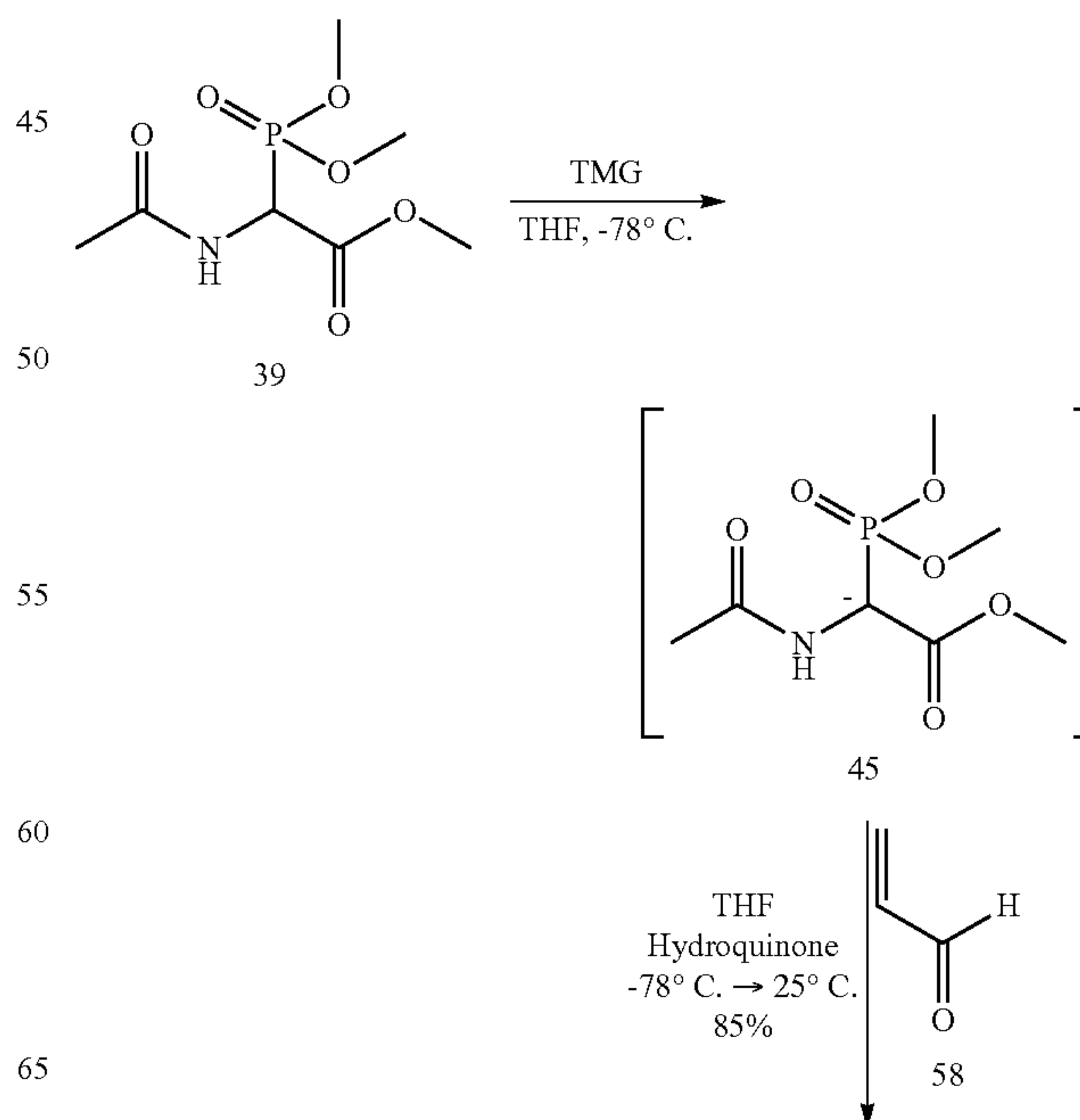
Scheme 4.4
