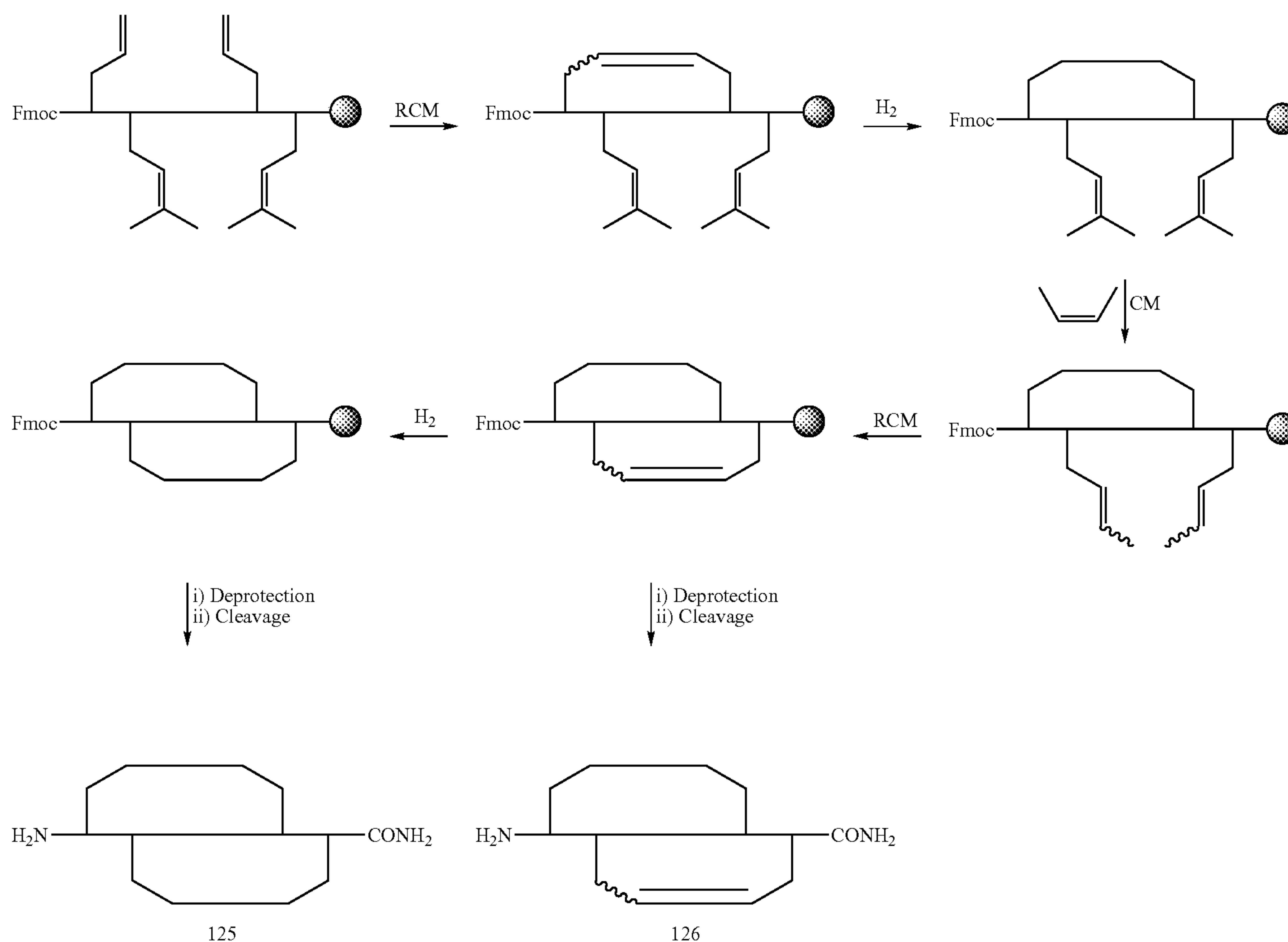
Scheme 6.21
