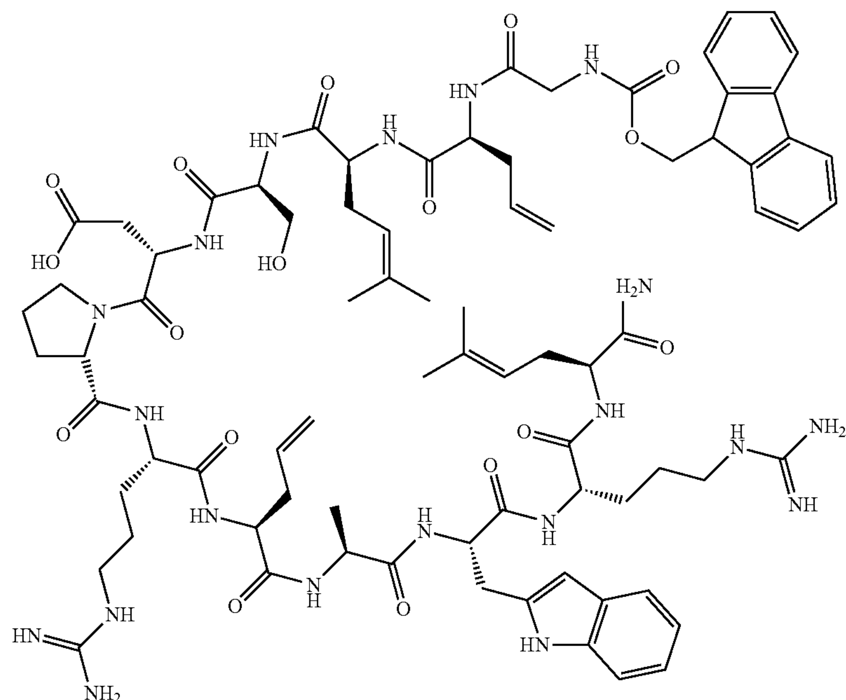
[2,8]-Hag-[3,12]-Pre conotoxin ImI: Fmoc-Gly-Hag-Pre-Ser-Asp-Pro-Arg-Hag-Ala-Trp-Arg-Pre-NH 2 127 (SEQ ID NO: 35)
