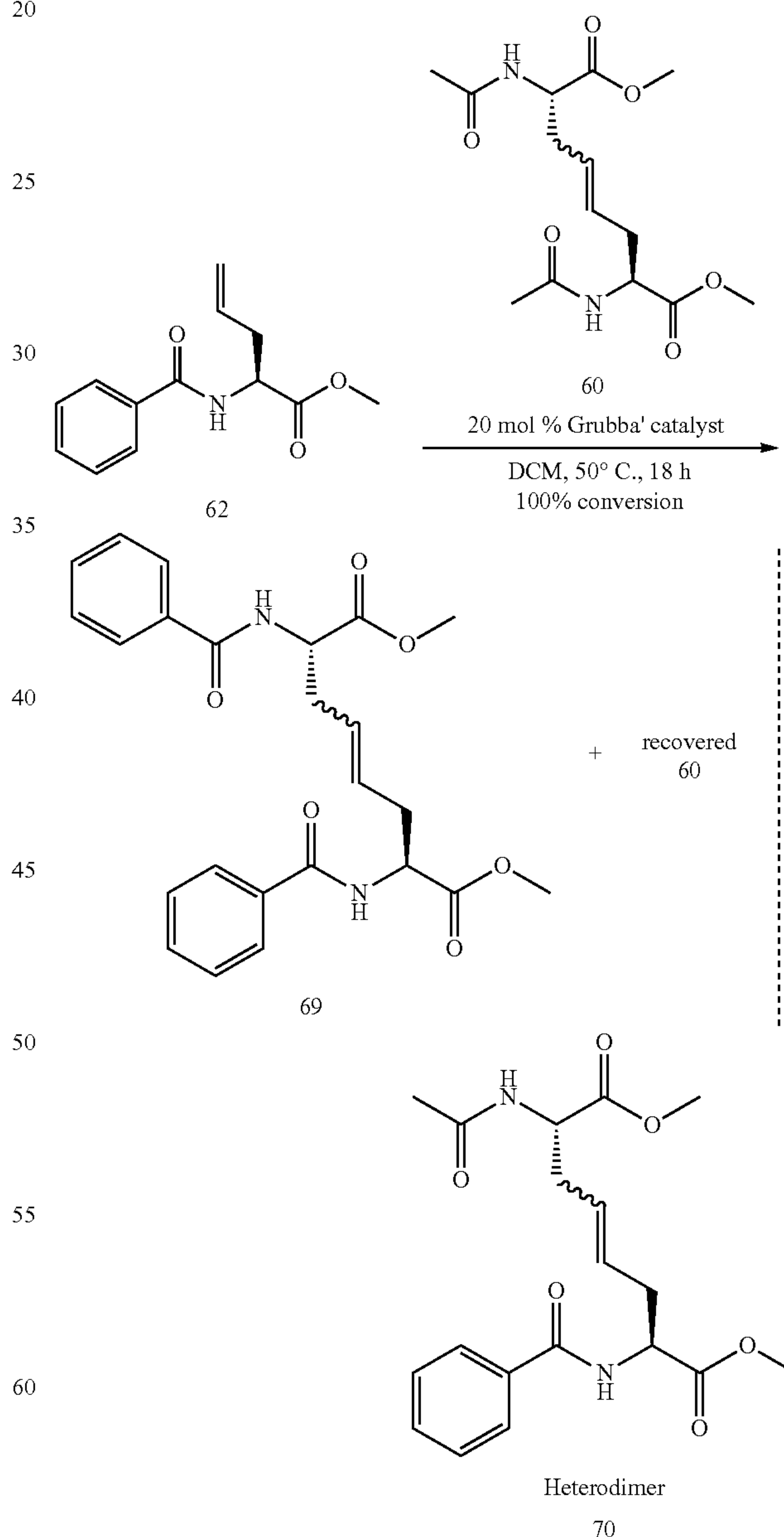
Scheme 4.18
