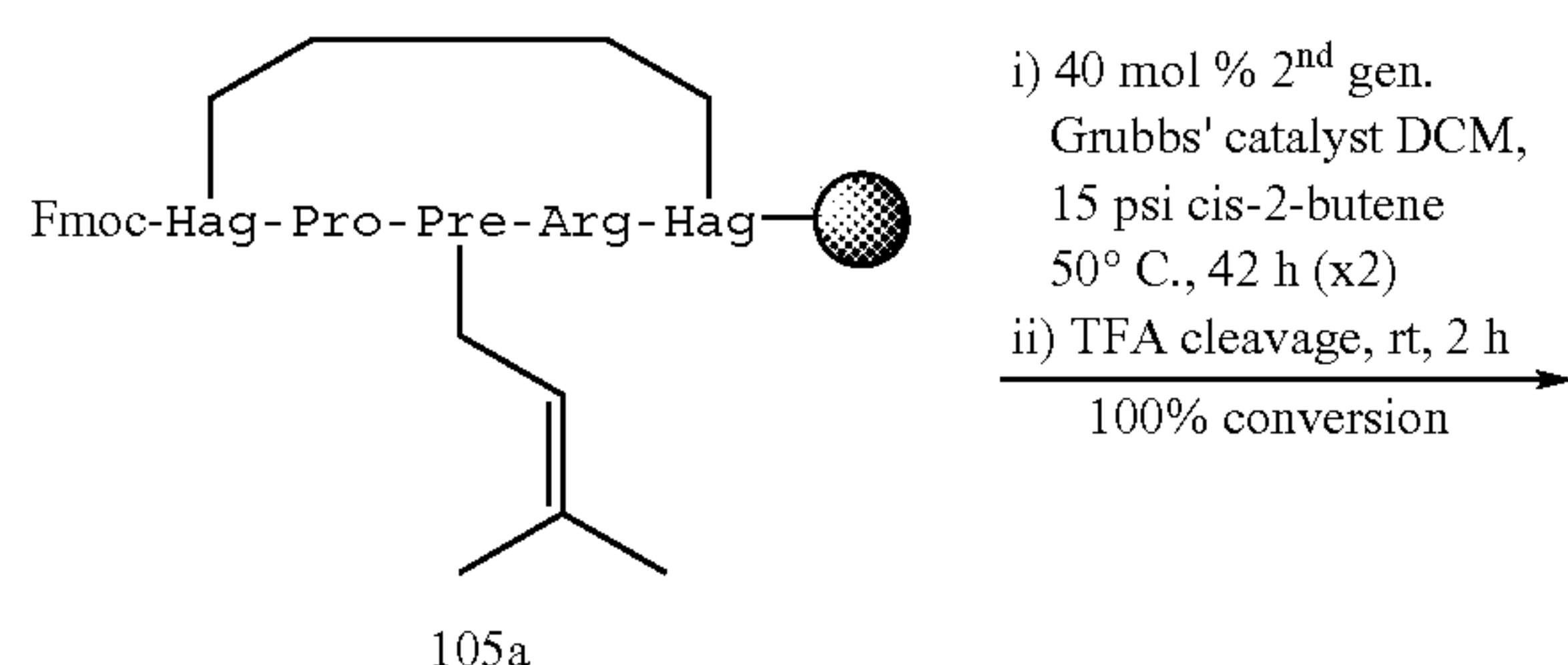
Scheme 6.11
