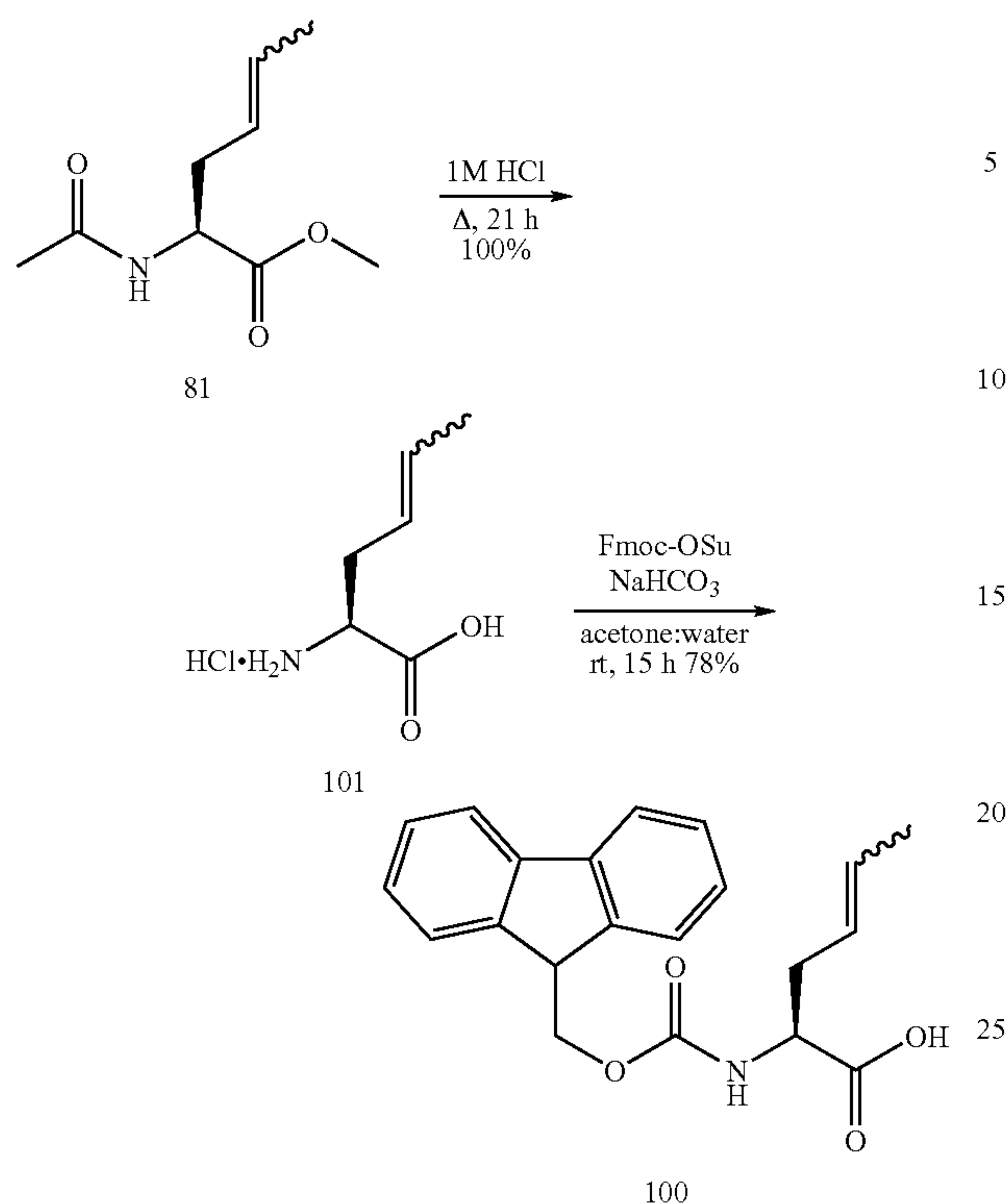
65 Scheme 6.5
