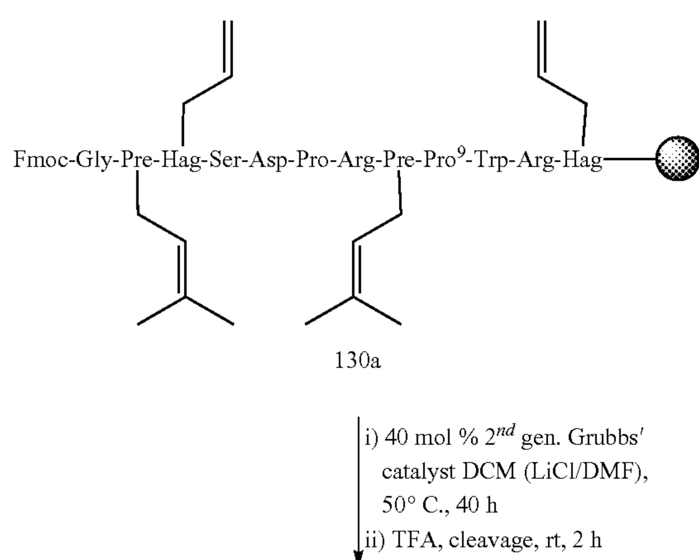
Scheme 6.23
