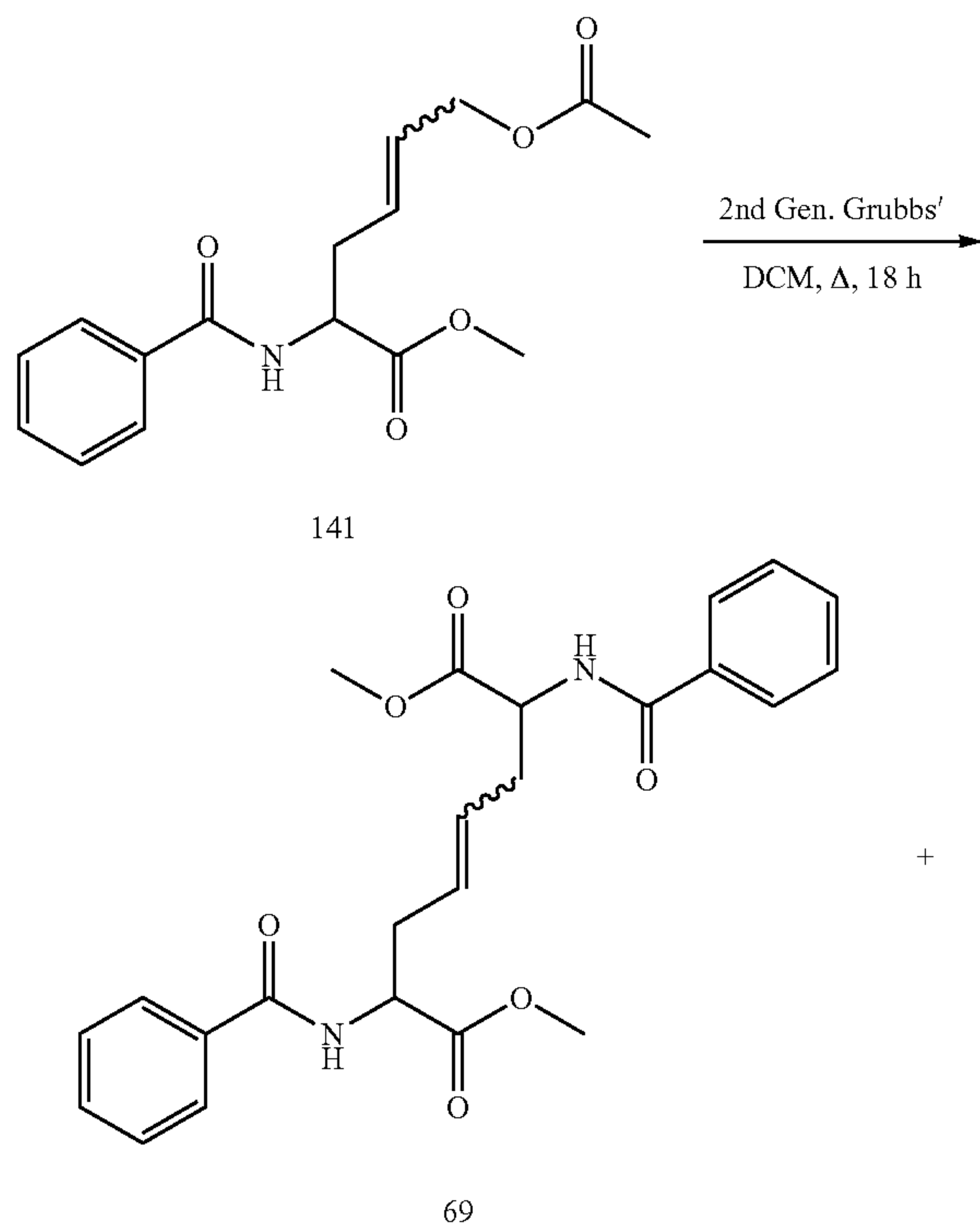
Scheme 6.33
