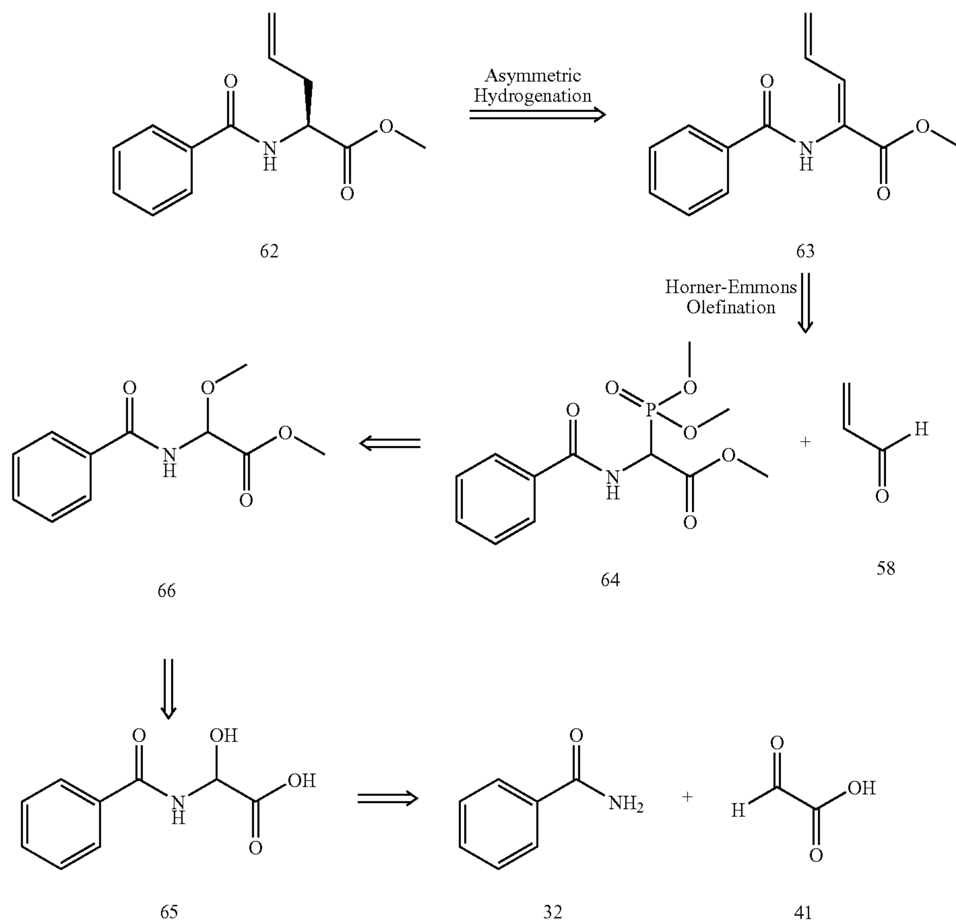
Scheme 4.11
