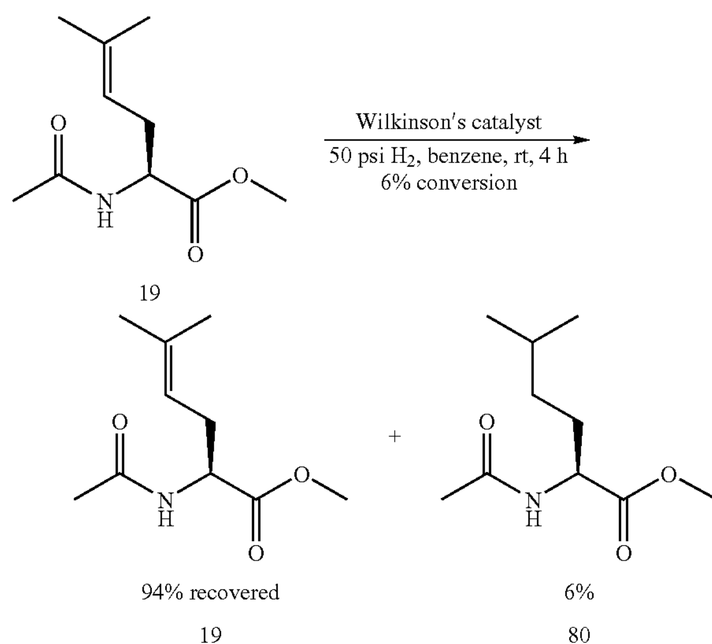
Scheme 4.31
