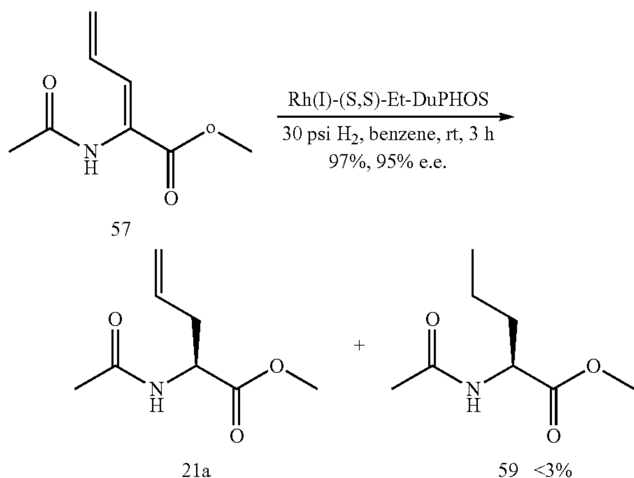
Scheme 4.5
