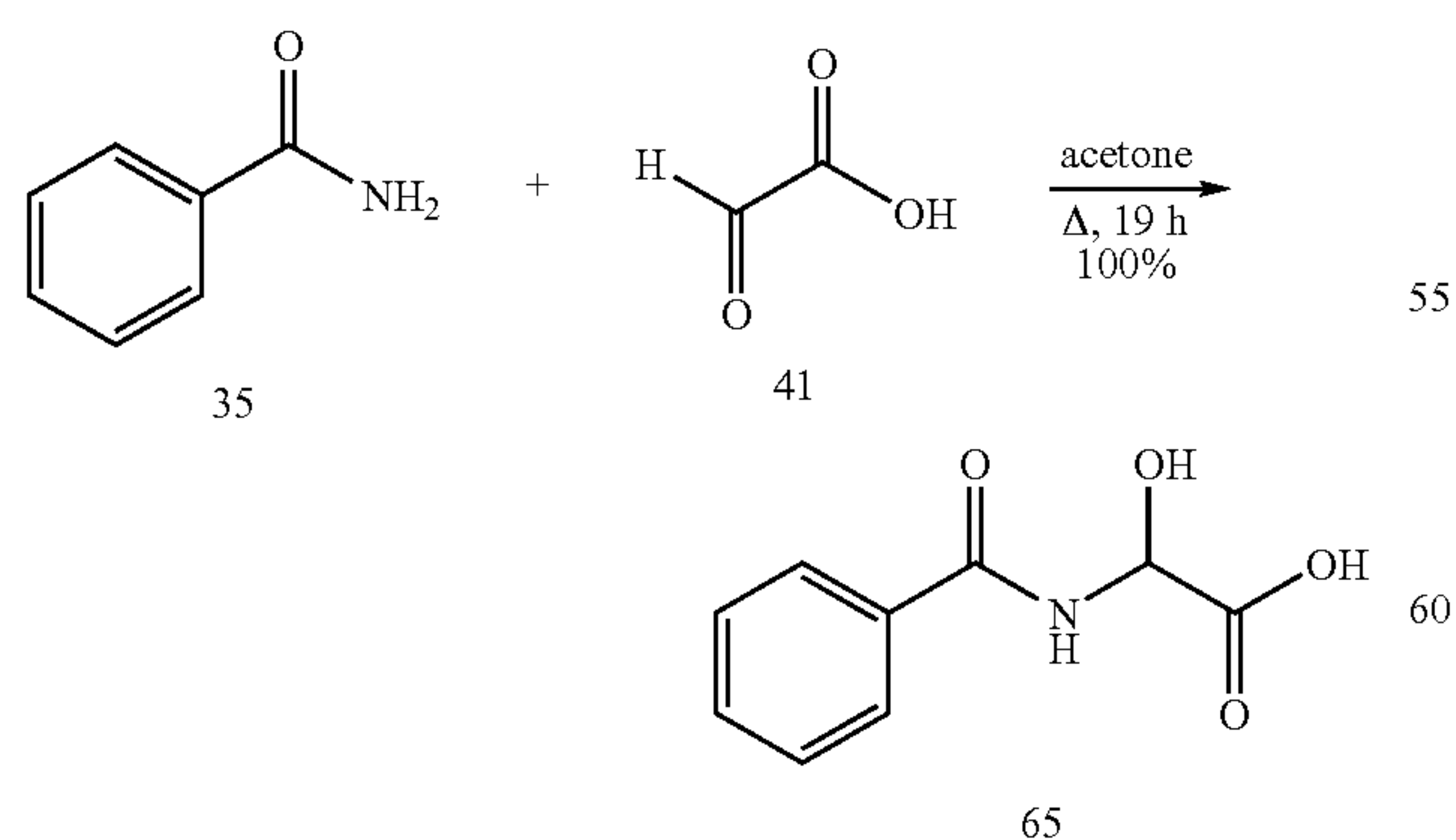
Scheme 4.12
