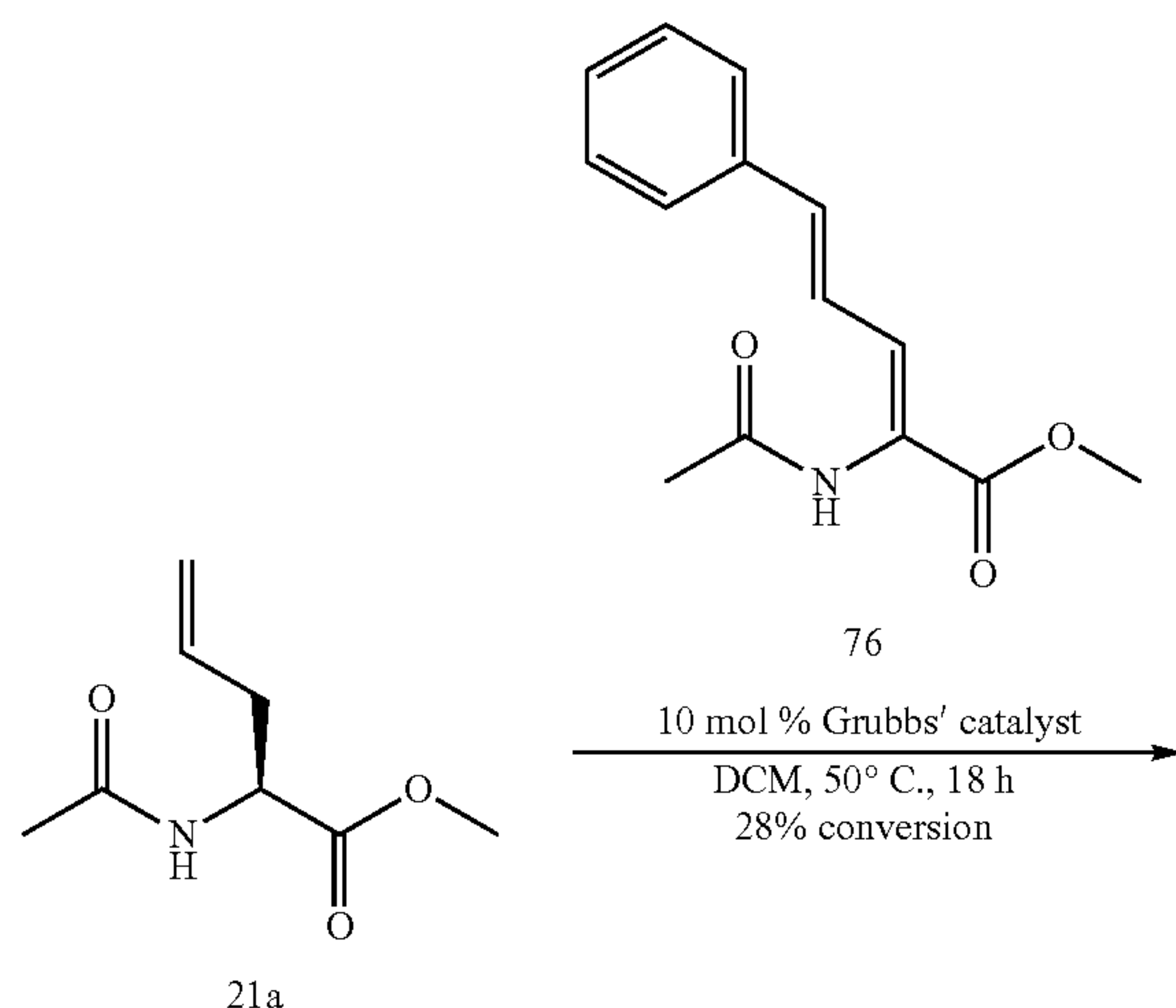
Scheme 4.24
