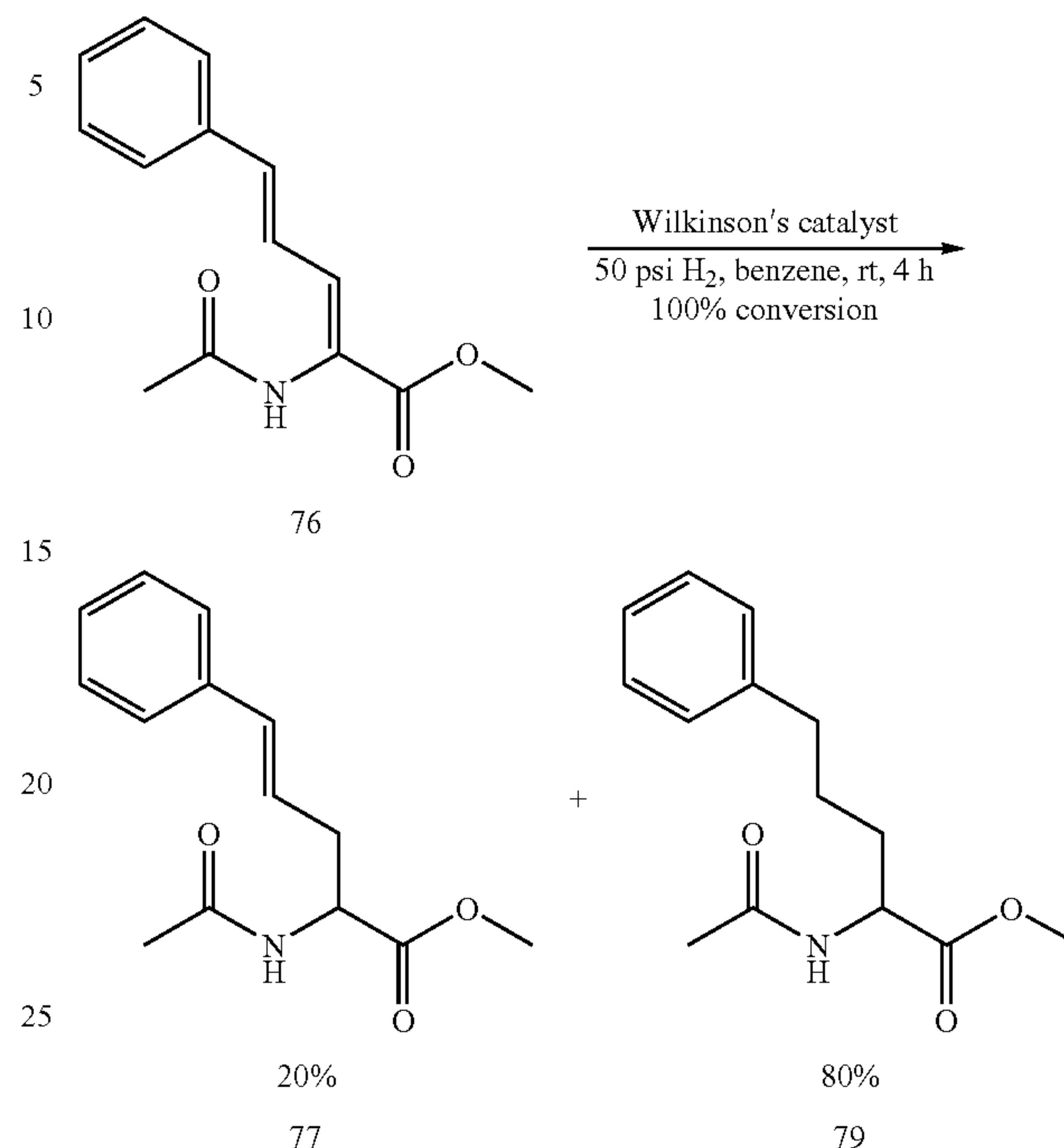
Scheme 4.28
