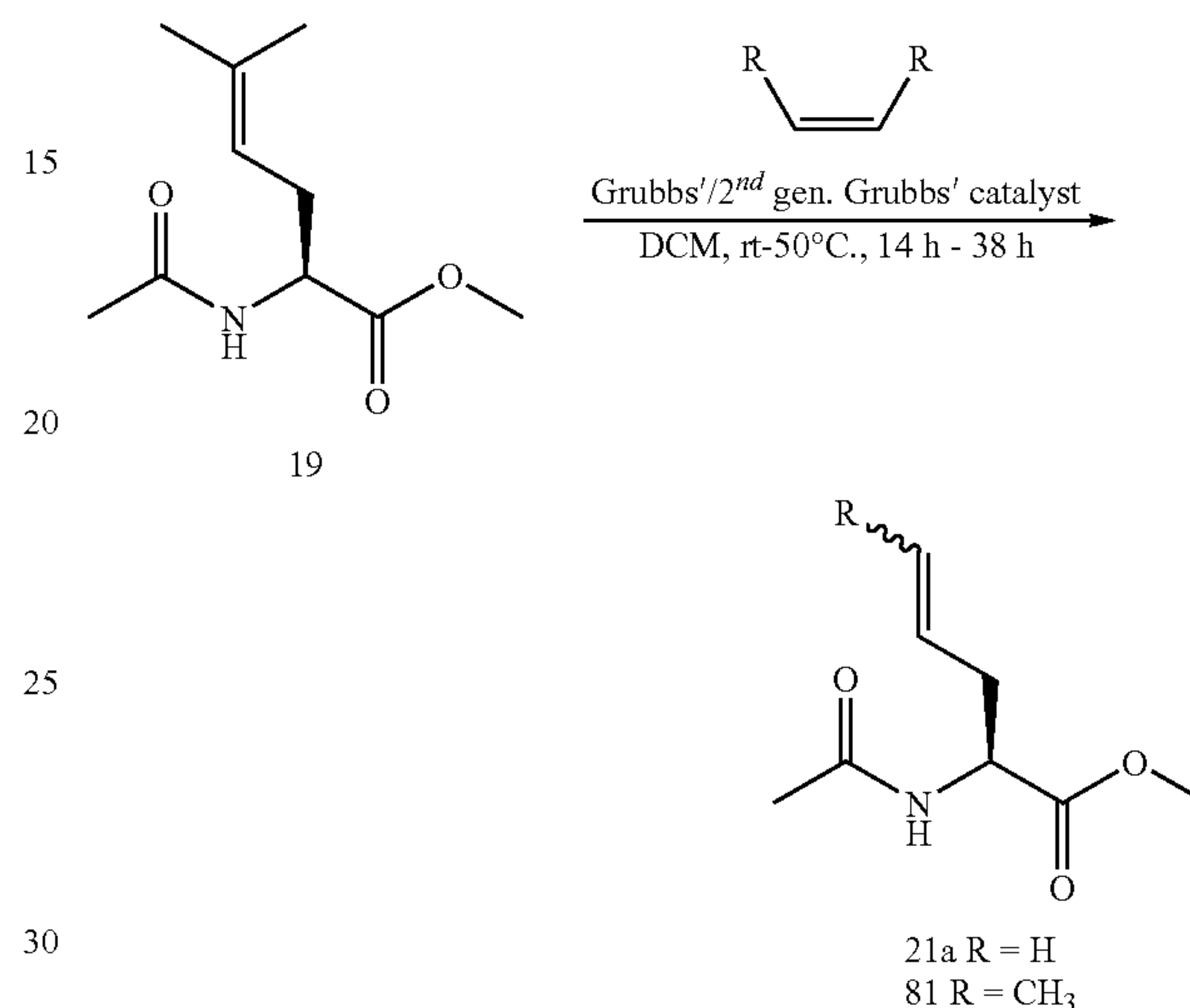
Scheme 4.33
