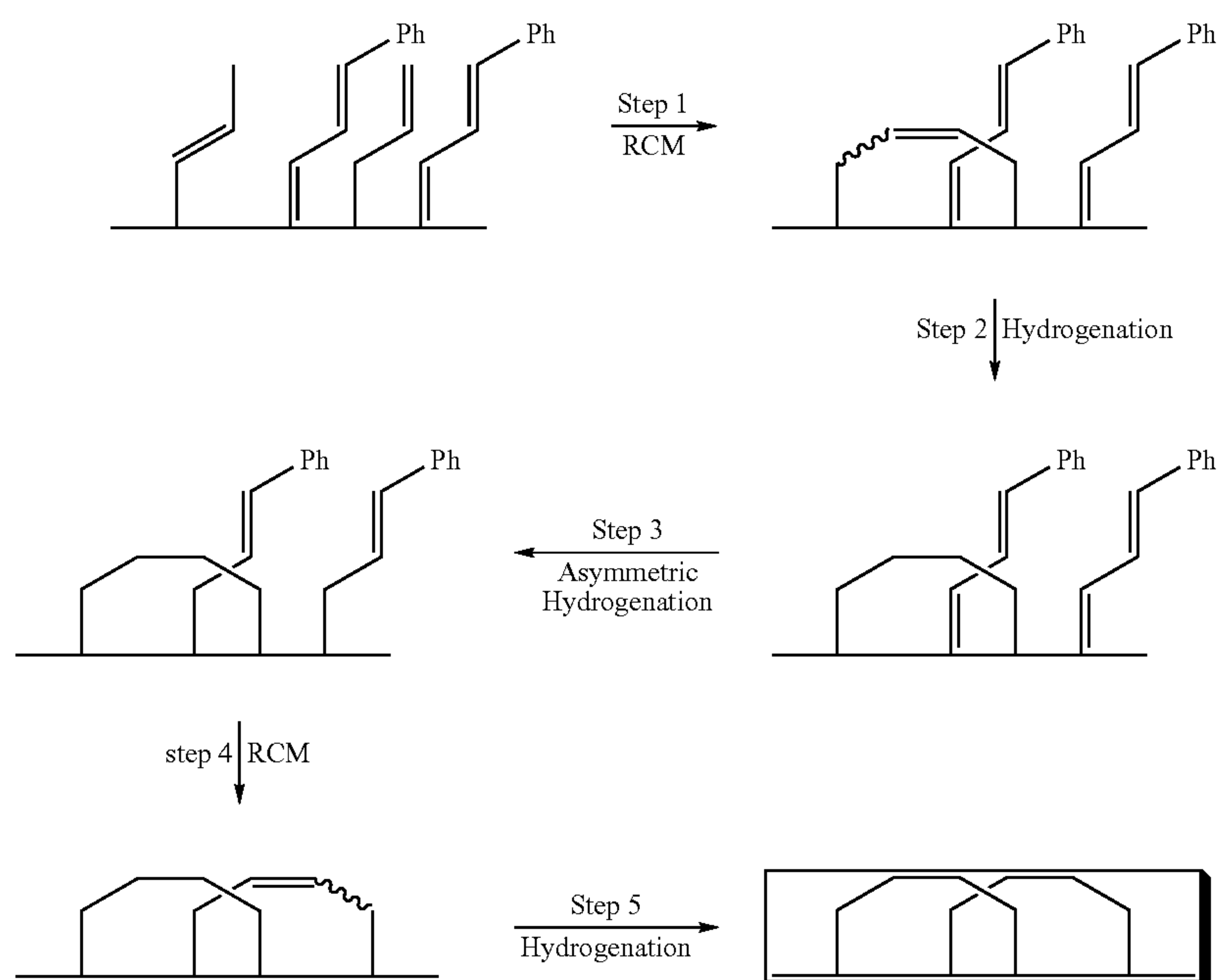
Scheme 4.27
