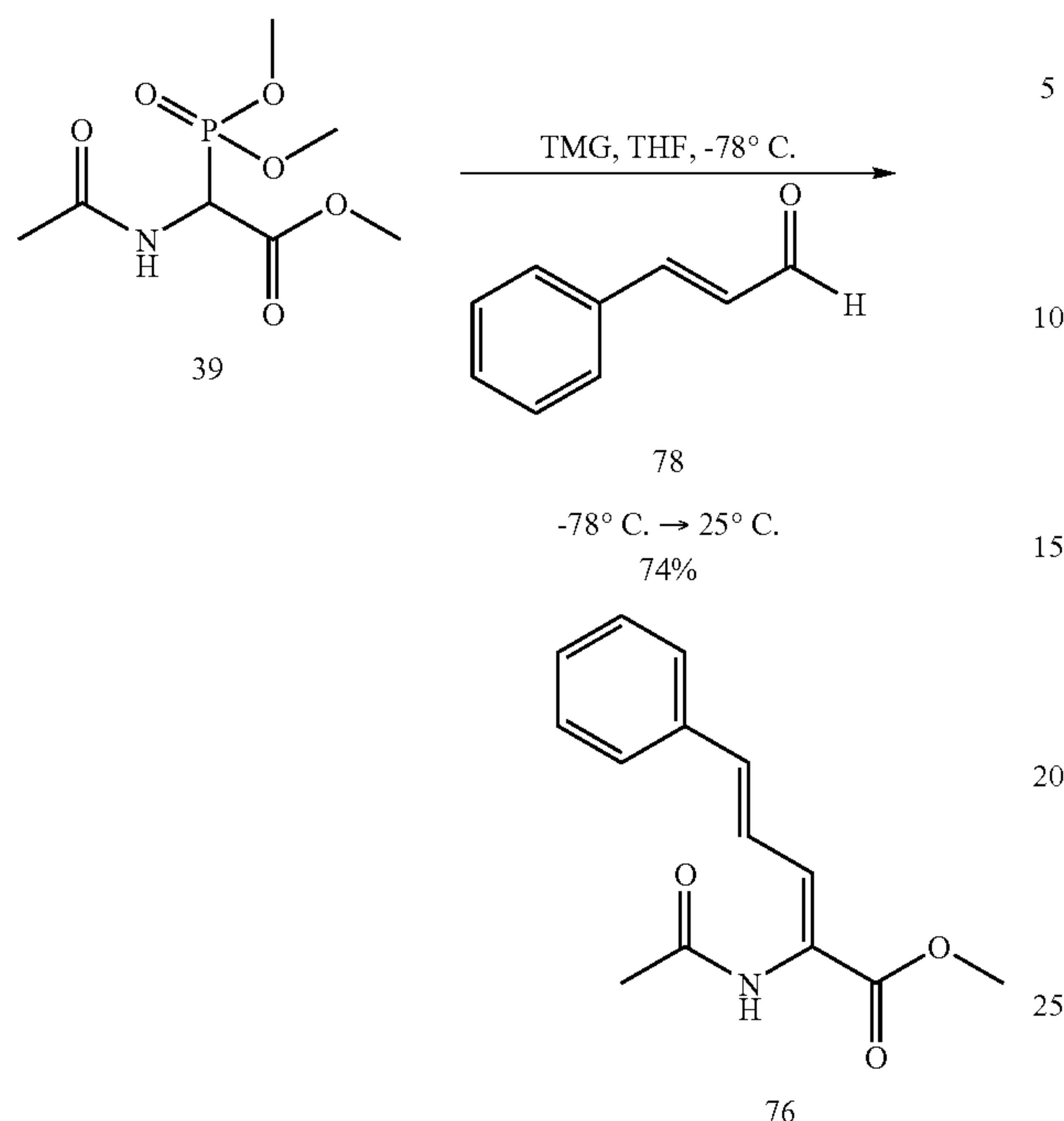
Scheme 4.23
