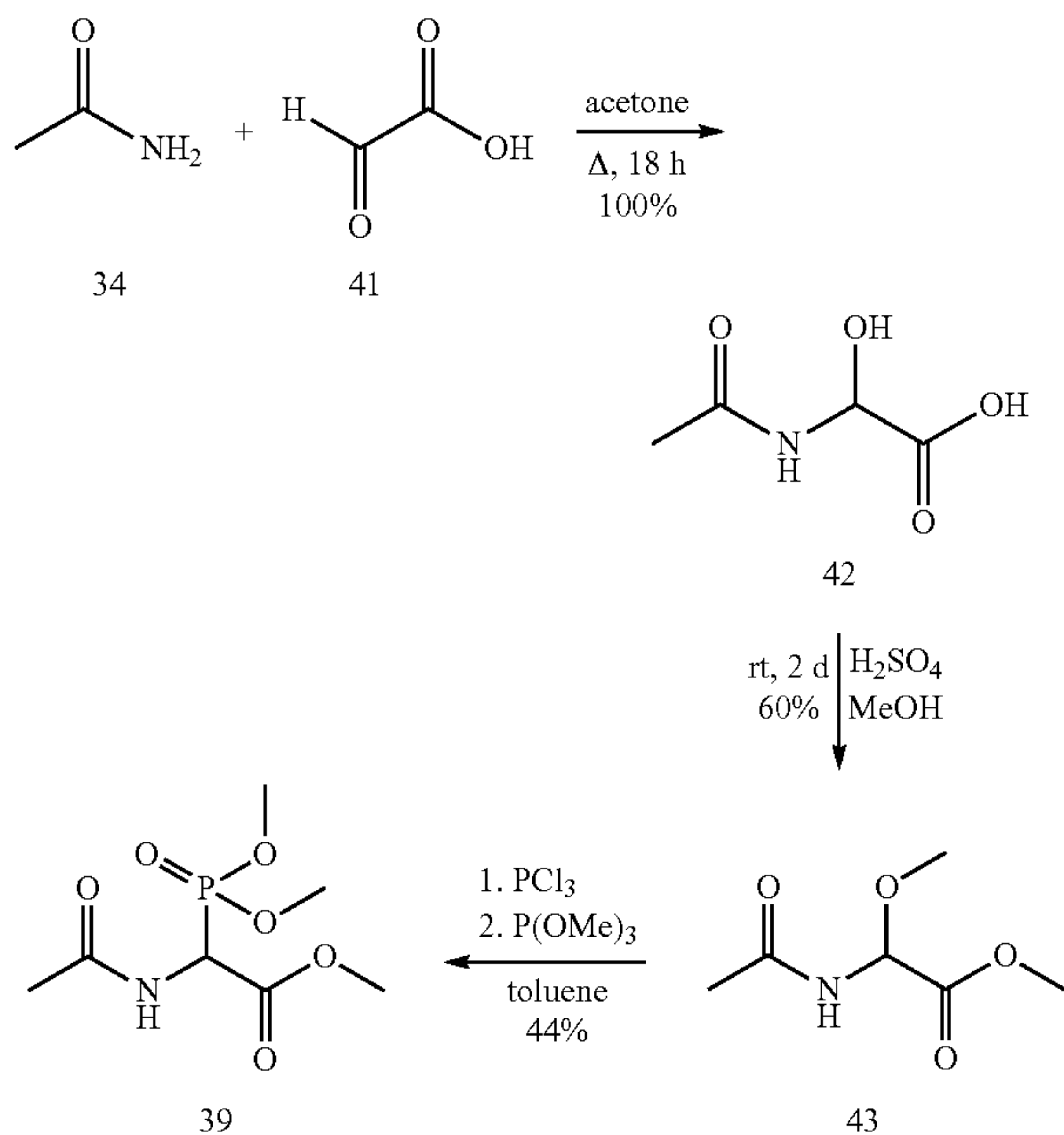
Scheme 4.3
