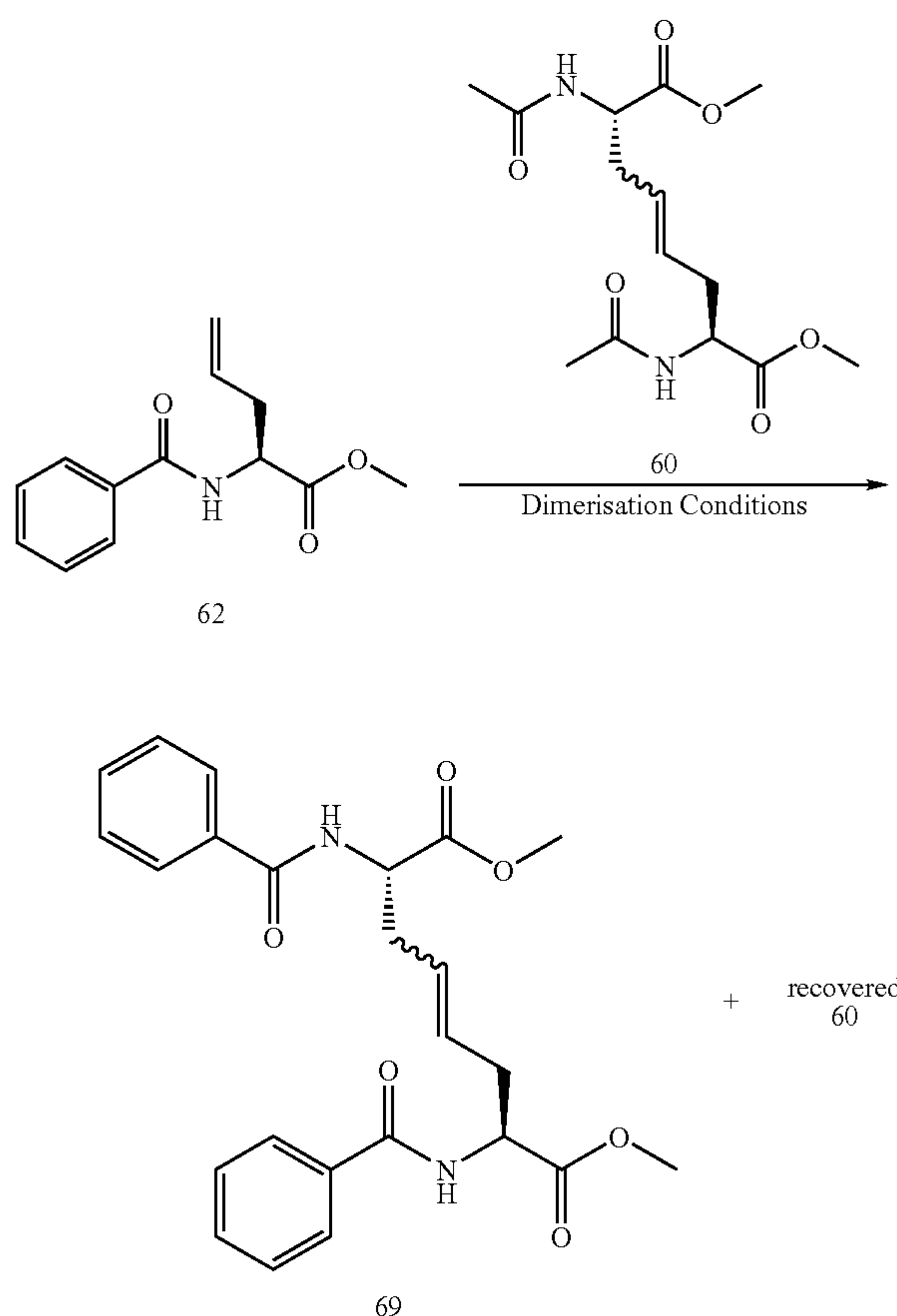
Scheme 4.10
