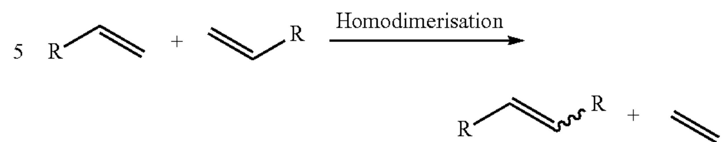
Scheme 4.6
