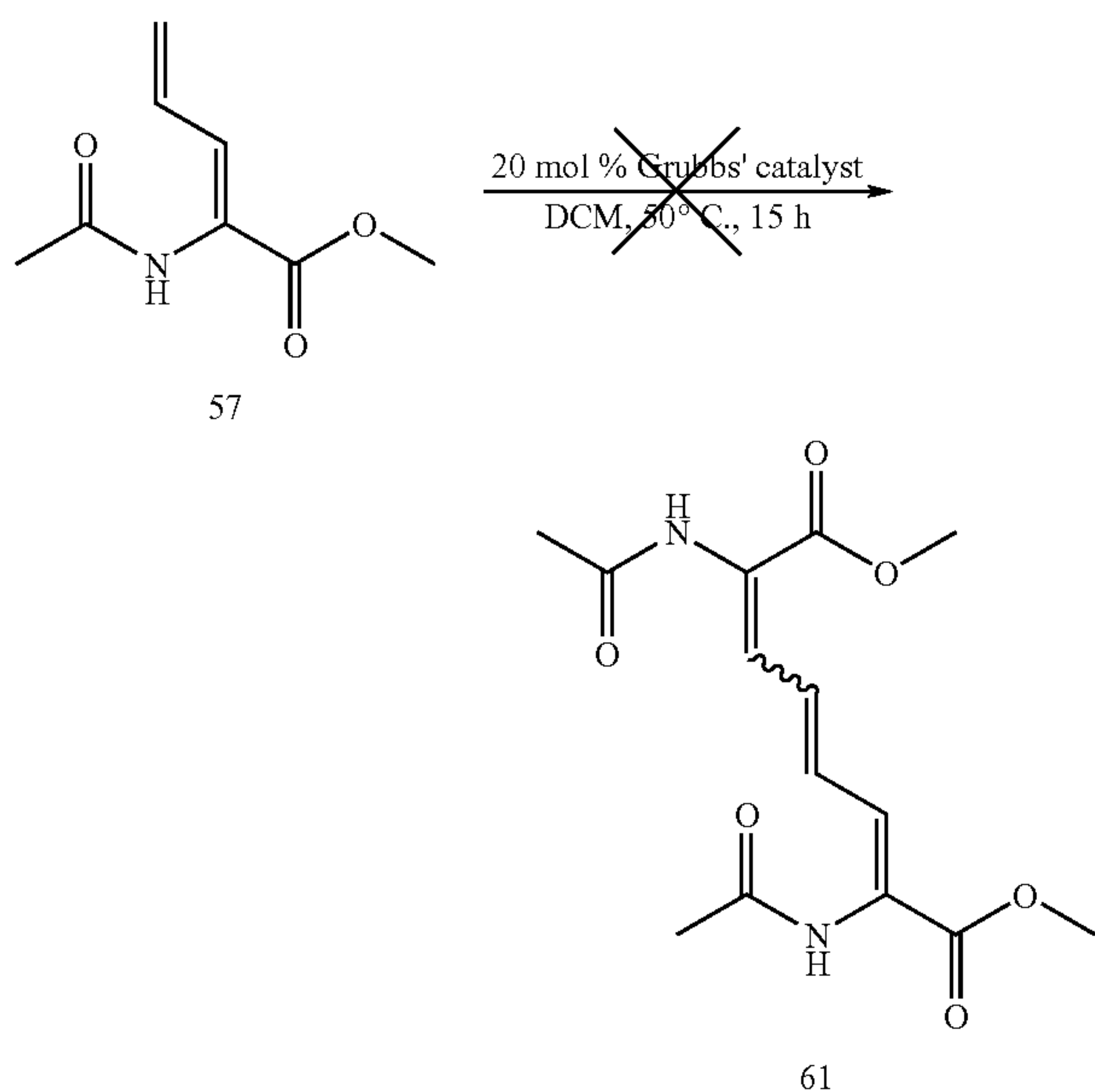
Scheme 4.9
