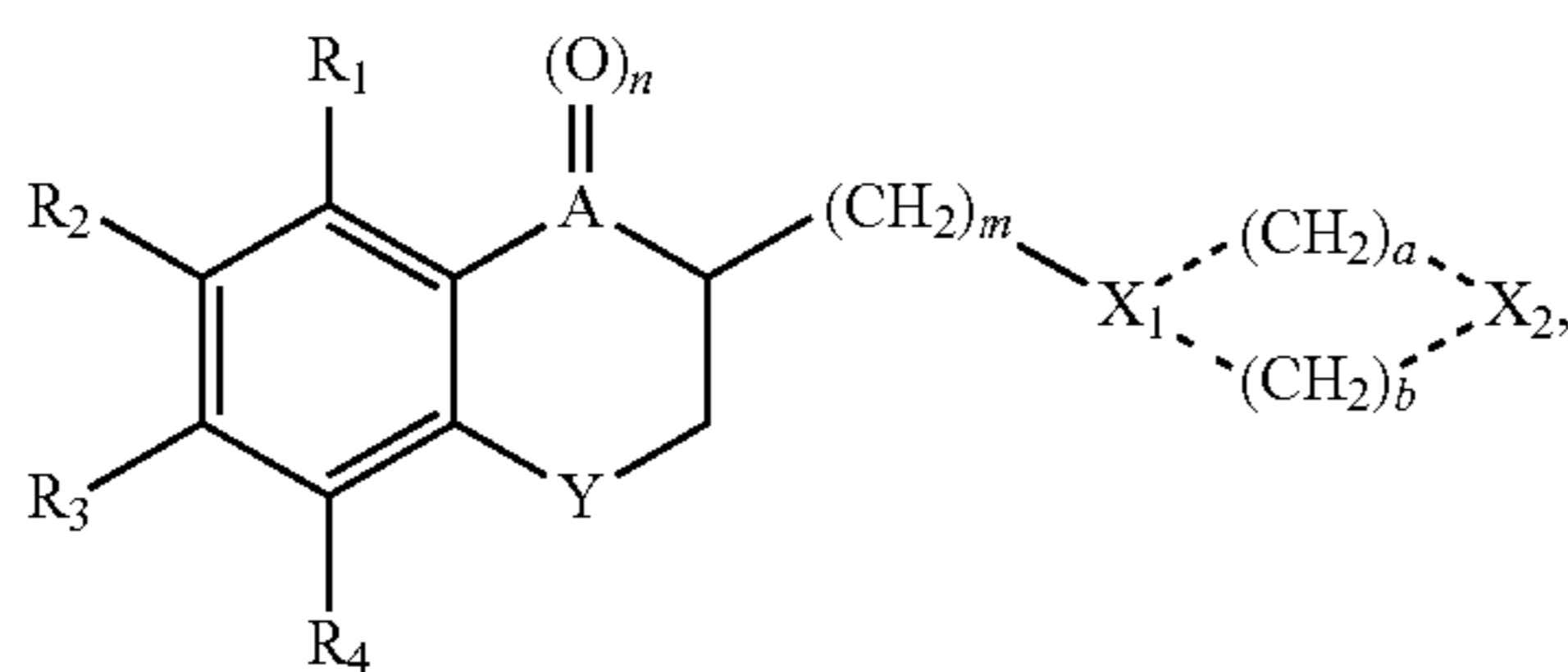
Formula VIIa
