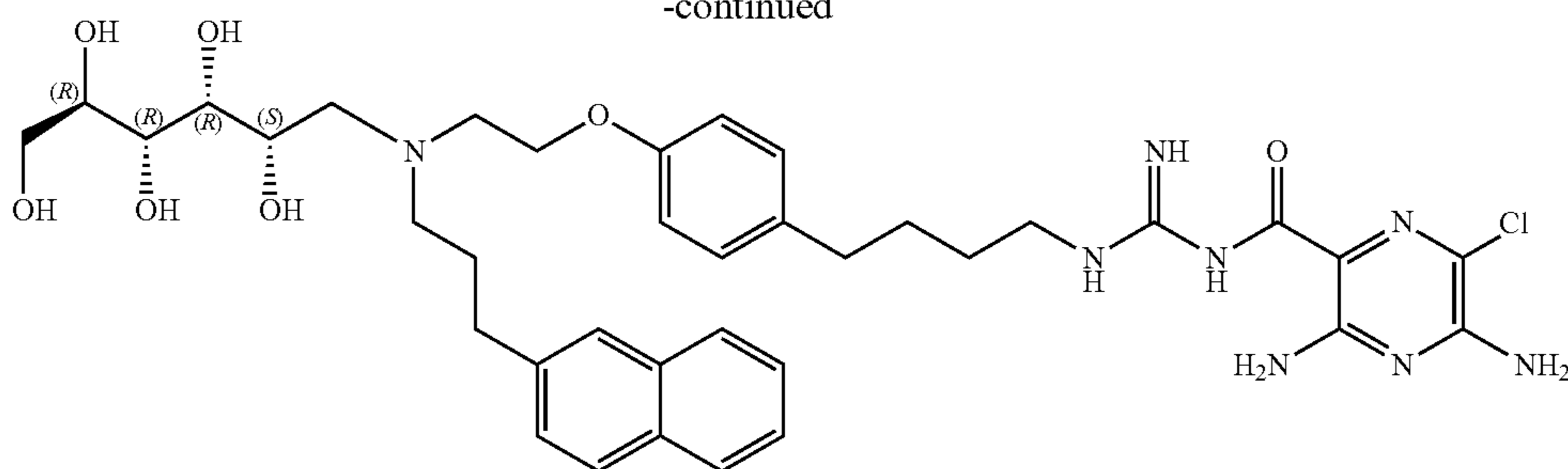
Compound 17
