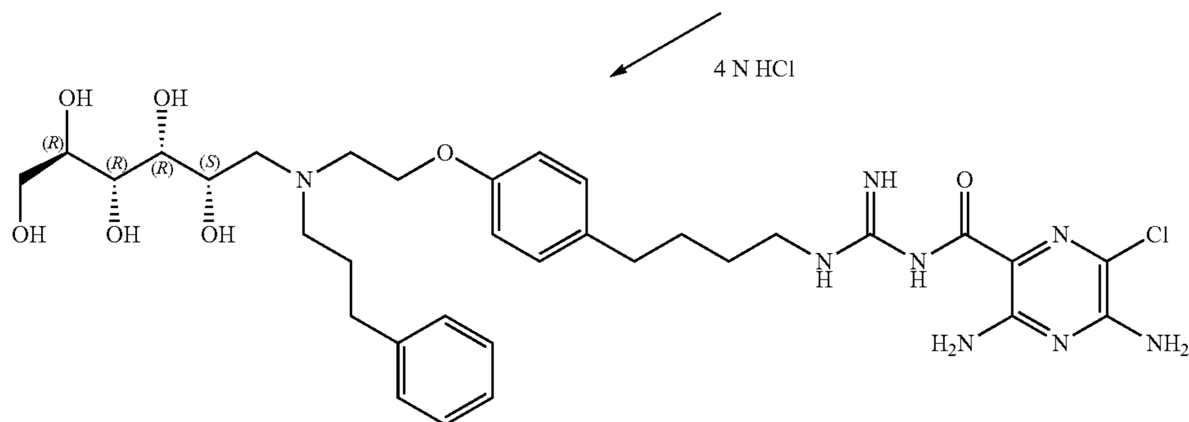
Compound 12
