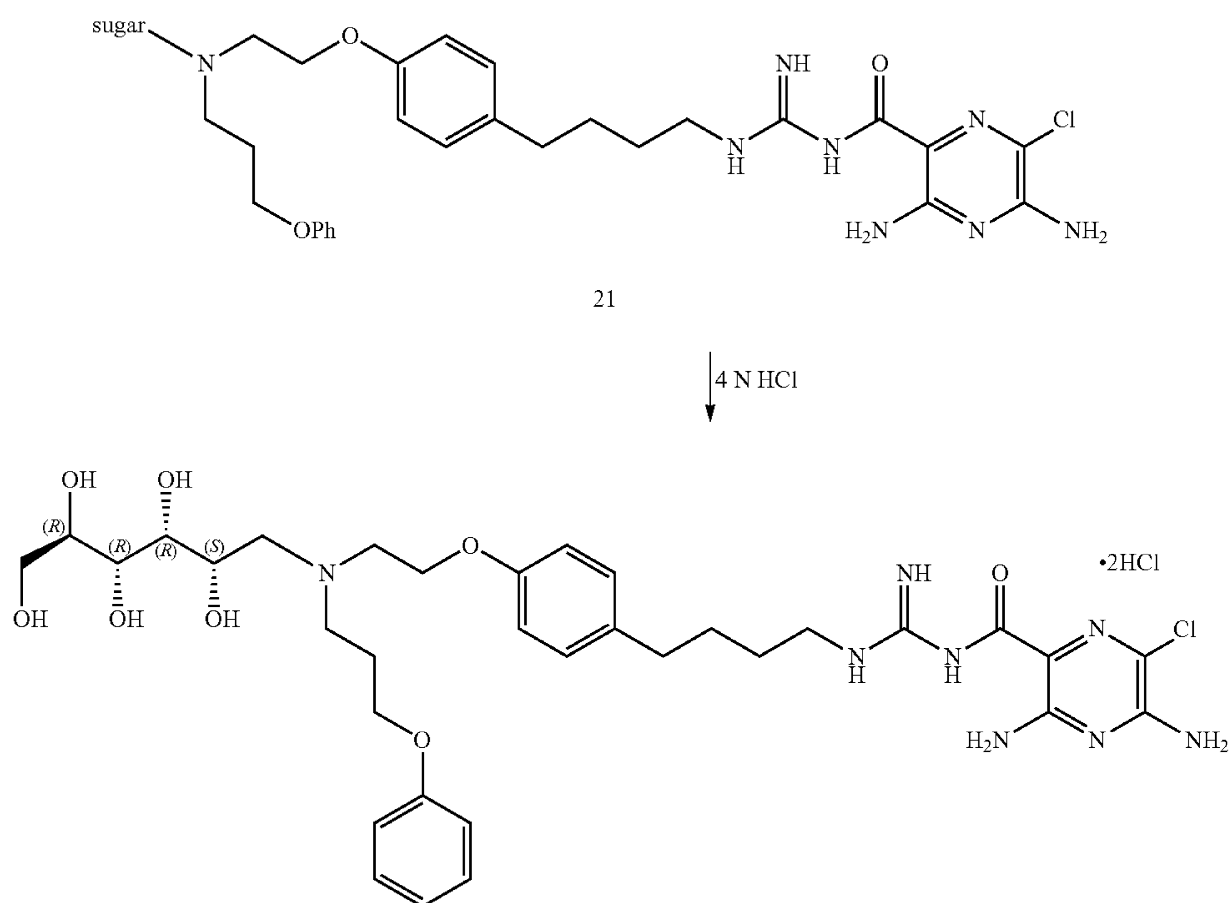
Compound 22
