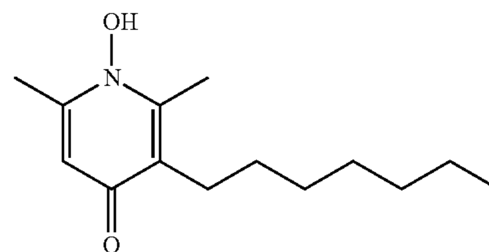
3-heptyl-1-hydroxy-2,6-dimethylpyridin-4(1H)-one (CPD-6)
