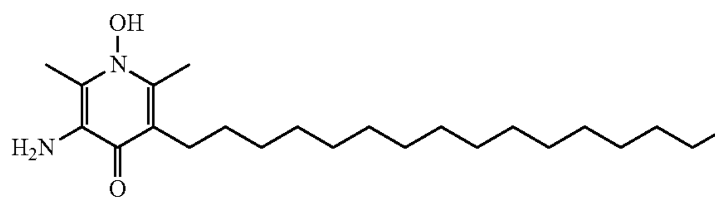
3-amino-5-hexadecyl-1-hydroxy-2,6-dimethylpyridin-4(1H)-one (CPD-4)
