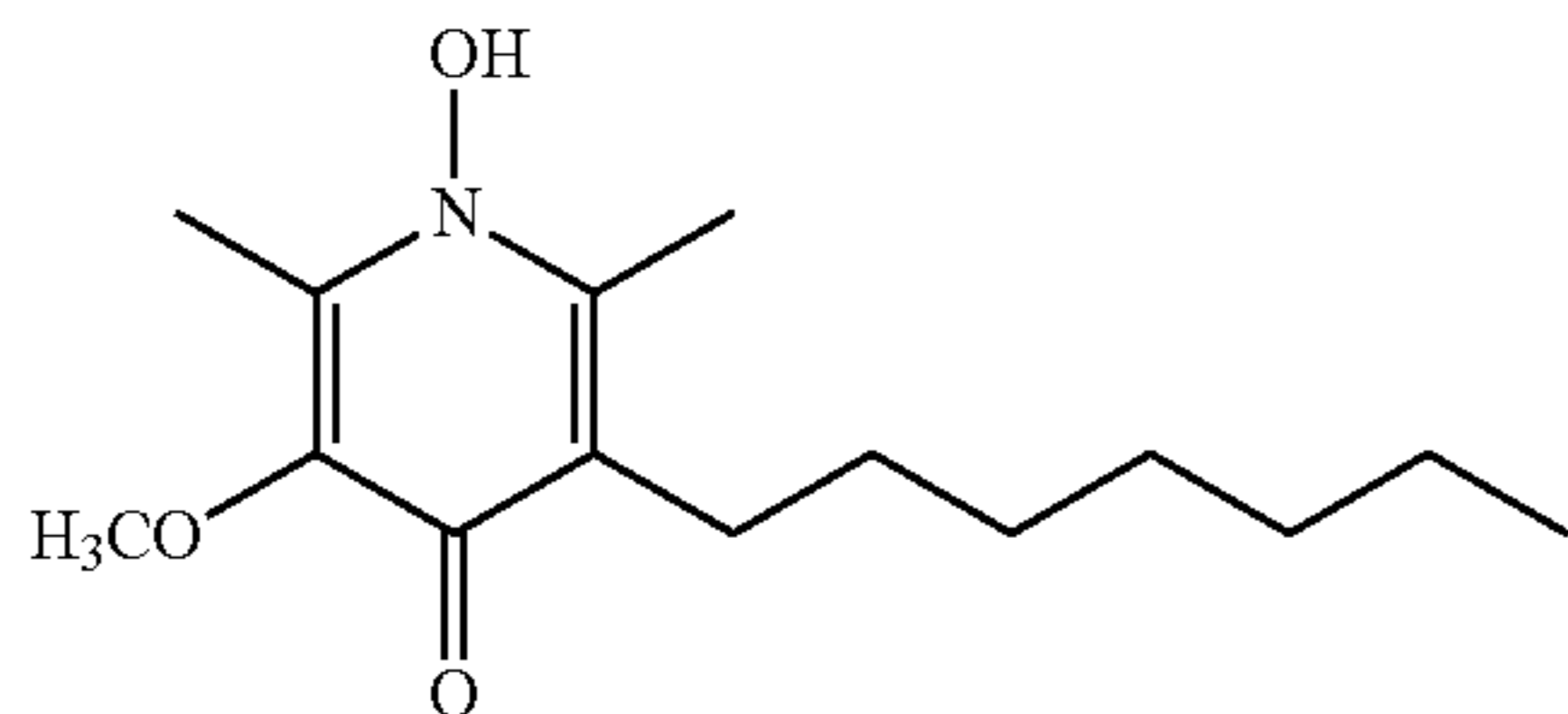
3-heptyl-1-hydroxy-5-methoxy-2,6-dimethylpyridin-4(1H)-one (CPD-5)
