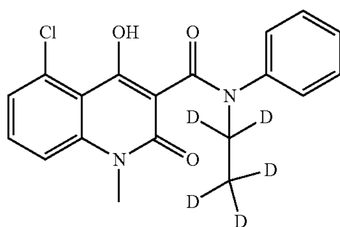
Compound 2
