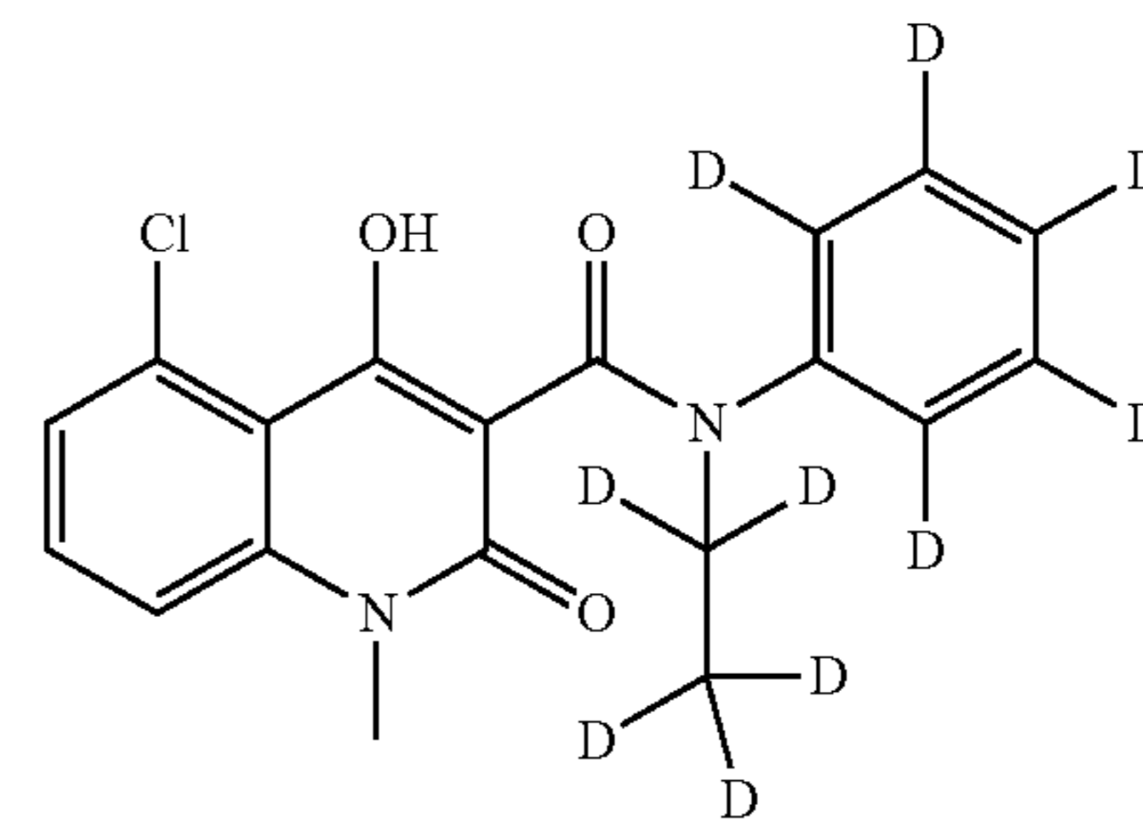
Compound 3
