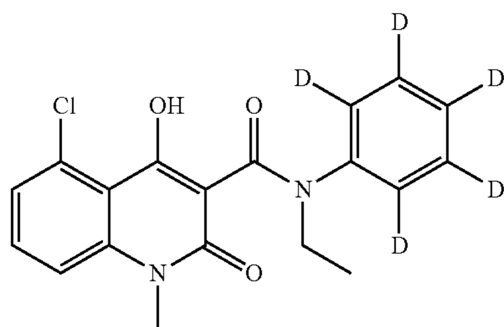
Compound 1
