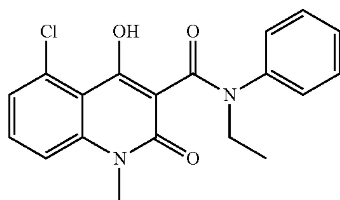
Laquinimod
