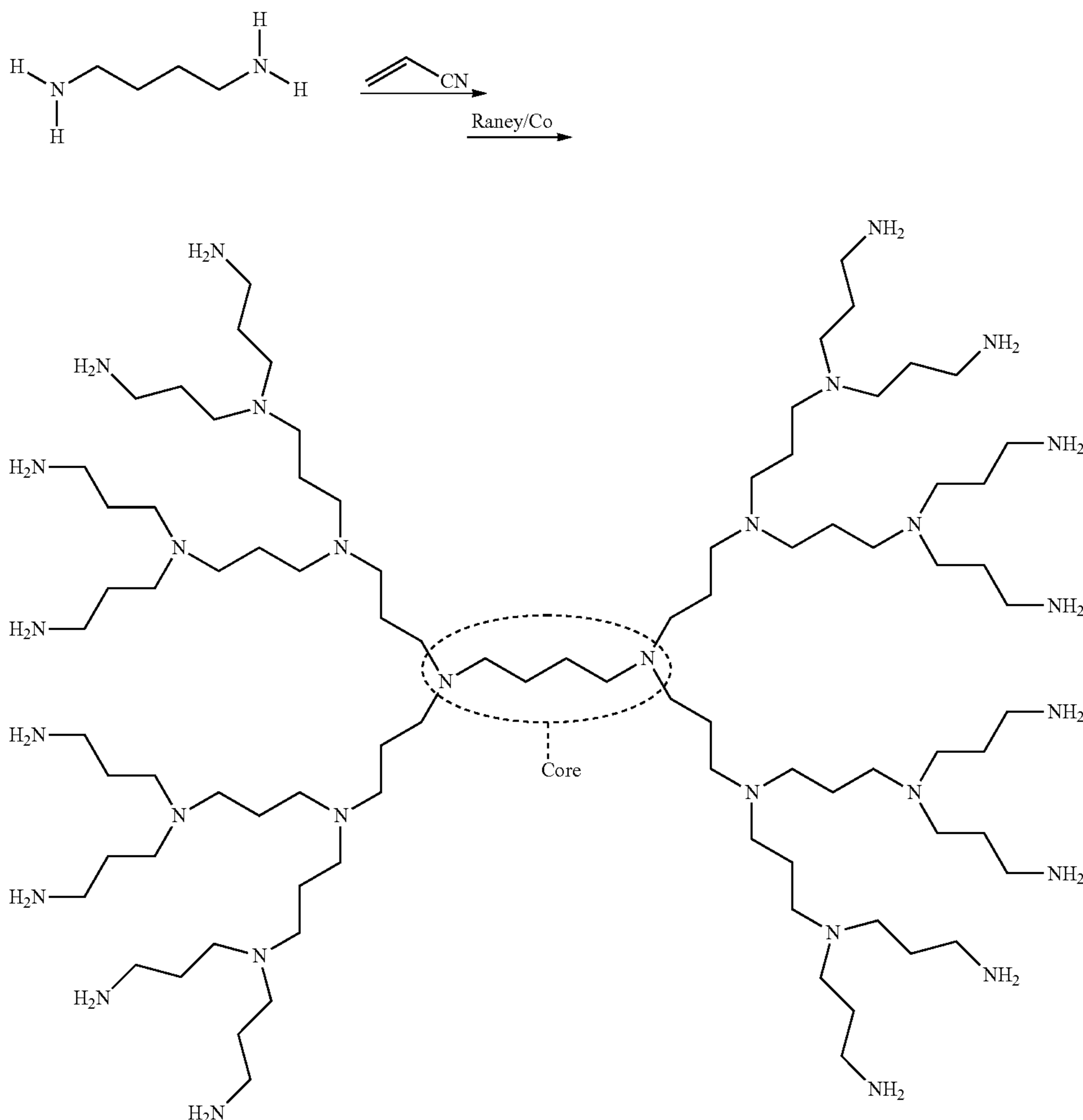
Scheme 3. Synthesis of PPI dendrimer.
