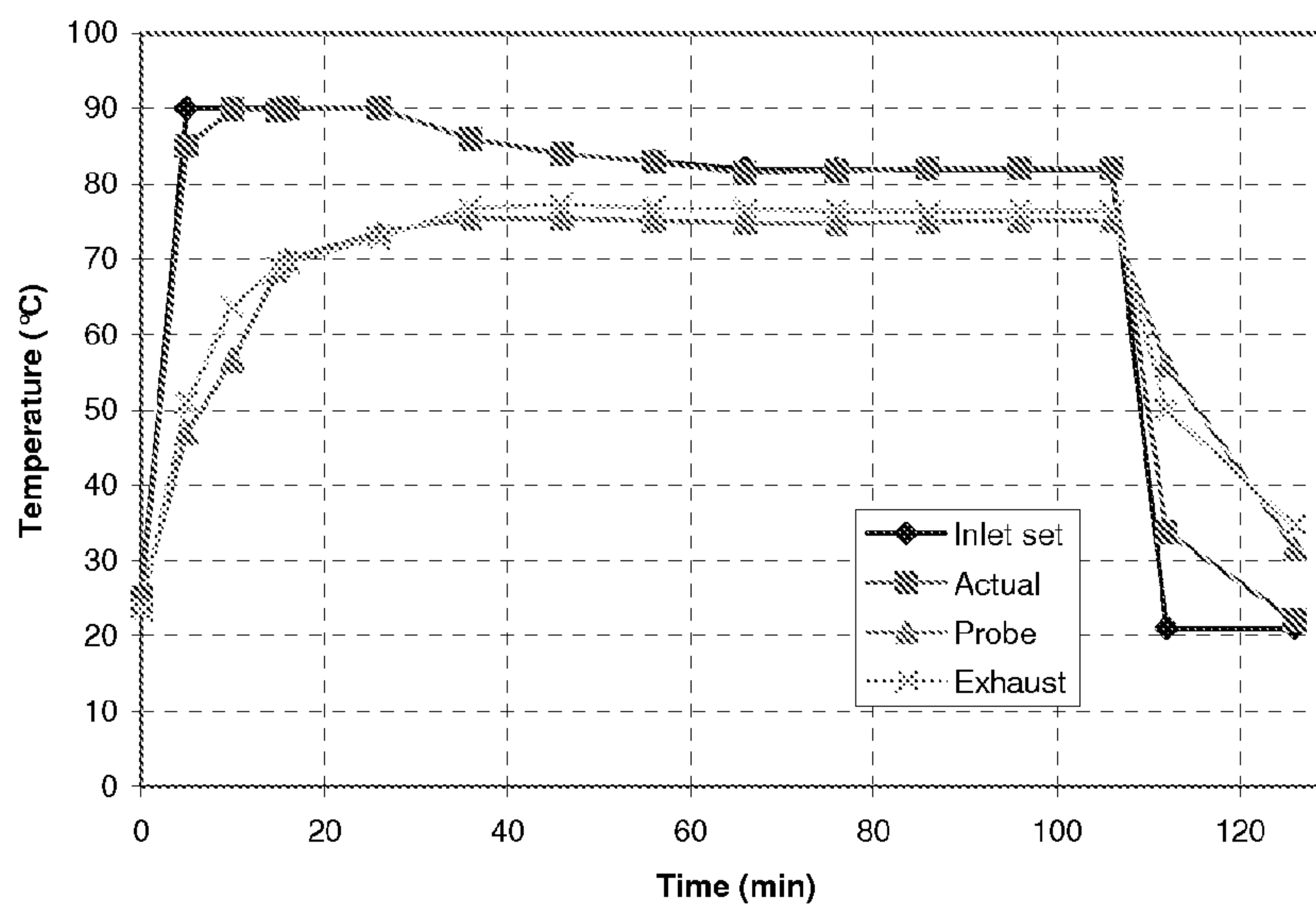
Curing of Example 13.4 Temperature Profile
