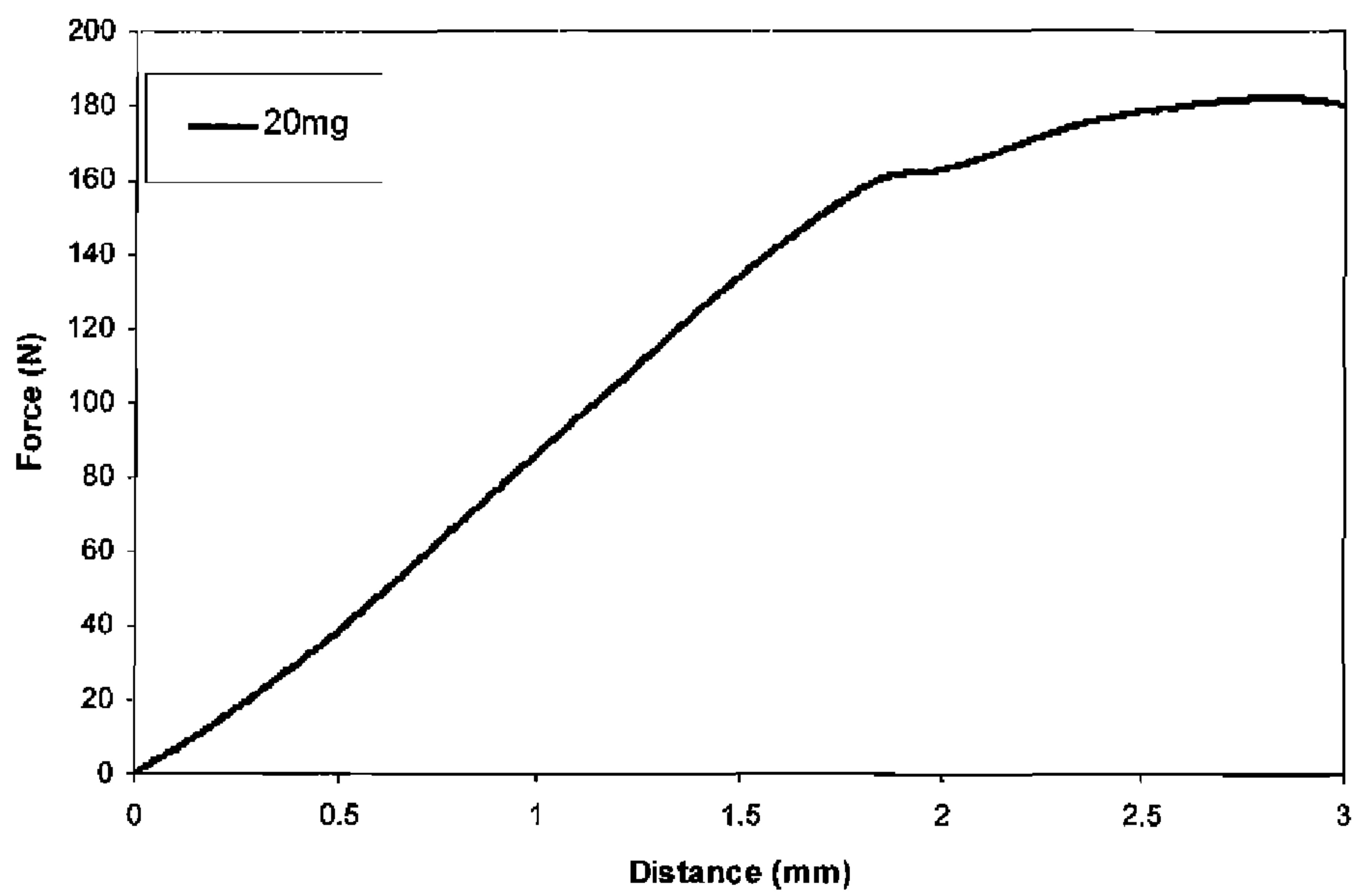
Example 20 Indentation Test of Example 14.3 tablet
