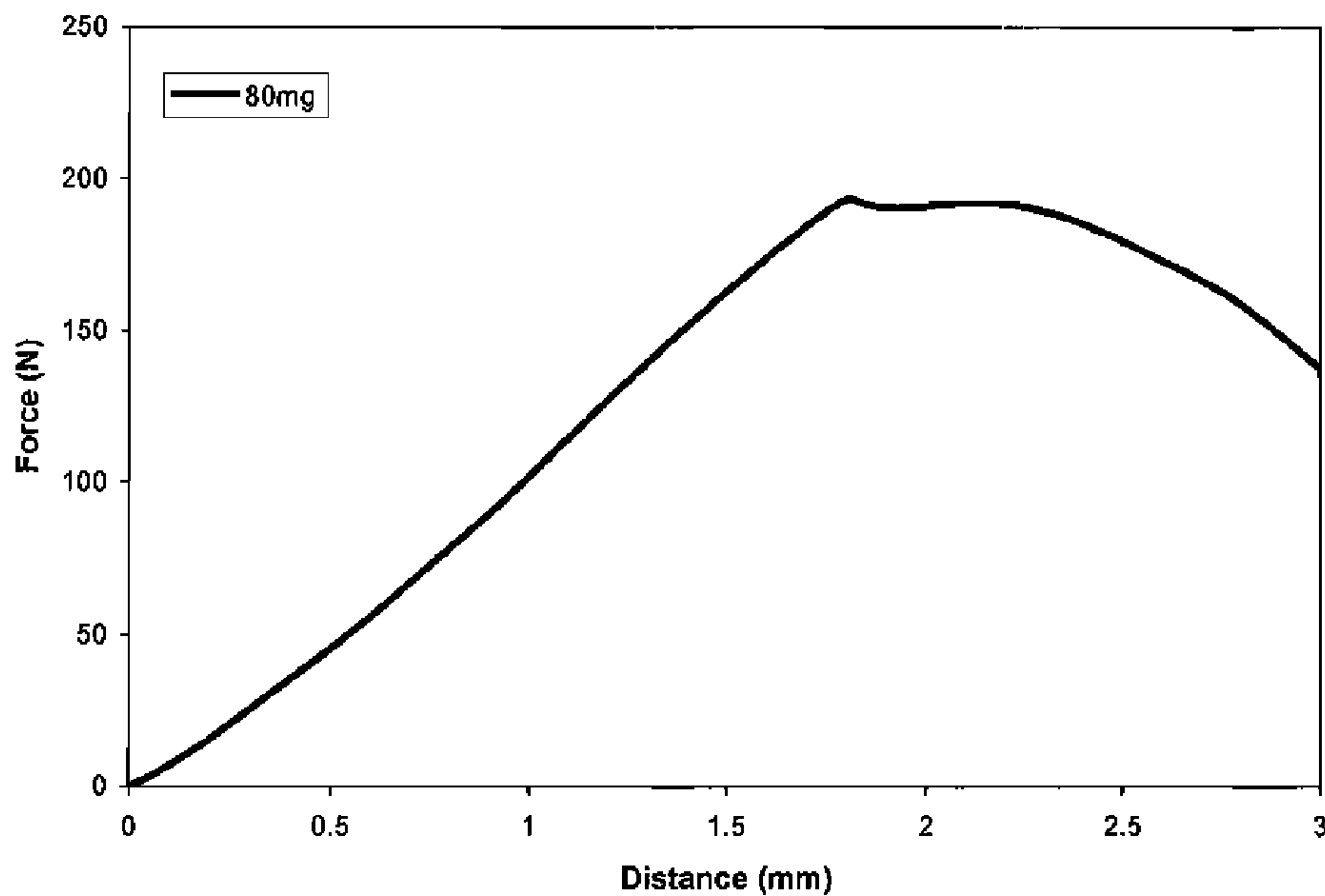
Example 20 Indentation Test of Example 18.2 tablet
