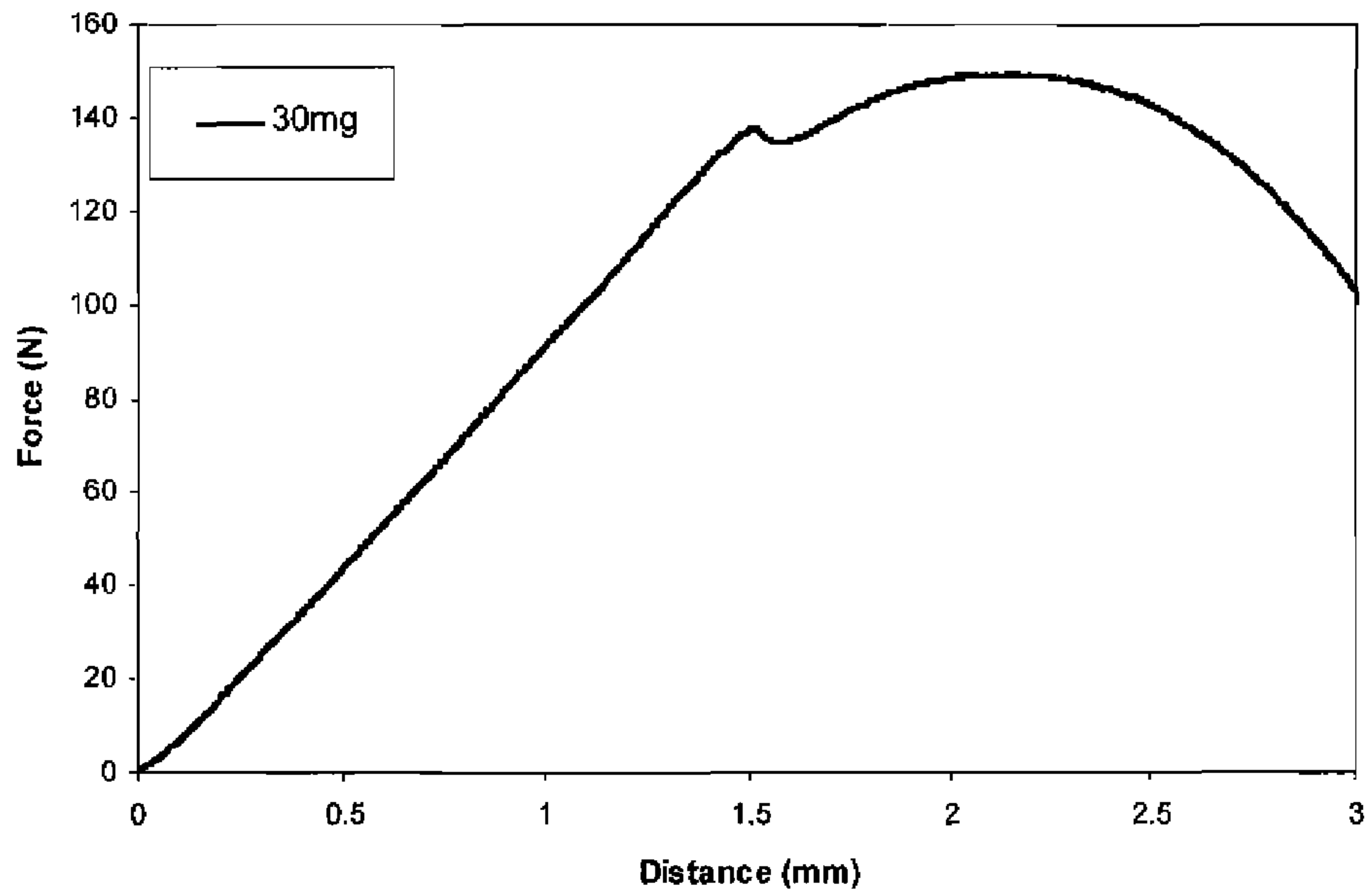
Example 20 Indentation Test of Example 14.4 tablet
