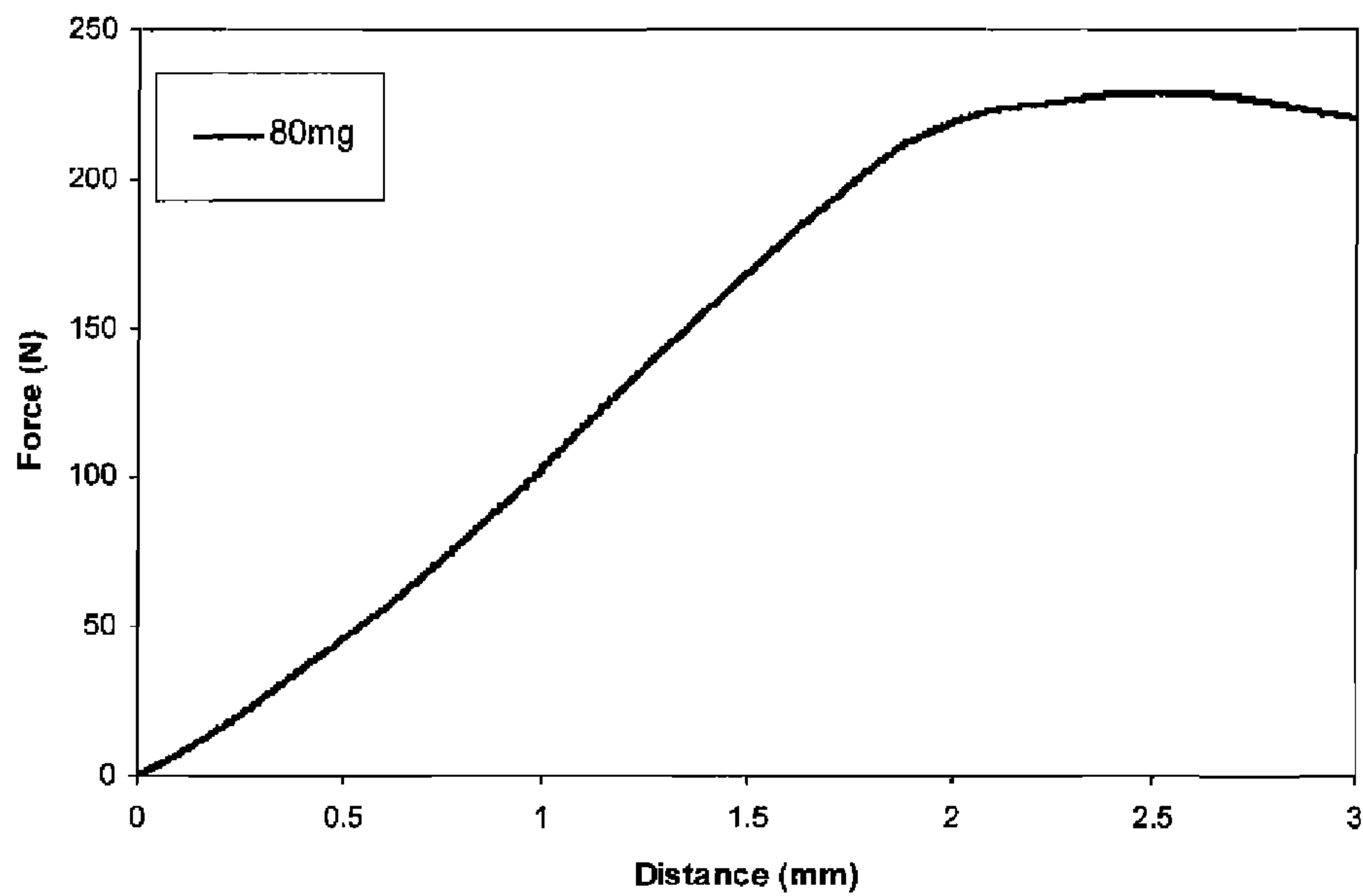
Example 20 Indentation Test of Example 16.2 tablet
