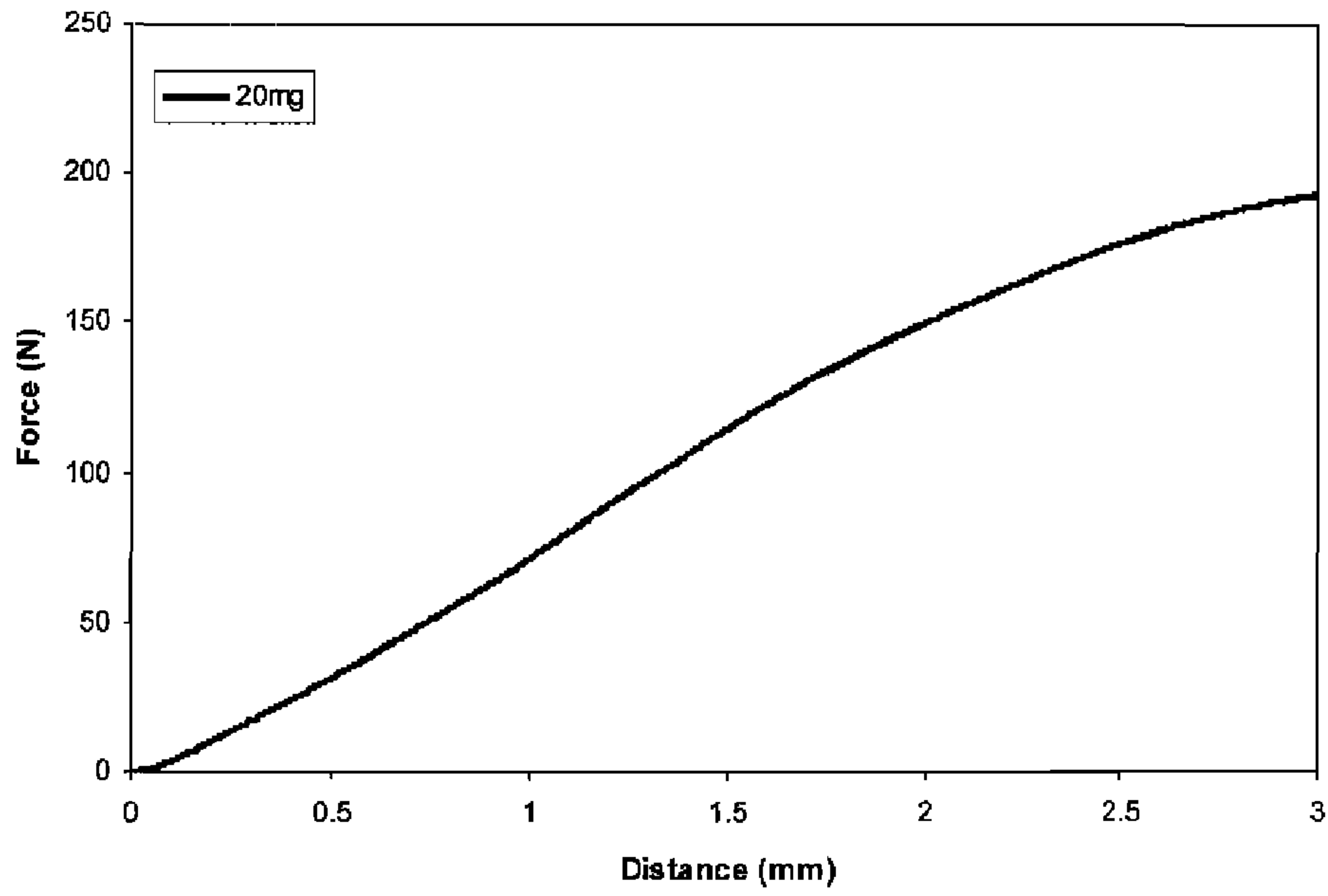
Example 20 Indentation Test of Example 13.3 tablet
