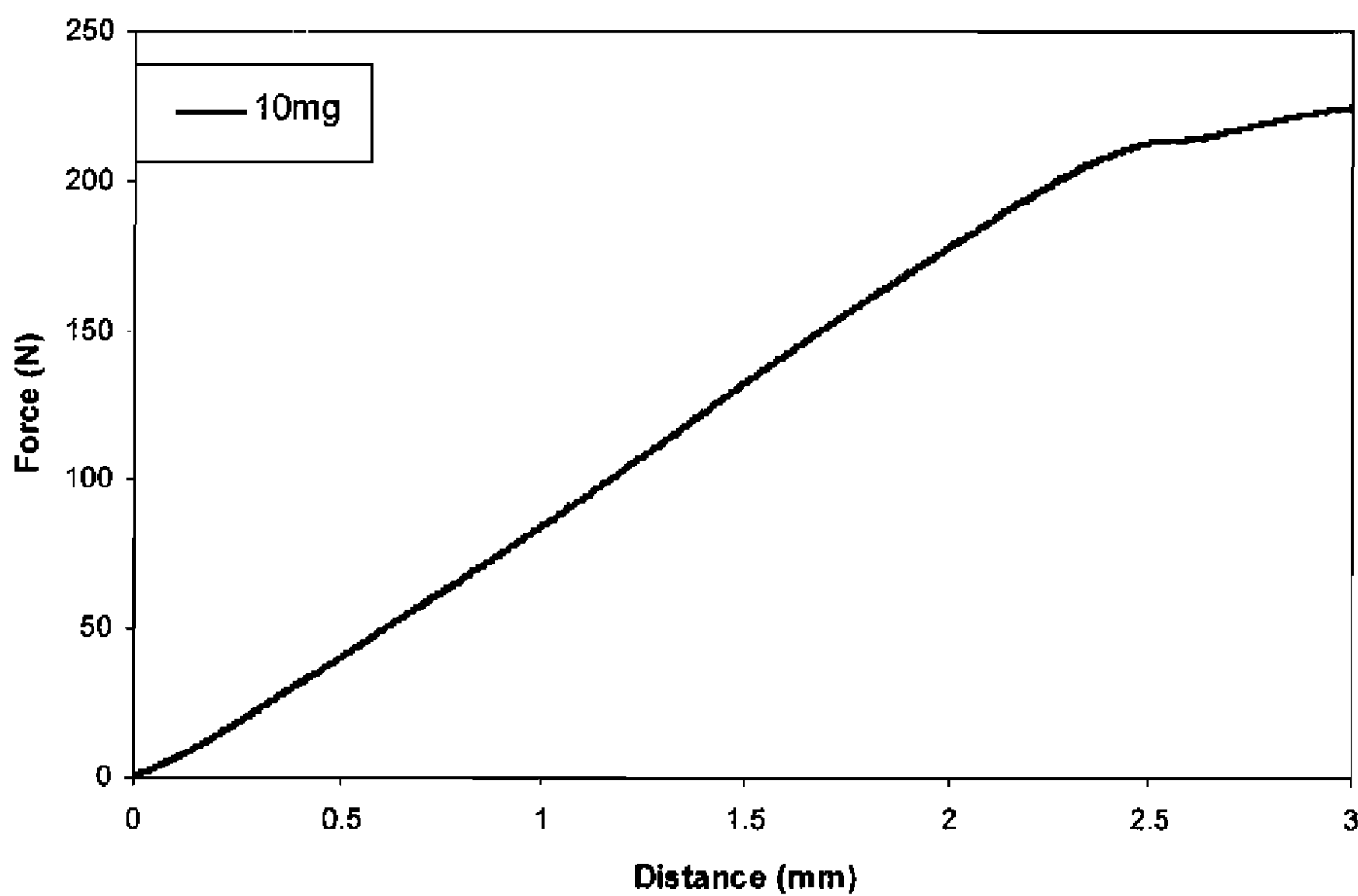
Example 20 Indentation Test of Example 14.1 tablet
