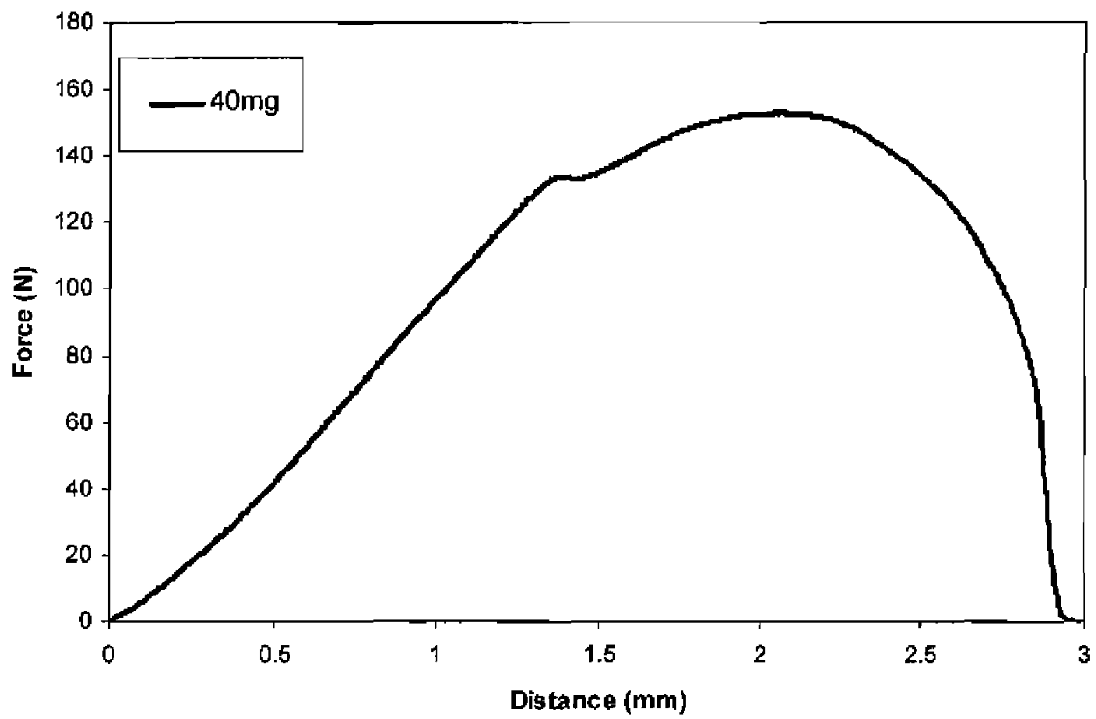
Example 20 Indentation Test of Example 14.5 tablet
