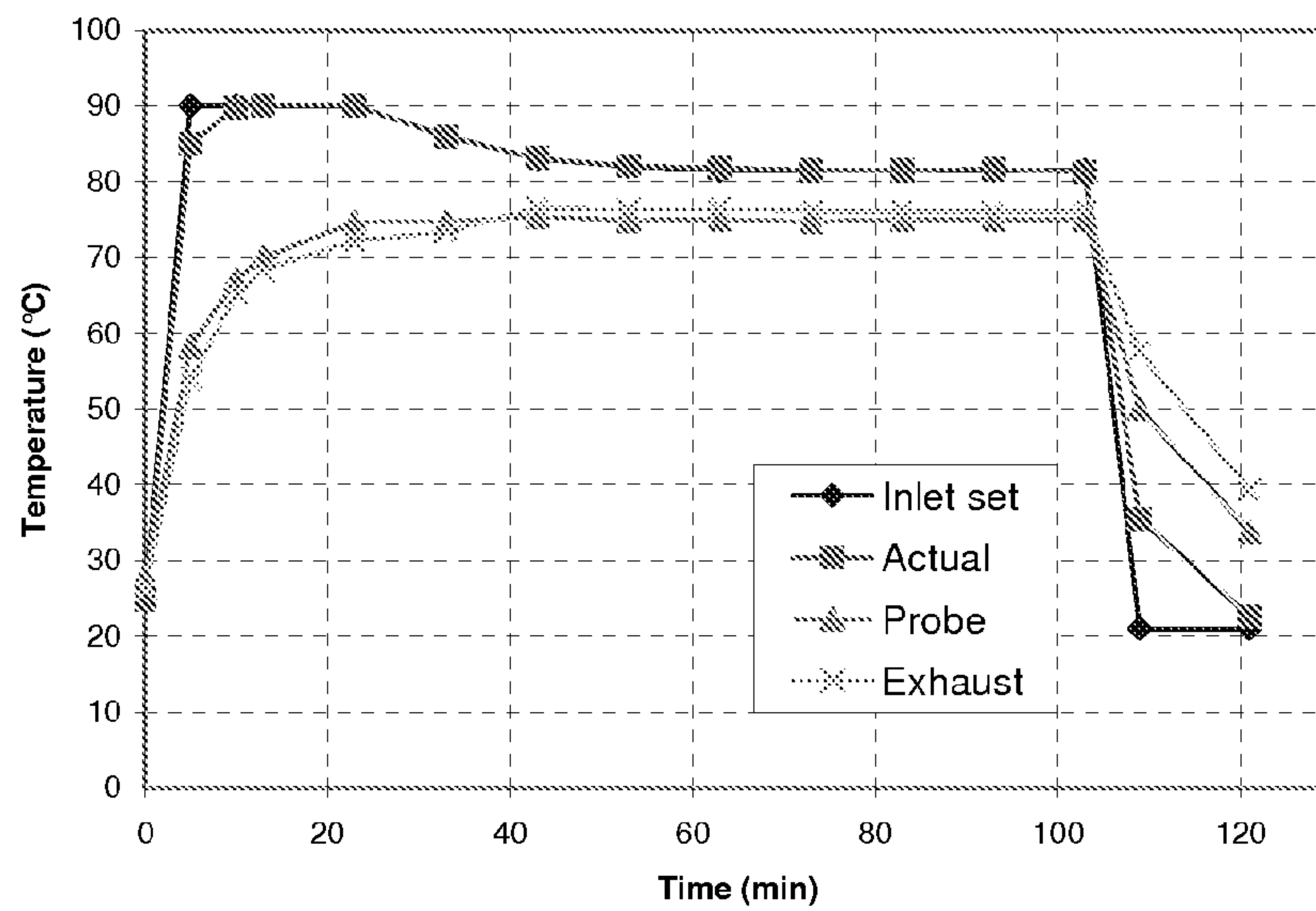
Curing of Example 13.3 Temperature Profile
