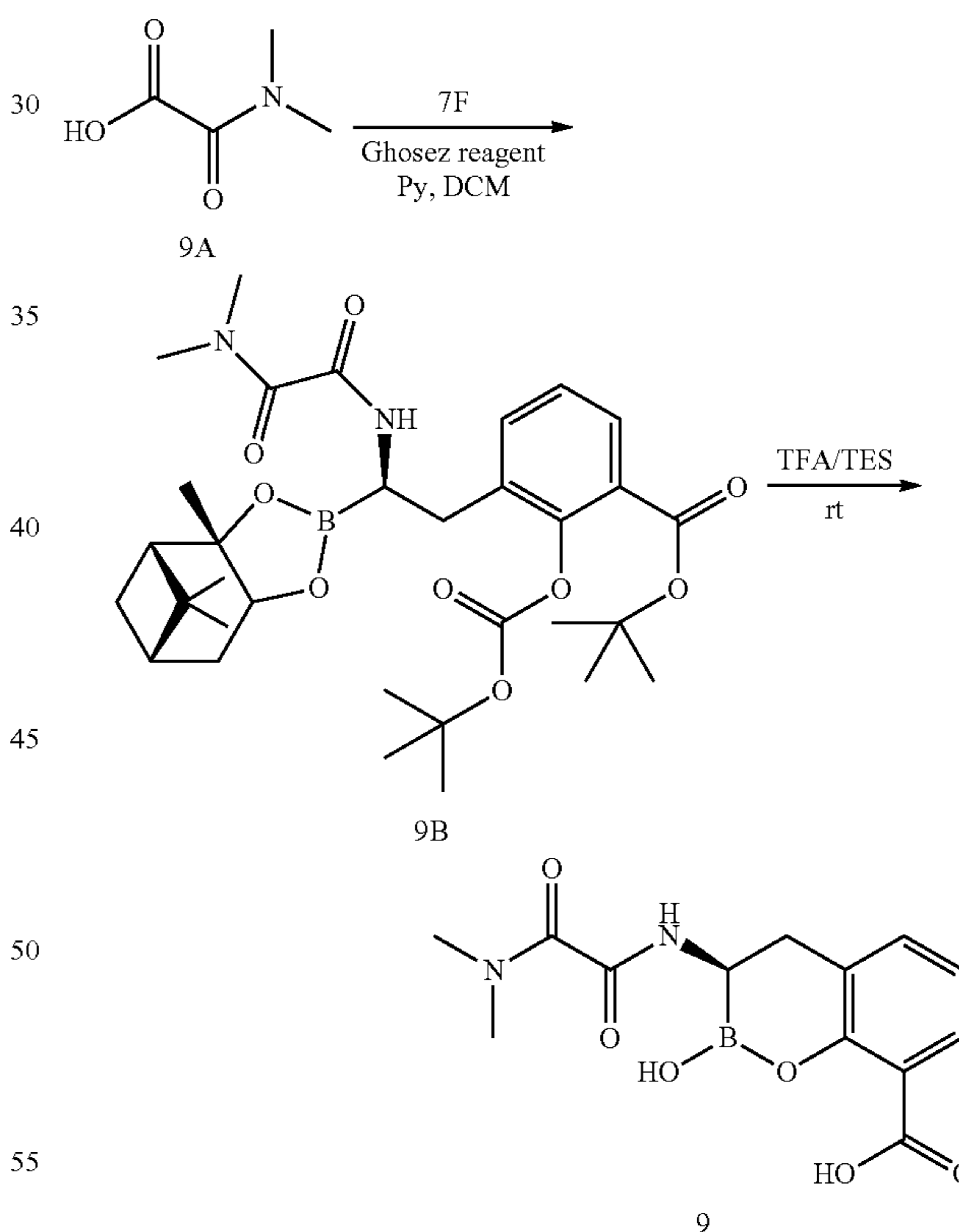
Scheme 12:
