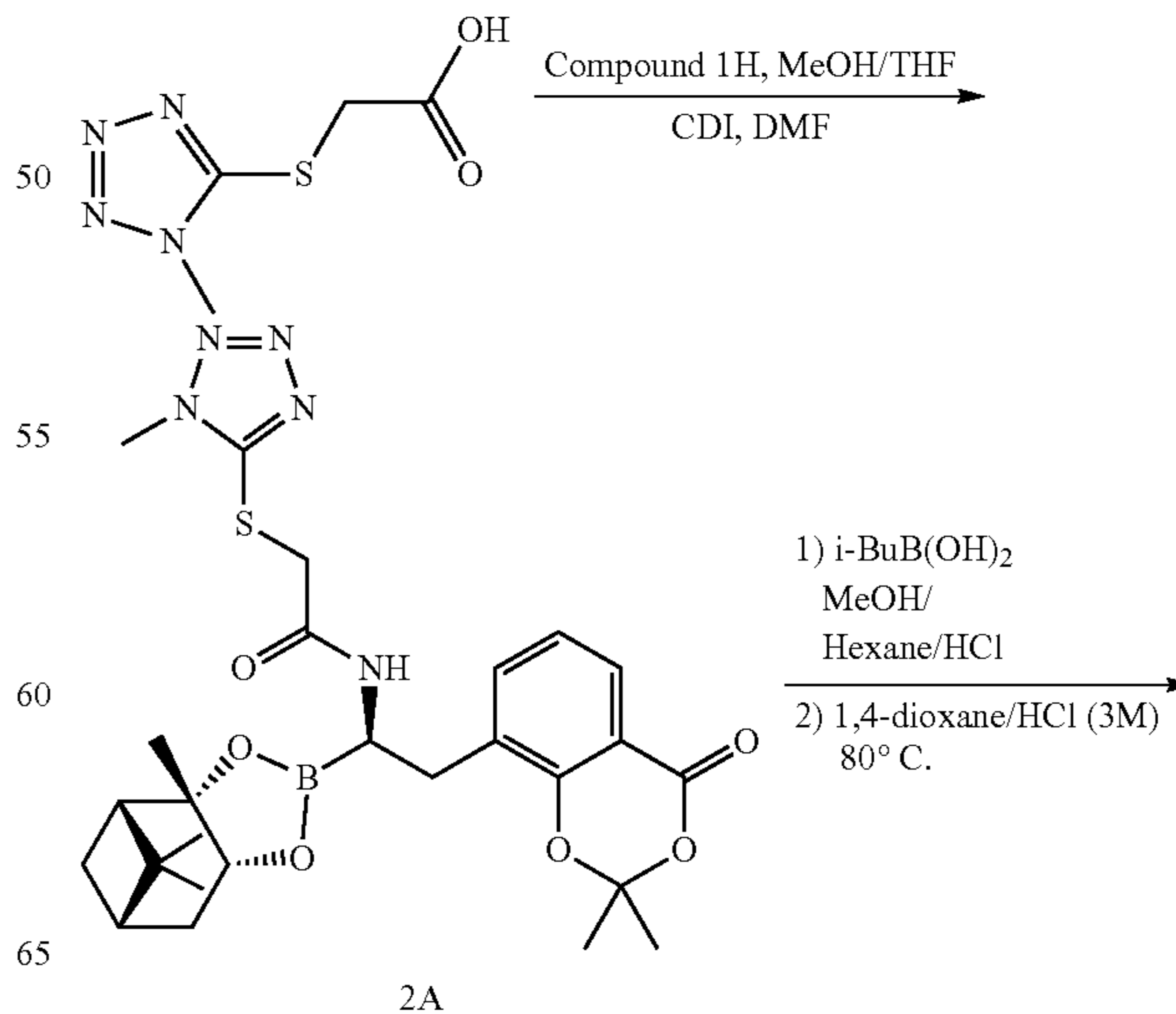
Scheme 5:
