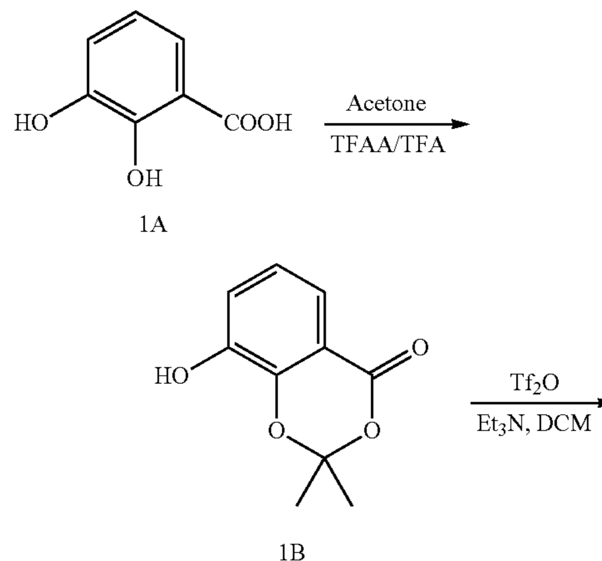
Scheme 3:
