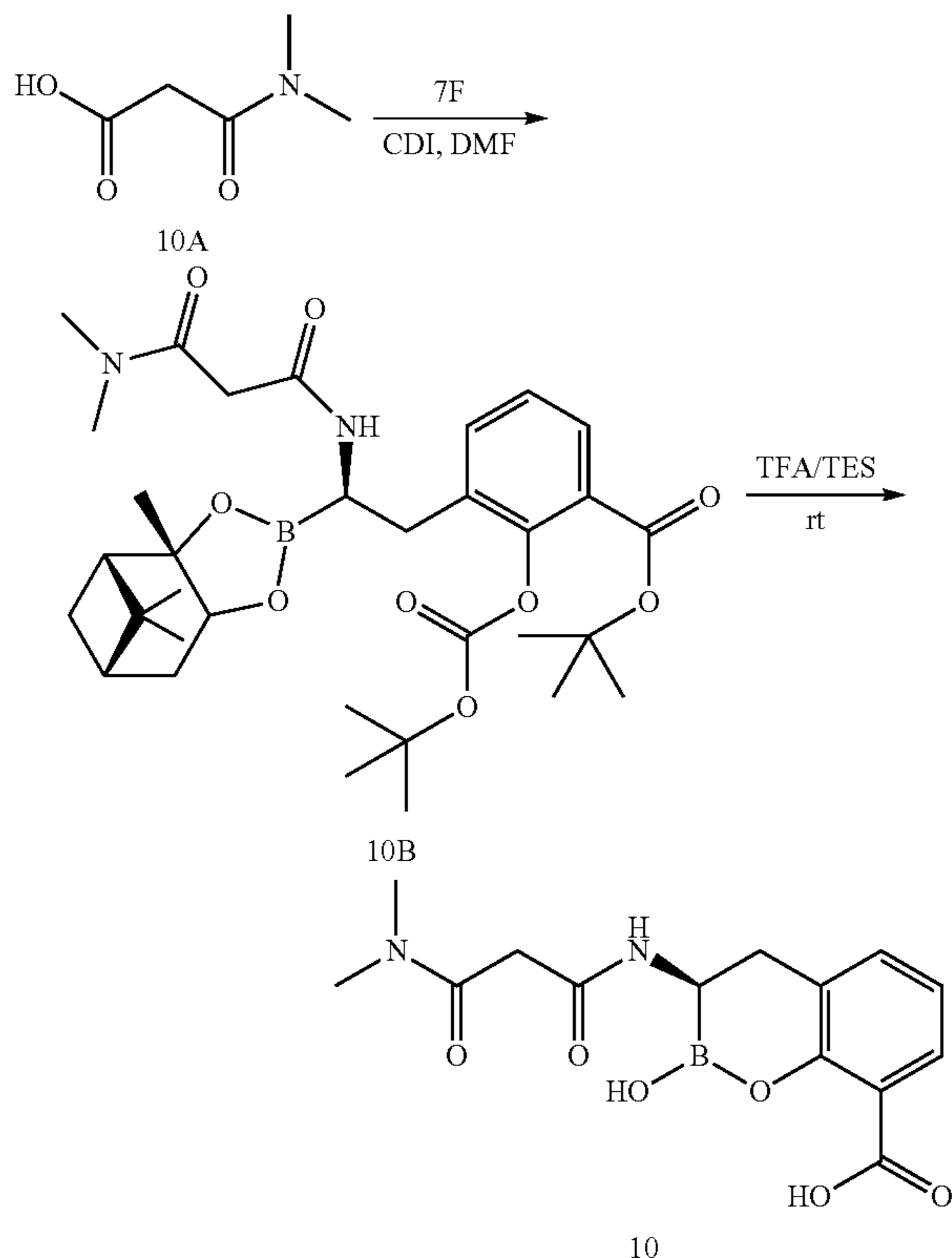
Scheme 13:
