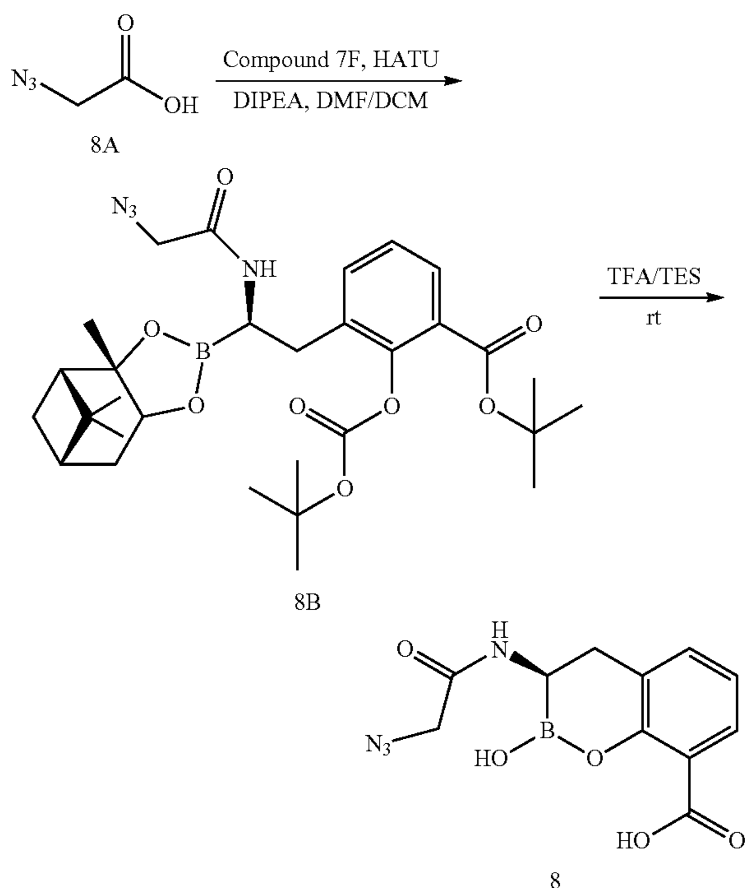
Scheme 11:
