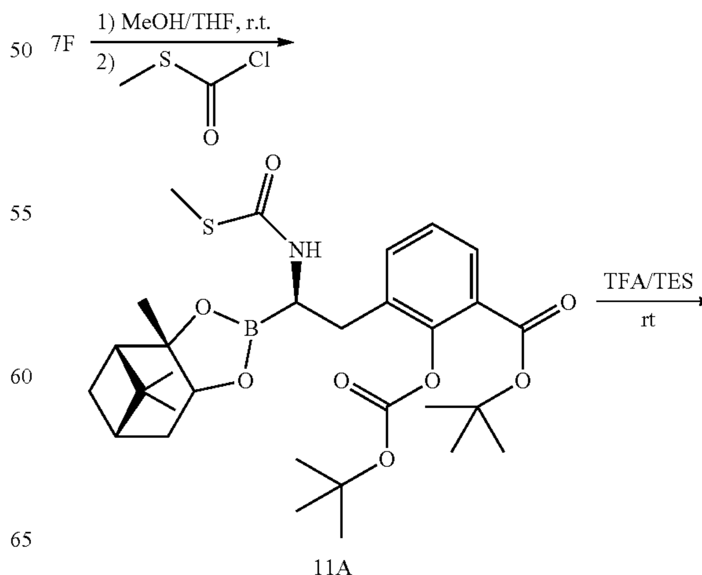
Scheme 14:
