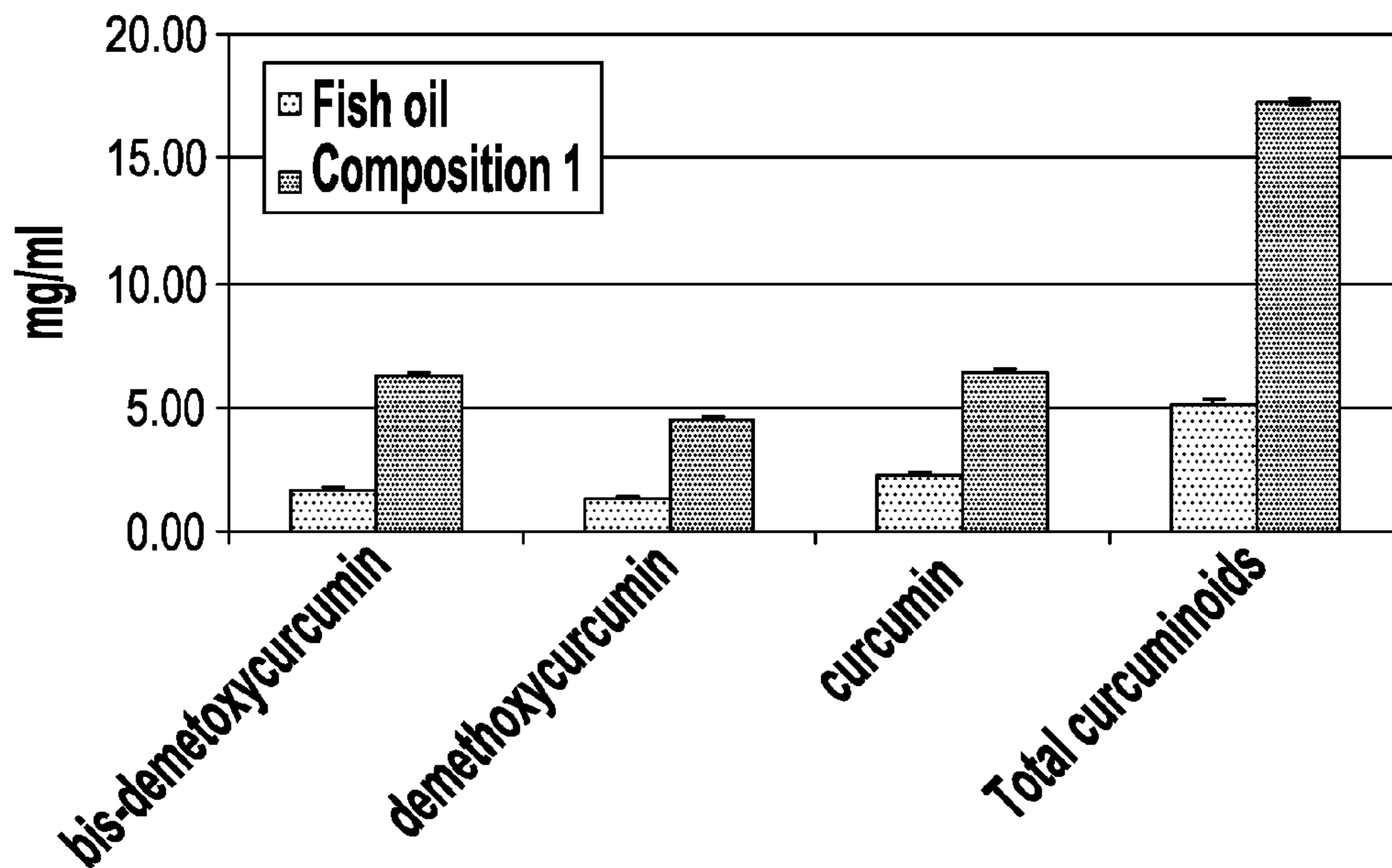
Curcuminoids solubility
