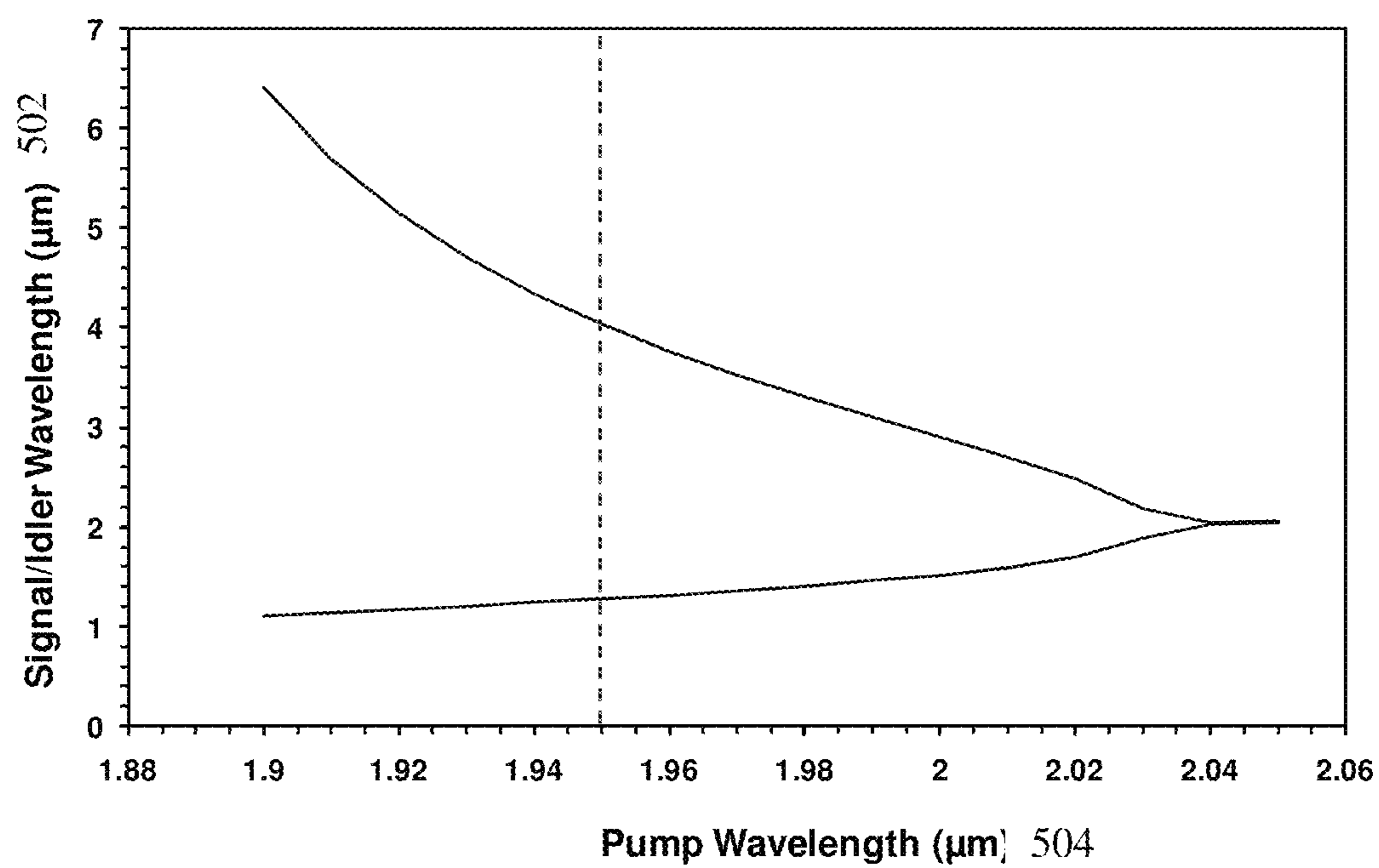
Phase matching curve for the \text{As}_2\text{S}_3 PCF with \Lambda = 3 \mu\text{m} and d/\Lambda = 0.3
