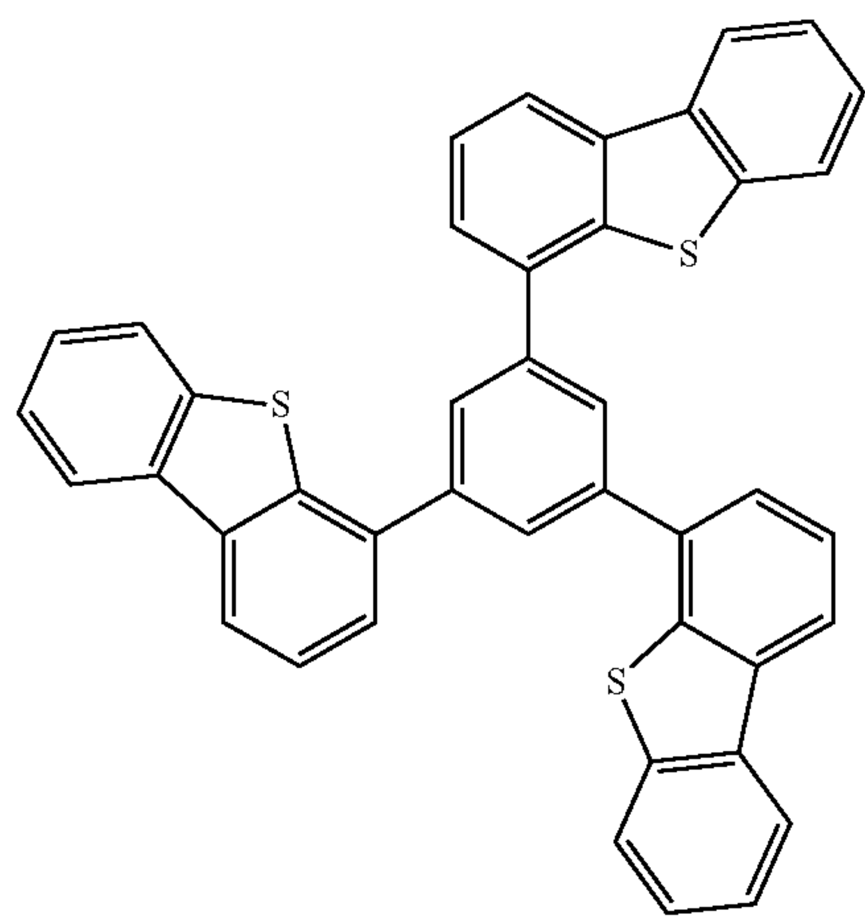
DBT3P-II
