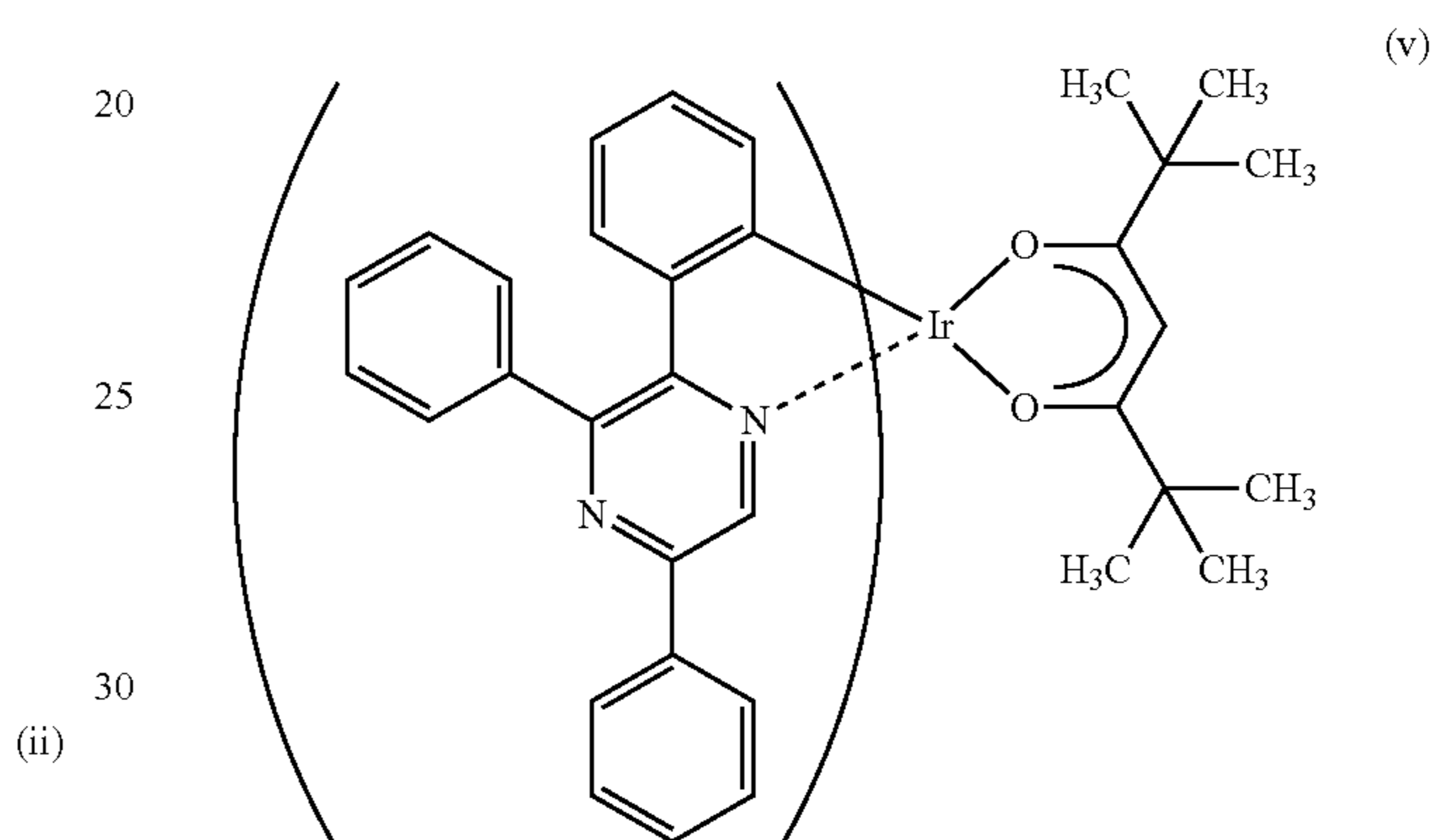
Ir(tppr) 2 (dpm)
