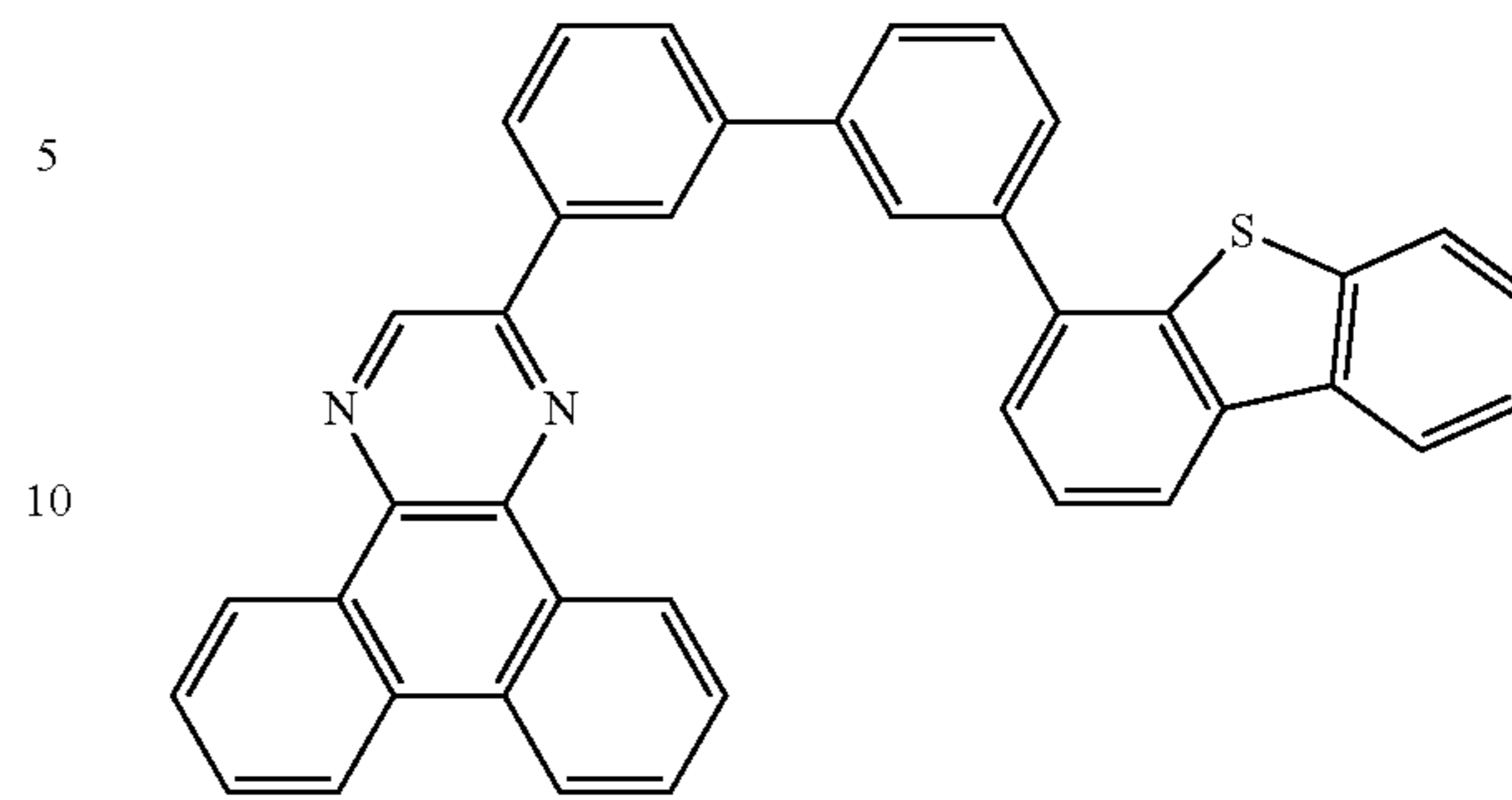
2mDBTBPDBq-II
