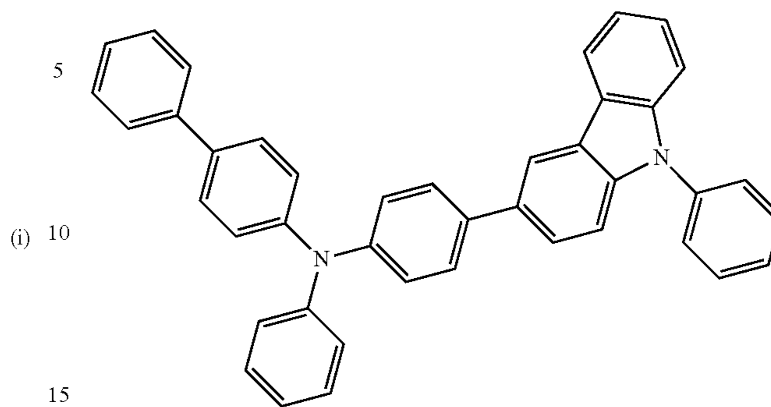
PCBA1BP
