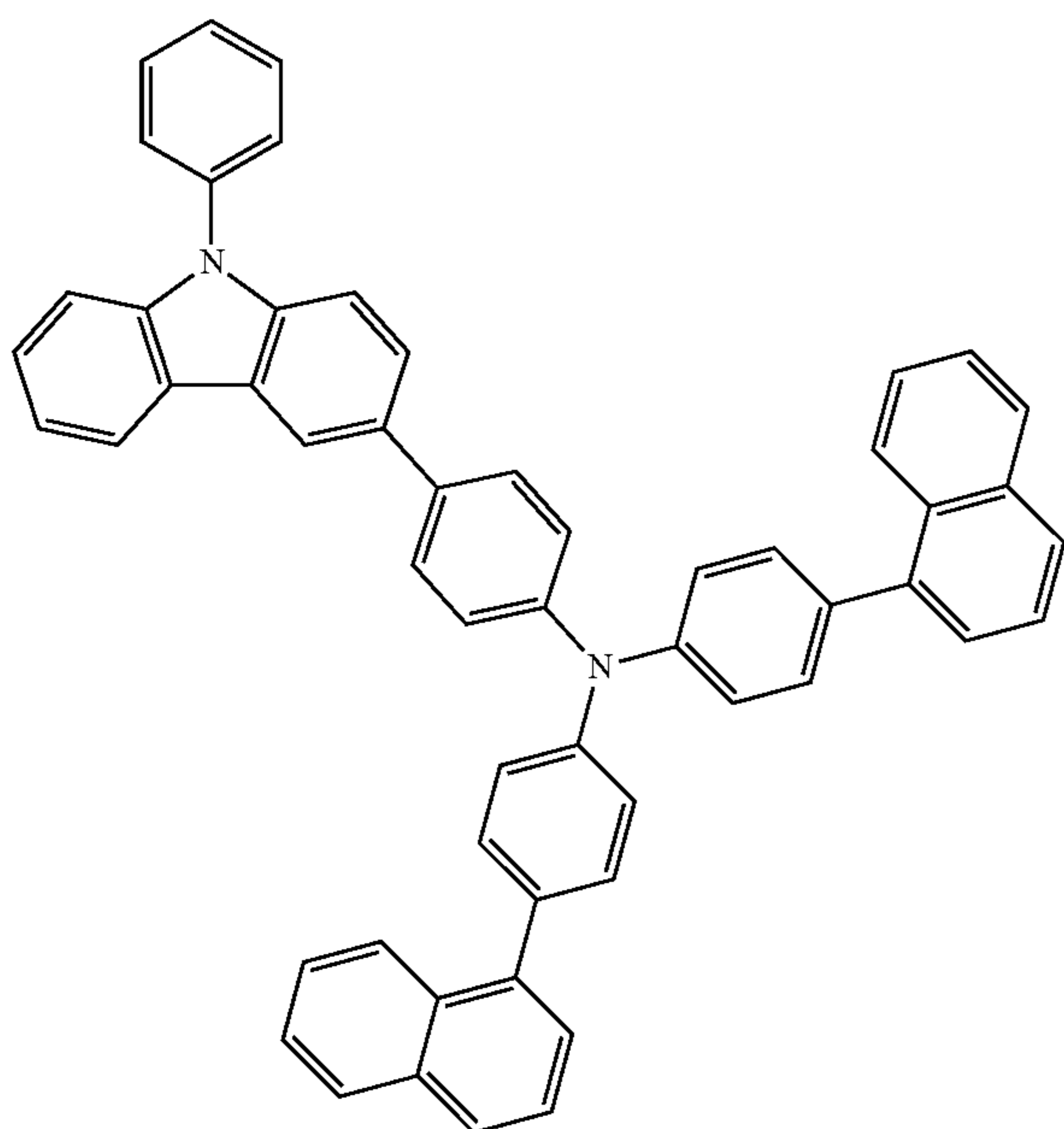
PCBNBB
