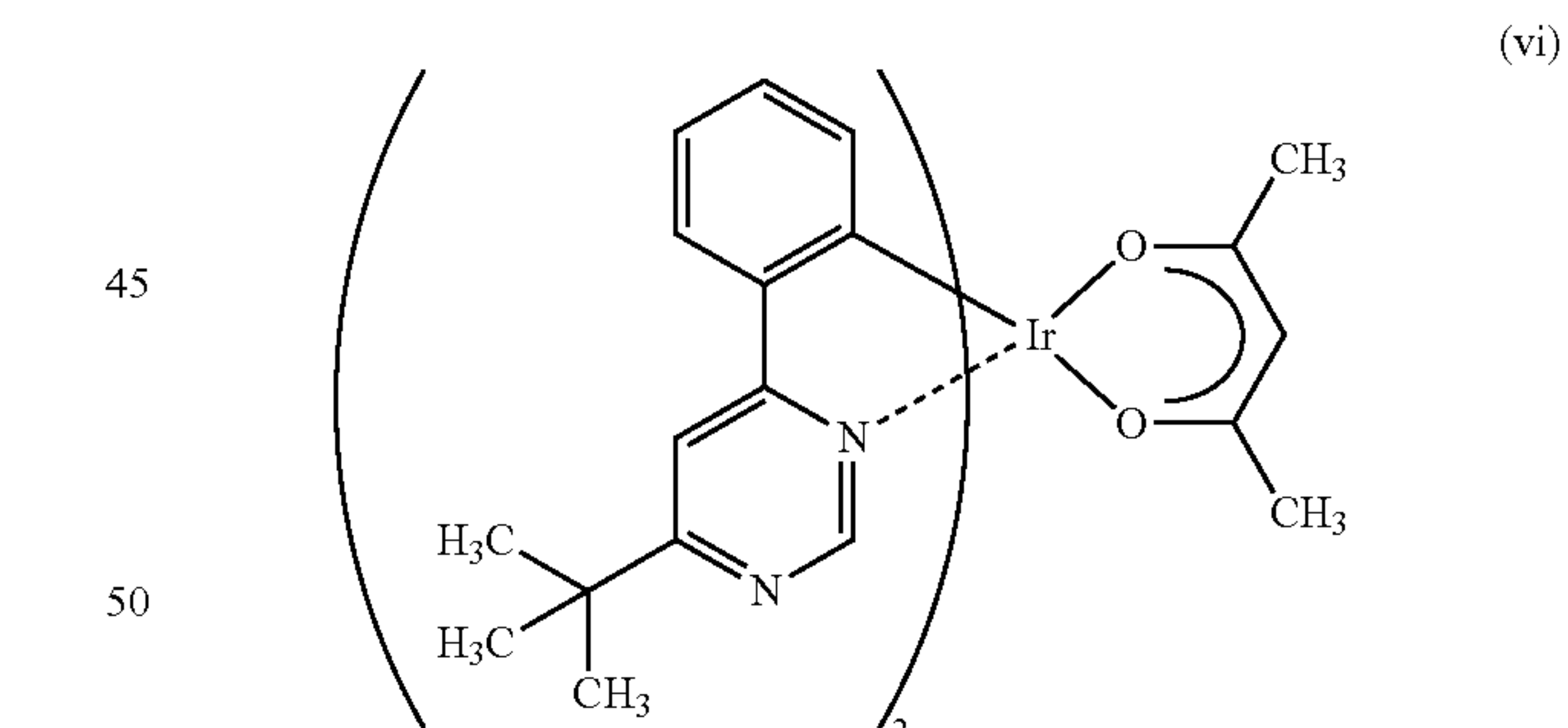
Ir(tBuppm) 2 (acac)
