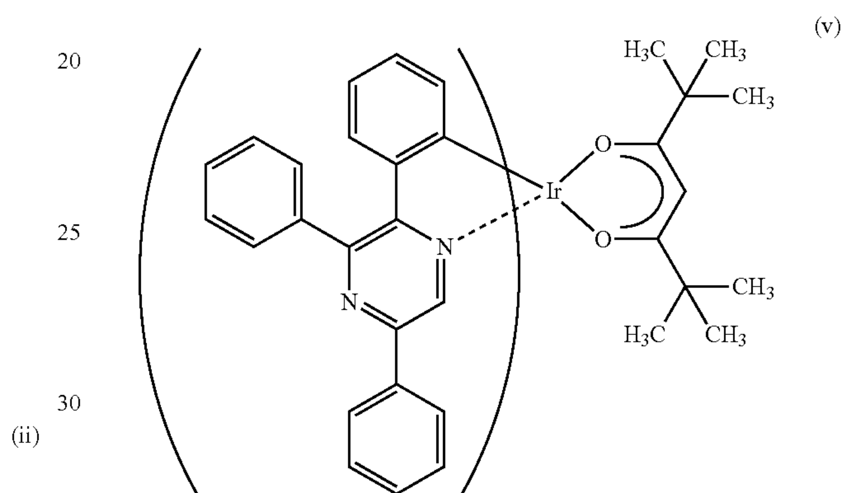
Ir(tppr) 2 (dpm)
