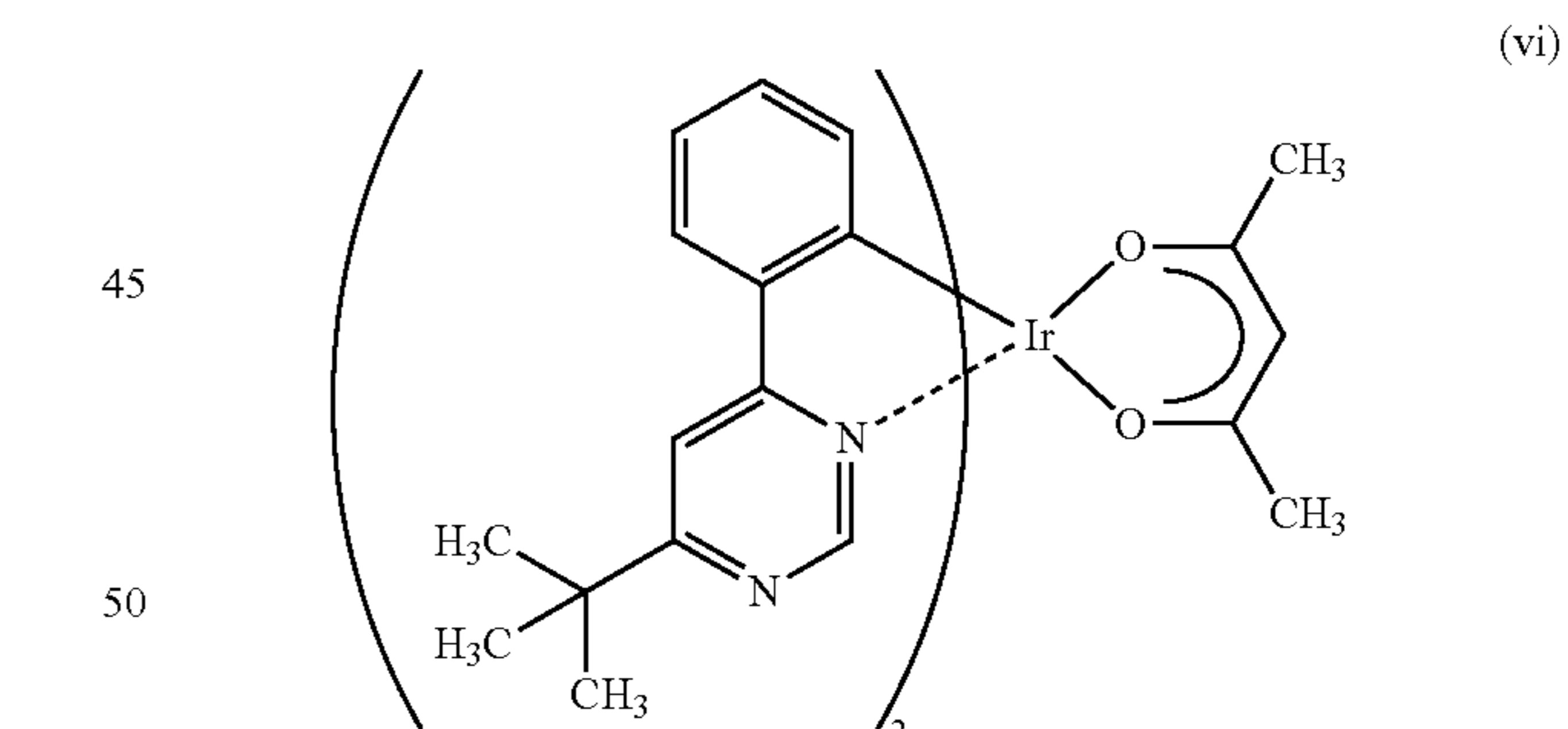
Ir(tBuppm) 2 (acac)
