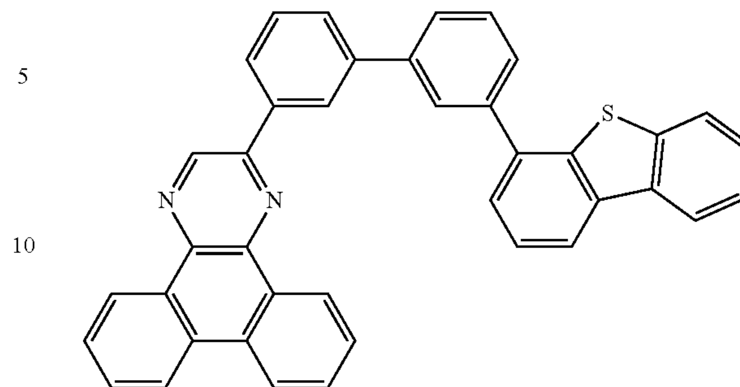
2mDBTBPDBq-II
