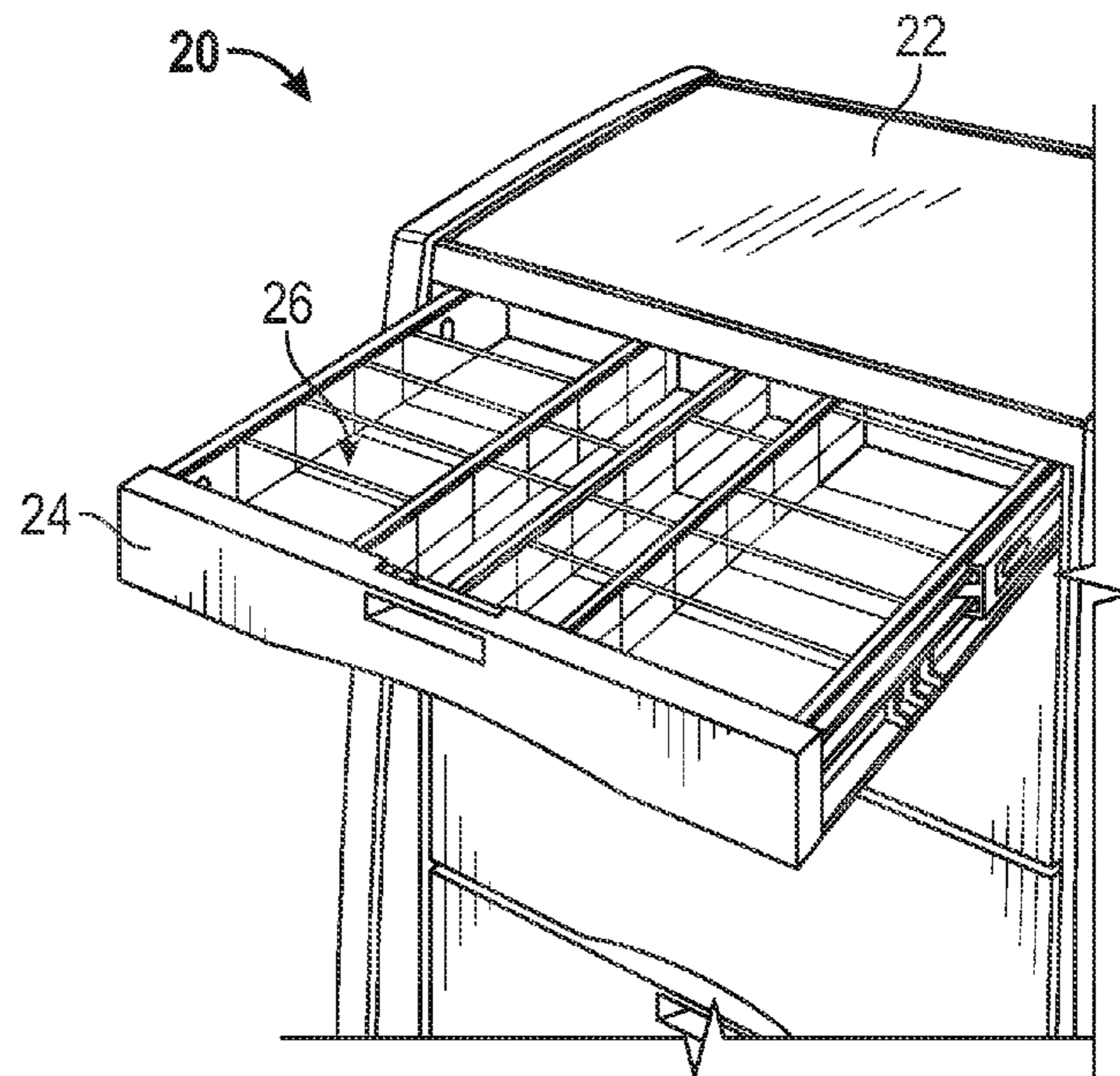
FIG. 1 (Prior Art)
