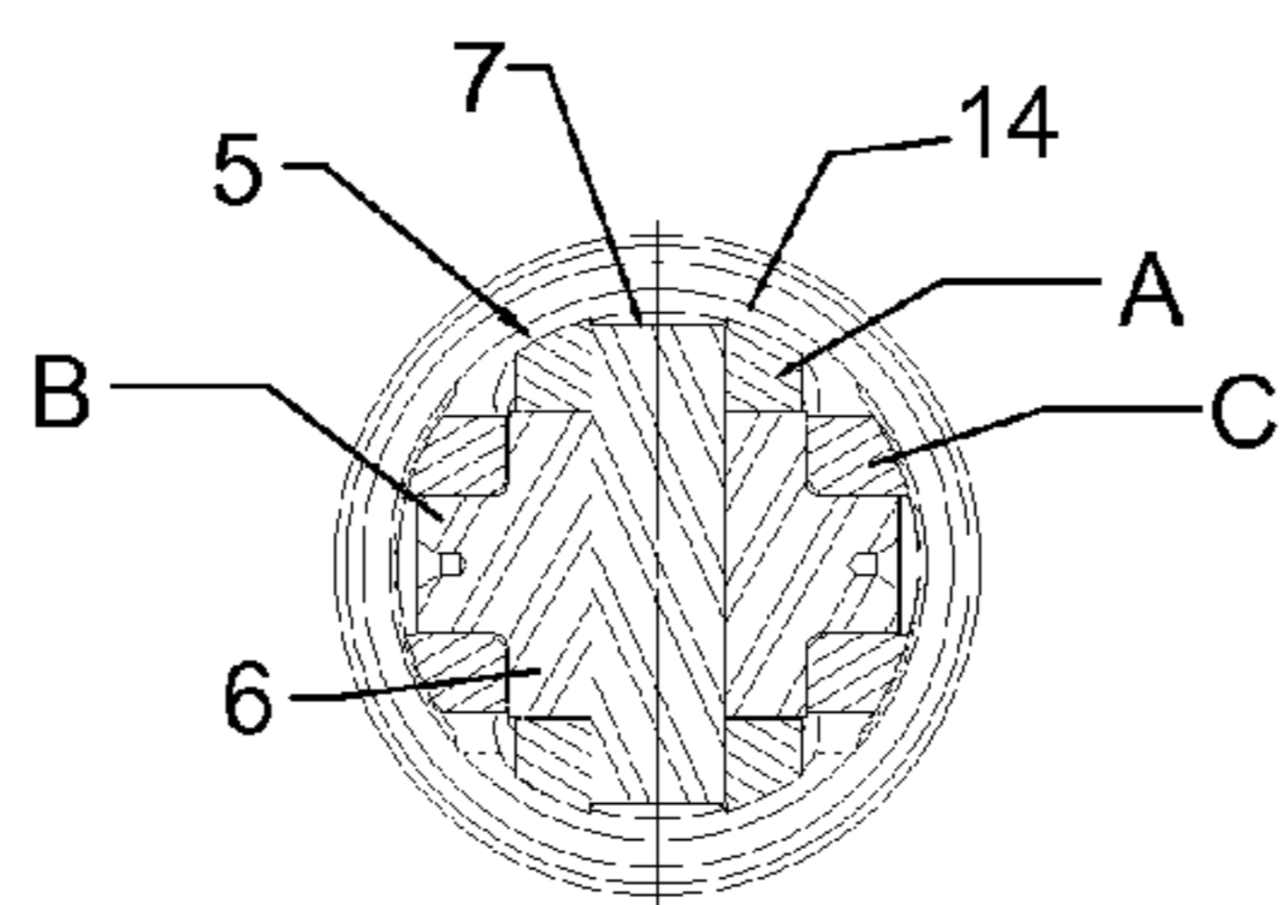
SECTION 1A-1A
