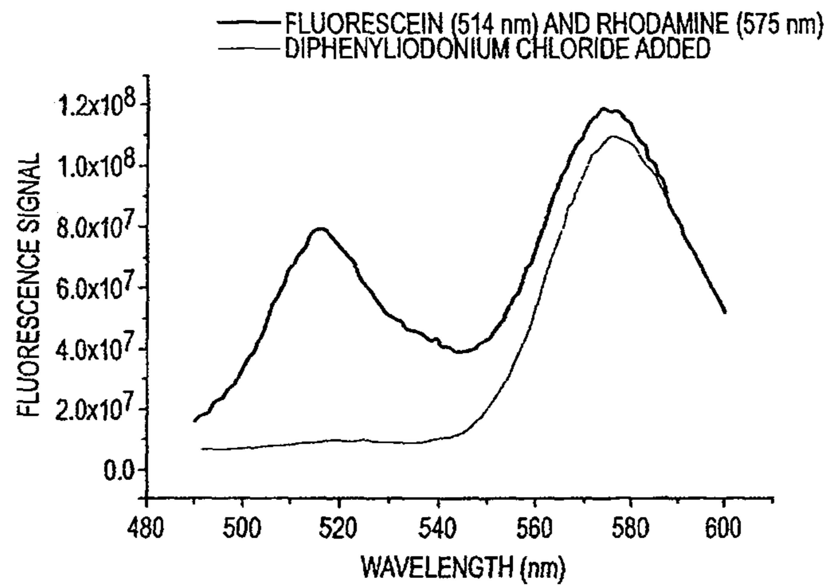
FLUORESCENCE SPECTRA OF EQUIMOLAR FLUORESCIN AND TETRA METHYLRHODAMINE BEFORE AND AFTER ADDITION OF DIPHENYLIODONIUM CHLORIDE
