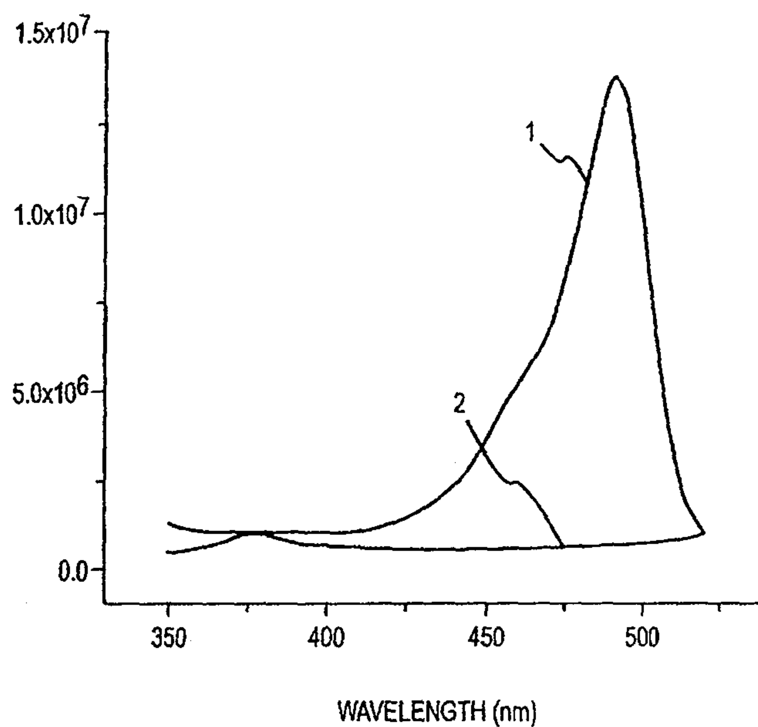
UV ABSORPTION SPECTRA: (1) FLUORESCIN (2) FLUORESCIN + DPI AFTER SINGLE FLASH FROM CAMERA STROBE
