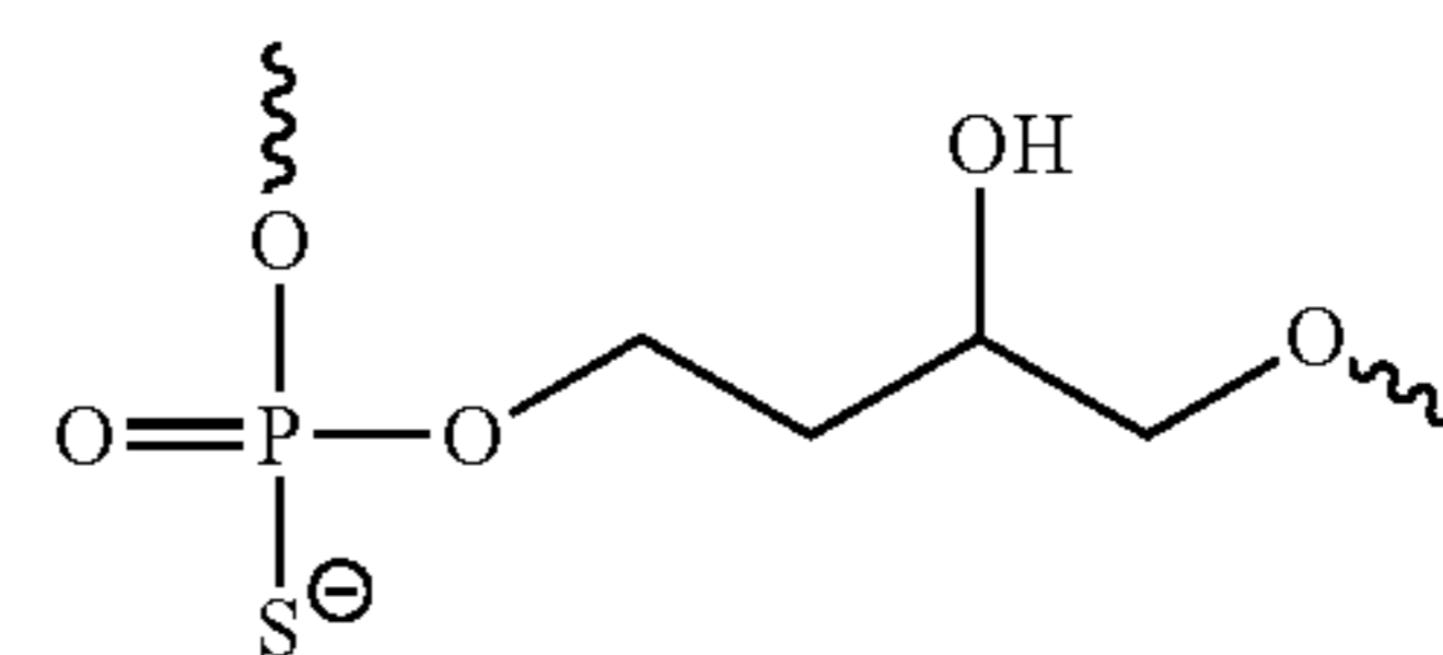
1,2,4-Butanetriol Linker
