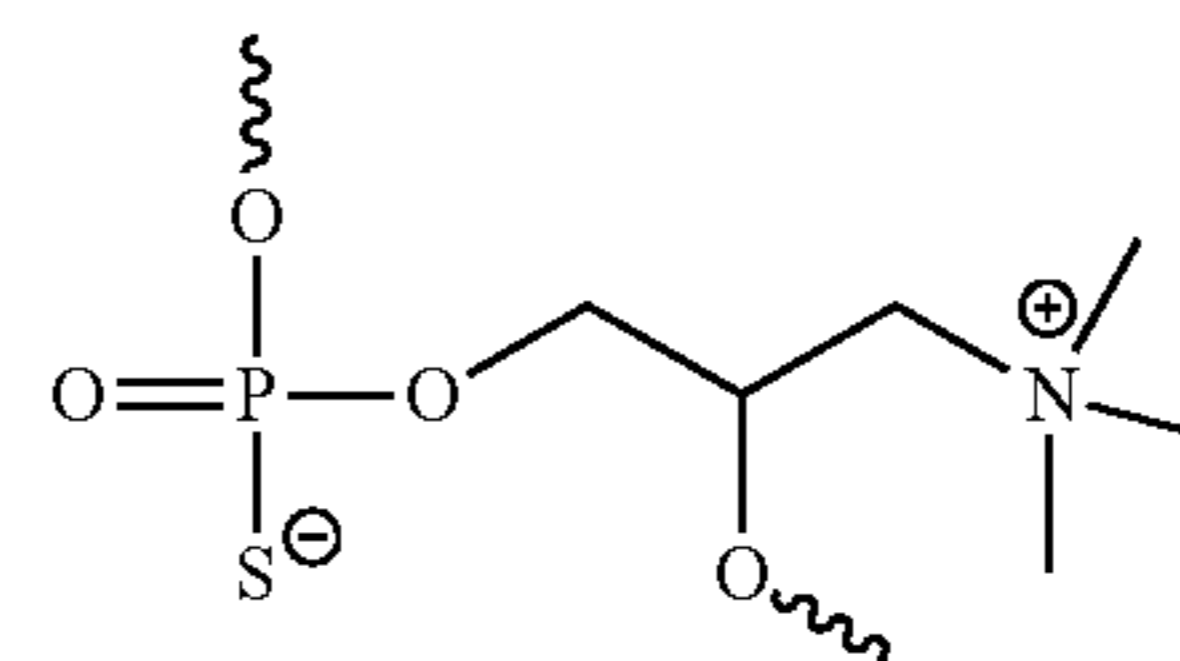
3-Trimethylamino-1,2-propanediol Linker
