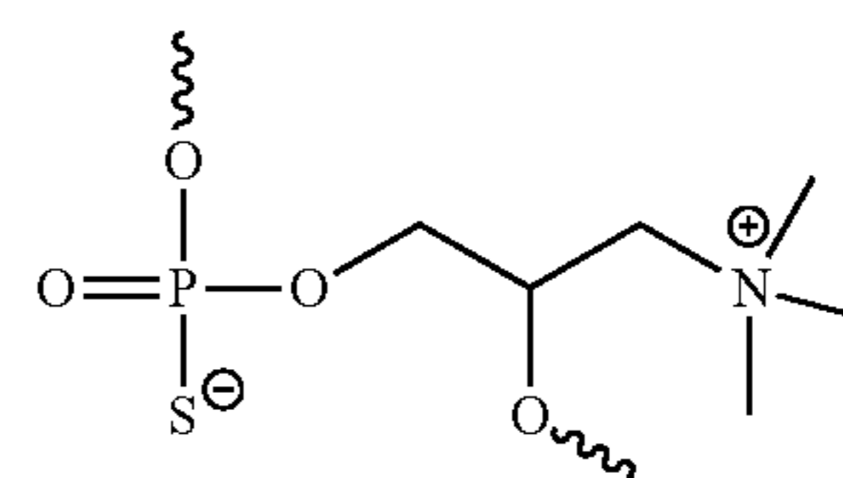
3-Trimethylamino-1,2-propanediol Linker
