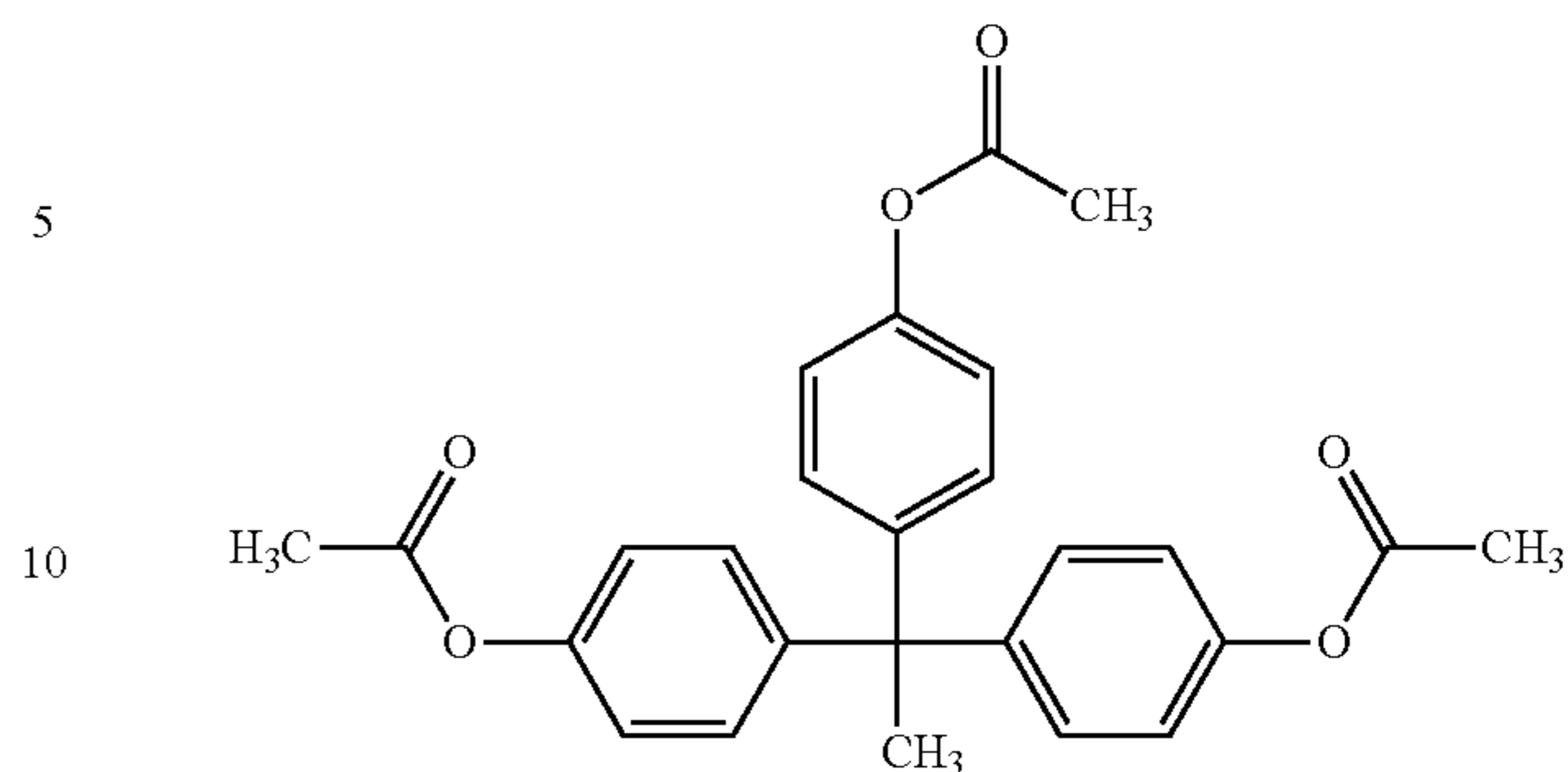
1,1,1-Tris-(4-acetoxyphenyl)ethane (I-9)
