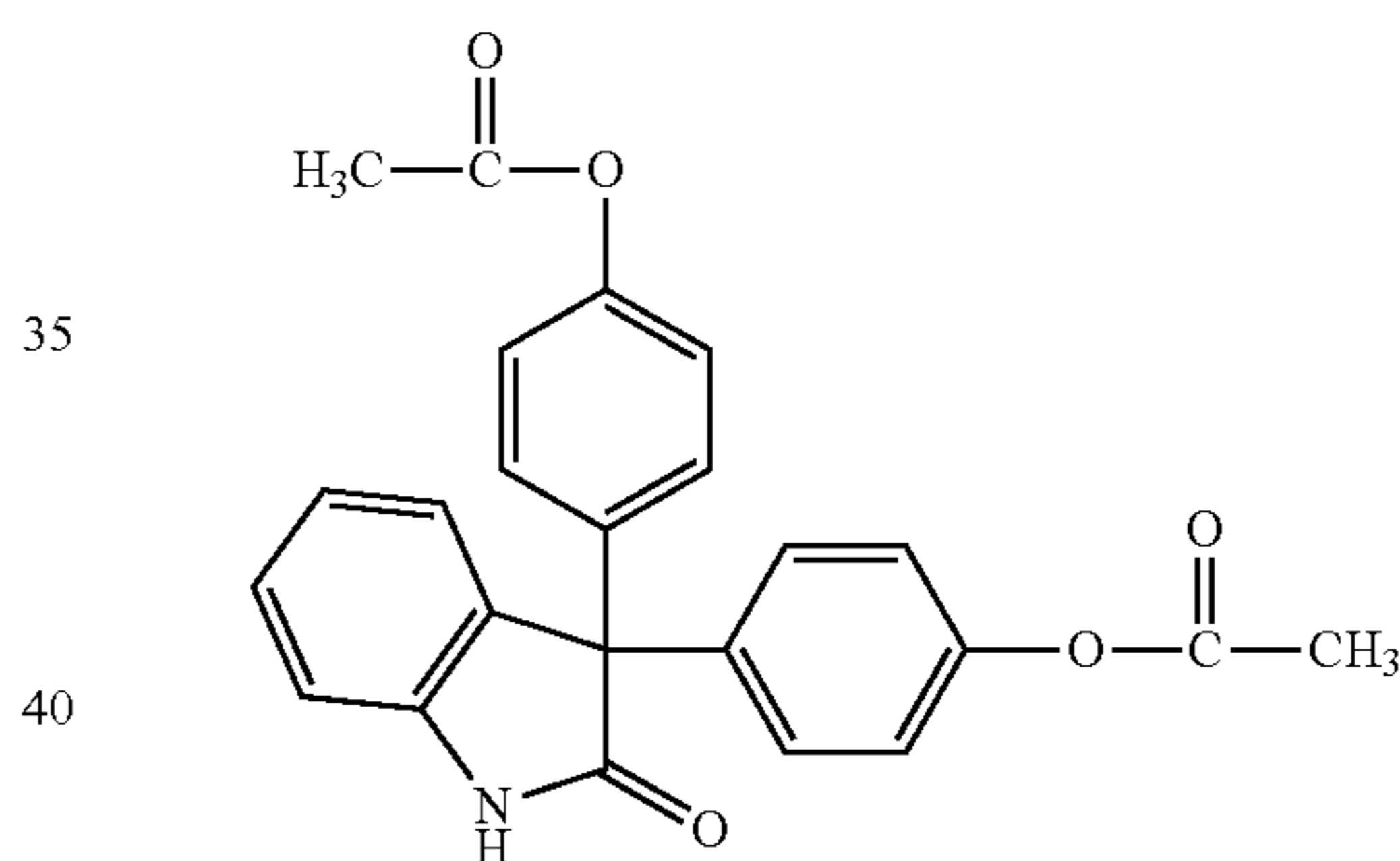
3,3-Bis[4-(acetyloxy)phenyl]-1,3-dihydro-2H-indol-2-one (I-16)
