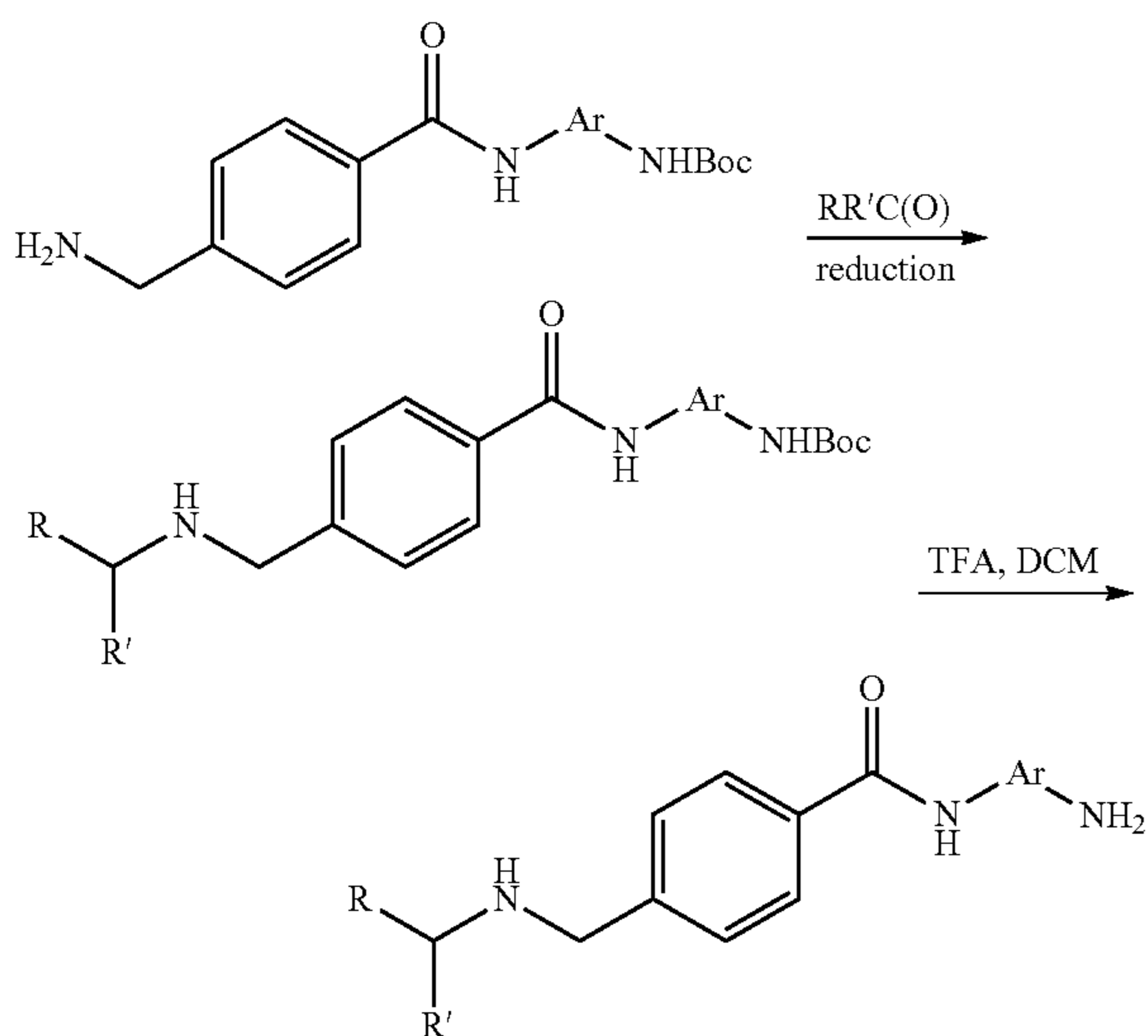
Scheme 11
