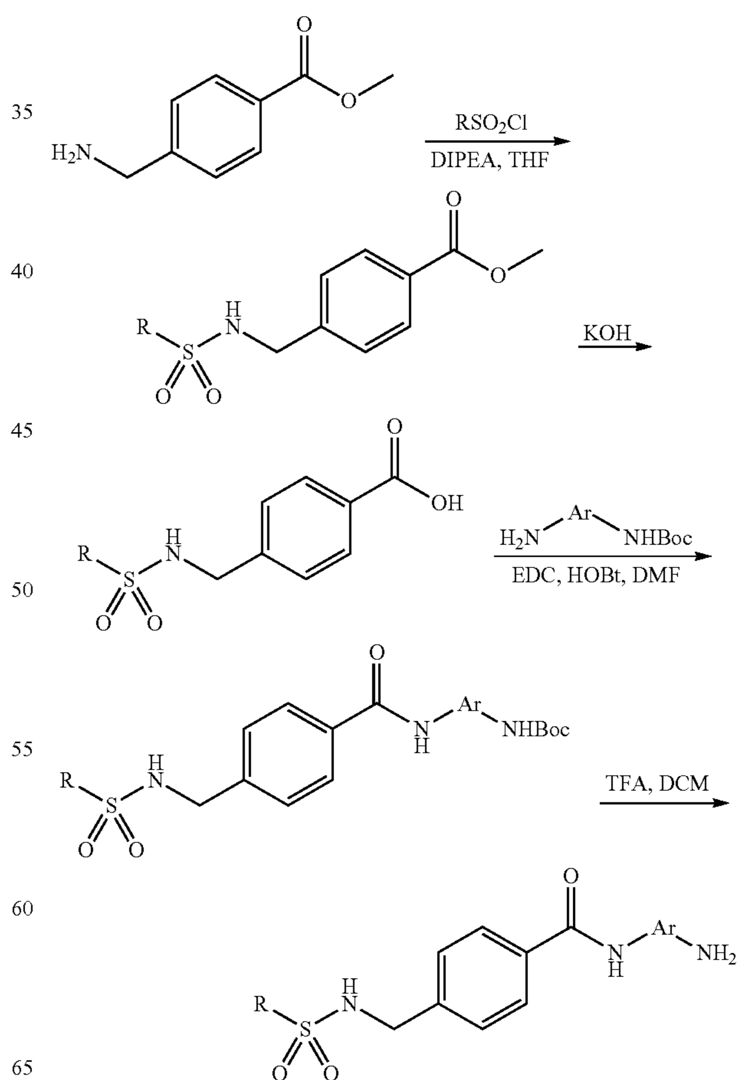
Scheme 5
