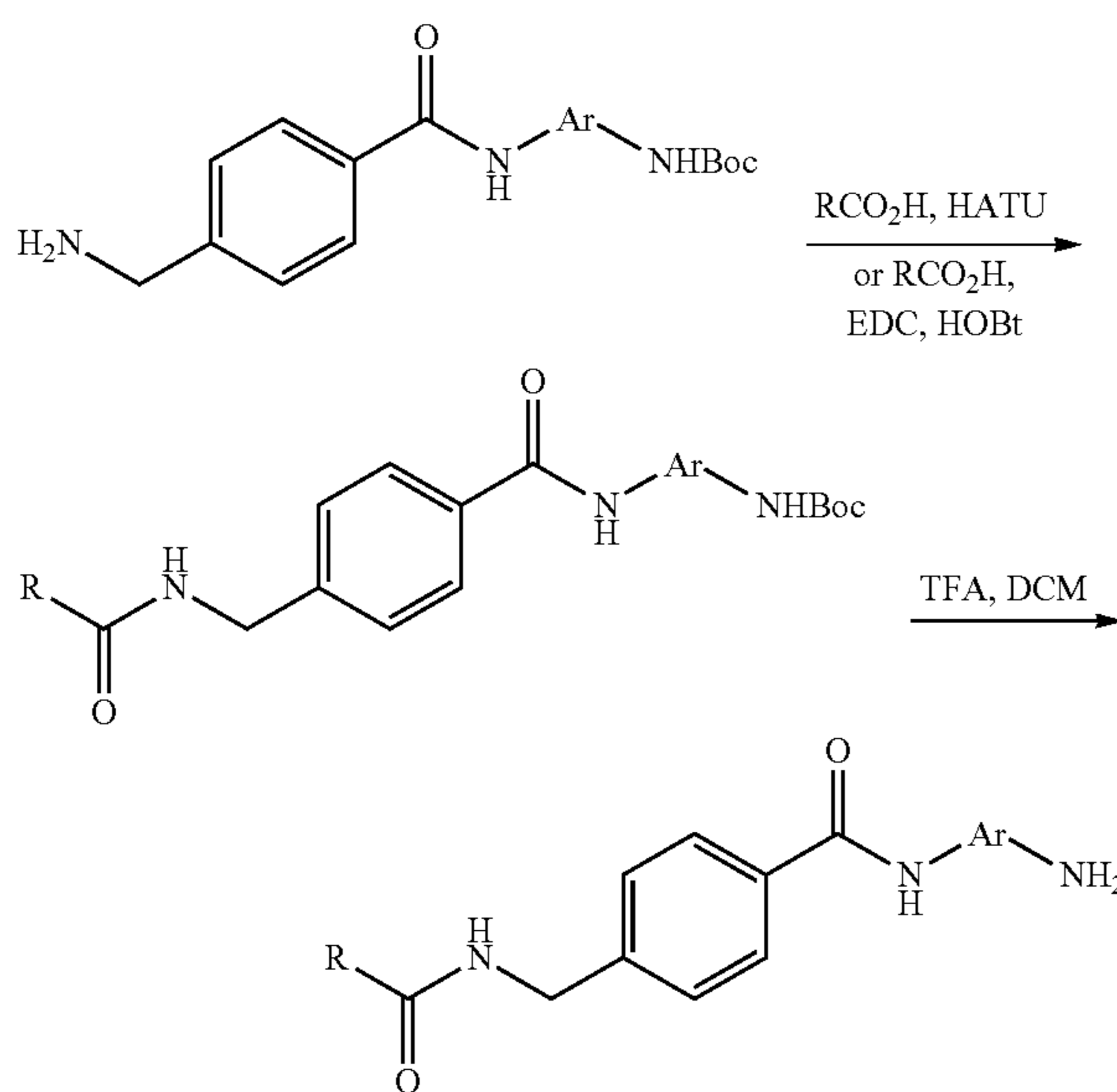
Scheme 3
