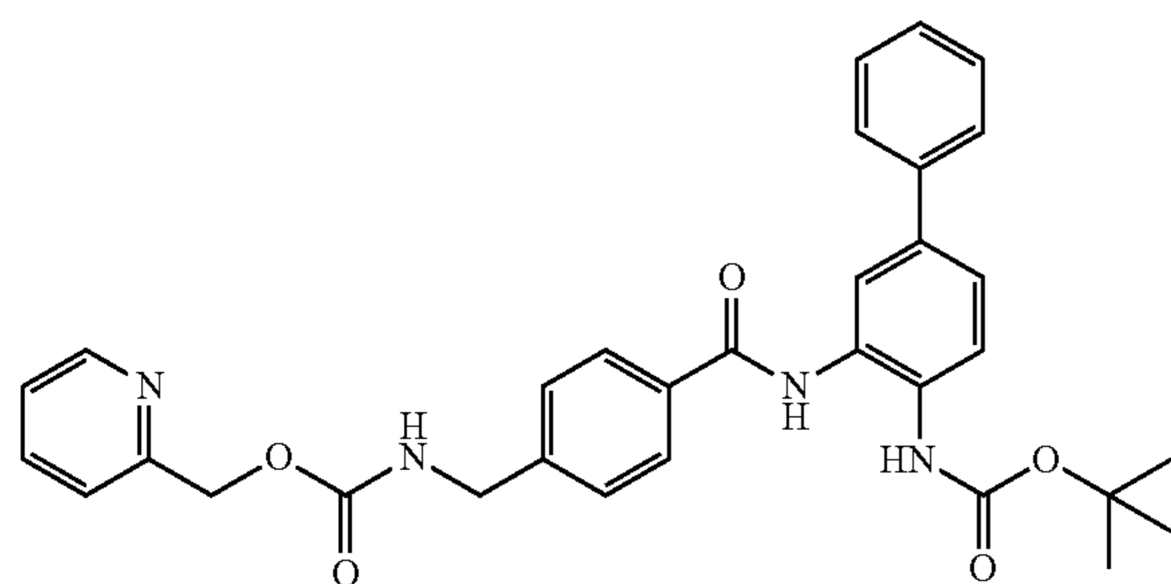
1,1-dimethylethyl {3-[(4-(((pyridin-2-ylmethyl)oxy)carbonyl)amino)methyl]phenyl}carbonyl amino]biphenyl-4-yl} carbamate
