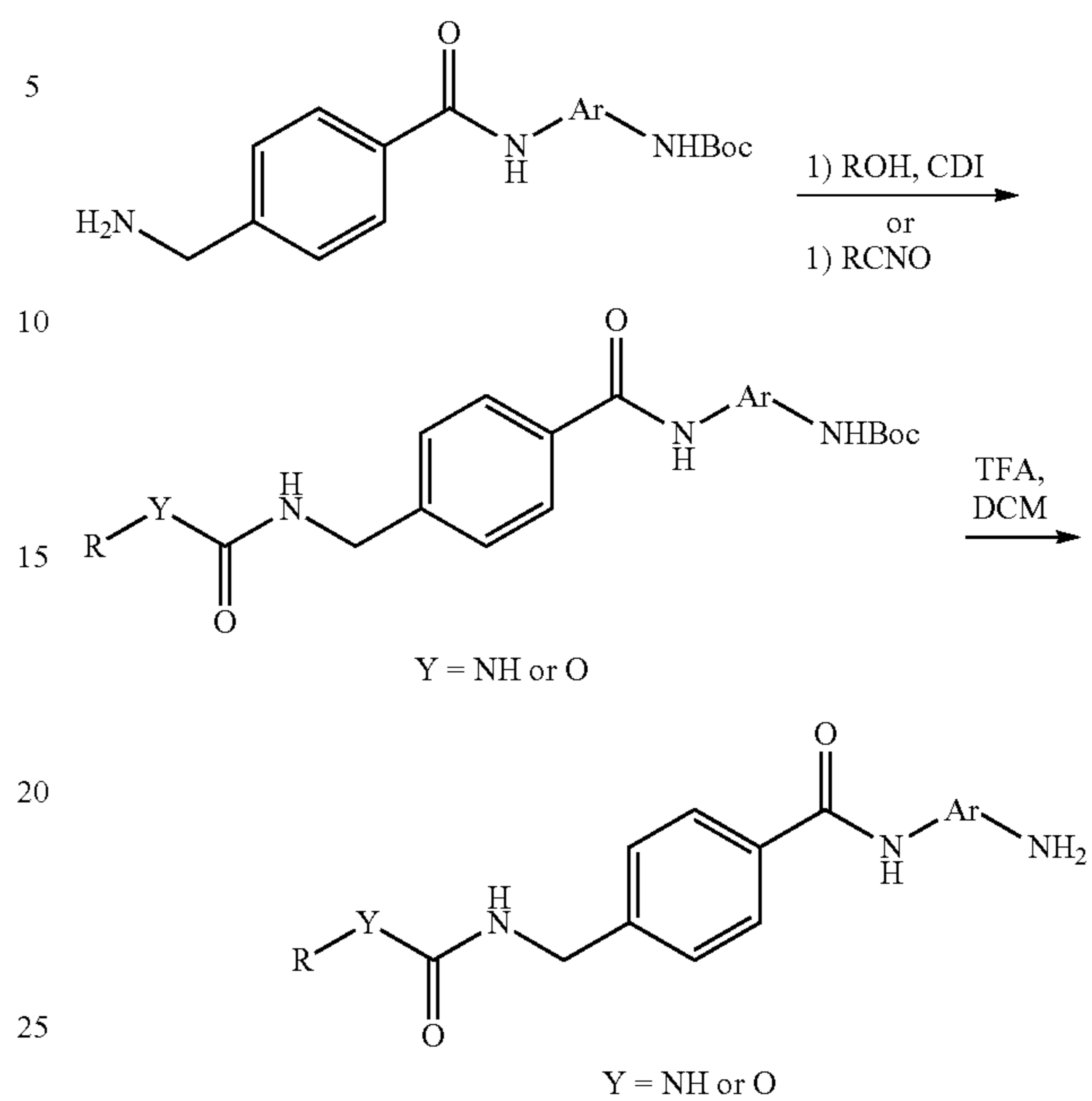
Scheme 4
