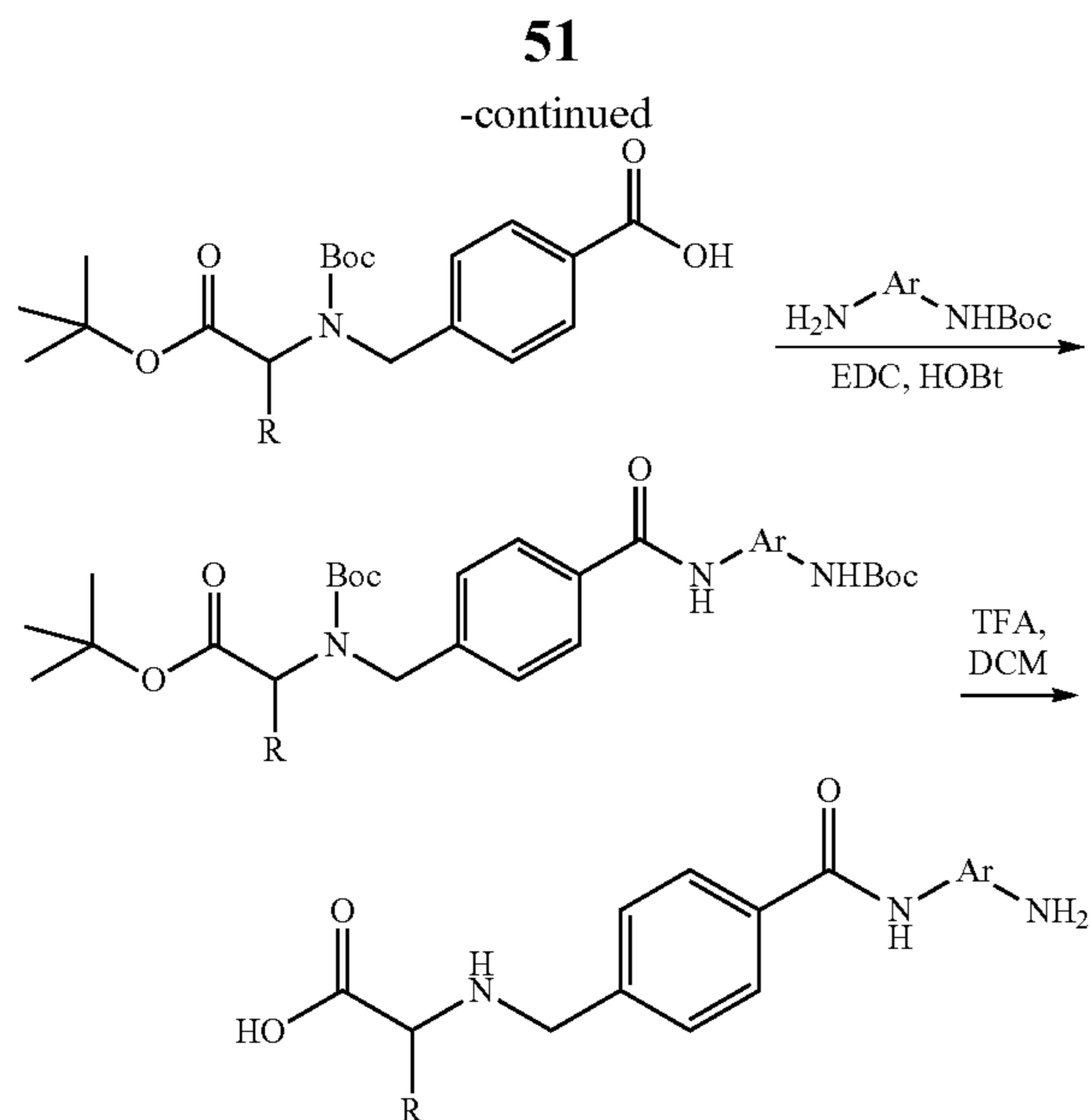
Scheme 11
