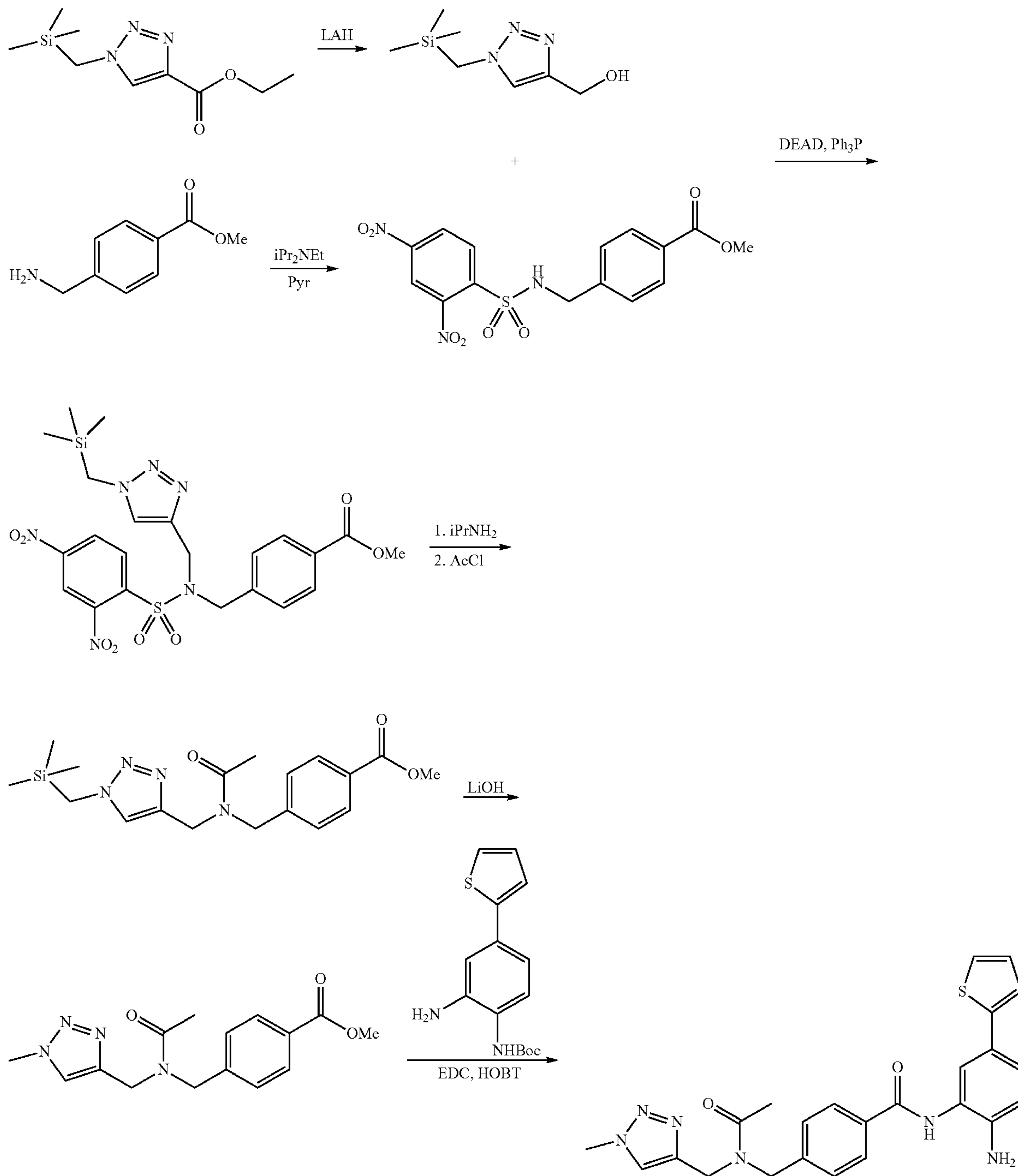
Scheme 9
