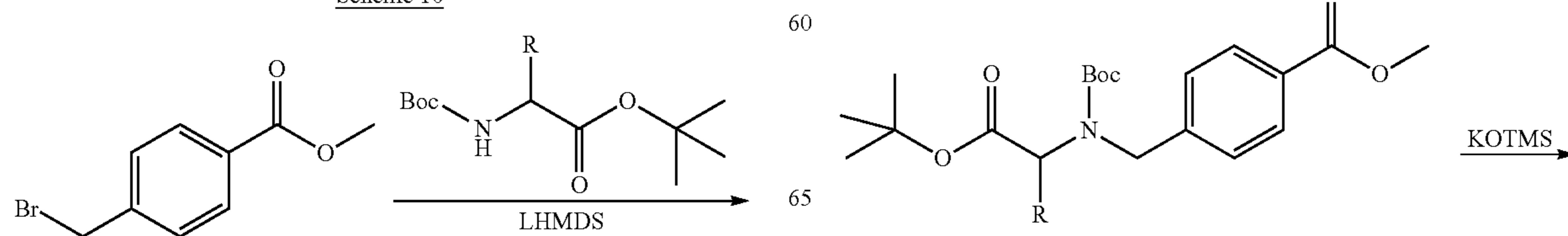
Scheme 10
