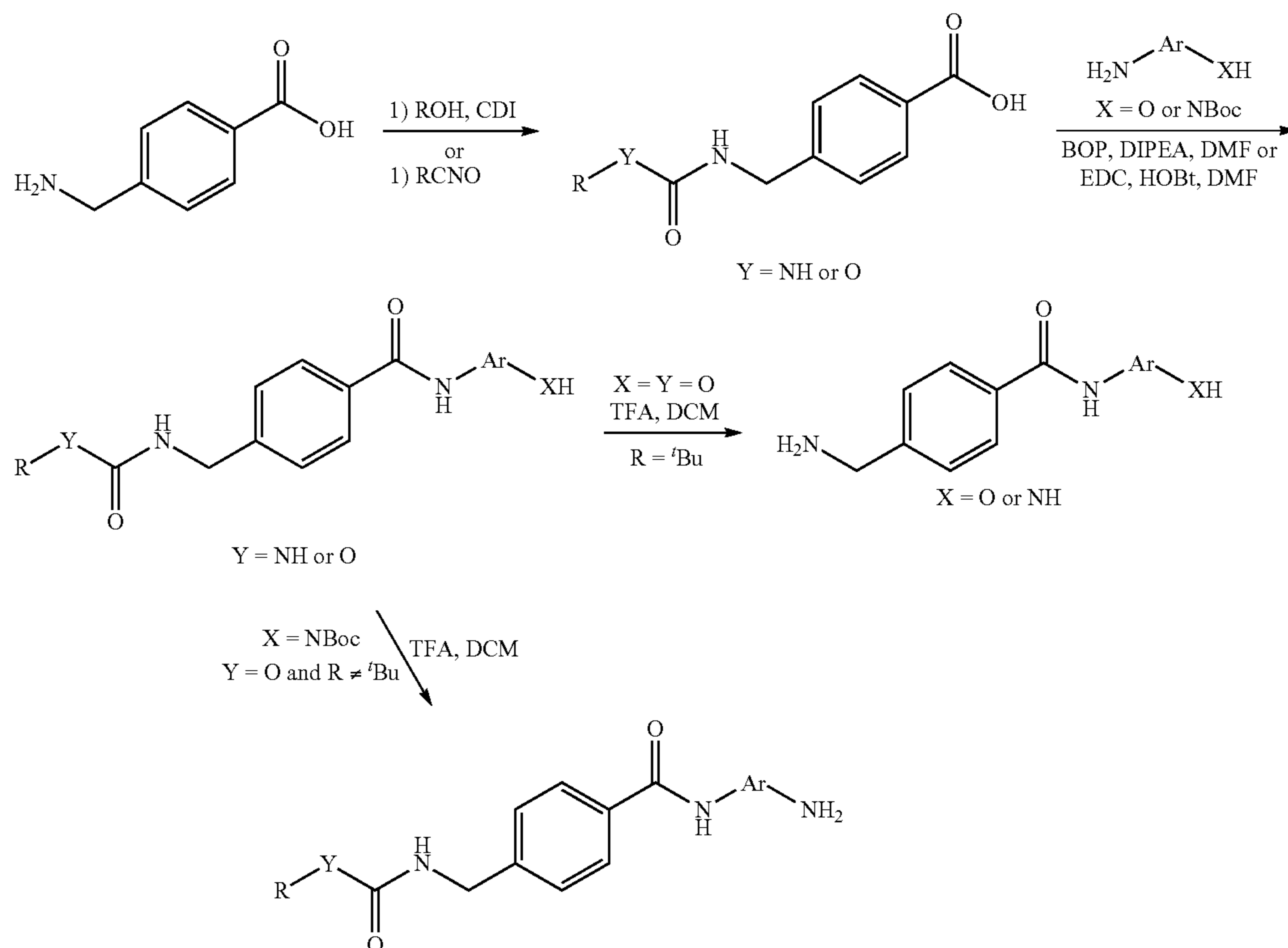
Scheme 1
